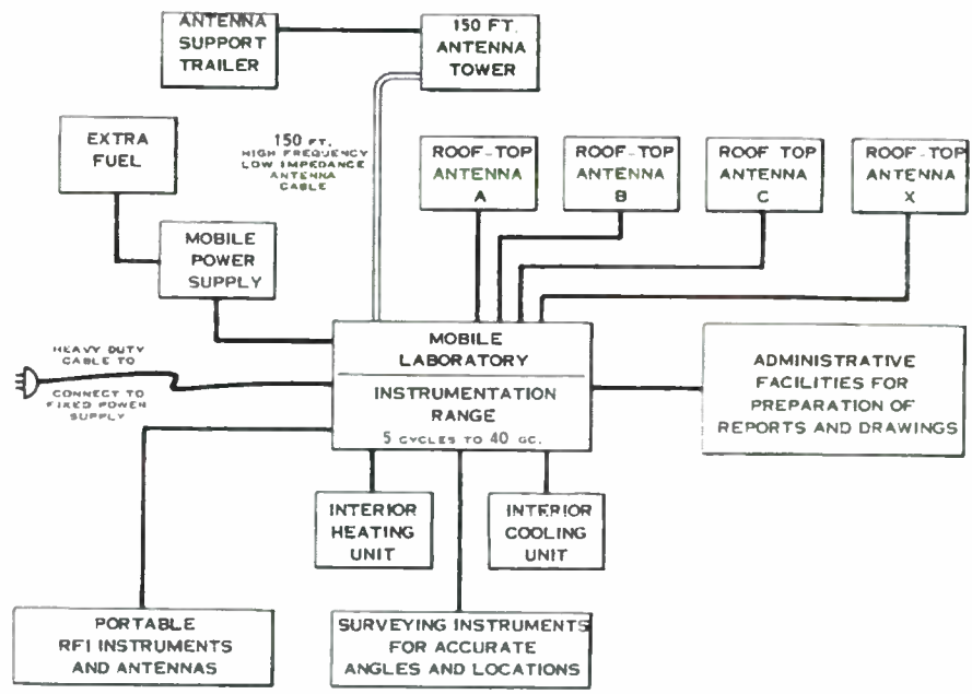
Figure 3-4. Block Diagram of Major Items in Mobile RF Laboratory
