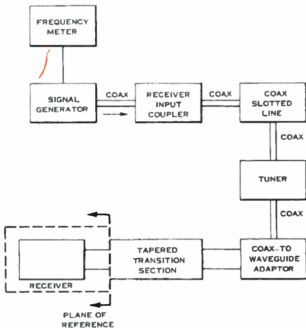
Figure 7-27. Test Setup For Spurious Response Tests
