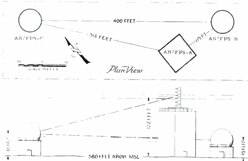
Figure 7-2. Profile Showing Propagation Path Between the Three Radars
