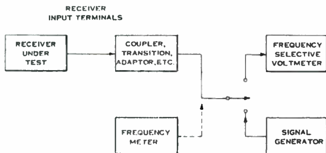
Figure 7-41. Receiving Radiation-Measurement Block Diagram
