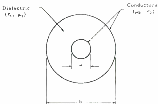
Figure 2-14. Coaxial Cable Parameters
