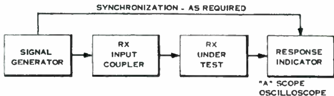
Figure 7-22. Test Setup for Radar Receiver Sensitivity Tests
