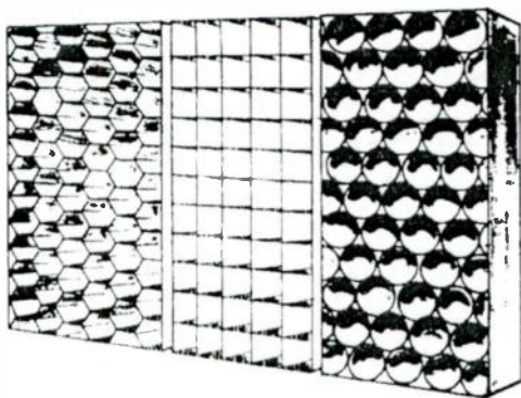
Figure 5-2 Waveguide-Below-Cut Off Type of Ventilation Grids for Shielded Enclosures (SHIELDING IN RIVINGTON N. J.)
