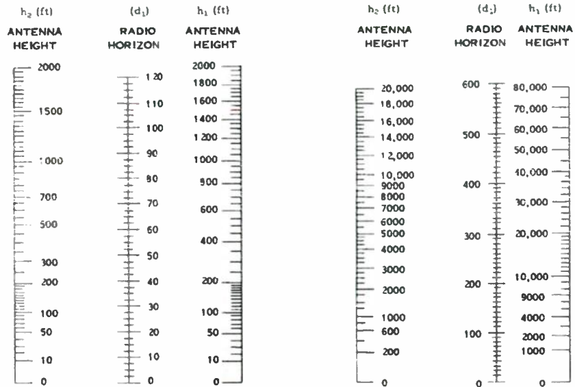
Figure 2-21. Nomographs Giving Radio Horizon Distance
