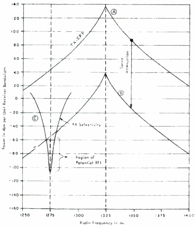
Figure 7-32. Typical RFI Situation (Adjacent Channel Interference Shown)
