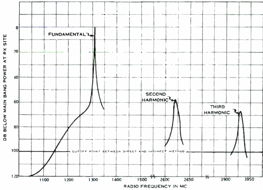
Figure 7-8. Sample L-Band Radar Transmitter Spectral Signature. Measured in Far Field
