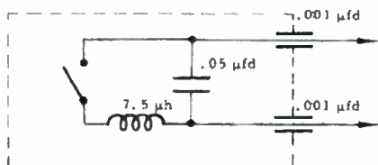
Figure 3-53. Suppression Circuit
