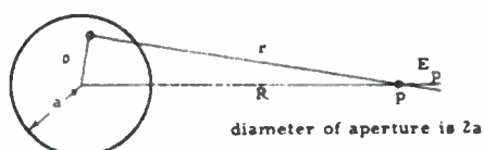
Figure 6-1. Geometry for Calculating the Fresnel Region Fields of a Circular Aperture
