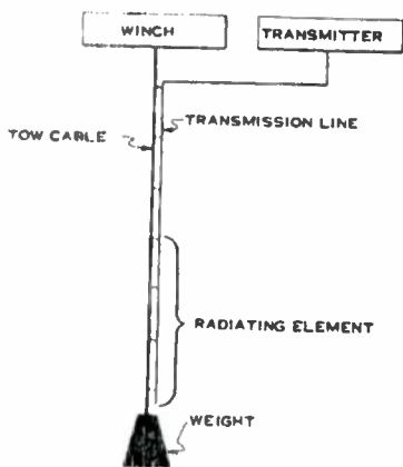
Figure 3-12. Vertical Polarization
