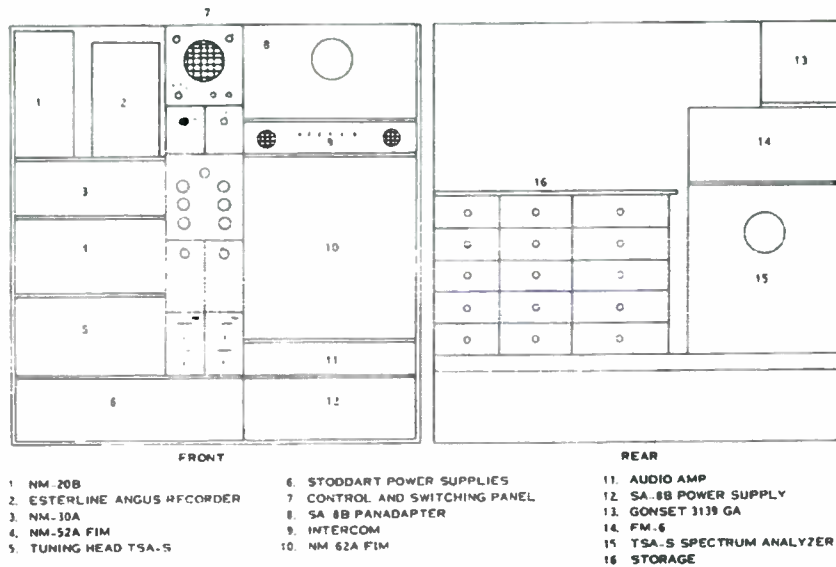
Figure 3-1. Layout of Van Interior
