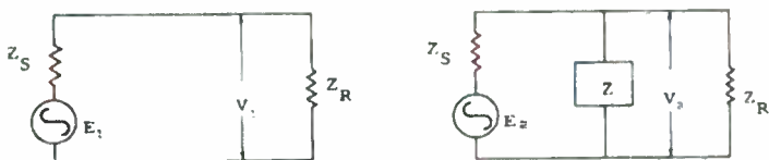
Figure II-1. Equivalent Circuits Used In the Derivation of the Insertion-Loss Ratio
