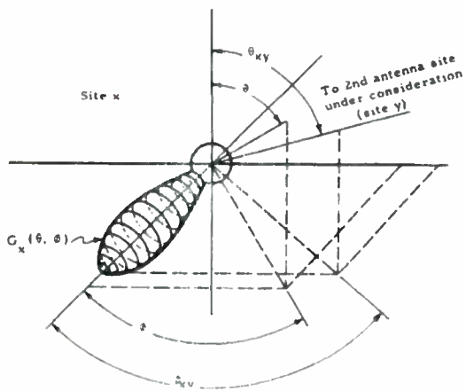
Figure 2-12. Three Dimensional Antenna Pattern Considerations
