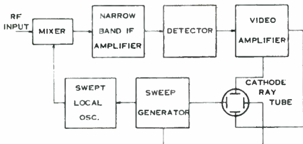
Figure 4-10. Simplified Block Diagram of a Spectrum Analyzer
