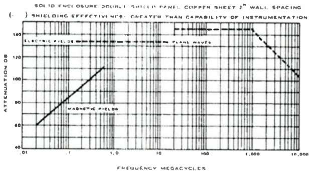
Figure 5-1. Attenuation Curve of Typical Shielded Enclosure
