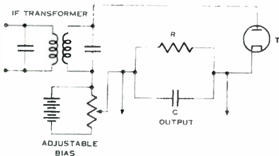
Figure 4-3. Detector With Adjustable Bias
