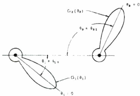
Figure 2-11. Off-Axis Pointing Geometry for Two Dimensional Case
