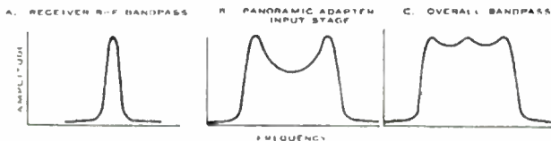
Figure 4-12. Selectivity Curves
