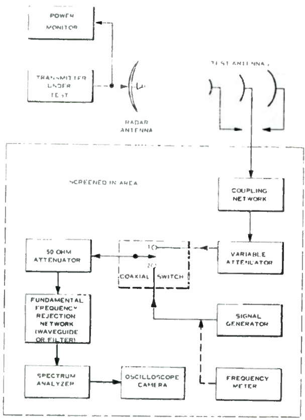
Figure 7-14. Transmitter Open-Field Emission Spectra Measurement Setup
