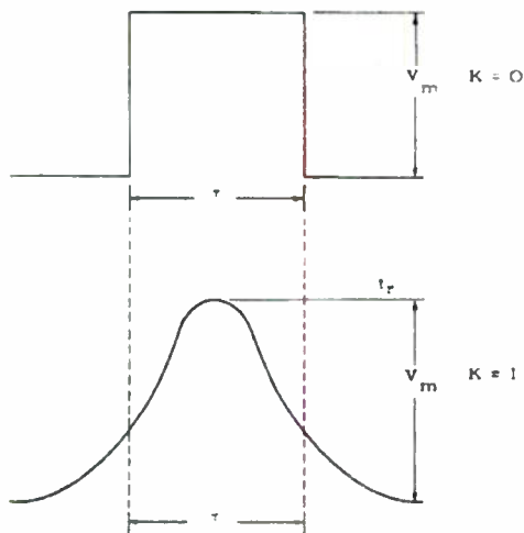
Figure 2-9. Special Pulse Shapes
