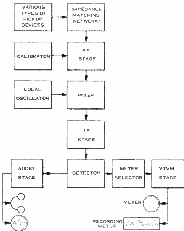
Figure 4-1. Block Diagram of a typical Radio Interference Meter
