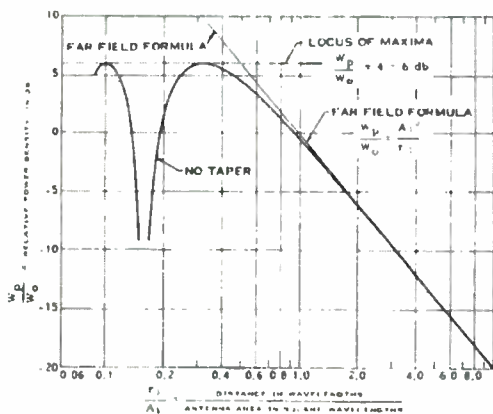
Figure 6-2. Power Density vs Distance for Uniformly Illuminated Round Aperture
