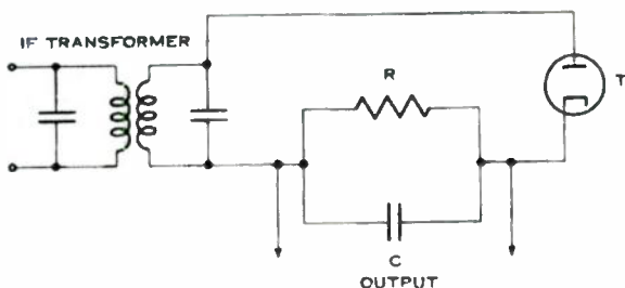
Figure 4-2. Basic Detector Circuit
