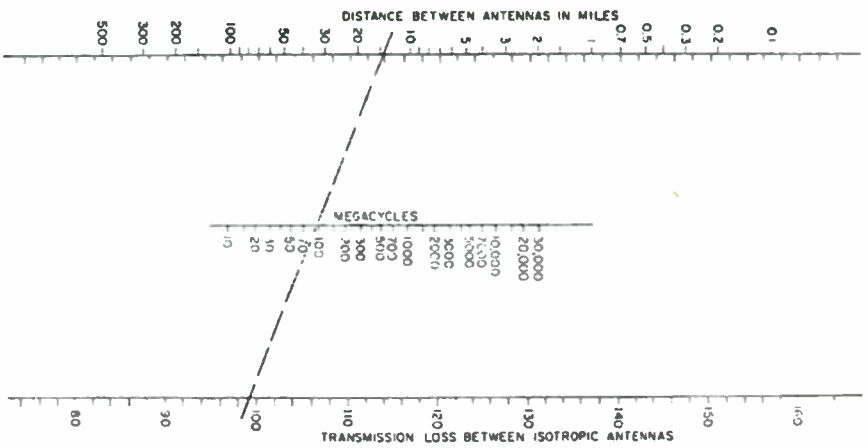
2-46 Figure 2-23. Free Space Transmission Loss
