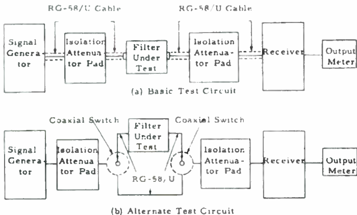
Figure I-1. Circuit for Measuring Insertion Loss of Filters
