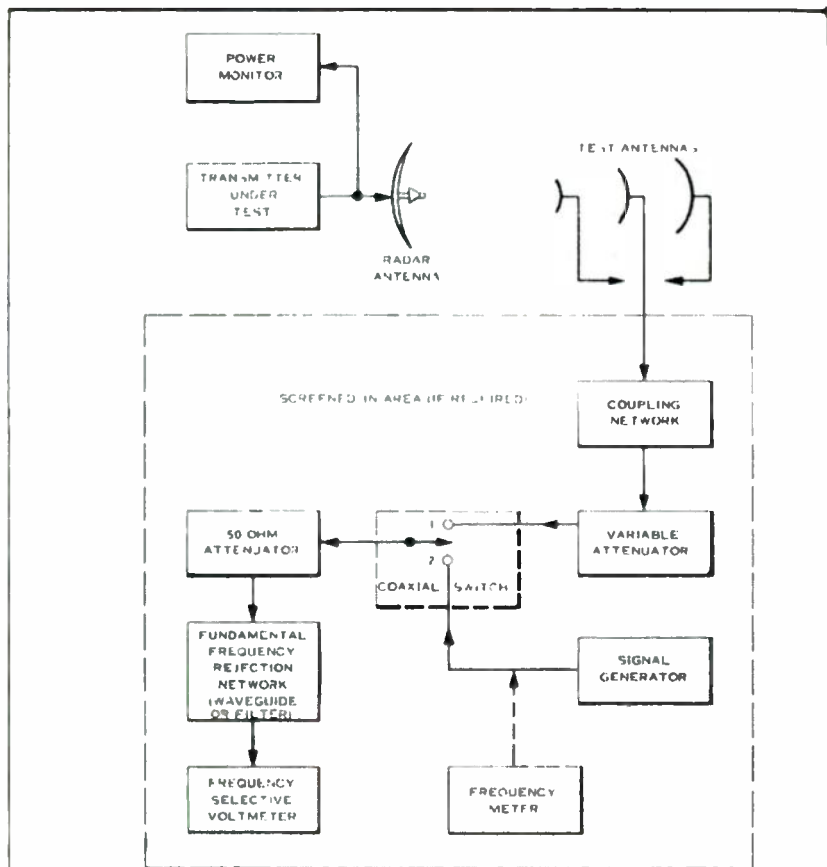
Figure 7-9. Transmitter Open Field Spurious Emission Measurement Setup
