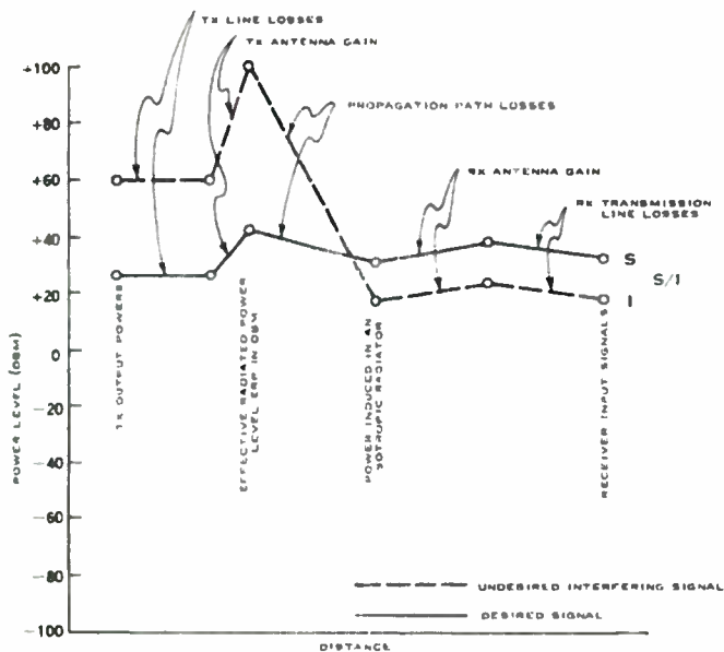
Figure 2-1. Graphical Illustration of Basic Interference Parameters
