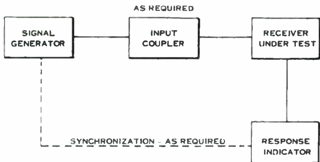
Figure 7-37. Dynamic Range Test Setup
