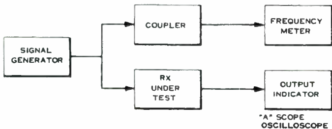
Figure 7-24. Selectivity Measurement Test Setup
