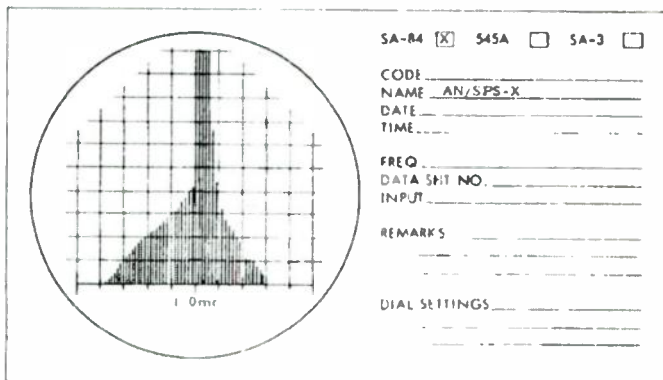
Figure 7-12. Transmitter Spectrum Signature of an L-Band Radar Set at Second Harmonic Frequency
