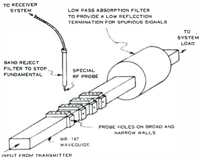
Figure 7-20. Signal Sampling Network
