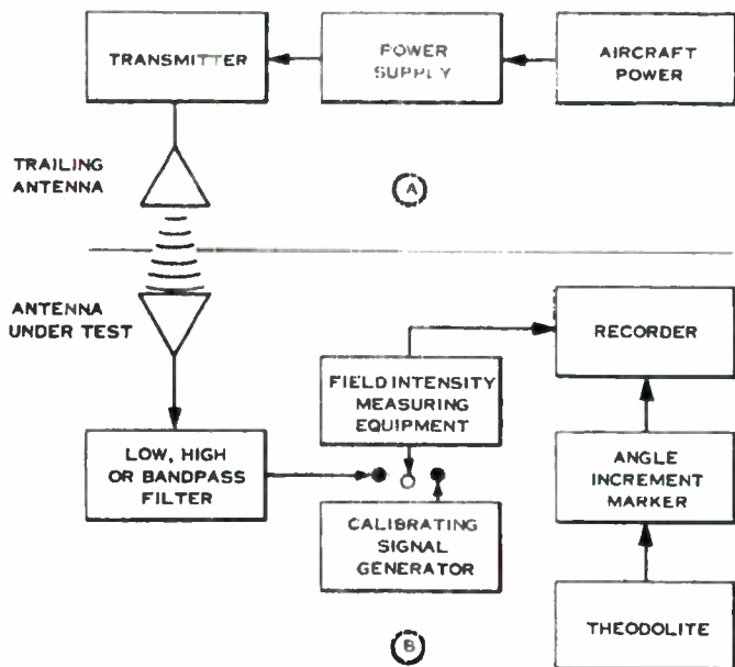
Figure 3-10. Block Diagram of Test Configuration
