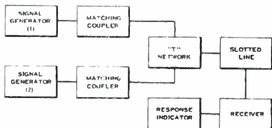
Figure 7-30. Intermodulation Test Setup
