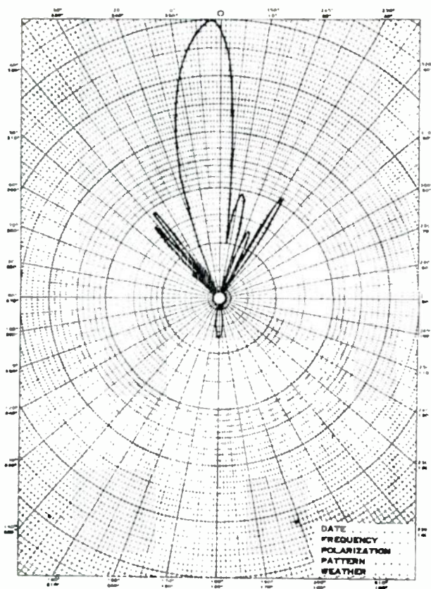
Figure 3-15 Horizontal Radiation Pattern
