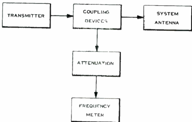
Figure 7-17. Carrier Frequency Stability Test Setup
