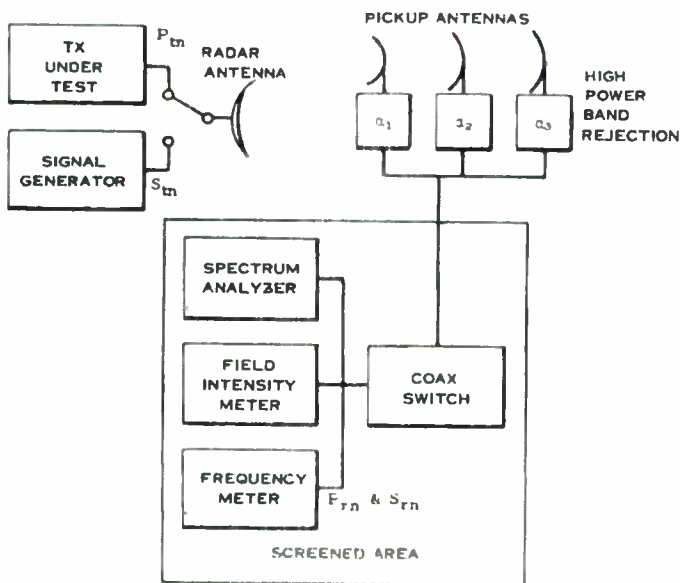
Figure 7-19. Radar 1 transmitter Signal Substitution Measurement Test Setup
