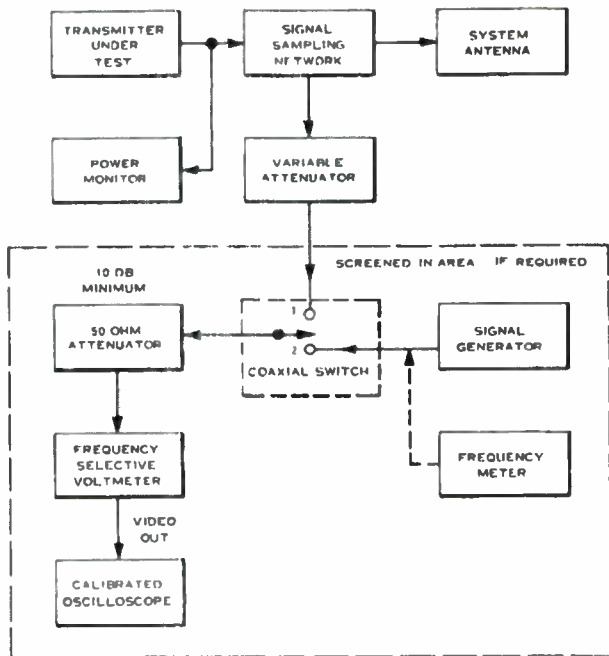
Figure 7-6. Transmitter Power Output Measurement Setup
