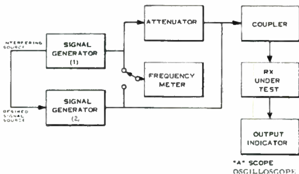
Figure 7-33. Test Setup for Adjacent Channel Tests
