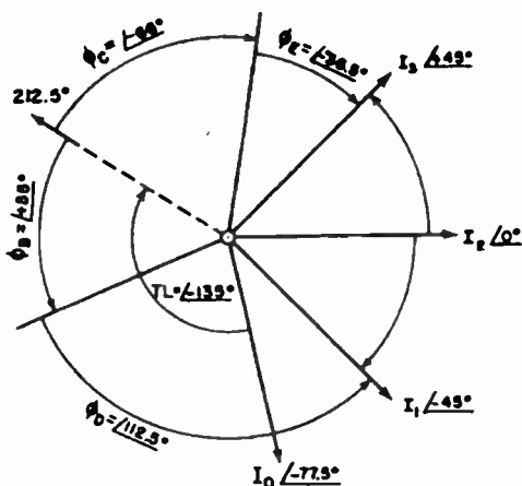
FIG. 2.25. Phasing diagram chosen for the array.
