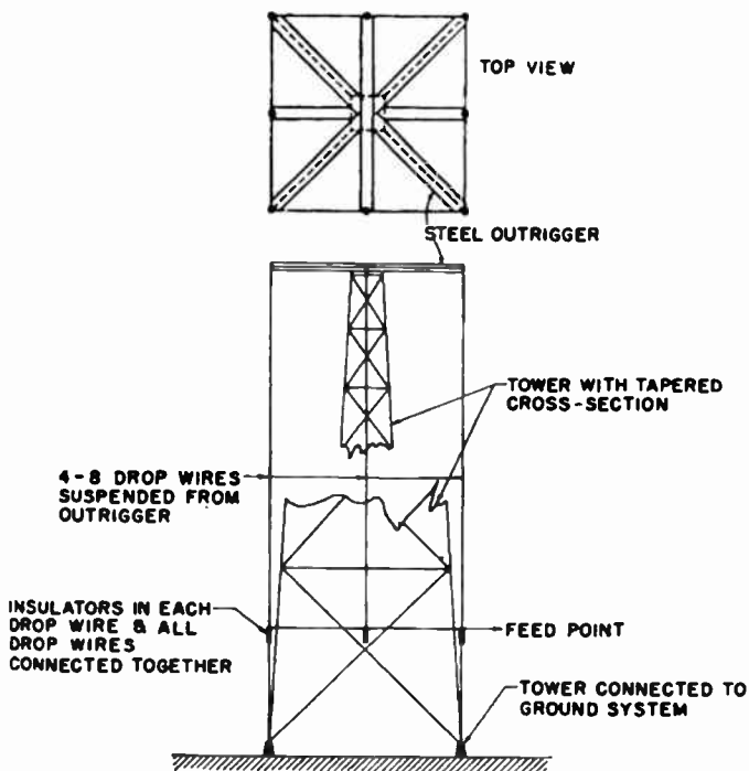
FIG. 2.14. Method of transforming a tapered tower to one of nearly uniform electrical section and using the folded unipole feed.
