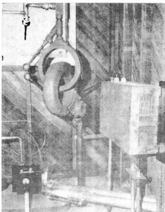
FIG. 2.69. Antenna coupling-house interior for a broadcast station (WNBC) with a plate-glass window insulator, Austin tower-lighting transformer, a monitoring rectifier, and the end of a 3½-inch concentric feeder. (Photographed during station construction. Courtesy of National Broadcasting Company.)
