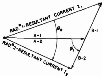
FIG. 2.23. Vector representation of mutual-impedance cancellation.
