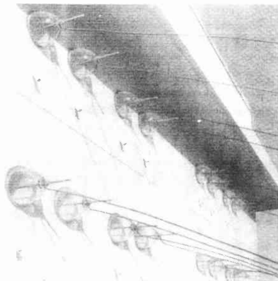
FIG. 4.85. Entrance details for eight balanced two-wire feeders as used by a 50-kilowatt high-frequency broadcast station in Rio de Janeiro. Pyrex bowl insulators (in pairs) serve as entrance insulators. Note the porcelain tubes used as ventilators to remove condensed moisture from the space in the wall between the bowl insulators. (Photograph courtesy of Radio Nacional, Rio de Janeiro and RCA International Division.)
