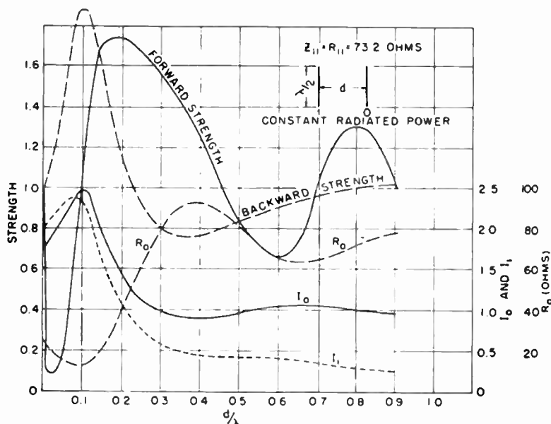
FIG. 3.35. Effect of parasitic dipole. (After Brown.)
