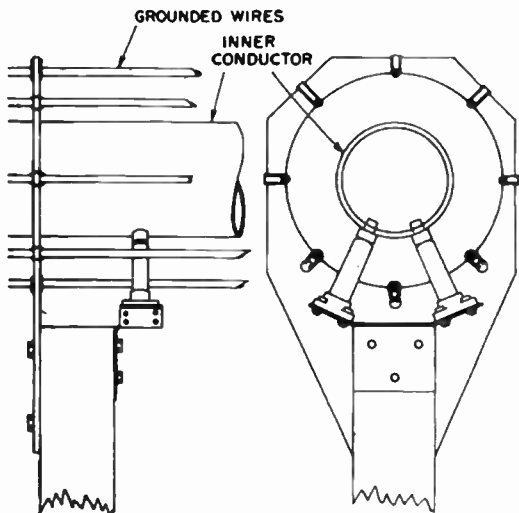
FIG. 4.10. Construction for type VIII feeder.
