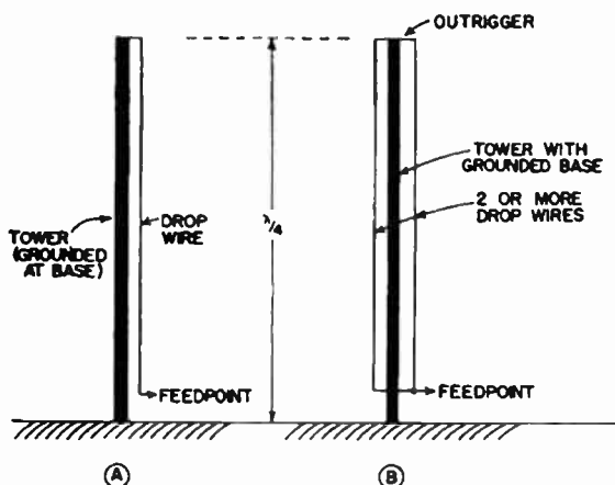
FIG. 2.13. Folded unipole principle for shunt-feeding vertical radiators.
