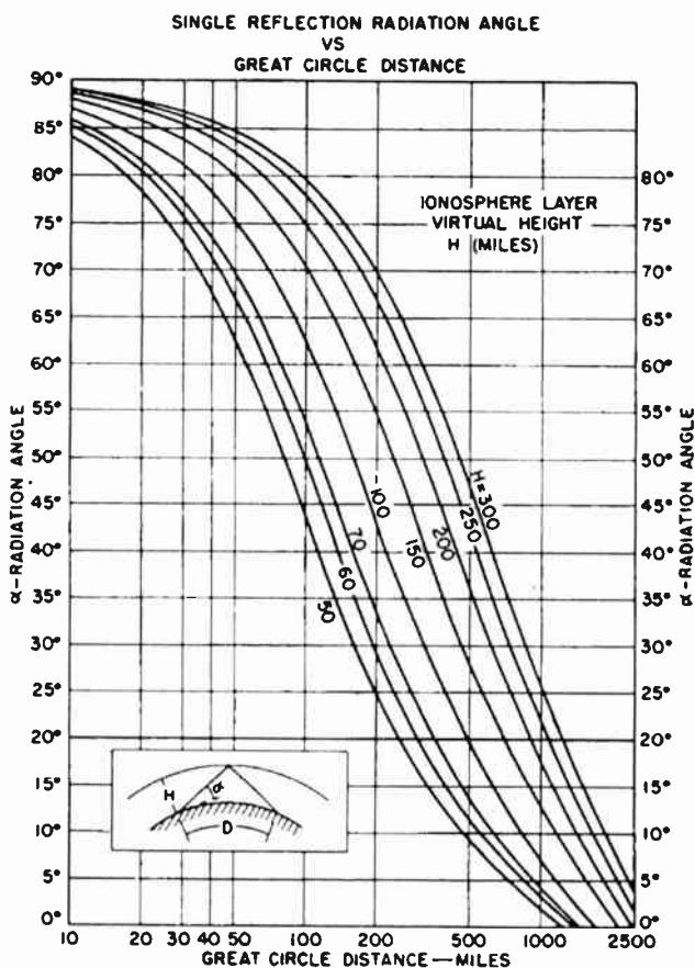
FIG. 2.3. Vertical radiation angles for sky-wave propagation.
