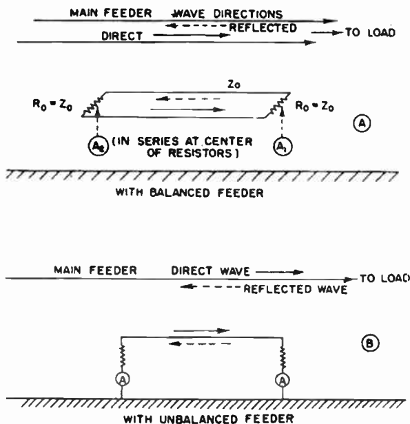
FIG. 4.82. Standing-wave indicators.
