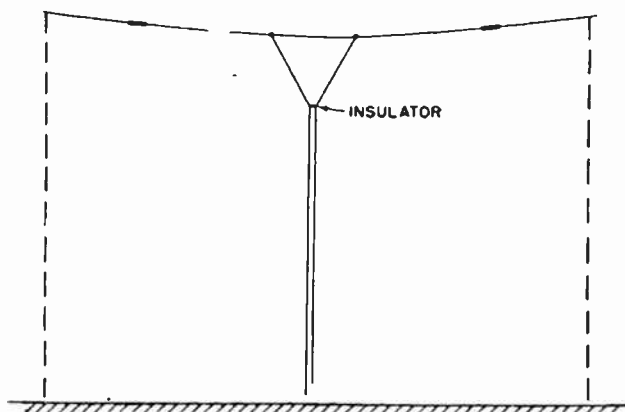
FIG. 3.19. Horizontal dipole antenna with shunt feed.
