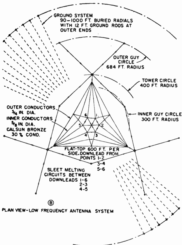
FIG. 1.34. Plan view of antenna shown in Fig. 1.33.
