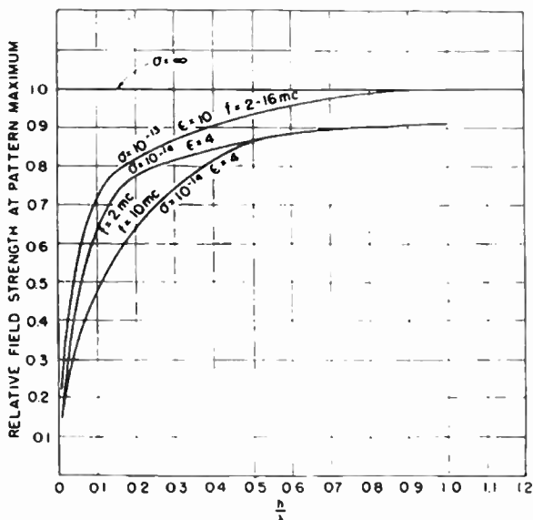
FIG. 3.17. Effect of ground conductivity on maximum field strength from a horizontal dipole antenna.
