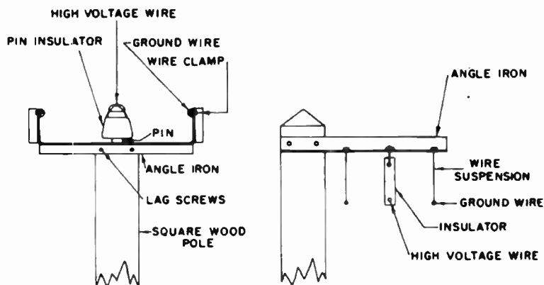
FIG. 4.6. Constructions for type V feeder.
