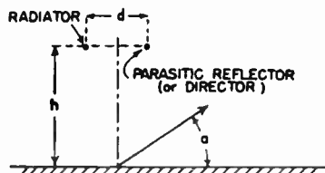
FIG. 3.34. Geometry of horizontal dipole with parasitic reflector.
