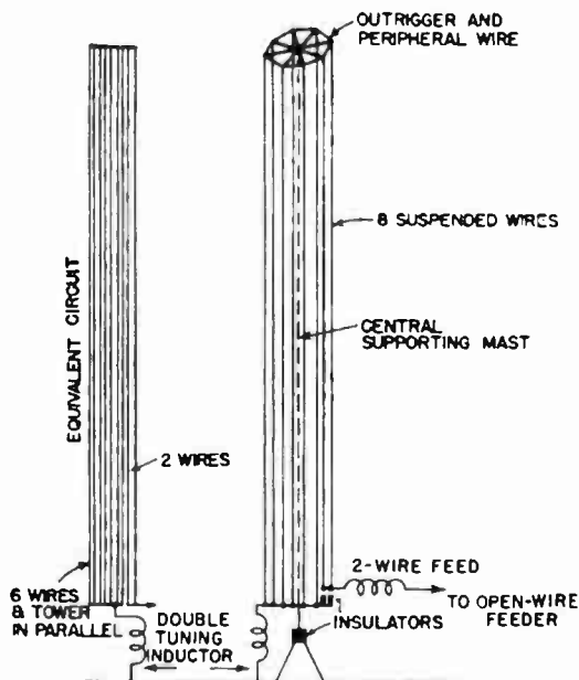
FIG. 1.11. Multiple-tuned low-frequency broadcast antenna.
