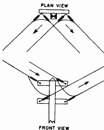
FIG. 4.21. Method of making a corner in a two-wire balanced line to maintain equal wire lengths.
