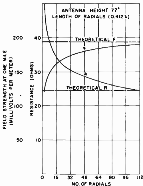
FIG. 2.19. Field strength for a 77-degree vertical radiator as a function of the number of 0.412-wavelength radial ground wires, 1,000 watts antenna input. (After Brown, Levin, and Epstein.)
