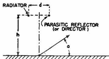
FIG. 3.34. Geometry of horizontal dipole with parasitic reflector.
