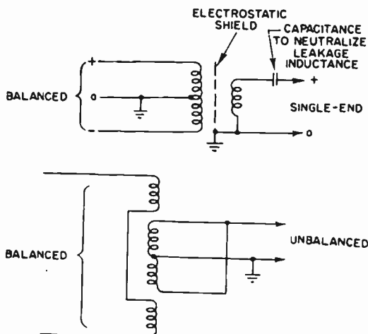
FIG. 4.46. Balance to unbalance transformers.
