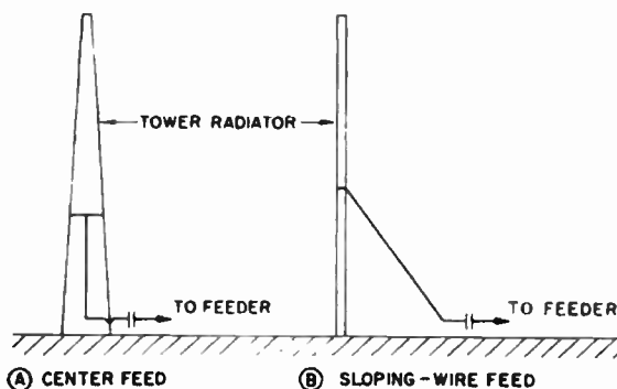
FIG. 2.8. Shunt-fed vertical radiators.
