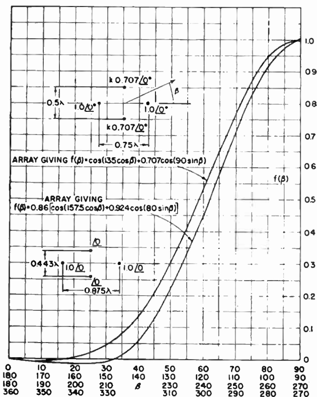
FIG. 2.46. Broad nulls obtained by crossed pairs of radiators.
