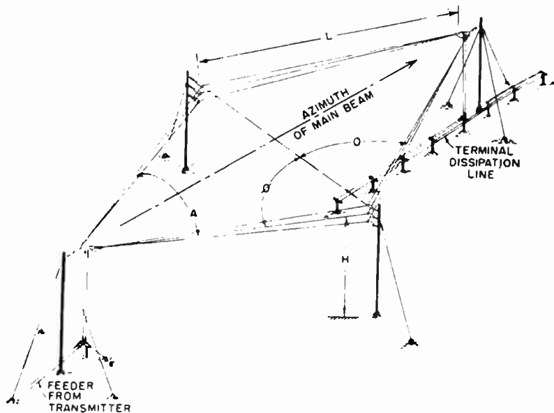
FIG. 3.77. Horizontal rhombic antenna (common three-wire form).
