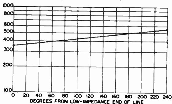
FIG. 4.42. Exponential taper computed graphically.
