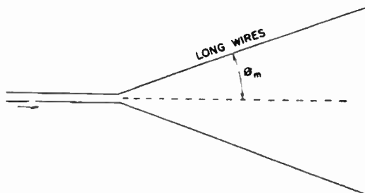
FIG. 3.73. Standing-wave V antenna.
