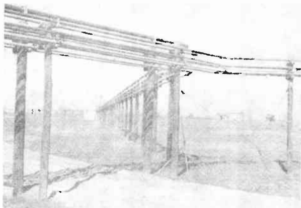
FIG. 4.77. Arrangement of pressurized coaxial feeders from the transmitter building to six radiators of the directive-antenna system for Station KTBS. (Photograph courtesy of W. M. Witty.)
