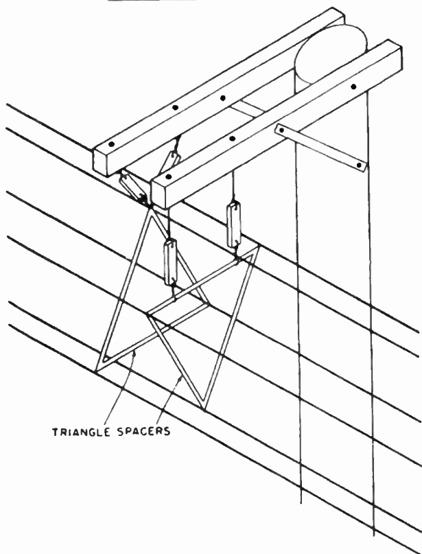
FIG. 4.28. Construction for type XIX feeder.
