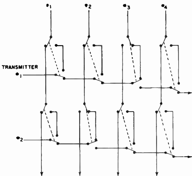
Fig. 4.54. Crossbar switching panel.
