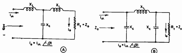
FIG. 4.44. Networks for feeder building-out sections.
