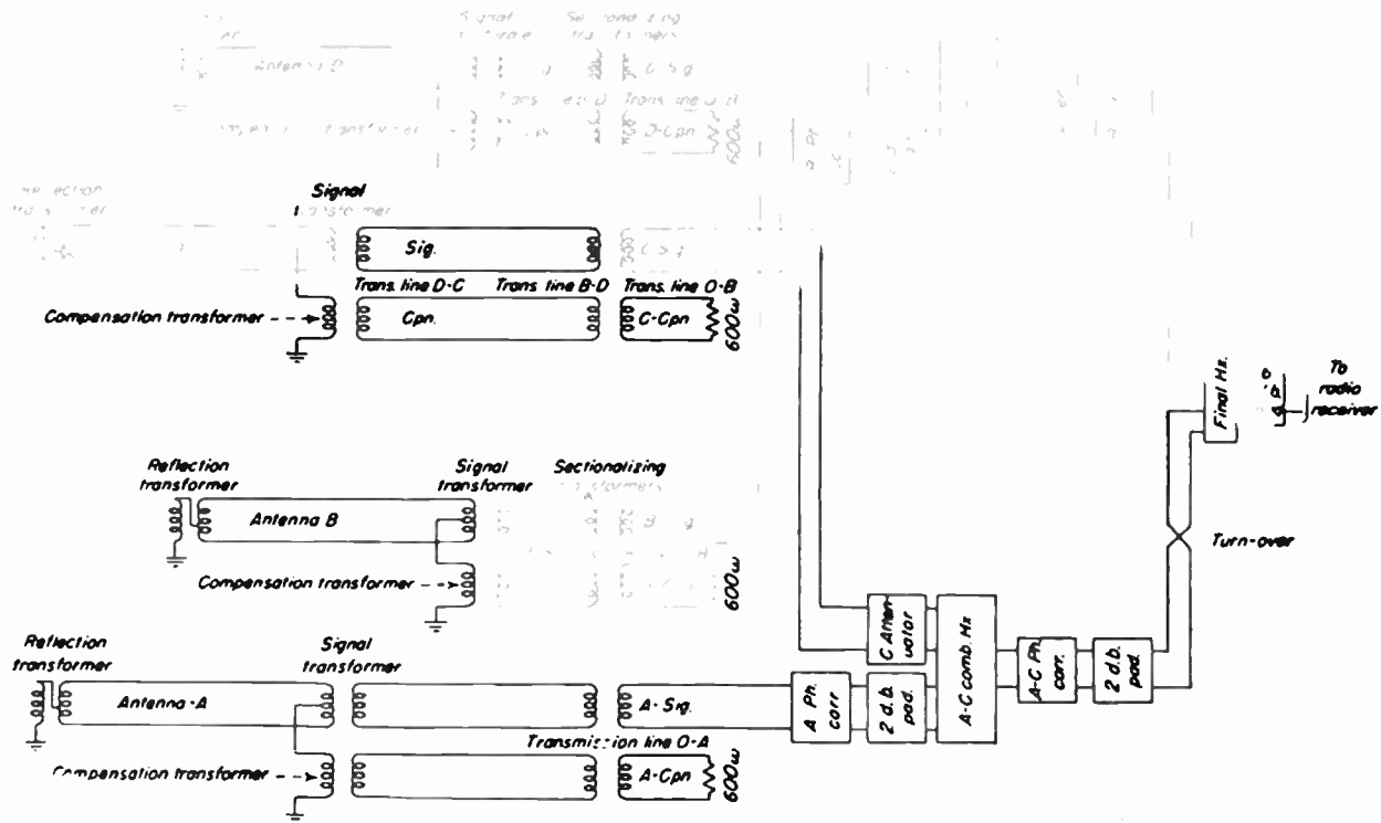
FIG. 1.21. Circuitry for the wave-antenna array at Houlton, Maine.
