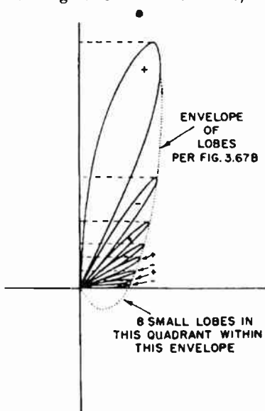
FIG. 3.69. Field pattern for a straight antenna eight wavelengths long with pure traveling wave.
