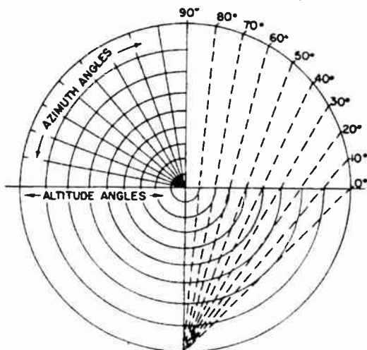
FIG. 3.82. Hemispherical coordinates derived by stereographic projection.
