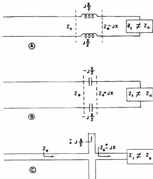
FIG. 4.40. Feeder matching, using series reactances.
