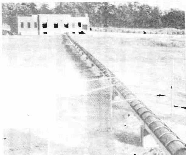
FIG. 4.74. Tile-covered coaxial feeder for 50-kilowatt medium-frequency amplitude-modulation broadcast station WNBC, Port Washington, New York. The station building is in the background. (Photograph courtesy of National Broadcasting Company.)
