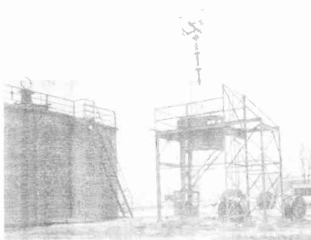
FIG. 1.43. Antenna down-lead detail for antenna built according to Figs. 1.33 and 1.34, showing down-lead counterweight and precautions at tuning-house entrance for large currents and high potentials. (Photograph courtesy of Royal Canadian Navy.)
