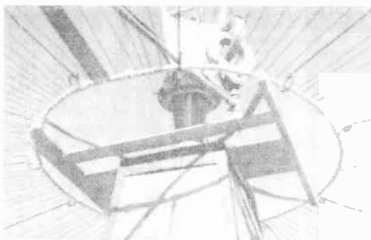
FIG. 1.15. Ground screen construction—center detail. (Photograph courtesy of W. M. Willy, consulting engineer.)
