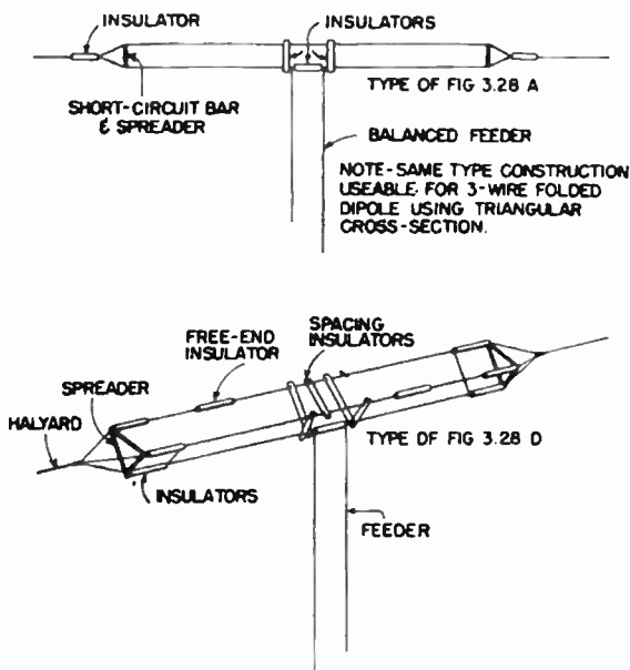
FIG. 3.29. Construction of folded dipoles.
