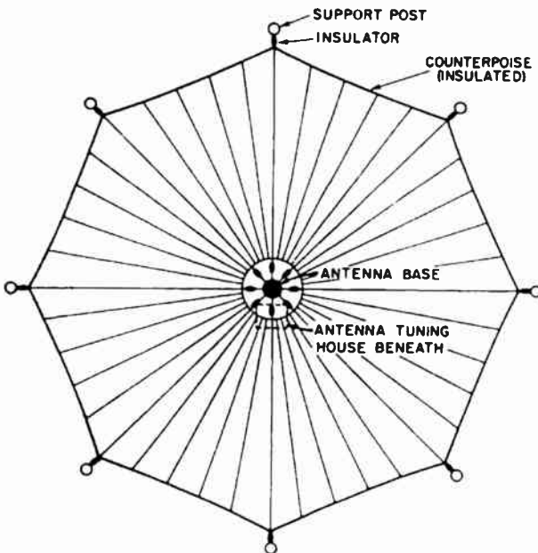
FIG. 1.14. Counterpoise (capacitance) ground.
