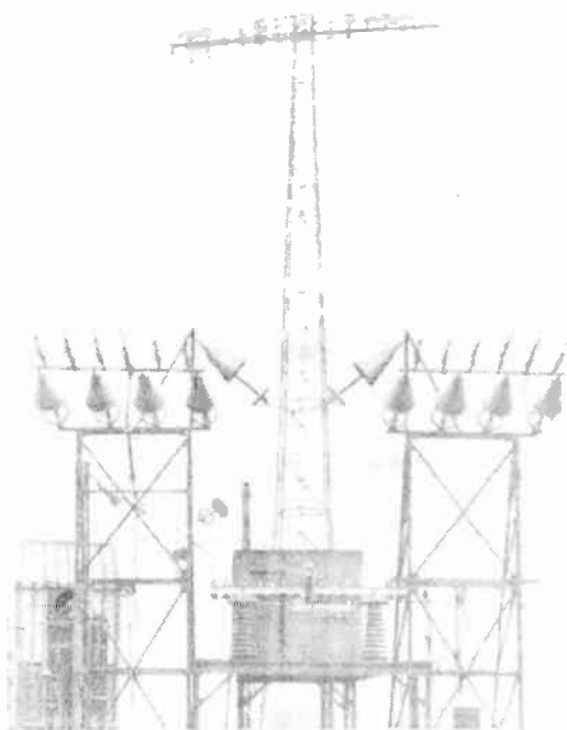
FIG. 1.37. Antenna down-lead details for the Rocky Point, New York, high-power very-low-frequency multiple-tuned antenna. (Photograph courtesy of RCA Communications, Inc., and Driz Duryea.)
