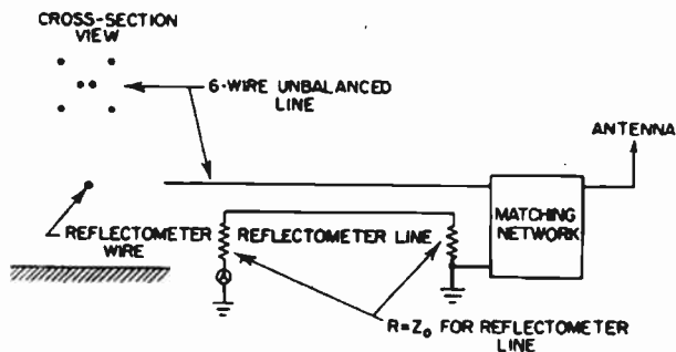
FIG. 4.63. Simplified reflectometer used with unbalanced open-wire line.
