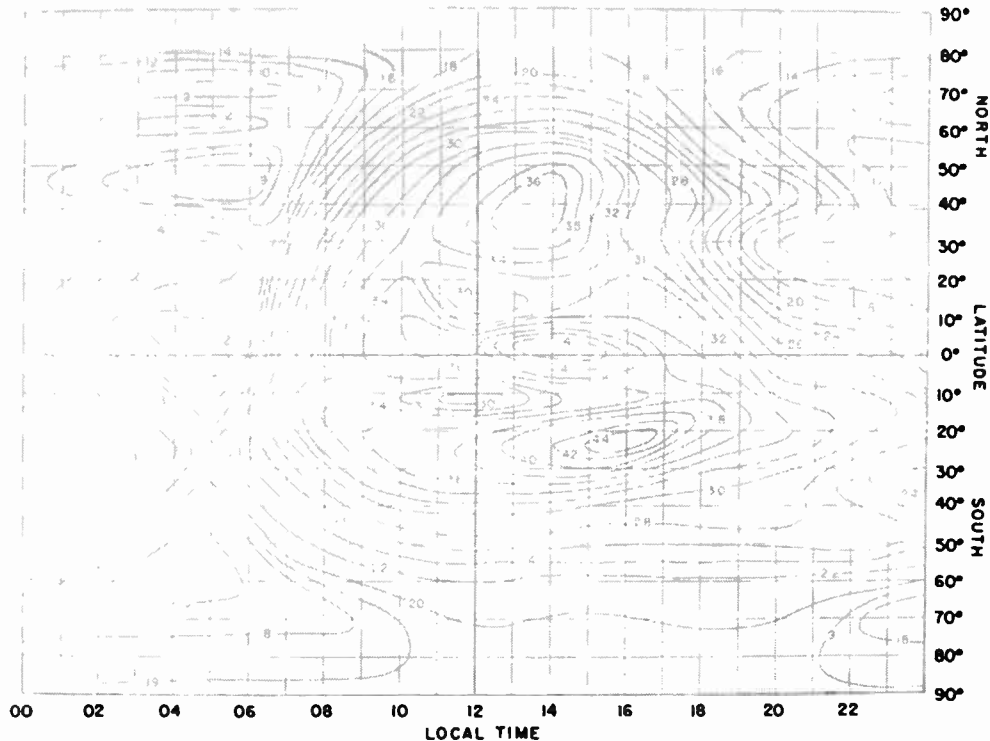
FIG. 3.3. F_2 , 4,000—maximum usable frequency in megacycles W zone, predicted for January, 1947. (After Central Radio Propagation Laboratory.)
