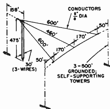
FIG. 1.29. Single-tuned inverted-L antenna with horizontal portion expanded.
