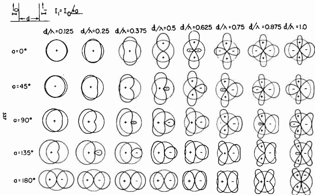
Chart of radiation patterns from two point sources having equal radiation fields, as functions of spacing and time-phase difference. For identical vertical radiators with equal currents, these are horizontal patterns. The radiating sources have their axis along the horizontal axis of each pattern, and the current in the right hand radiator has a leading time-phase with respect to that in the left-hand radiator. Polarity of fields of lobes is indicated. (After G. H. Brown.)
