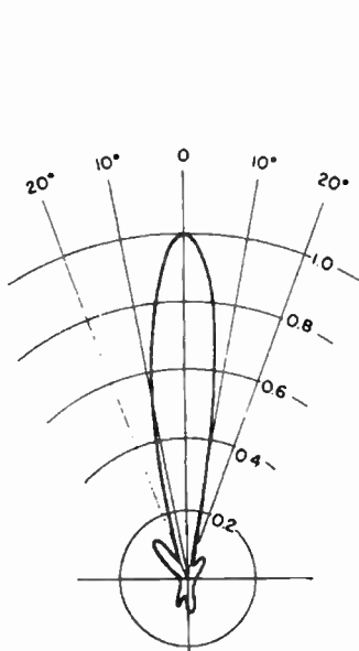
FIG. 3.94. Horizontal pattern for two-bay RCA fishbone array.
