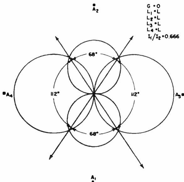
FIG. 1.23. Adcock array with squeezed courses.
