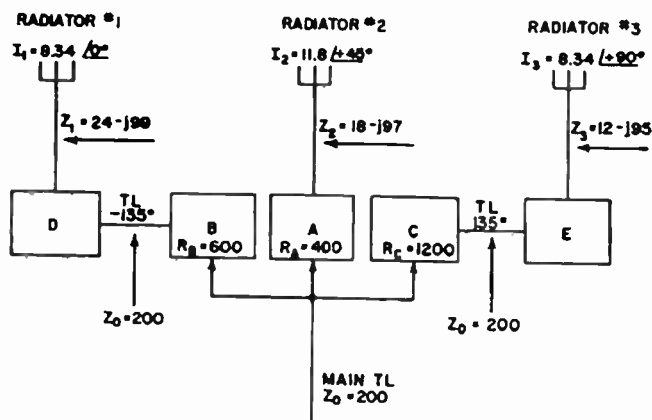
FIG. 2.24. Basic circuits for the array feeder system.
