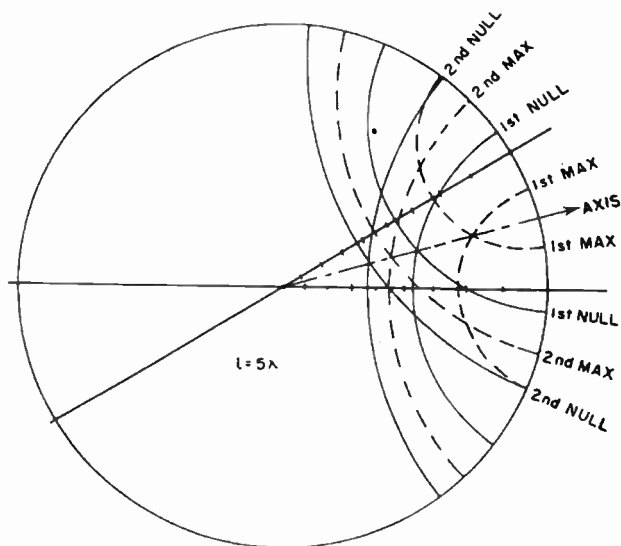
Fig. 3.87. Stereographic construction simplified for the determination of radiation lobes of first and second orders for a rhombic antenna with five wavelengths per side.
