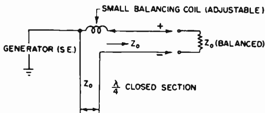
FIG. 4.49. Unbalance to balance transformer for open-wire lines.
