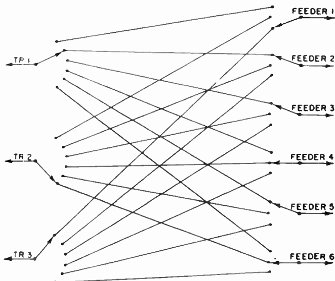
FIG. 4.57. Combination of multiposition switches.
