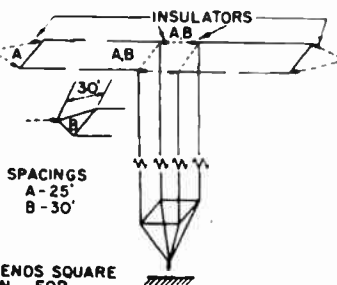
FIG. 1.31. Two-wire T antenna.
