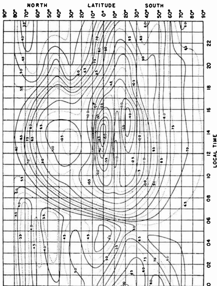
FIG. 3.2. F_1 , zero-maximum usable frequency in megacycles W zone, predicted for January, 1947. (After Central Radio Propagation Laboratory.)
