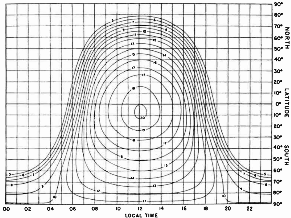
FIG. 3.4. E layer 2,000—maximum usable frequency in megacycles, predicted for January, 1947. (After Central Radio Propagation Laboratory.)
