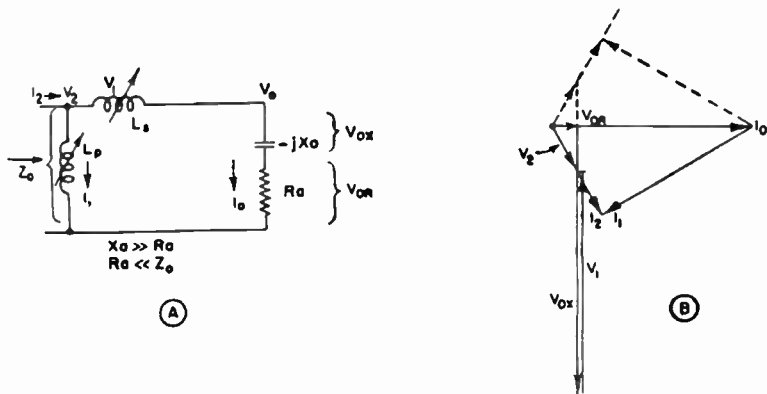
FIG. 4.32. Antenna-coupling circuit.
