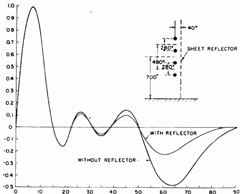
Fig. 3.53. Vertical pattern obtained by splitting secondary lobes.
