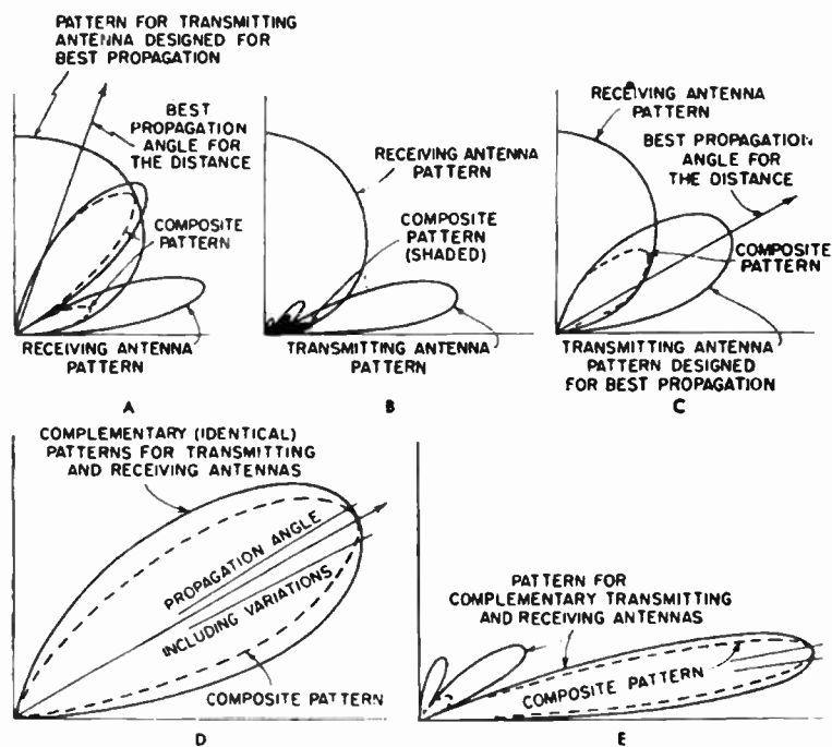
FIG. 3.10. Comparison of uncomplementary and complementary antennas.
