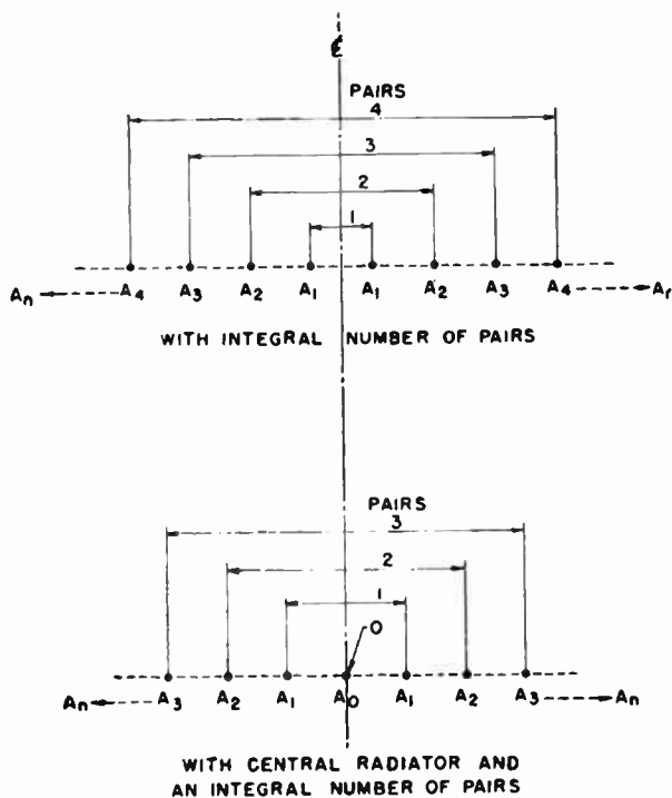
FIG. 3.64. Fourier current distributions for broadside patterns.
