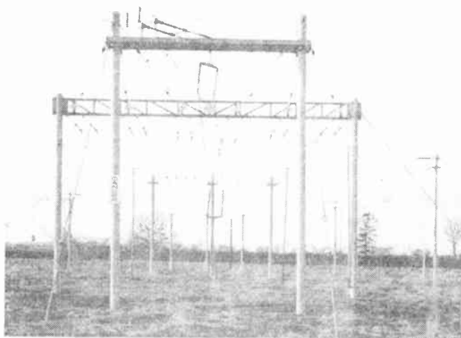
FIG. 194. A system of feeder and phasing sections associated with a slewable reversible dipole array with reflector curtain, for 100-kilowatt operation in the high-frequency broadcast service of the British Broadcasting Corporation. The photograph illustrates various assembly and rigging details, steel-post utilization, the use of cages of conductors to maintain uniform characteristic impedances, and the use of four-wire balanced side-connected feeders. A portion of the dipole array is seen in the background. Switching is accomplished manually, moving the flexible cage section to three positions. (Photograph by British Broadcasting Corporation and reproduced by courtesy of Institution of Electrical Engineers.)
