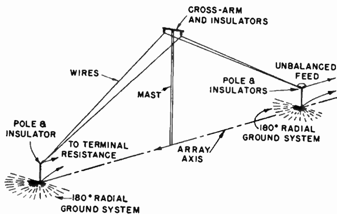
FIG. 3.96. Inverted-V traveling-wave antenna.
