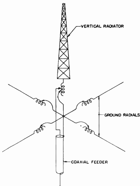
FIG. 2.32. Elementary grounding system for roof antenna.
