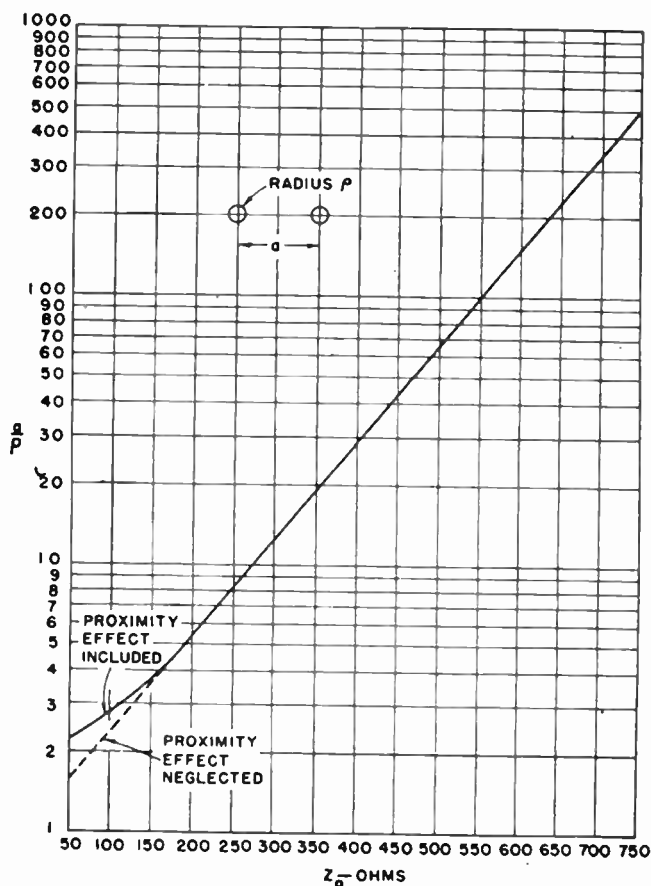
FIG. 4.23. Characteristic impedance of two-wire balanced feeder.
