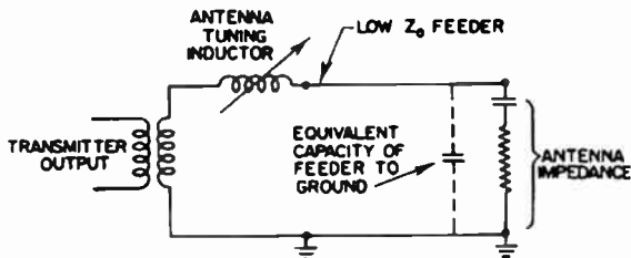
FIG. 4.31. Short feeder used as an extension leadin.
