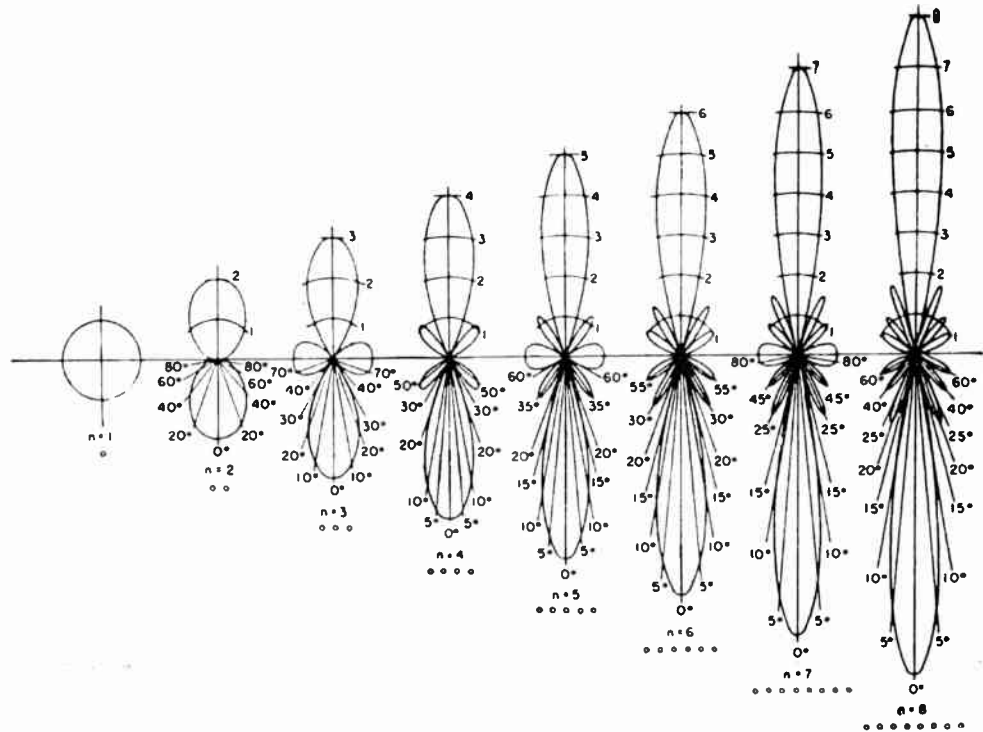
FIG. 3.46. Radiation patterns for horizontal row of vertical dipoles with unit current, cophased. (From RAF Signal Manual.)
