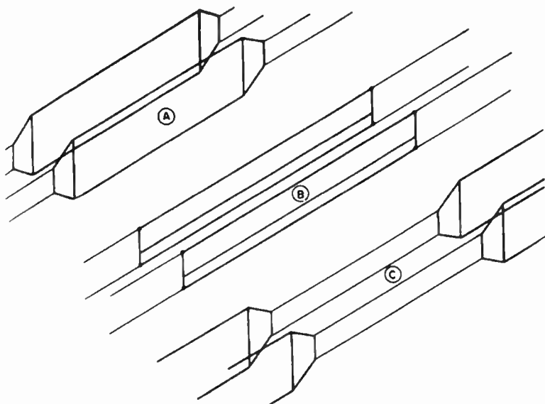
FIG. 4.35. Series impedance-transforming sections (four-wire line).
