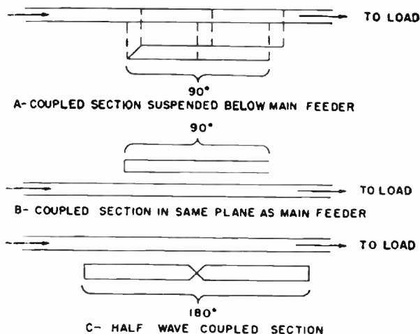
FIG. 4.41. Coupled sections for impedance matching.
