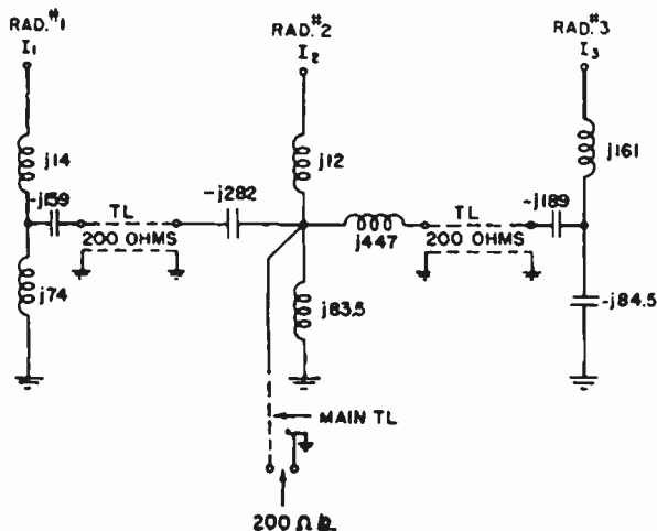
FIG. 2.31. Combined networks and feeder circuits.
