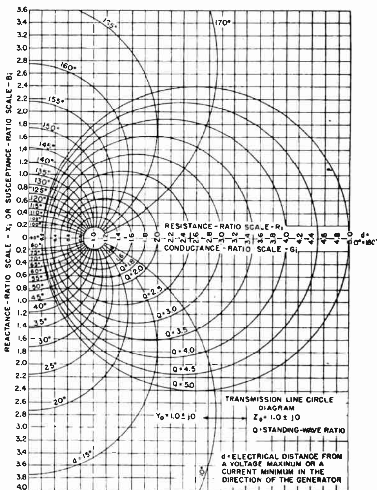
FIG. 4.58. Transmission-line circle diagram in rectangular coordinates.
