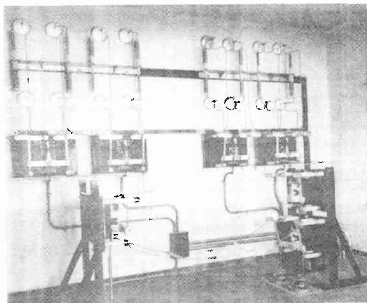
FIG. 4.93. Contactor switching system for a 50-kilowatt high-frequency broadcasting station at Rio de Janeiro, showing the branching circuits from one transmitter to eight two-wire balanced transmission lines feeding separate antennas. The contactors are low-capacitance double-pole double-throw devices designed for radio-frequency service. Balanced static drain coils, center-grounded, are associated with each feeder. (Photograph courtesy of Radio Nacional, Rio de Janeiro and RCA International Division.)
