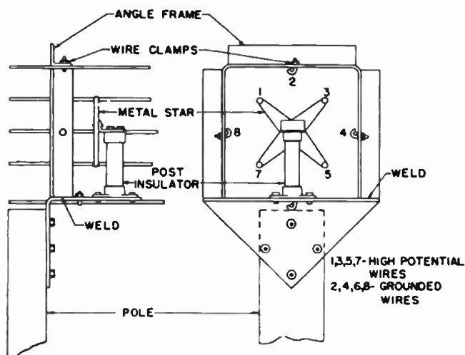
FIG. 4.16. Construction of type XII feeder.
