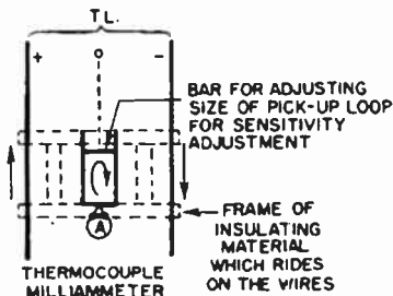
FIG. 4.64. Standing-wave indicator for balanced open-wire lines.
