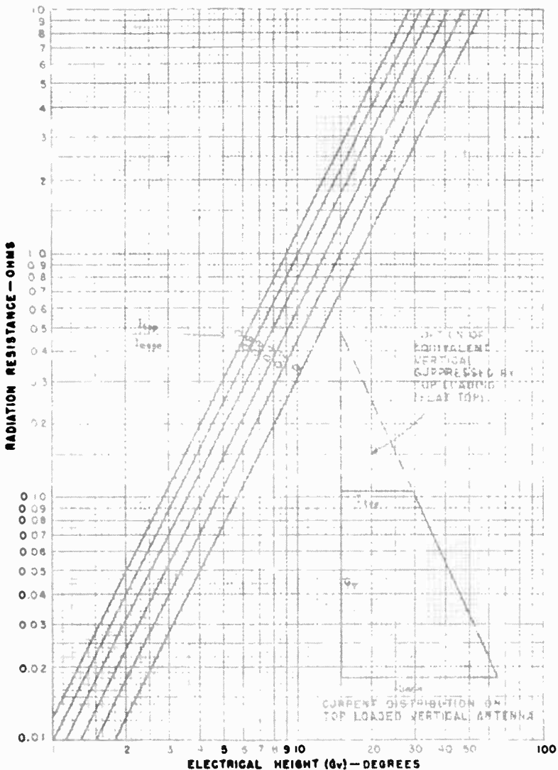
FIG. 1.2. Radiation resistance for electrically short antennas versus height of vertical portion (degrees) and ratio of currents at top and base of vertical portion.
