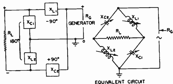
FIG. 4.45. Balance to unbalance transformer network.
