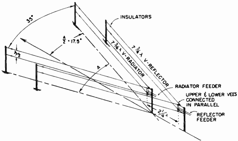
FIG. 3.76A. Scheme of the RCA Model D antenna.
