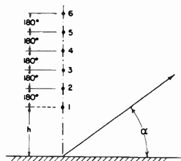
FIG. 3.37. Vertical stack of equal-current cophased dipoles.
