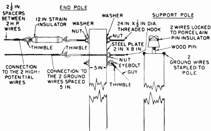
FIG. 4.13. Construction for type X feeder.
