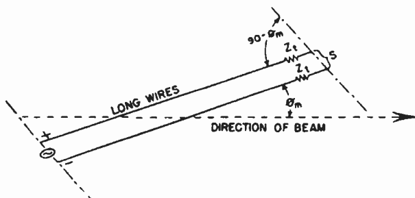
FIG. 3.72. Elementary two-wire traveling-wave antenna.
