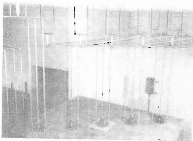
FIG. 4.107. Several feeders of the three-wire type V (two outer wires grounded with 235-ohm impedance for inside connections to directive-antenna tuning and phasing equipment. (Photograph courtesy of RCA Victor Company, Ltd., Montreal.)
