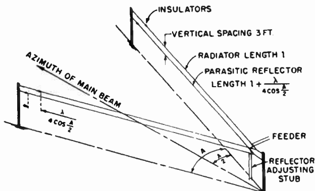
FIG. 3.76B. Scheme of the RCA Model G antenna.
