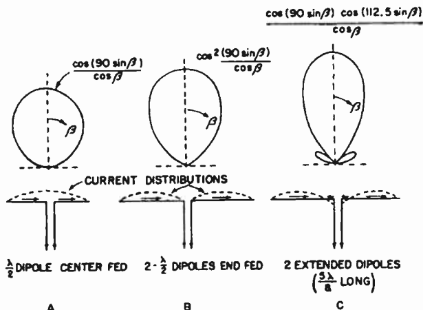
FIG. 3.31. Double dipoles and approximate patterns.
