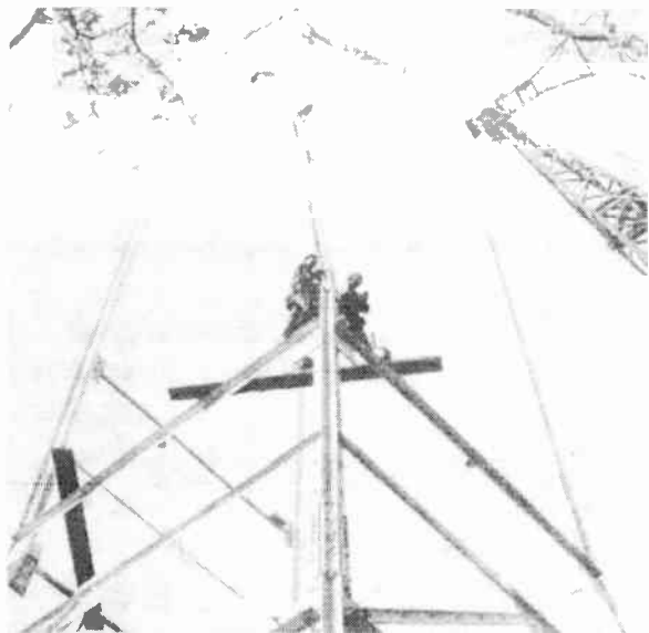
FIG. 2.57. A self-supporting broadcast radiator during construction.
