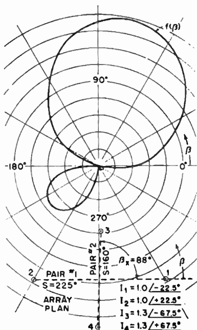
FIG. 2.49. Polar resultant pattern redrawn from Fig. 2.48.
