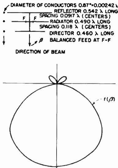
FIG. 3.36. Director-reflector array. (Data by Brown.)
