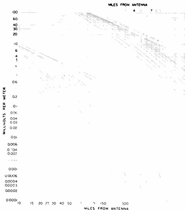
FIG. 2.2. Ground-wave field-strength versus distance curves for 970 to 1,030 kilocycles based on 100 millivolts per meter unattenuated at 1 mile along the ground (Federal Communications Commission.)
