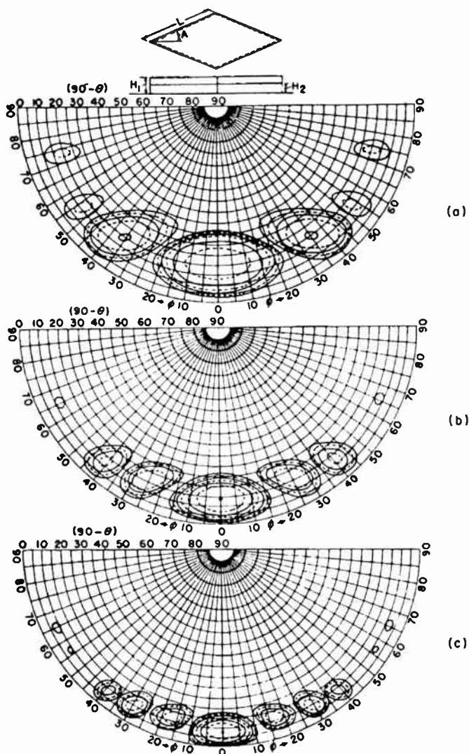
FIG. 3.88. Two-layer rhombic antenna patterns of following geometry (After Christiansen.):
