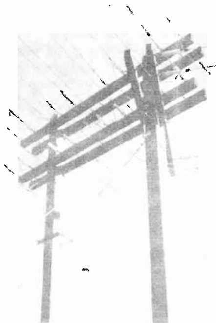
FIG. 4.84. Strain-pole assembly for eight balanced two-wire feeders, with two feeders routed from this support to antennas to the right. These feeders are used to feed any one of eight antennas from a 50-kilowatt high-frequency broadcast transmitter. Steatite block insulators are attached to eyeboits on the crossarms by clevises. The feeder wires are formed in eyes to attach to the insulators and are closed with pressed-metal retainers. (Photograph courtesy of Radio Nacional, Rio de Janeiro and RCA International Division.)
