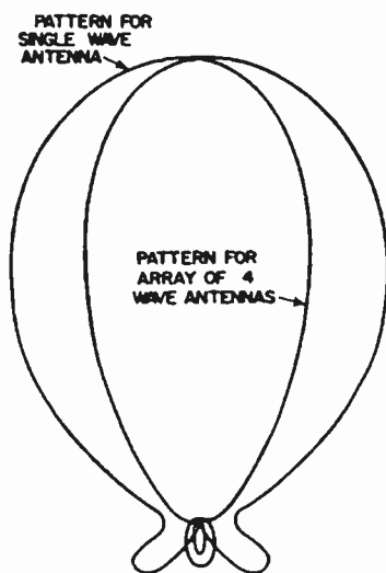
FIG. 1.20. Measured response patterns for one element and for an array of four wave antennas used at the receiving station of the American Telephone & Telegraph Co. at Houlton, Maine.
