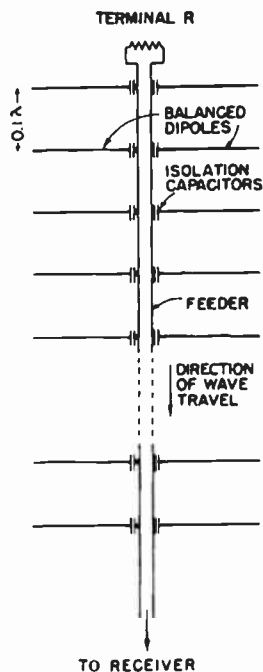
FIG. 3.92. RCA fishbone-antenna circuitry.
