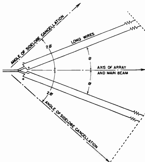
FIG. 3.75. Double traveling-wave V antenna.
