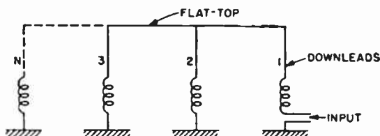
FIG. 1.7. Principle of multiple tuning.
