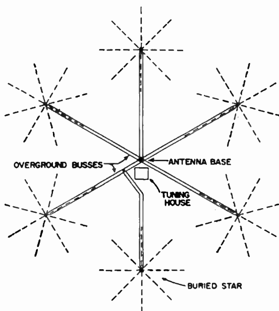
FIG. 1.13. A single circle of star grounds.
