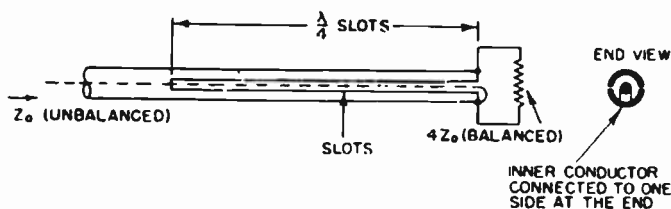
FIG. 4.51. Split-sheath coaxial unbalance to balance transformer.
