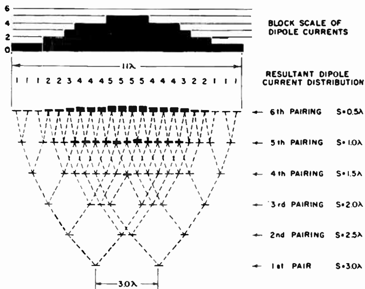
FIG. 3.60. Synthesis of current distribution that gives the pattern of Fig. 3.59.
