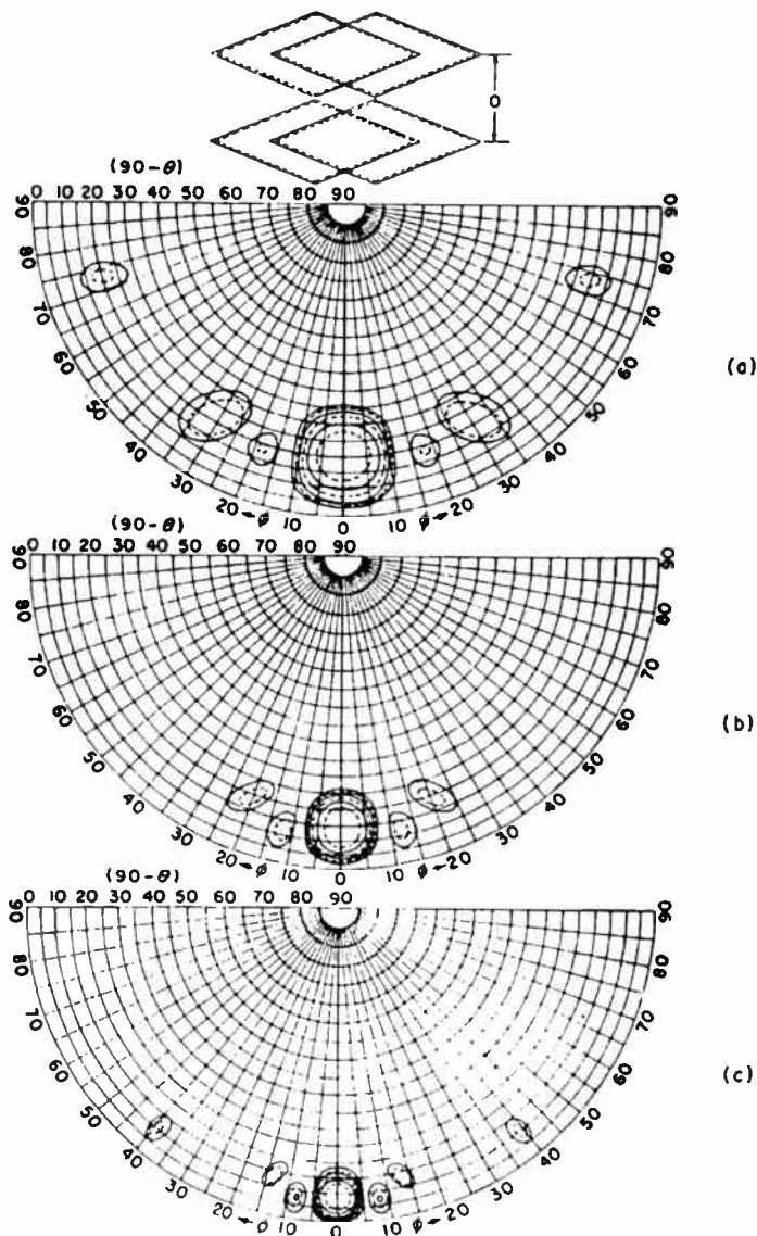
FIG. 3.91. Radiation patterns for two arrays of the type of Fig. 3.90 in broadside but with major axis spacings as follows: (a) 2.33\lambda ; (b) 3.50\lambda ; (c) 5.25\lambda . (After Christianesen.)
