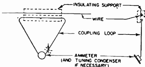
FIG. 4.66. Loop-coupled ammeter for individual open-wire measurements.
