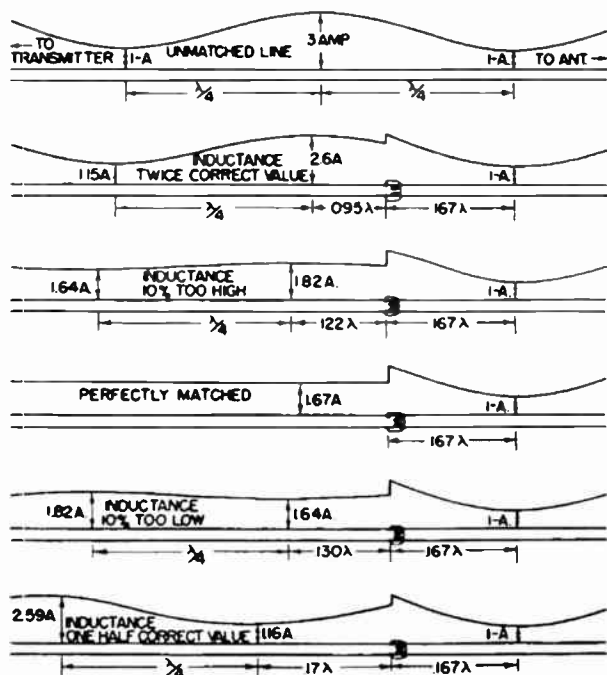
FIG. 4.39. Example of impedance matching by shunt coil. (After Carter.)
