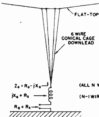
FIG. 1.9. Flat-top antenna with conical cage down lead.
