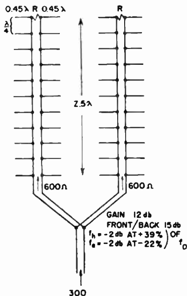
FIG. 3.95. English type HAD fishbone antenna (two-bay).
