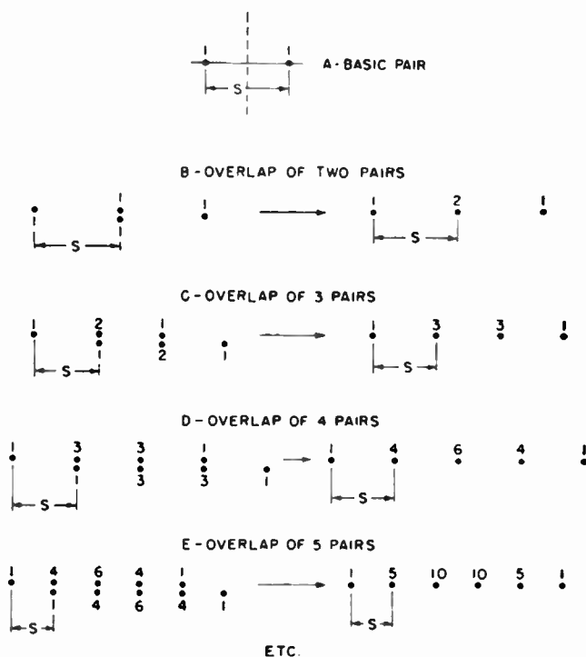
FIG. 3.54. Binomial current distributions for broadside arrays.
