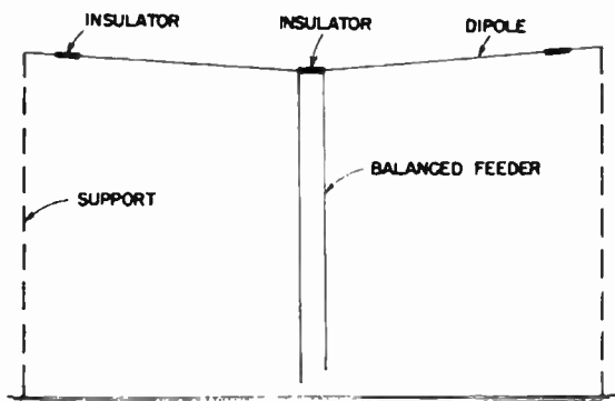
FIG. 3.21. Horizontal dipole antenna center-fed by a balanced feeder.
