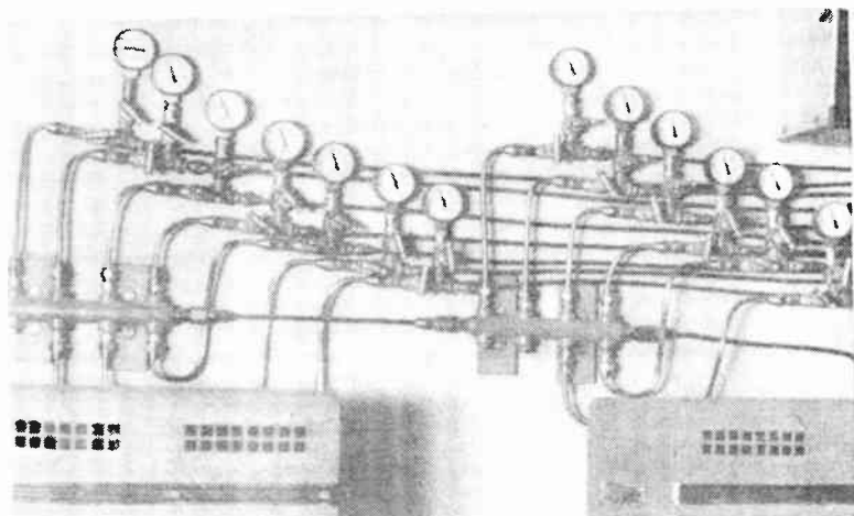
FIG. 4.78. Details showing pressure gauges for the dehydrated-air-distribution system for the coaxial feeders of Fig. 4.77 at Station KTBS. (Photograph courtesy of W. M. Witty.)
