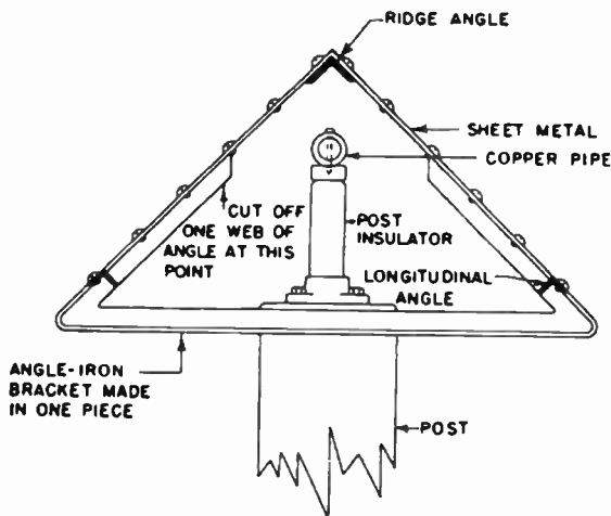
FIG. 4.18. Construction of type XIII feeder.
