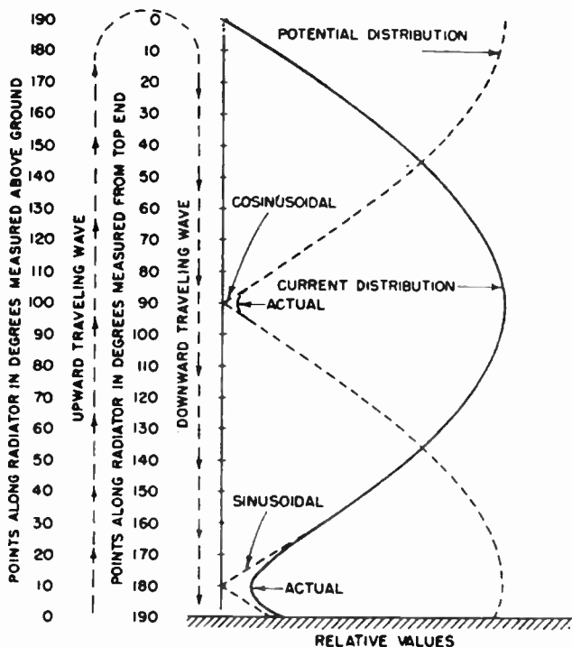
FIG. 2.5. Comparison of current distributions for sine and actual relative values on a 190-degree uniform vertical radiator.
