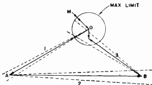
FIG. 2.51. Examination of pattern stability by vector diagram of fields in null region.
