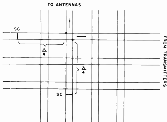
FIG. 4.53. Crossbar switching with dead-end elimination.
