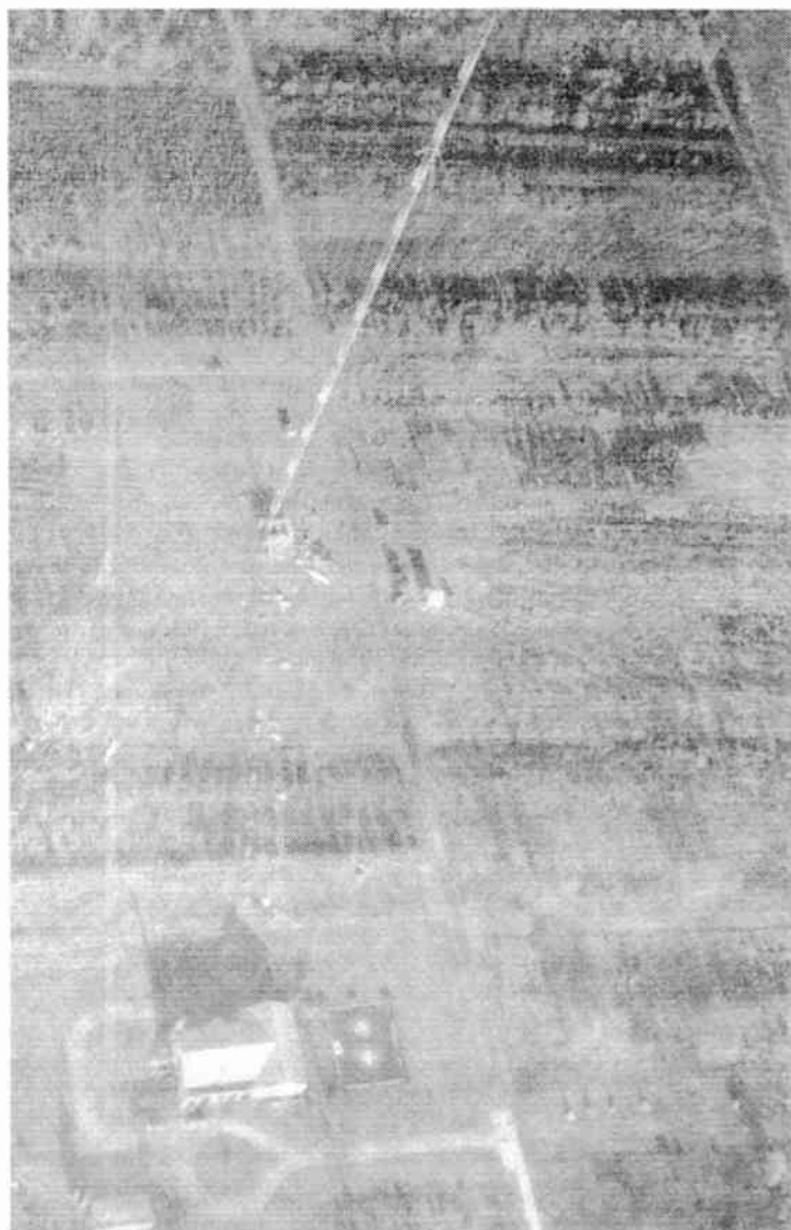
FIG. 2.52. Aerial view of a high-power broadcasting station (Radio Station WJZ when it was located at Bound Brook, New Jersey), showing the station building, the 750-foot radiator, and the freshly furrowed ground where the ground wires were plowed into the soil. (Photograph courtesy of National Broadcasting Company.)
