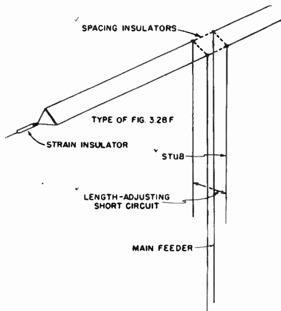
FIG. 3.30. Adjustable two-wire folded dipole.
