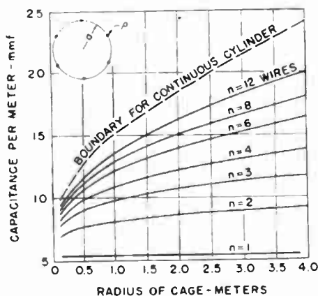
FIG. 3.24. Relation between cylindrical cage and continuous cylinder. (After W
