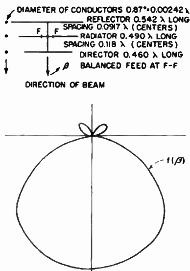
FIG. 3.36. Director-reflector array. (Data by Brown.)
