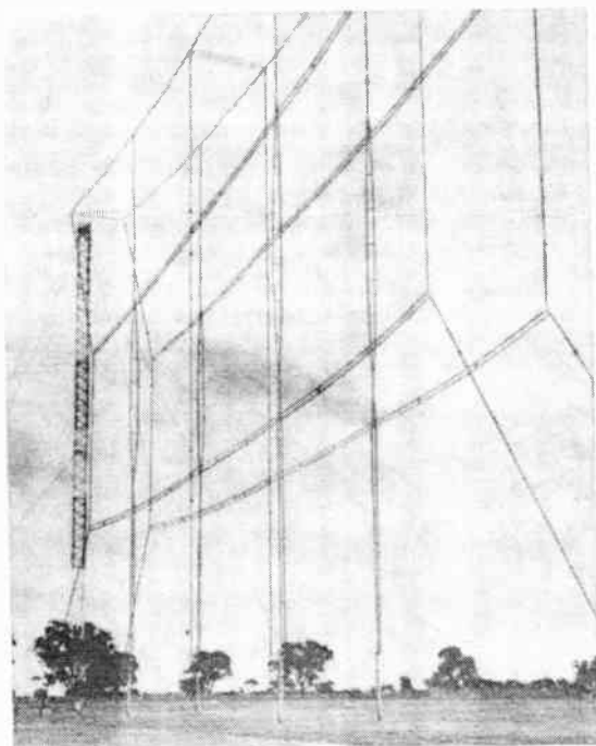
FIG. 3.106. View of a horizontal dipole array using two-wire dipoles. (Photograph courtesy of Australian Postmaster-General's Office.)
