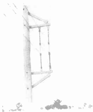
FIG. 4.90. A method of construction for the four-wire side-connected balanced feeder. (Photograph courtesy of Australian Postmaster-General's Office.)
