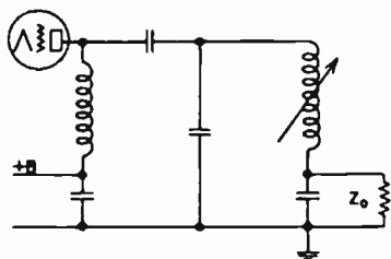
FIG. 4.33. Transmitter output-coupling circuit.
