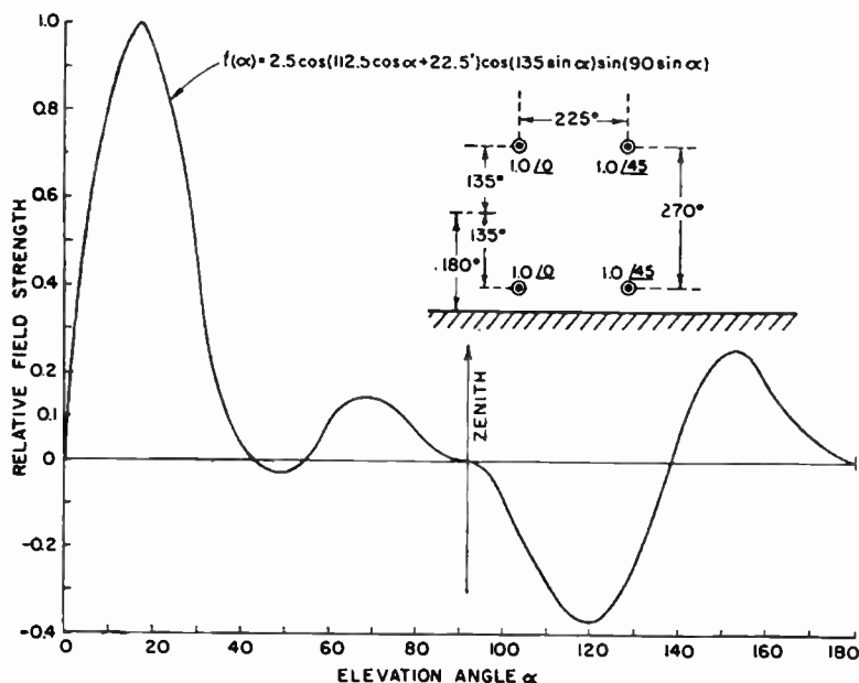
FIG. 3.40. Vertical-plane pattern for the array shown.
