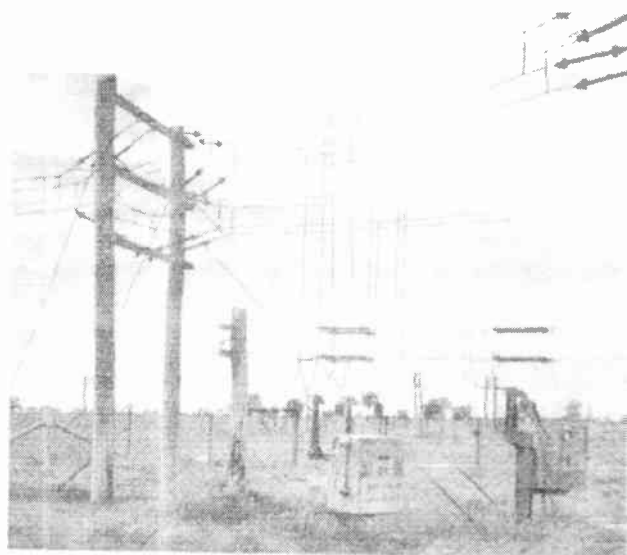
FIG. 4.92. Reversing junction for a dipole-array feed with four-wire side-connected balanced feeders, showing quarter-wave stubs and short-circuiting switches. (Photograph courtesy of Australian Postmaster-General's Office.)
