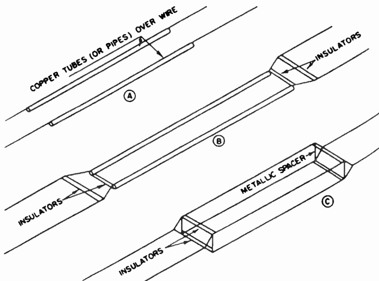
FIG. 4.34. Series impedance-transforming sections (two-wire line).
