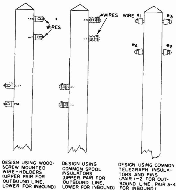
FIG. 4.60. Economical arrangements for dissipation lines.
