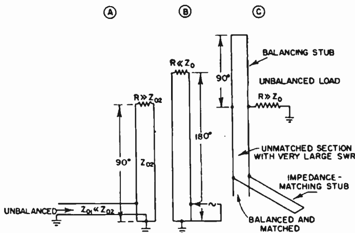
FIG. 4.50. Impedance-matching unbalance to balance circuits.
