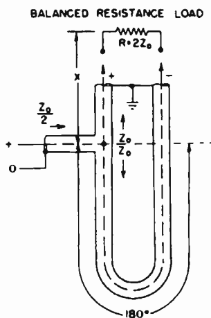
FIG. 4.47. Half-wavelength line transformer from unbalance to balance.
