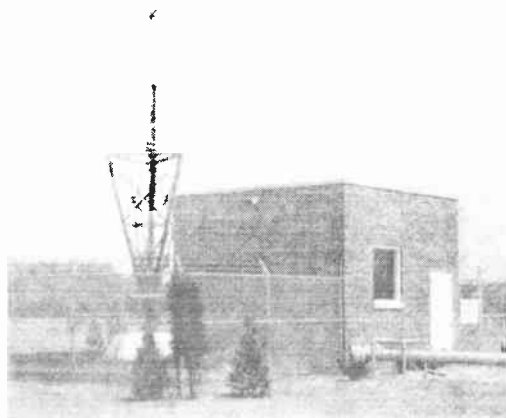
FIG. 2.54. Base of a guyed broadcast vertical radiator, coupling house, protective fence, and the 10-inch concentric transmission line suitable for 500-kilowatt service. Radio Station WJZ at Bound Brook, New Jersey (location now at Lodi, New Jersey). (Photograph courtesy of National Broadcasting Company.)
