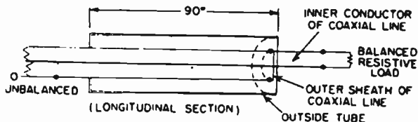
FIG. 4.48. Coaxial "bazooka," or balun.
