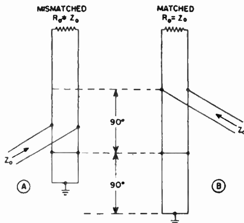
FIG. 4.36. Impedance matching by parallel feed.
