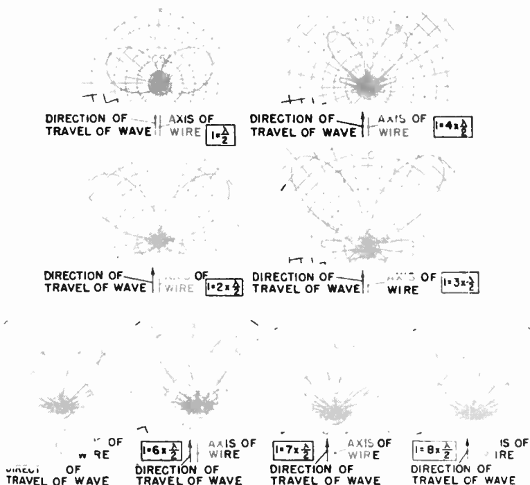
Fig. 3.68. Field patterns due to a straight wire carrying traveling waves. (From RAP Signal Manual .)
