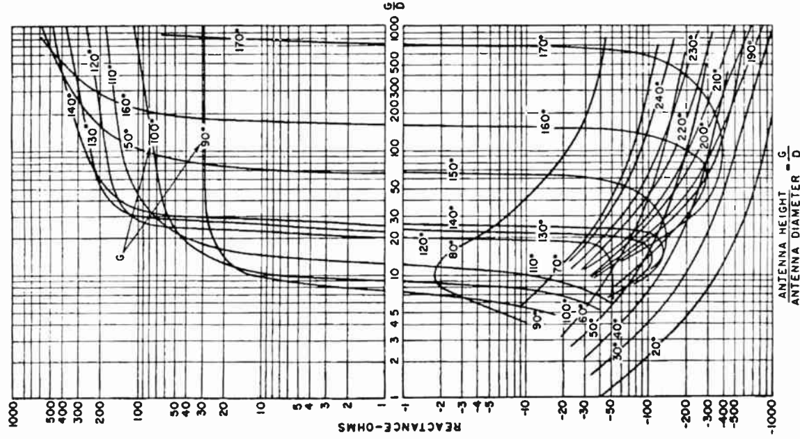
FIG. 2.16. Measured base (series) reactance for cylindrical vertical radiators over perfectly conducting ground. (After Broun and Woodward.)
