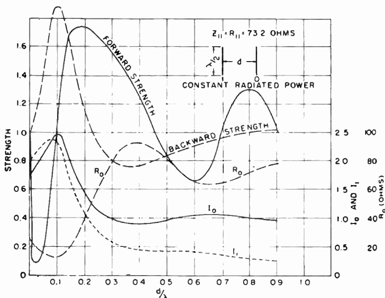
FIG. 3.35. Effect of parasitic dipole. (After Brown.)
