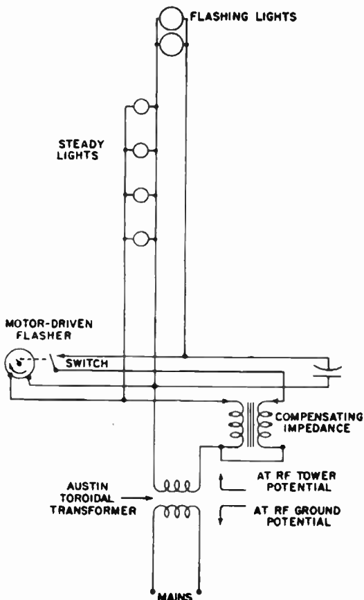
FIG. 2.34. Radio-tower-lighting system.
