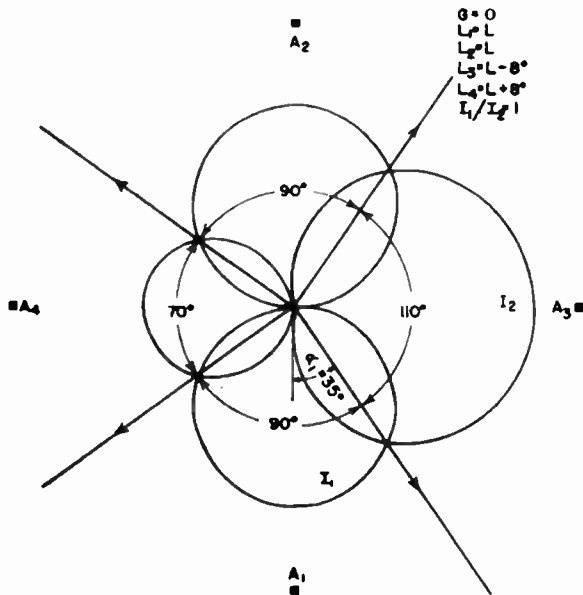
FIG. 1.25. Adcock array pattern with one antiphased pair and one pair out of antiphased relationship.
