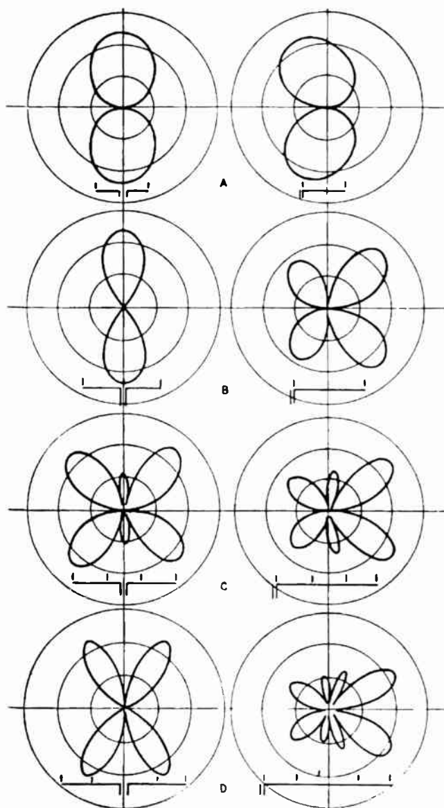
FIG. 3.23. Comparative effects of center feed and end feed. (After Leckner.)
