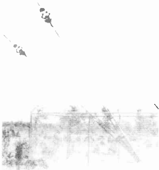
FIG. 2.58. Anchor for guy cables for two levels, used with a guyed broadcast vertical radiator. (Photograph courtesy of National Broadcasting Company.)
