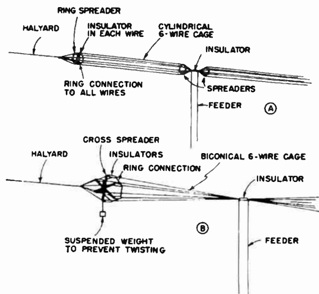
FIG. 3.27. Constructions for cylindrical and biconical cage antennas.
