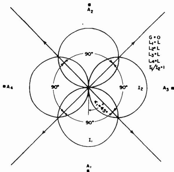
FIG. 1.22. Adcock array for four 90-degree courses.
