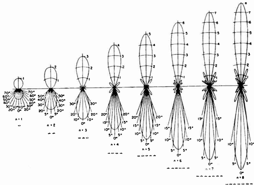
FIG. 3.41. Patterns for collinear cophased equicurrent dipoles. (From RAF Signal Manual.)
