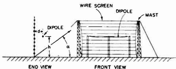
FIG. 3.33. Horizontal dipole with passive screen reflector for unidirectional radiation.
