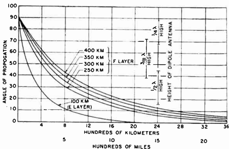
FIG. 3.14. Vertical radiation angles for one-hop circuits.
