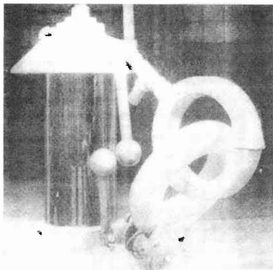
FIG. 2.63. A safety-core oil-filled tower-base insulator with a tower-lighting transformer and safety gap assembled. (Photograph courtesy of A. O. Austin.)
