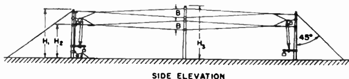
Fig. 3.89. Construction for two-layer rhombic antenna.
