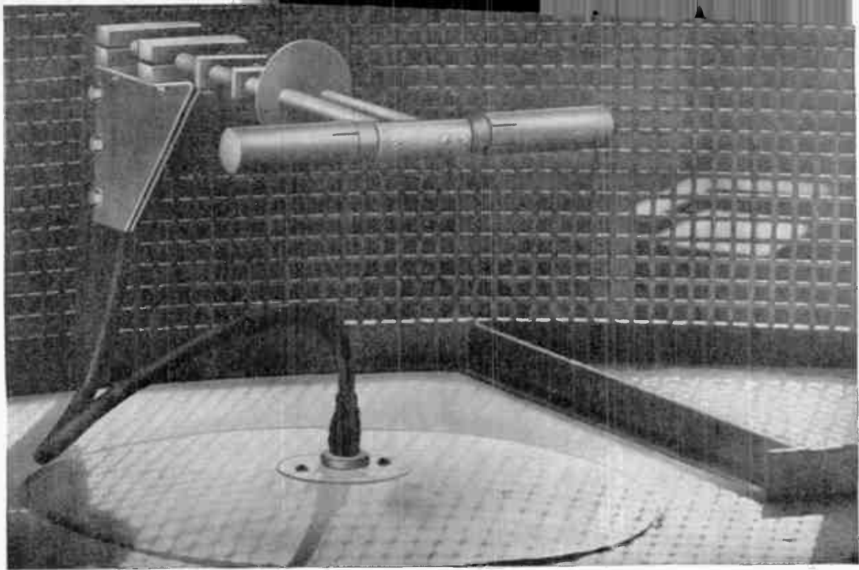
COLORED TELEVISION ROTATING RECEIVING ANTENNA
