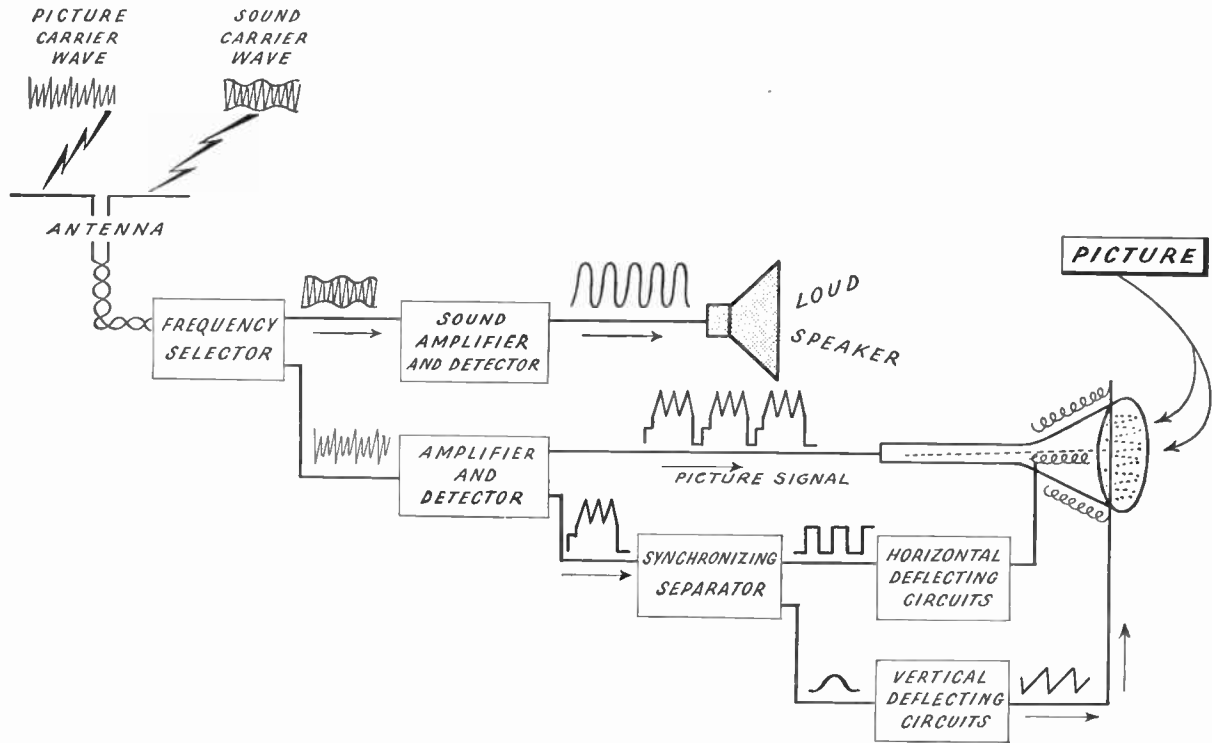
BLOCK DIAGRAM OF TELEVISION
