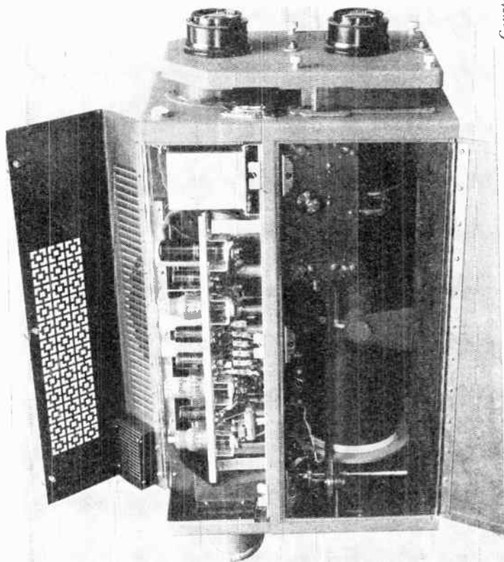
INSIDE VIEW OF STANDARD PICKUP CAMERA
