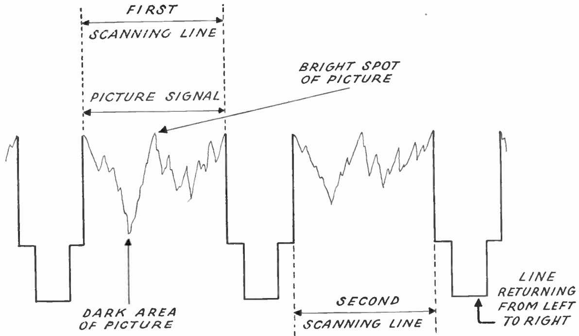
ELECTRONIC SIGNAL PRODUCED BY TELEVISION CAMERA
