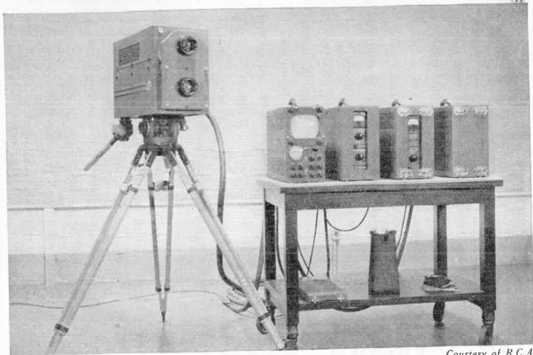
CAMERA AND REMOTE PICKUP EQUIPMENT USED FOR TELECASTING SPORTS EVENTS
