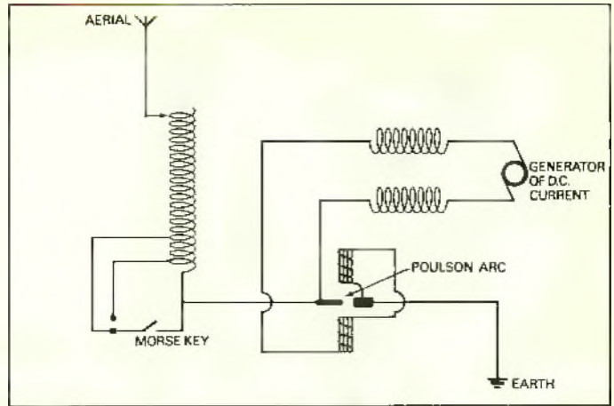
B Poulson Arc Continuous-Wave System, as used by the Federal Telegraph Company of America, c. 1910.
