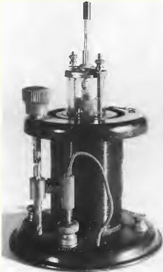
32 Golstone crystal set by Ward & Goldstone Ltd., c. 1925. Moulded ebonite base, and 'archimedean' slide coil tuning. Price 7s 6d (37½p).
