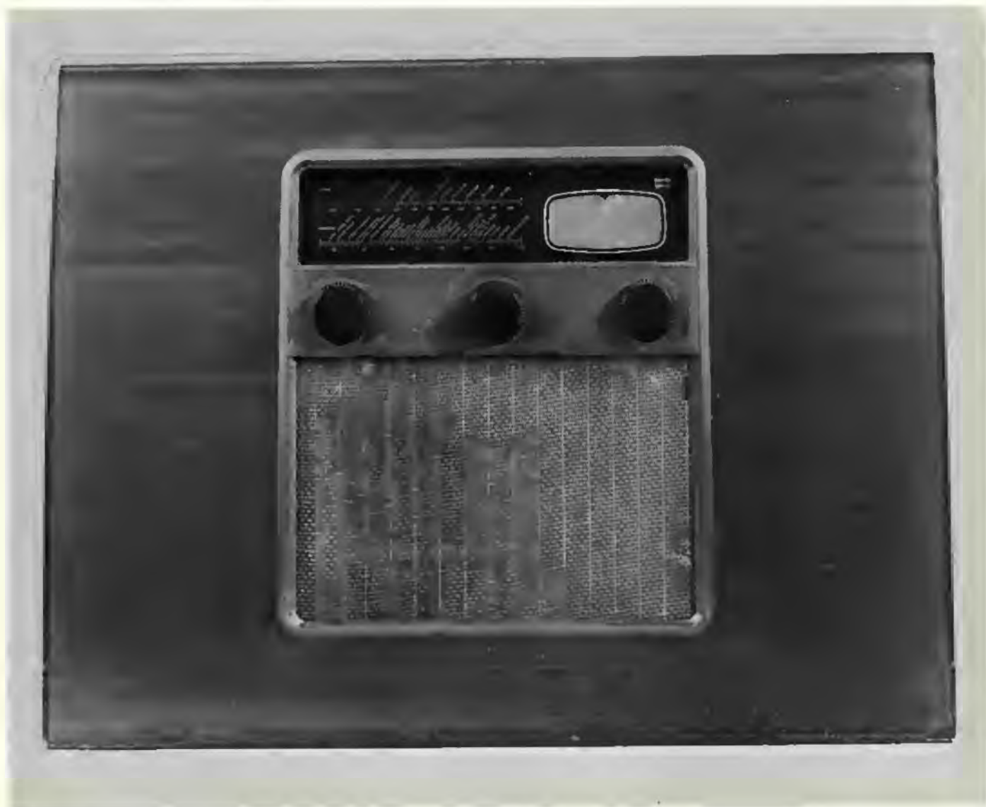
122 Murphy 'Baffle Board' Receiver Type A104, 1946, designed by A. F. Thwaites, and featured in the 'Britain Can Make It' Exhibition of 1946. 24" x 18"; 6 3/4" deep. Four- valve (plus rectifier) A.C. mains superhet.
