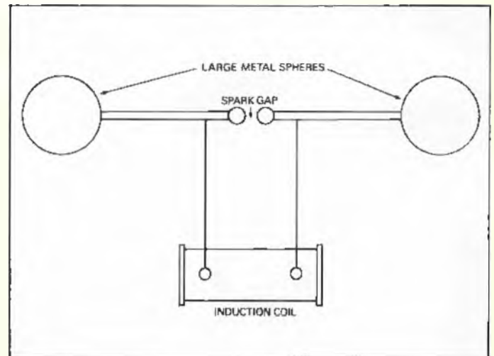
2 The oscillator designed by Hertz.
