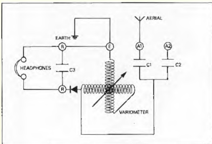
37 Variometer circuit (see ill. 36).
