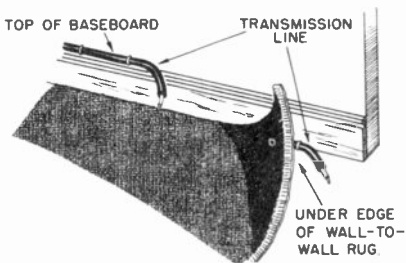
Figure 29. Two methods of running transmission line inside of building.
