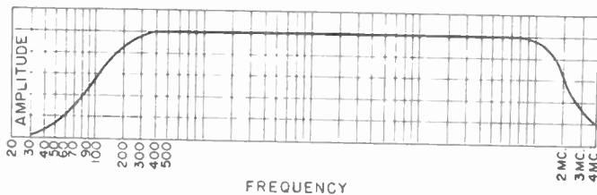
Figure 60. Response curve of video amplifier.
