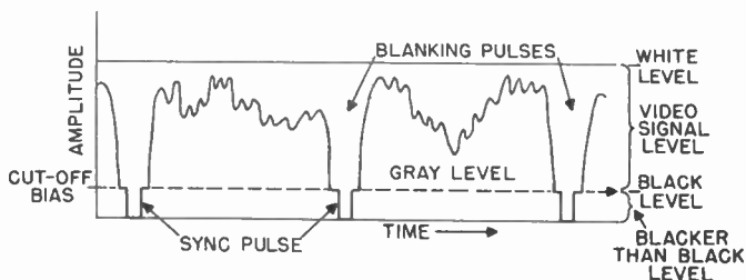
Figure 63. Combined sync, blanking, and video signals.
