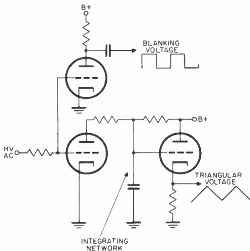
Figure 12. Circuit for generating triangular wave and blanking pulse.
