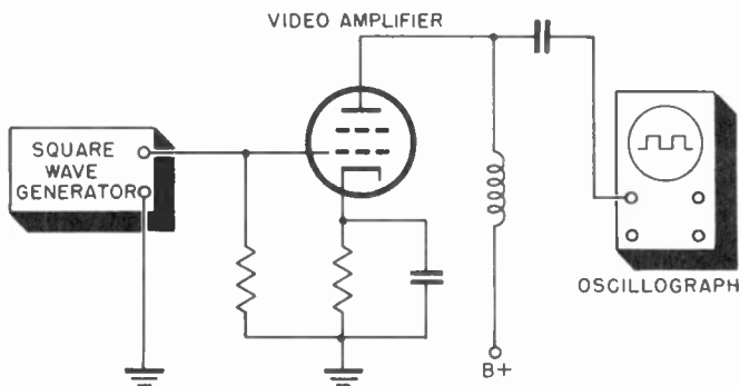
Figure 67. Connections used to adjust video amplifier using square wave generator and oscillograph.
