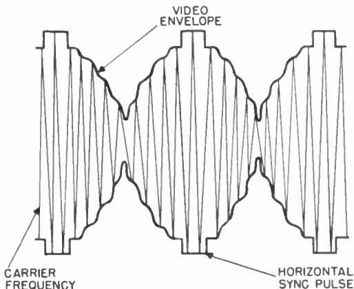
Figure 64. Radio-frequency carrier modulated by the composite video signal. The polarity of the video signal is said to be negative because maximum amplitude of the carrier corresponds to the tips of the sync pulses.
