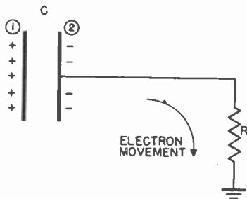
Figure 41. Each globule on the mosaic acts like a condenser.
