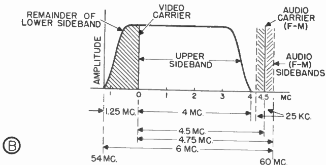
Figure 71B The bandwidth of a television channel is reduced to six megacycles by partially suppressing the lower side-band.
