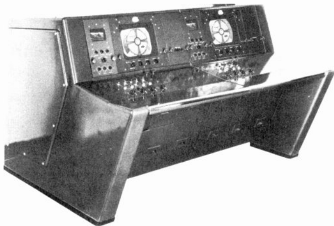
Figure 65. Preview and On-the-Air desks used in master control. (courtesy DuMont)
