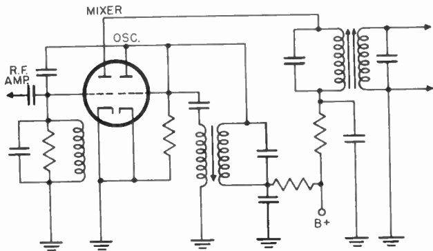
Figure 17. Dual triode mixer-oscillator using grid injection.
