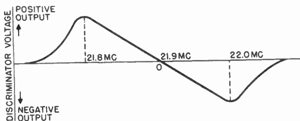
Figure 172. Response curve of typical television receiver discriminator.
