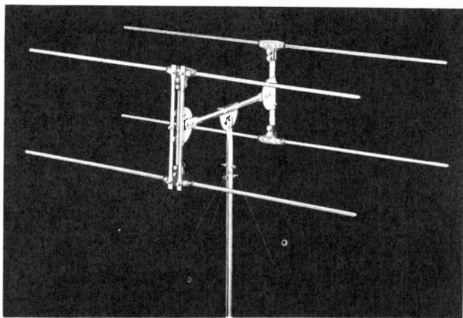
Figure 60. Stacked dipoles and reflectors. (courtesy Camco)
