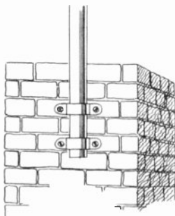
Figure 17. Antenna pole fastened to chimney with two pipe clamps.
