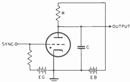
Figure 5. Gas triode sawtooth generator.
