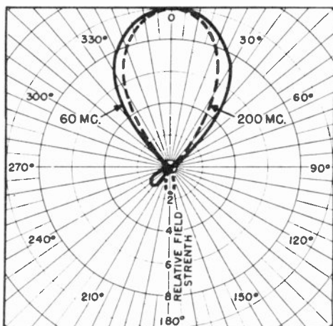
Figure 58. Field patterns of duo-folded dipole at 60 and 200 Mc.
