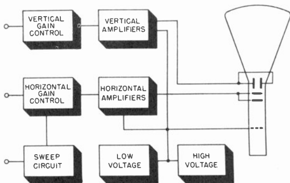
Figure 1. Block diagram of cathode-ray oscillograph.
