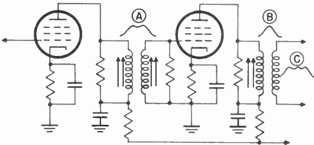
Figure 40. Simplified schematic and response curves of peaked and overcoupled i-f amplifier.
