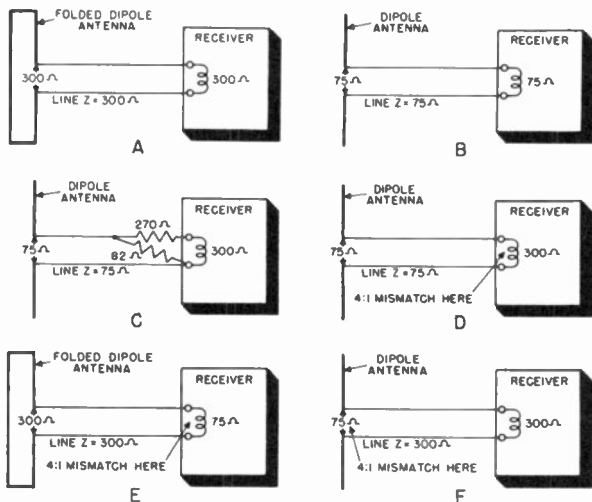
Figure 21. Examples of matched and mismatched antenna systems.
