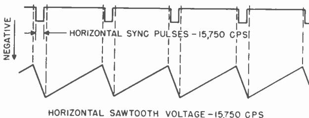
Figure 61. Horizontal sync pulses occur during retrace period of horizontal sawtooth voltage.
