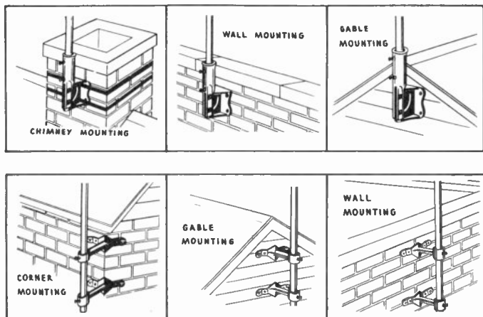
Figure 24. Two types of mounting brackets and the manner in which they are used. (courtesy General Cement).
