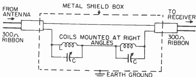
Figure 40. Circuit for wave trap.
