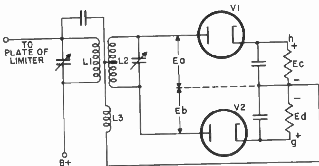
Figure 173. Foster-Seeley discriminator.
