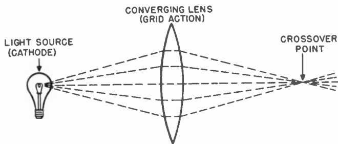
Figure 15. The focusing of an electron beam is similar to the action of a lens on a beam of light.
