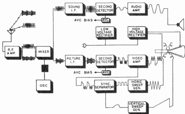
Figure 3. Block diagram of a television receiver with waveforms at input and output of stages.
