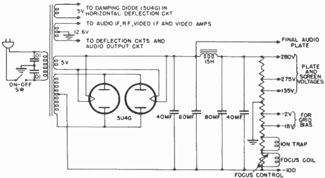
Figure 144. Complete low-voltage supply as used in television receivers.
