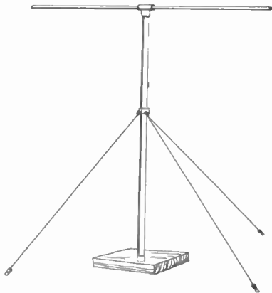
Figure 21. Mounting antenna on a roof.
