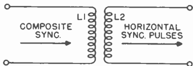
Figure 91. Transformer type differentiating circuit.
