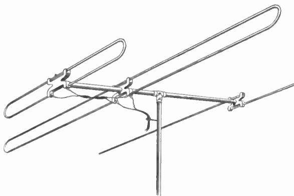
Figure 57. Duo-folded dipole parasitic array.
