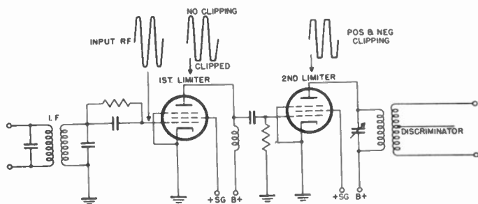
Figure 167. Dual or cascade limiter.
