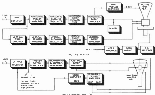
Figure 36. Block diagram of picture and oscillograph monitor.
