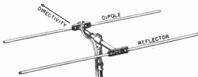
Figure 51. Dipole and reflector.
