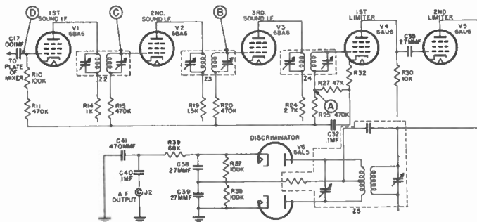
Figure 63. Simplified schematic of sound channel showing points used to connect instruments for alignment.
