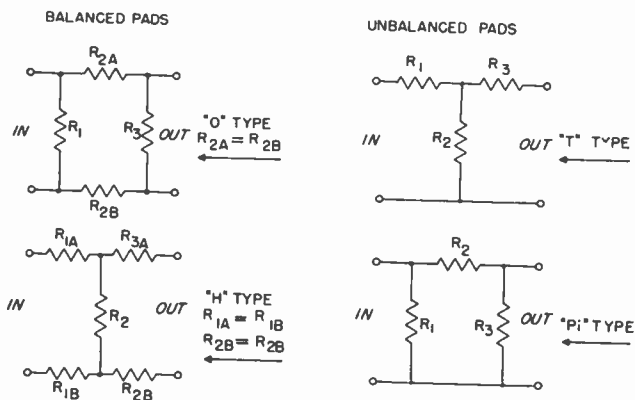
Figure 38. Attenuator network and component values.
