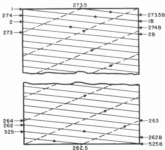
Figure 57. Method of forming interlaced scanning pattern.
