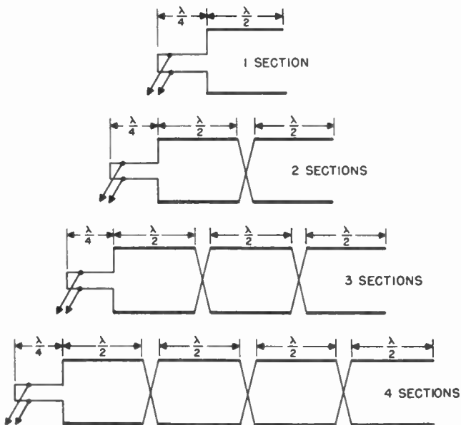
Figure 70. End-fed flat-top antenna arrays (top view).
