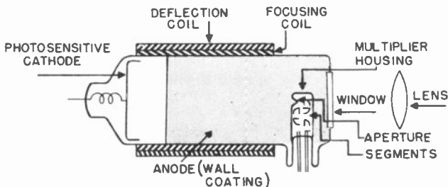
Figure 3. Construction of the image dissector.
