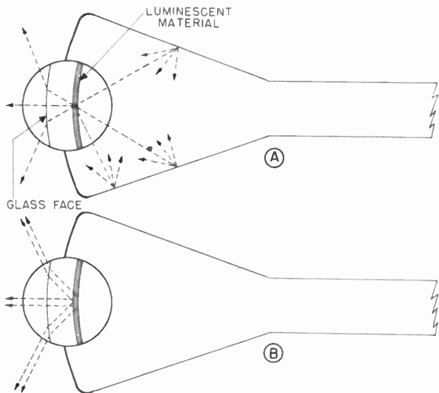
Figure 126. How aluminum backing increases image brightness.
