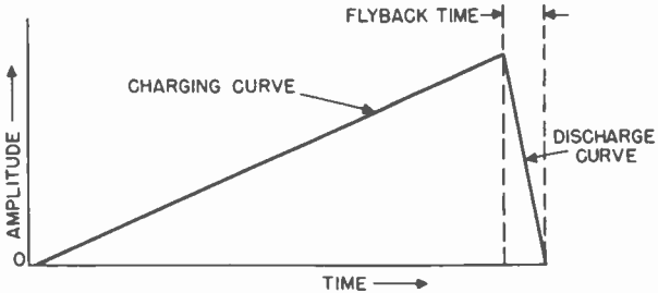
Figure 32. A sawtooth voltage.
