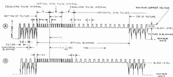
Figure 19. Standard F.C.C. television signal.
