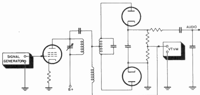
Figure 62. Connections used when checking limiter performance.
