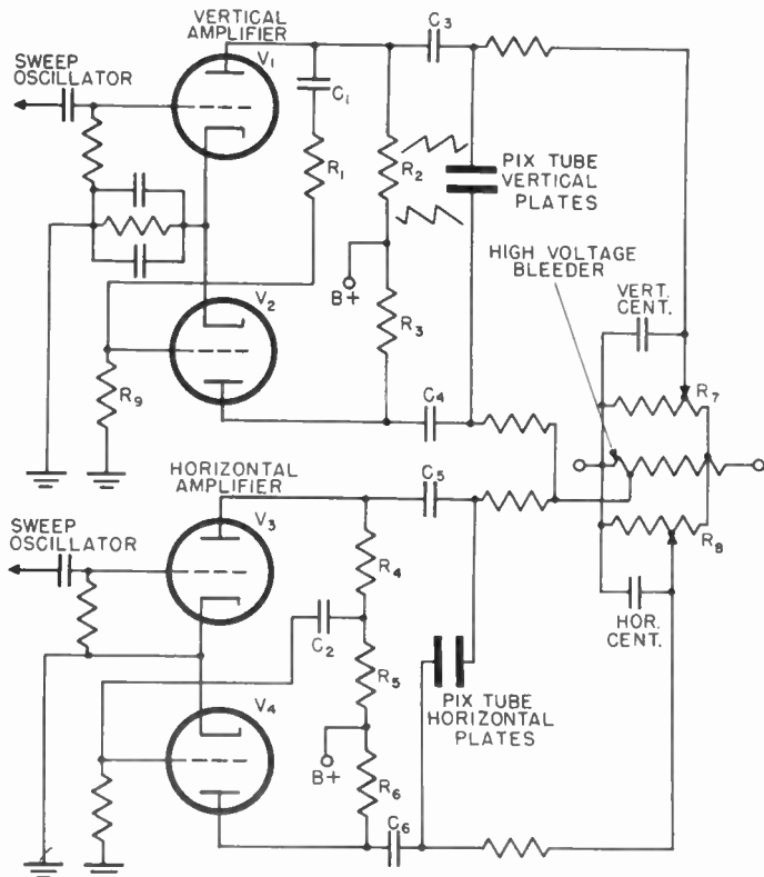
Figure 113. Push-pull vertical and horizontal sync circuits for electrostatic deflection.
