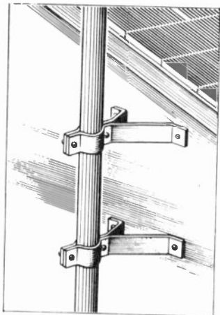
Figure 19. Wall mounting bracket. (courtesy Taco)
