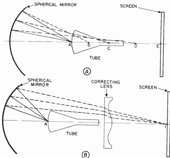
Figure 135. Function of correcting lens in Schmidt projection system.
