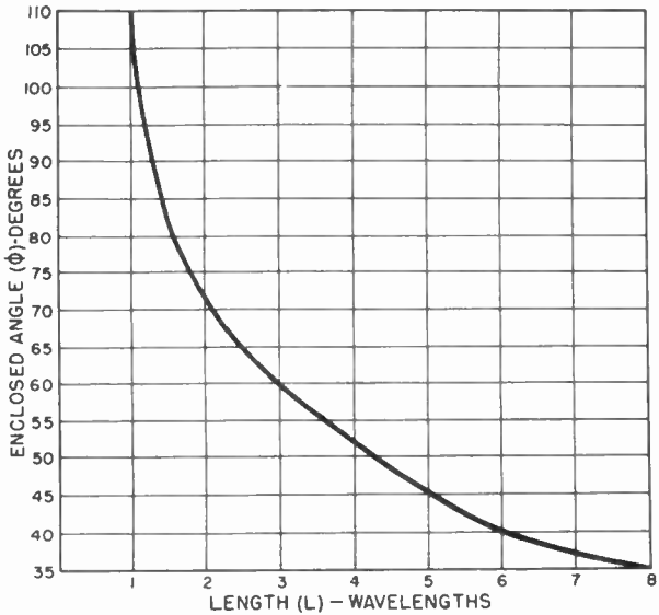
Figure 75. Curve showing change in enclosed angle of V antenna with various frequencies.
