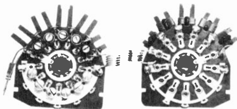
Figure 3. Wafer switches and coils used in RCA tuner. (courtesy RCA)
