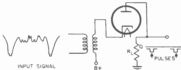
Figure 80. Diode sync clipper.
