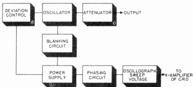
Figure 9. Block diagram of fundamental frequency wobulator.
