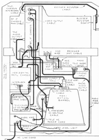
Figure 51. Arrangement of chassis in RCA console Model PTK. (courtesy RCA)
