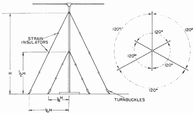
Figure 27. Guy-wire spacing.
