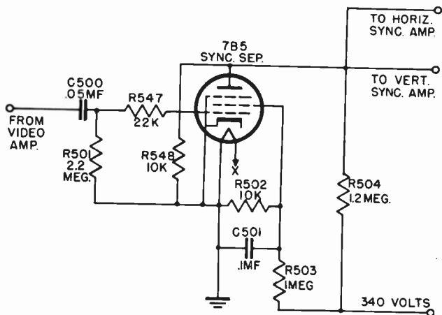
Figure 24. Sync separator.
