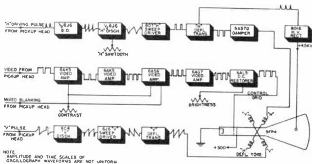
Figure 18. Block diagram of circuits of electronic viewfinder.
