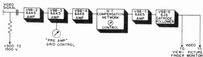
Figure 16. Block diagram of video amplifier used in image orthicon camera.
