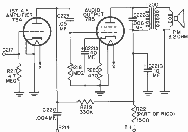
Figure 29. Audio amplifier.
