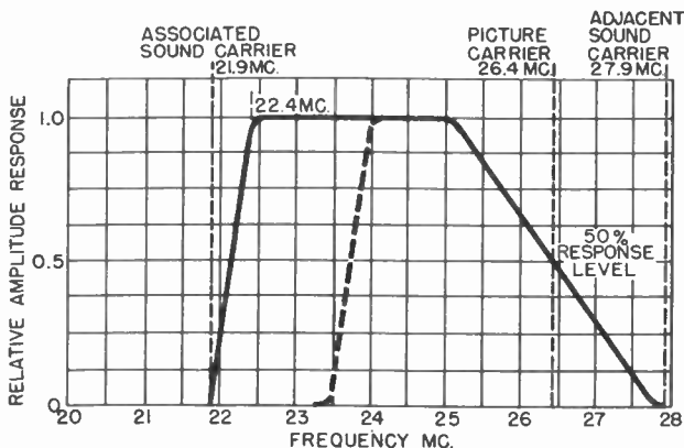
Figure 33. The ideal response curve for a television receiver.
