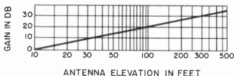
Figure 5. Gain in field intensity of a horizontally polarized dipole antenna when it is raised from low elevation.
