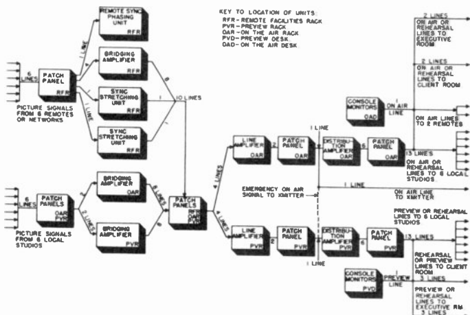
Figure 66. Block diagram of signal paths through station facilities.
