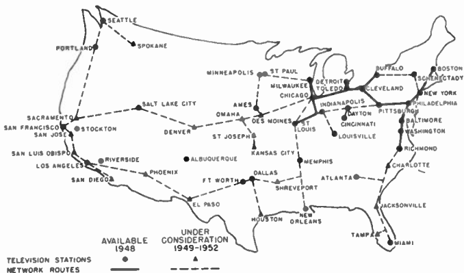
Figure 1. Network routes of the American Telephone and Telegraph Company, showing the cities which will be linked by coaxial cables.
