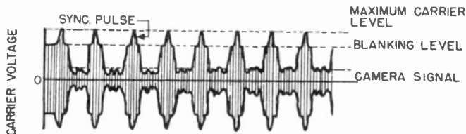
Figure 57. Modulated television carrier.
