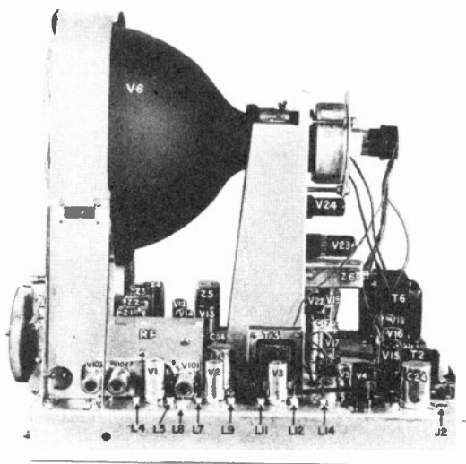
Figure 30. Main chassis of Scott Model 13-A.
