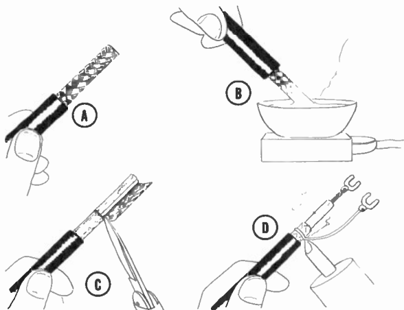
Figure 12. Finishing end of coaxial cable by tinning end of cable and scoring tinned braid. A, cut back rubber insulation. B, dip braid into solder. C, score braid and peel off. D, attach lead and lug to braid.
