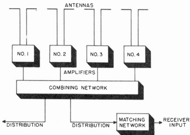
Figure 84. Block diagram of Intra-Video master antenna system.
