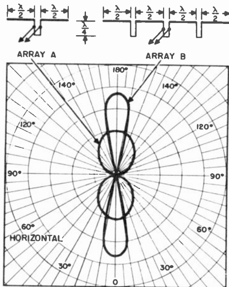
Figure 64. Two types of collinear phased arrays.
