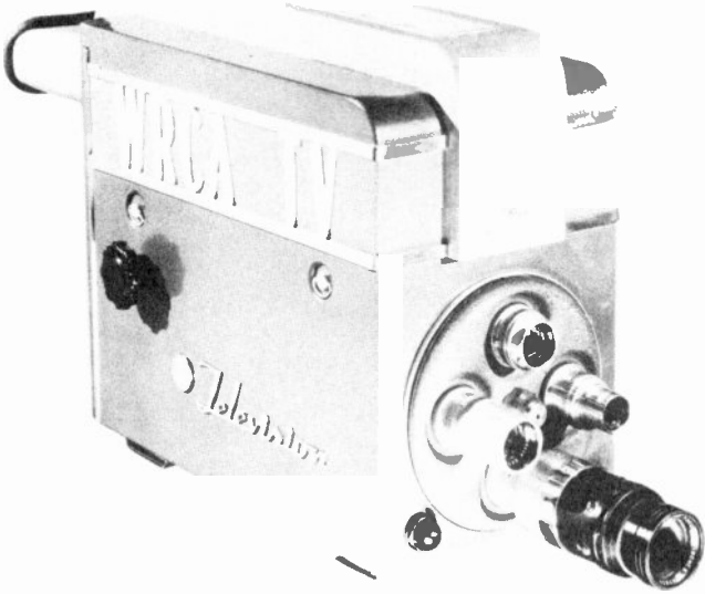
Figure 6. Image orthicon camera. (courtesy RCA)
