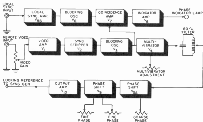
Figure 68. Block diagram of sync phasing unit.
