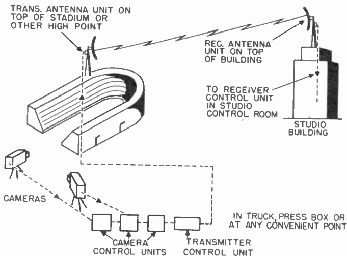
Figure 106. Microwave relay from remote pickup point to studio.
