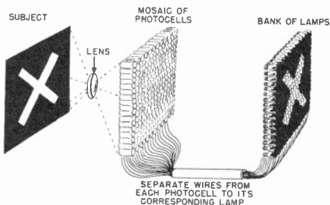
Figure 6. The Carey television system.
