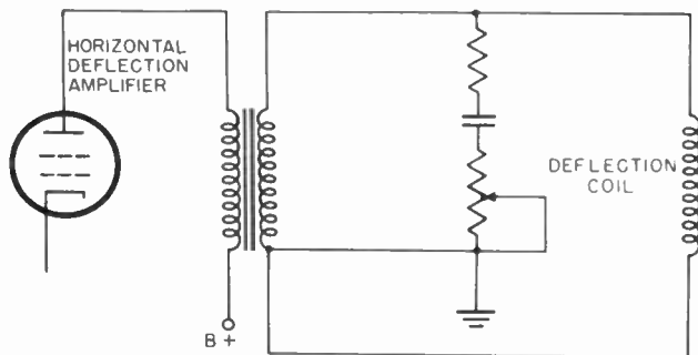
Figure 121. Simplified schematic of damping circuit using resistor and capacitor.
