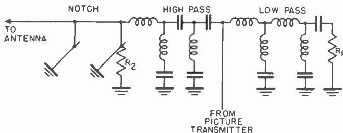
Figure 47. Vestigial sideband filter.
