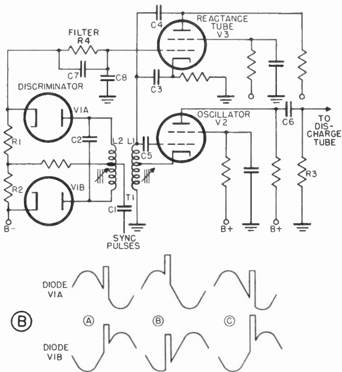
Figure 100. Automatic frequency control circuit which eliminates need for manual hold control.
