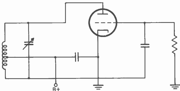
Figure 10. Series-fed Hartley oscillator.
