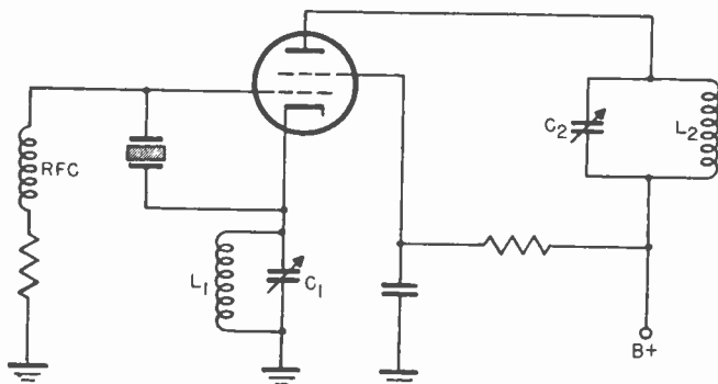
Figure 44. Tri-tet oscillator.
