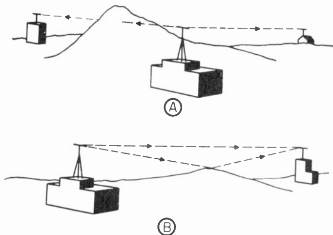
Figure 10. (A) Television signal weakened by intervening hill. (B) Multipath reflection caused by a "bounce" signal.
