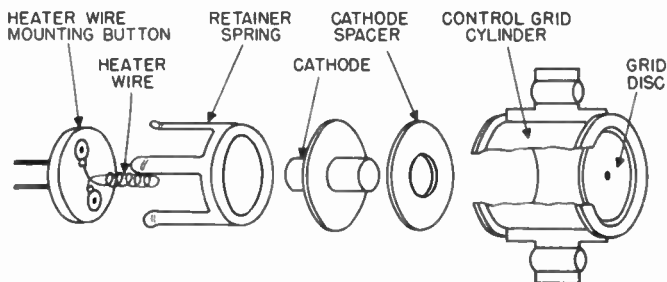
Figure 6. The cathode-grid assembly.
