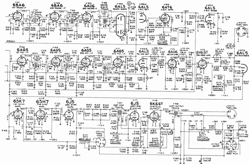
Figure 53. Video, sound, and vertical sweep circuits.
