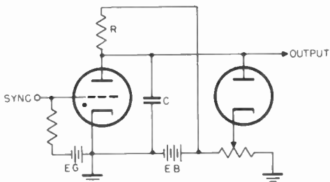
Figure 6. Gas triode circuit for generating driven or triggered sweep.
