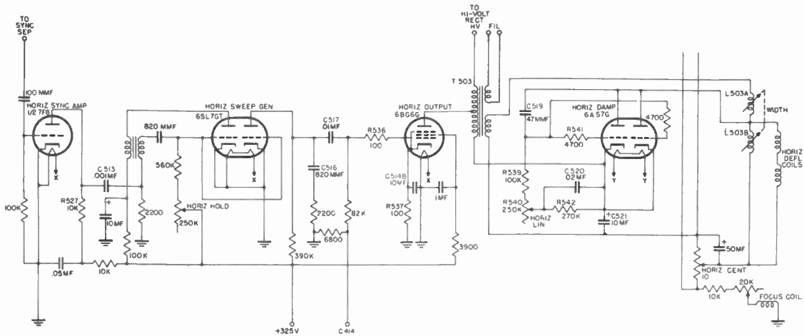
Figure 26. Horizontal-deflection circuits.
