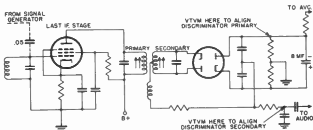
Figure 57. Connections used when aligning ratio detector using v.t.v.m.
