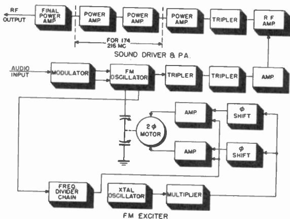
Figure 112. Block diagram of RCA sound transmitter.
