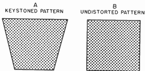
Figure 47. A shows a keystone pattern. B shows correct scanning pattern, obtained on mosaic when keystone distortion is eliminated.
