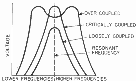
Figure 38. Effect of coupling on the response of a tuned circuit.
