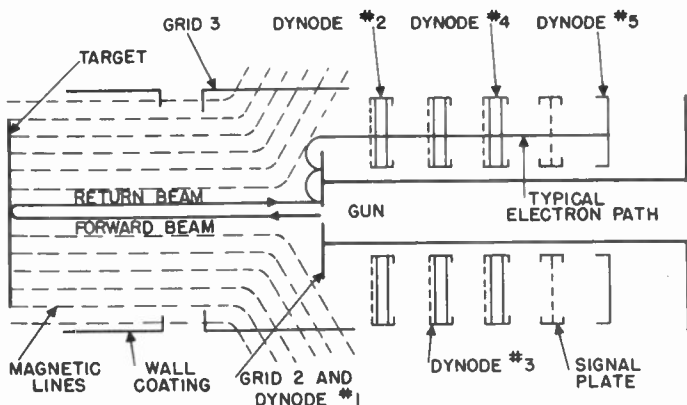
Figure 10. Electron Multiplier Section of the image orthicon.
