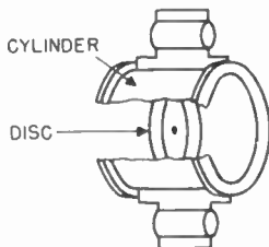
Figure 9. The accelerating electrode assembly.
