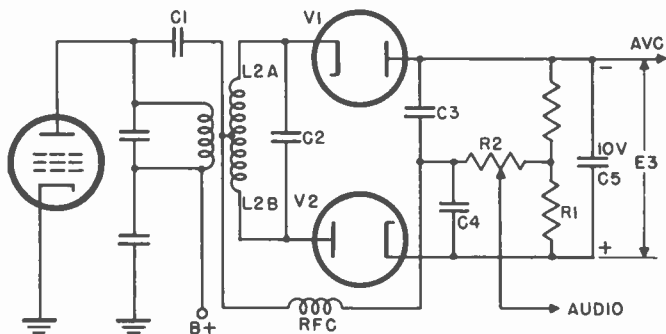
Figure 175. Simple ratio detector.
