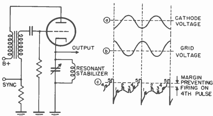
Figure 24. Stabilized blocking oscillator frequency divider.
