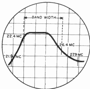
Figure 46. Video i-f response curve using tuned circuits only.
