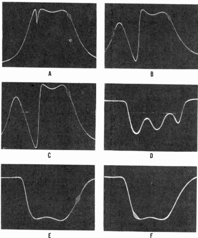
Figure 73. Response curves obtained when aligning video i-f amplifiers.
