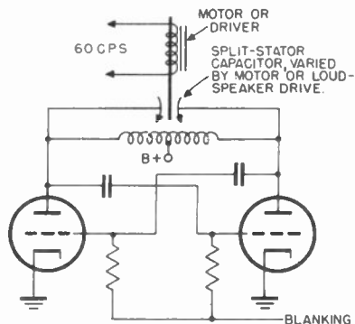
Figure 10. Variable capacitor circuit for wobulator.
