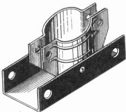
Figure 22. Mast base. (courtesy Taco)
