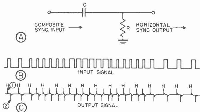
Figure 88. A, differentiating circuit. B, input and output waveforms of circuit in A.
