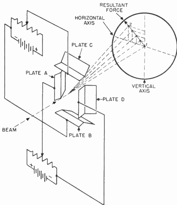
Figure 29. The horizontal and vertical deflection plates, with separate sources of voltage connected to them.
