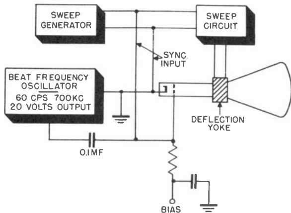
Figure 50. Method used to check linearity of scanning circuits.
