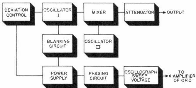
Figure 11. Block diagram of beat frequency wobbulator.
