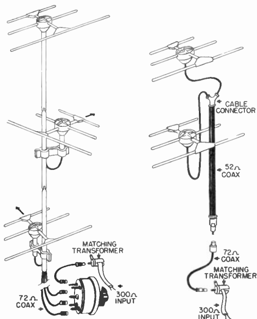
Figure 44. Typical application of coaxial switch.
