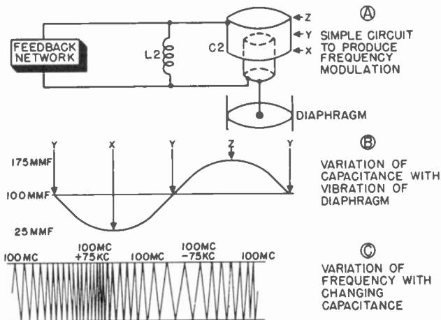
Figure 158. Simple method of frequency modulation.
