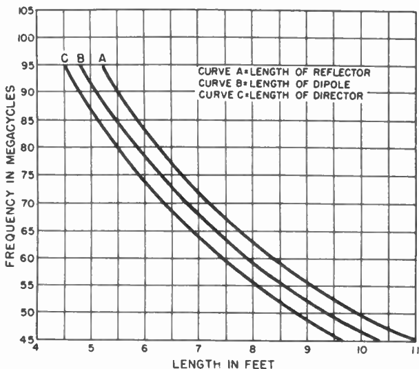
Figure 52. Curves showing length in feet of dipole, reflector, or director for frequencies between 45 and 95 Mc.
