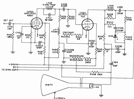
Figure 23. Video amplifier.
