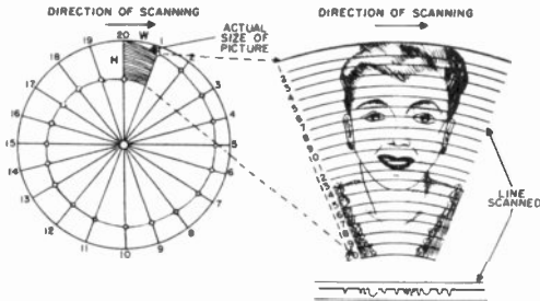
Figure 10. Rotating disc used in Nipkow's television system.
