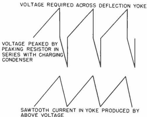
Figure 52. Voltage and current waveforms required for magnetic deflection.
