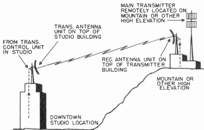
Figure 105. Typical use of microwave relay equipment between studio and transmitter.
