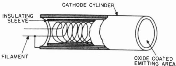
Figure 12. Heater and cathode assembly.
