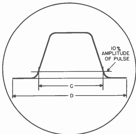
Figure 120. Sine wave sweep method of measuring pulse duration.
