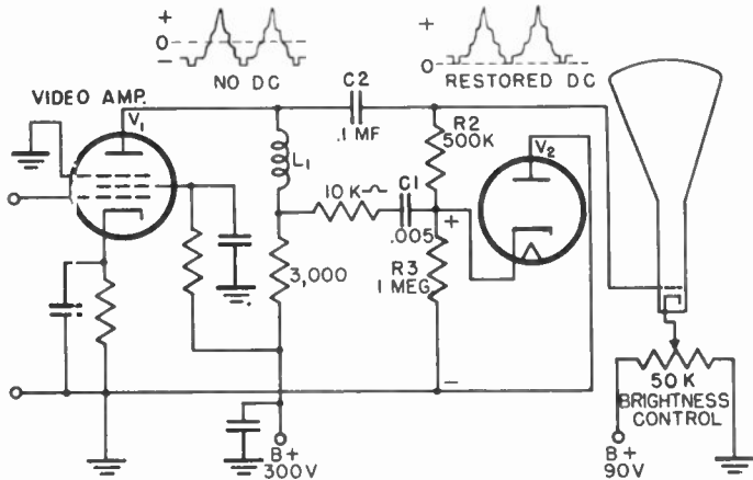
Figure 71. Schematic of diode d-c restorer.
