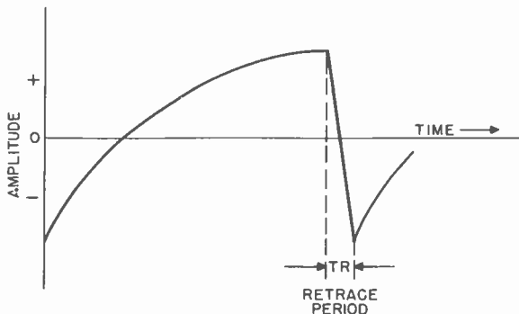
Figure 56. Shape of sawtooth voltage which produces non-linear pattern shown in Figure 55.
