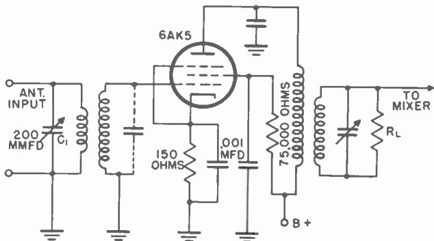
Figure 5. Pentode r-f amplifier.
