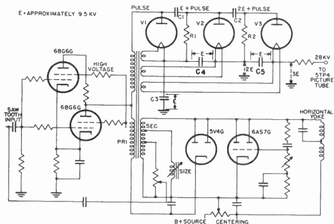
Figure 155. Kickback high-voltage supply for projection receiver.
