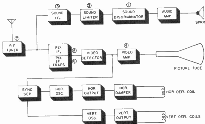
Figure 55. Order in which sound and video circuits are aligned.
