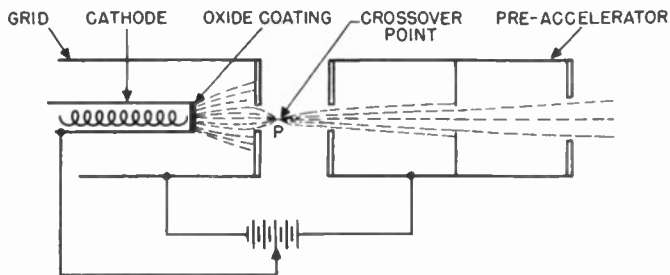
Figure 14. The "crossover" point of the electron beam is between the grid and the pre-accelerator electrode.
