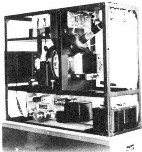
Figure 96. Iconoscope film pickup camera without shield covers. (courtesy DuMont)
