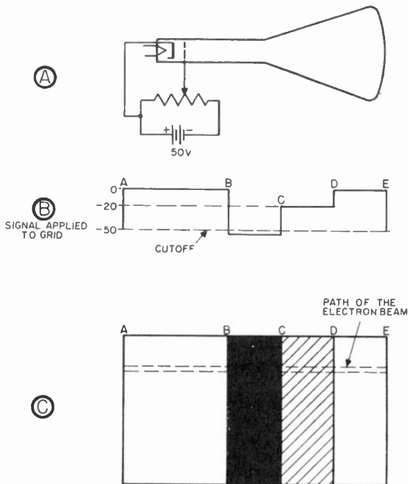
Figure 37. Forming an image on the screen.
