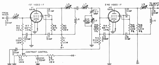
Figure 77. Gain control by varying the grid bias on remote cutoff pentode i-f amplifiers.
