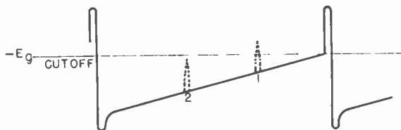
Figure 95. Horizontal sync pulse (1) is of sufficient amplitude to trigger oscillator. Equalizing amplitude at (2) does not trigger oscillator because of position on grid voltage curve.
