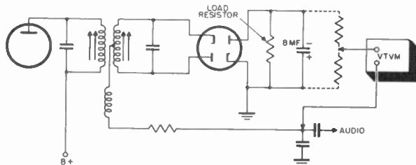
Figure 58. Use of series resistors to obtain midpoint when aligning ratio detector.
