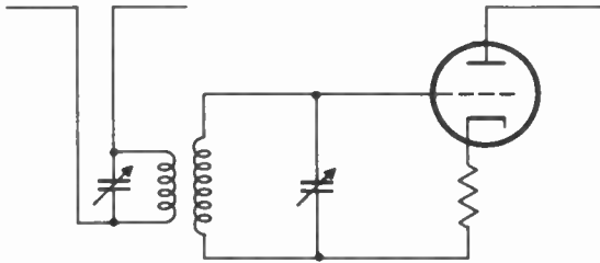
Figure 29. Antenna coupling circuit using tuned primary and secondary.
