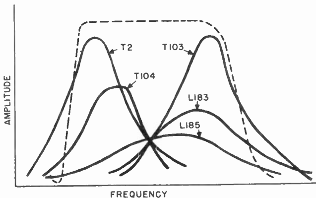
Figure 54. Relative gain and selectivity of each coil in staggered i-f amplifier. Resulting overall response curve is shown dotted in background.
