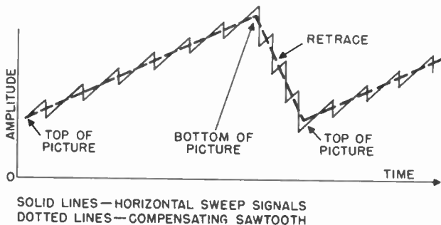
Figure 48. Compensating signal for overcoming keystone.
