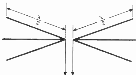
Figure 44. Full-wave fan antenna.
