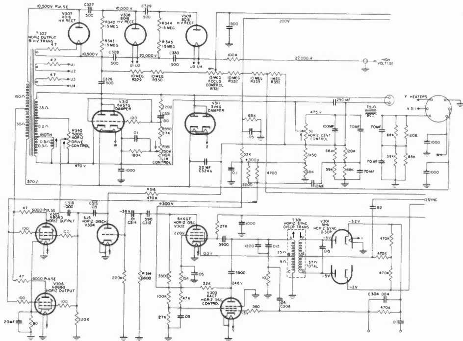
Figure 56. Horizontal deflection circuit and high voltage power supply.
