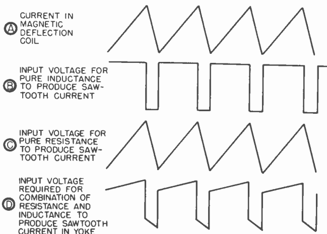
Figure 114. Waveforms of current and voltage in magnetic deflection systems.
