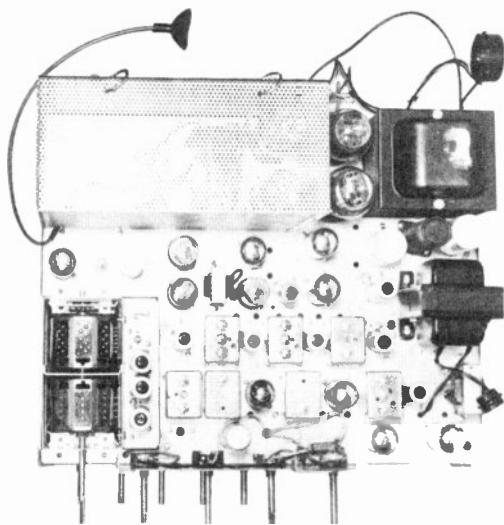
Figure 20. Chassis layout of Philco Model 48-1000. (courtesy Philco)
