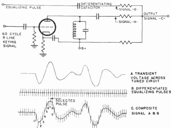
Figure 30. Forming the 60-cycle, three-line keying signal.
