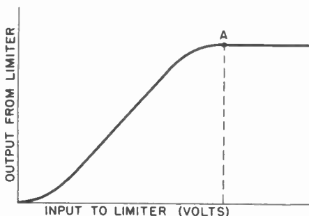
Figure 61. Limiter curve.
