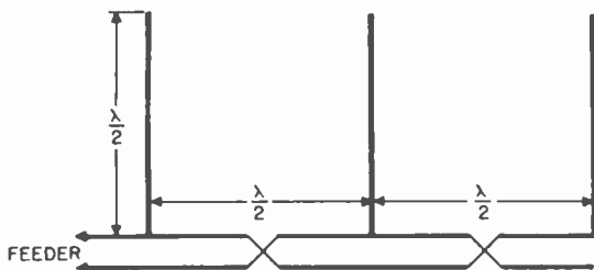
Figure 65. Broadside array.
