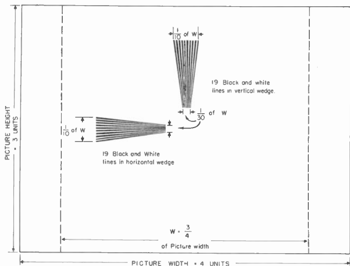
Figure 3. Method used to compute calibration numbers on resolution wedges.
