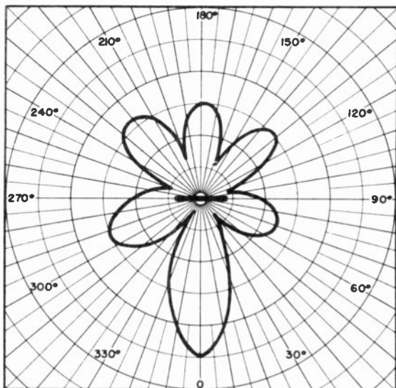
Figure 41. Field pattern of bat-wing antenna at 180 Mc.
