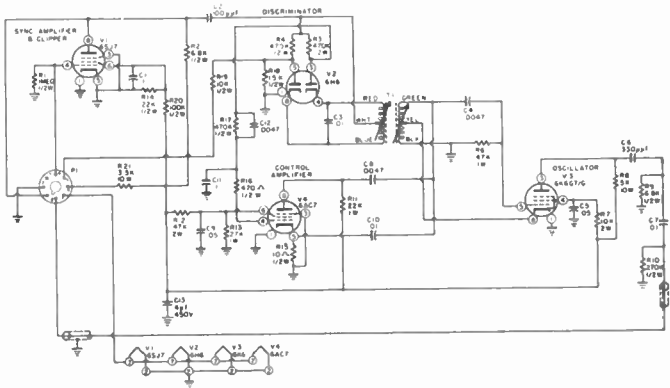
Figure 49B. Sync stabilizer schematic.
