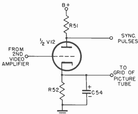
Figure 18. Sync separator and d-c restorer.
