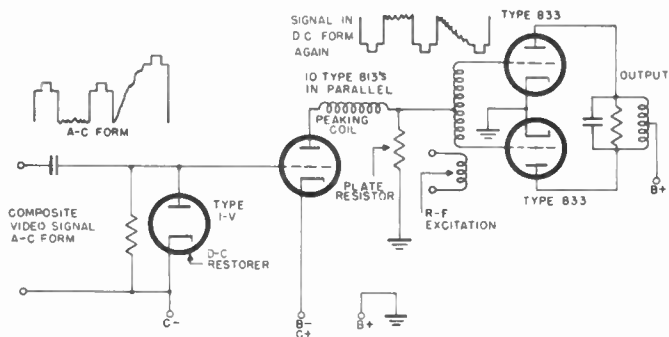
Figure 56. D-C reinsertion in grid circuit of video modulator
