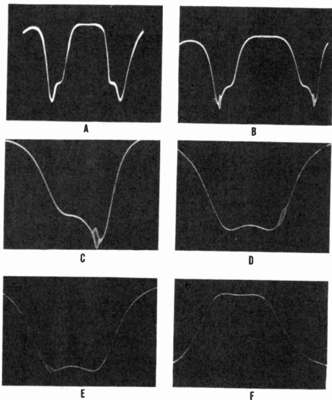
Figure 72. Response curves obtained when aligning video i-f amplifiers. A. Dual response curve, B. Birdie at 26.4 Mc, C. Single response curve, D. Birdie 1 db down from flat top, E. Birdie at 22.4 Mc, F. Birdie at 26.4 Mc.
