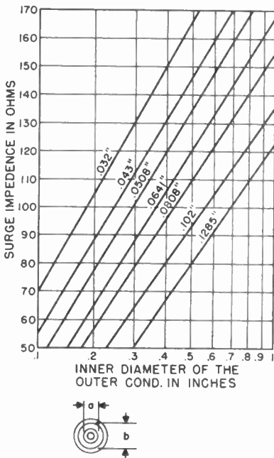
Figure 19. Characteristic impedance of coaxial transmission lines.
