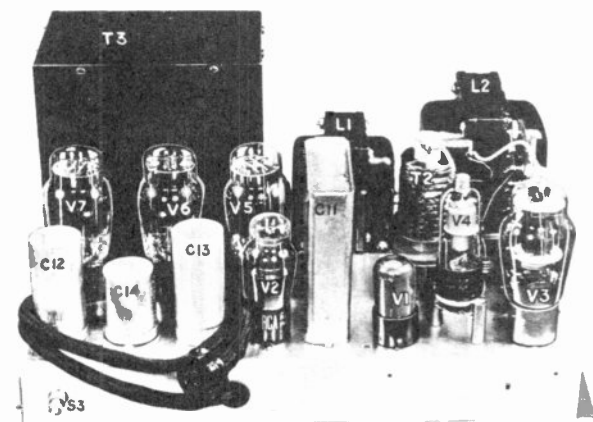
Figure 31. Power supply chassis.
