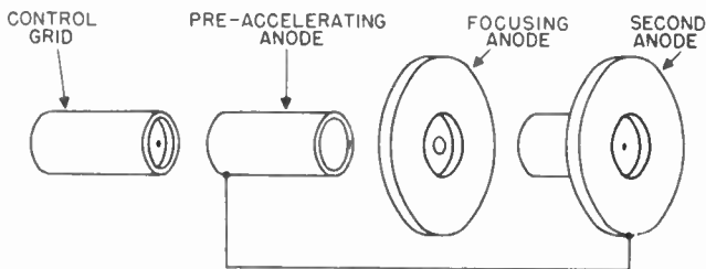
Figure 16. The pre-accelerator electrode is inserted between the control grid and the focusing anode.
