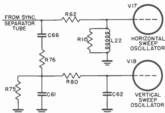
Figure 19. Networks for separating horizontal and vertical sync pulses.
