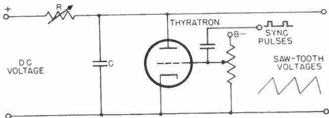
Figure 107. Thyatron saw-tooth generator circuit.
