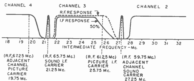
Figure 35. The relationship between the response of a television receiver, the television signal, and signals in adjacent channels.
