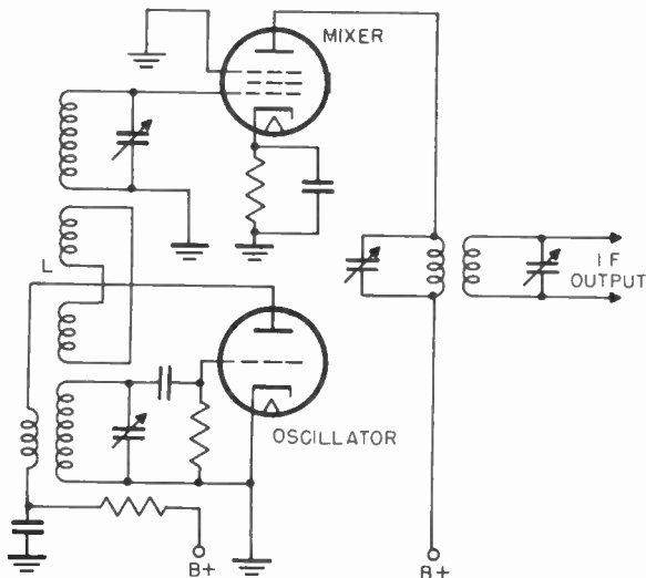
Figure 15. Inductively-coupled mixer-oscillator.
