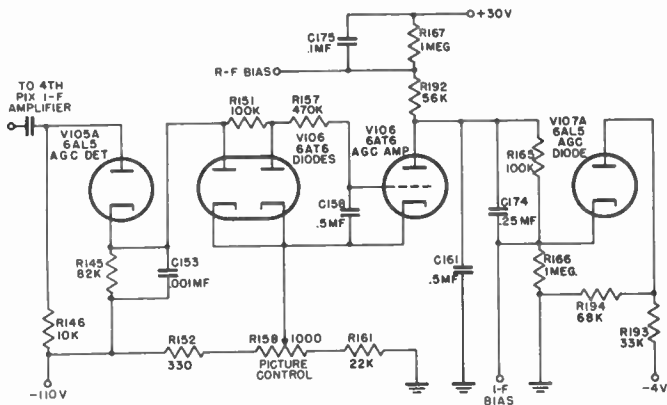
Figure 55. A.G.C. circuit.
