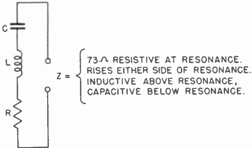
Figure 30. Equivalent circuit of a dipole antenna.
