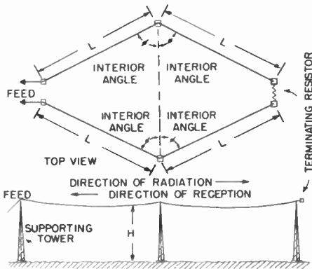
Figure 76. Rhombic antenna.
