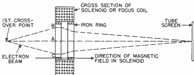
Figure 25. Focusing of an electron beam by a magnetic field inside of a solenoid.
