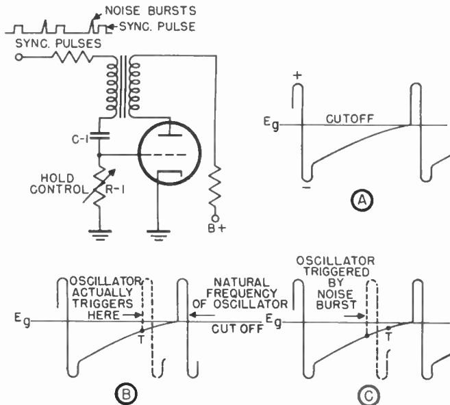
Figure 98. How noise affects the operation of blocking oscillator circuit.
