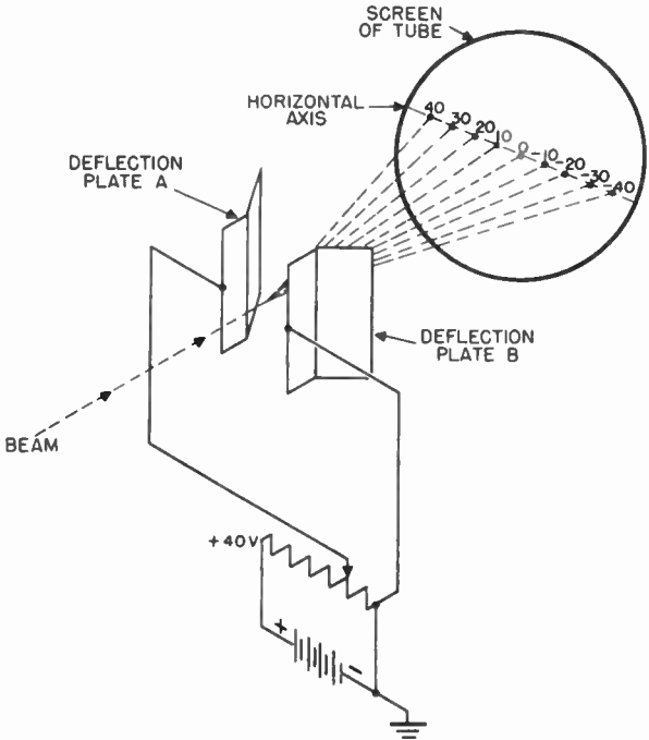
Figure 28. The electron beam is moved horizontally when a d-c potential is applied to the horizontal deflection plates.
