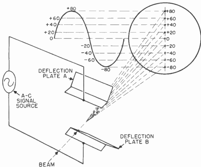
Figure 30. The electron beam traces out a vertical line when a high frequency sine wave is applied to the vertical deflection plates.
