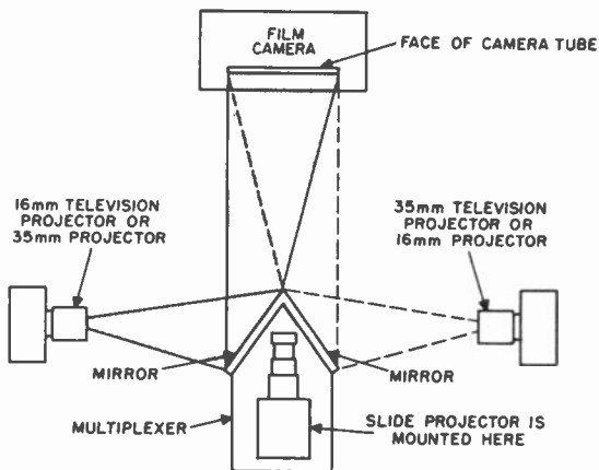
Figure 99. Physical layout of film multiplexer.
