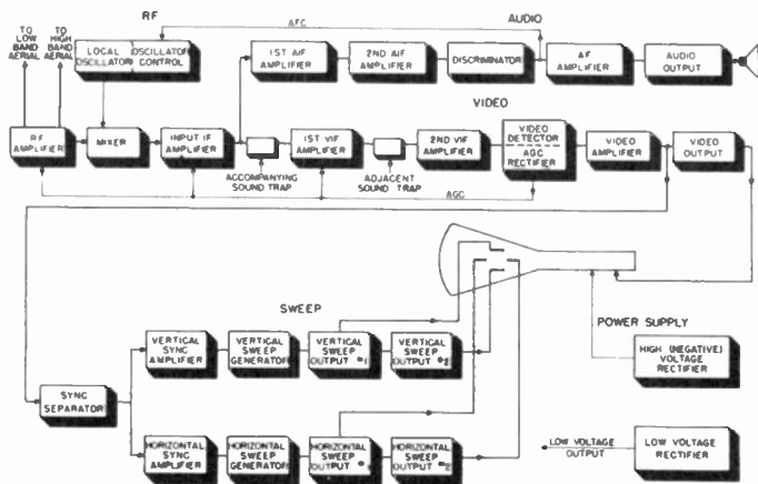
Figure 180. Block diagram of television receiver using seven-inch tube.
