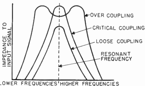
Figure 25. The effect of coupling on the response of a tuned circuit.
