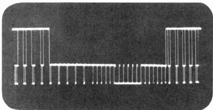
Figure 122. Vertical blanking interval. (courtesy DuMont)
