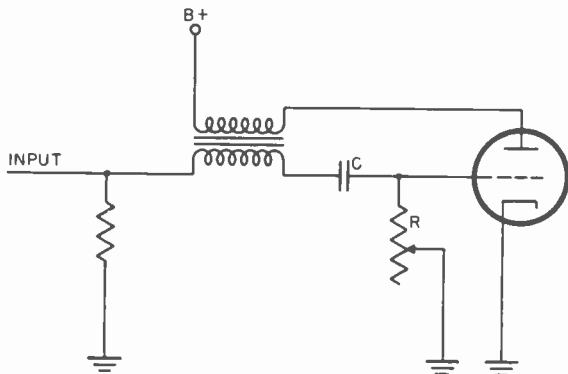
Figure 93. Blocking oscillator circuit.
