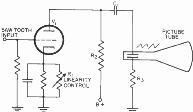
Figure 111. Sweep amplifier for use with electrostatic deflection.
