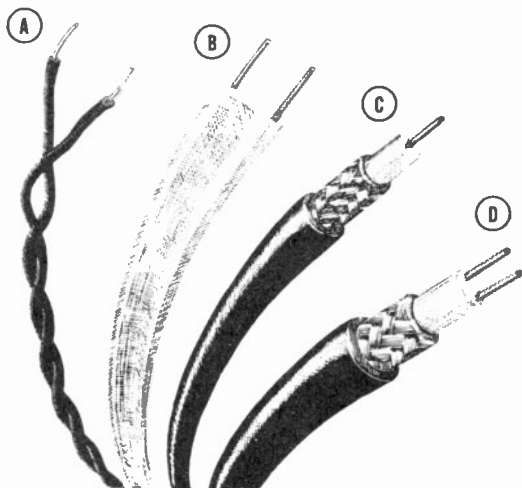
Figure 16 Four types of transmission lines. (A) Twisted pair. (B) Two-wire line (C) Coaxial line. (D) Shielded pair.
