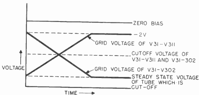
Figure 78. Curve of bias changes which occur in switching amplifiers.
