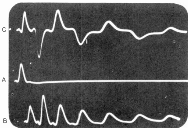
Figure 131. Oscillograms showing patterns obtained for properly and improperly matched transmission line.
