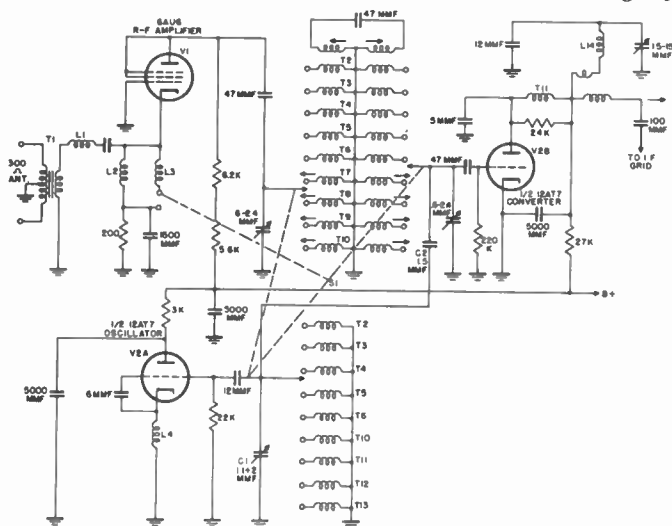
Figure 4. Schematic diagram of G.E. tuner.
