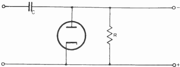
Figure 55. Circuit of diode d-c restoration circuit.
