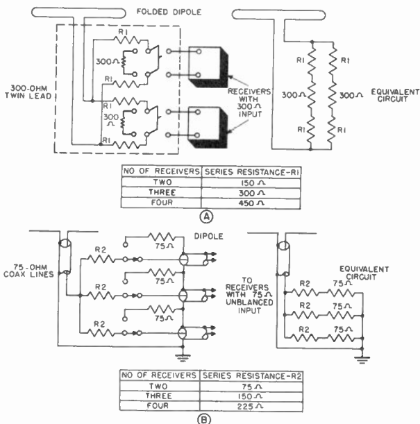
Figure 87. Simple master antenna system.
