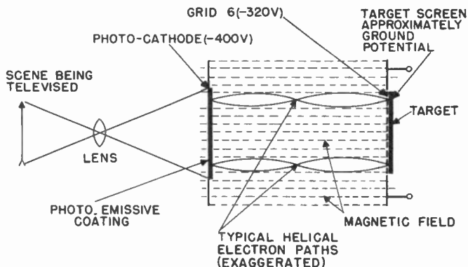
Figure 8. Multiplier section of the image orthicon.
