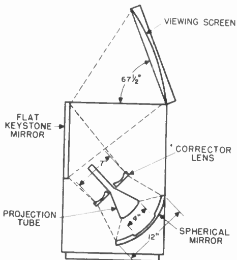
Figure 138. The Philco version of the Schmidt optical system.
