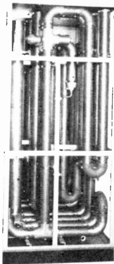
Figure 110. Vestigial sideband filter. (courtesy RCA)
