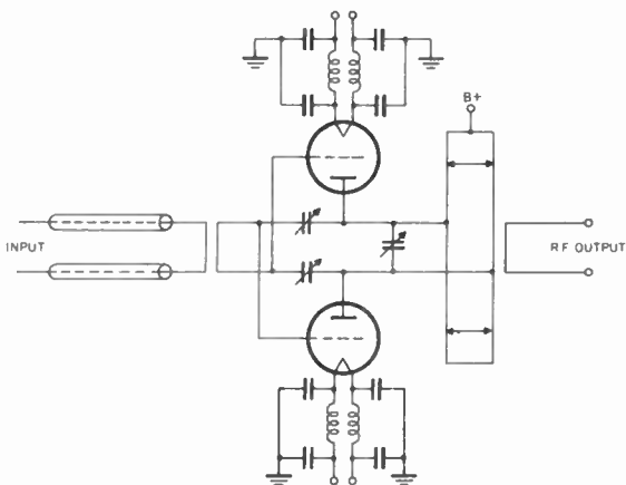
Figure 50. Wideband r-f amplifier circuit.
