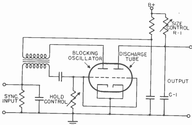
Figure 110. Blocking oscillator discharge circuit using dual triode.
