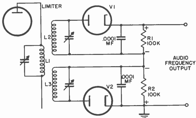
Figure 170. Simple discriminator circuit.
