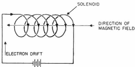
Figure 24. Direction of magnetic field in a solenoid.
