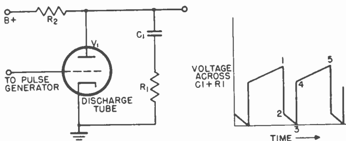
Figure 115. Discharge tube with peaking circuit.
