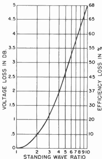
Figure 15. Curve showing the voltage loss in db and the efficiency loss in percent for various standing wave ratios.
