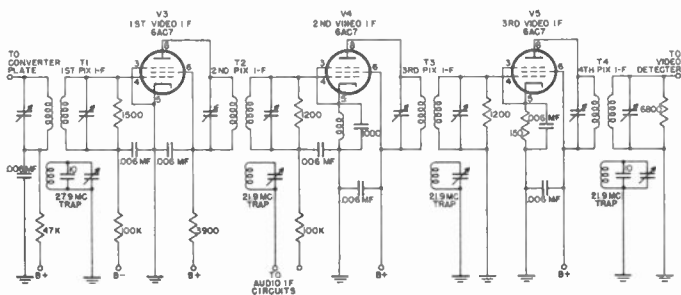
Figure 50. Overcoupled i-f amplifier with wavetraps.
