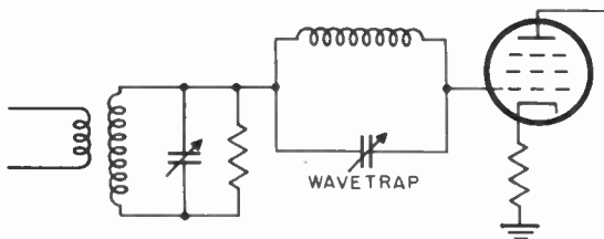
Figure 47. Simplified circuit of i-f amplifier with grid wave-trap.
