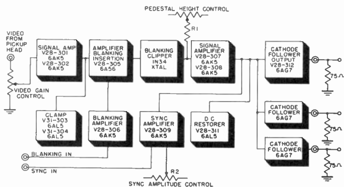
Figure 37. Block diagram of mixing and distribution amplifier.
