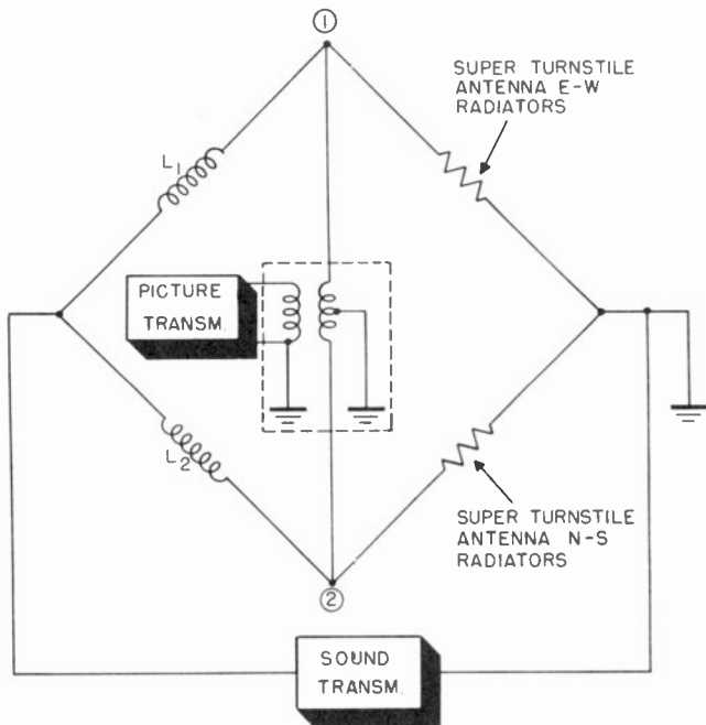
Figure 58. Circuit of diplexer.
