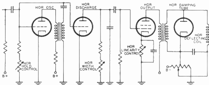
Figure 119. Simplified schematic of horizontal sweep circuit with damping tube.
