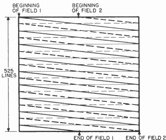
Figure 53B Interlaced scanning pattern.
