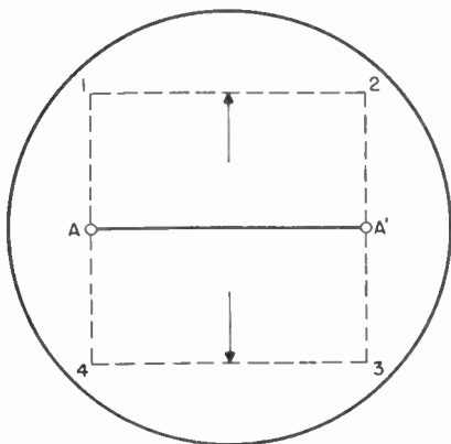
Figure 31. Raster pattern traced out by two sine waves, of equal amplitude, but of different frequency, which are applied to the vertical and horizontal deflection plates.
