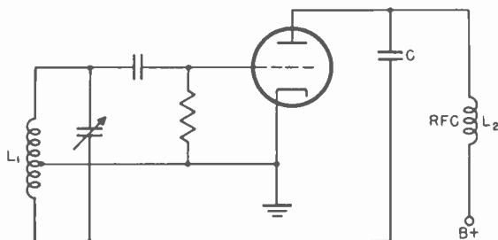
Figure 9. Shunt-fed Hartley oscillator.
