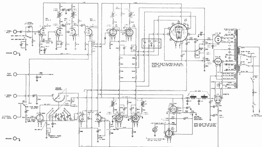
Figure 8. Schematic circuit of Du Mont Type 208B.
