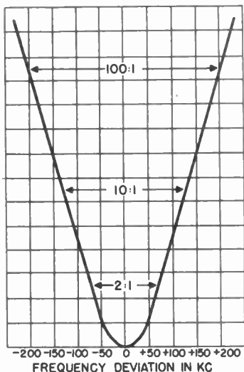
Figure 162. Typical i-f amplifier response curve.
