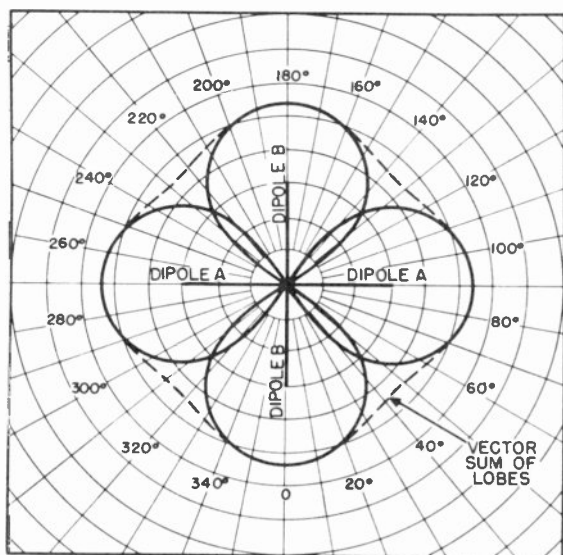
Figure 34. Horizontal field pattern of crossed dipole antenna.
