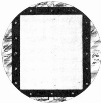
Figure 40. The mosaic of an iconoscope tube.
