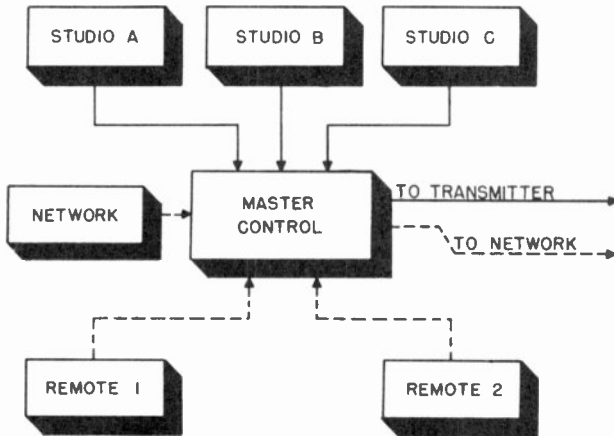
Figure 63. Block diagram of facilities of a small television station.
