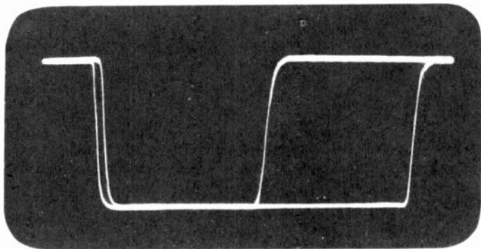
Figure 125. Superimposed horizontal sync pulse and equalizing pulse used to check interlace.
