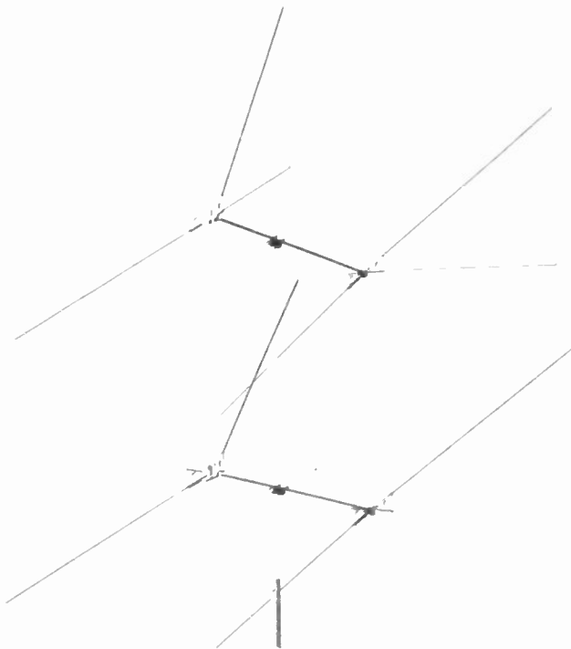
Figure 62. Four-unit double-V stacked antenna. (courtesy Telrex)
