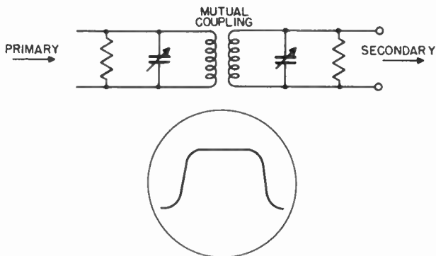
Figure 49. Overcoupled circuit and its response characteristic.
