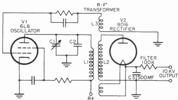
Figure 146. Circuit of an r-f high-voltage power supply.
