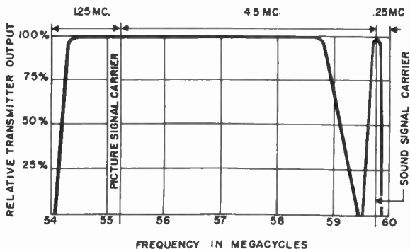
Figure 4. A typical television channel.
