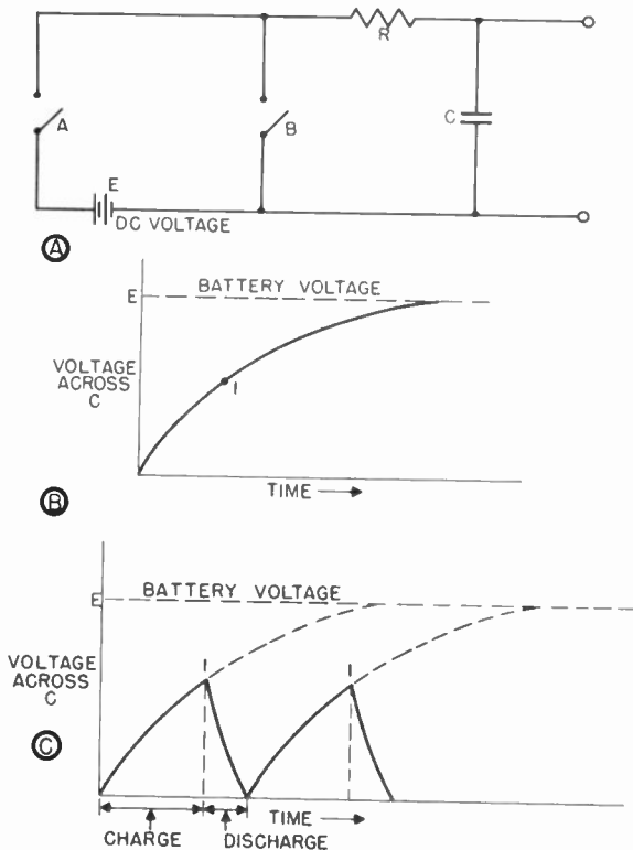
Figure 104. Simple method for producing saw-tooth voltage.
