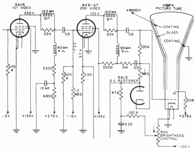
Figure 65. Two stage video amplifier using shunt and series peaking.
