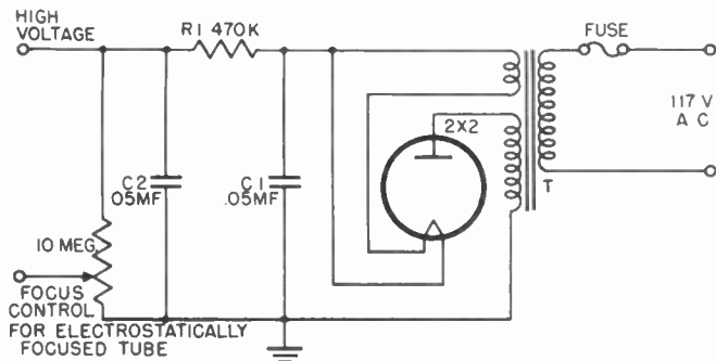
Figure 145. Circuit of a 60-cycle, high-voltage supply.
