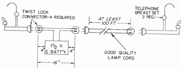
Figure 7. Battery-operated phone system.
