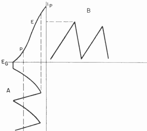
Figure 112. Removal of non-linearity from saw-tooth by operating on curved portion of characteristic curve.
