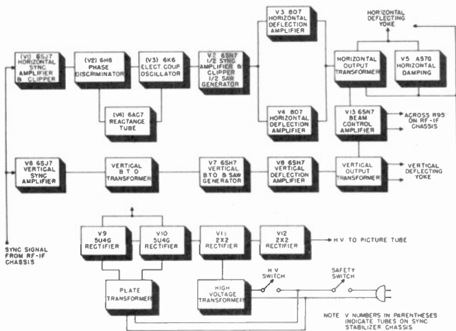
Figure 48. Block diagram of sweep chassis.
