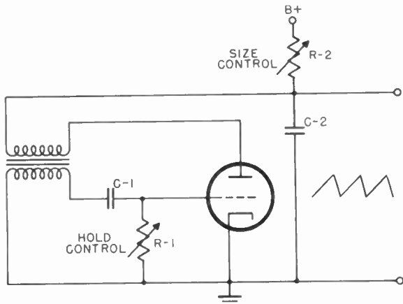
Figure 109. Blocking oscillator and discharge circuit.
