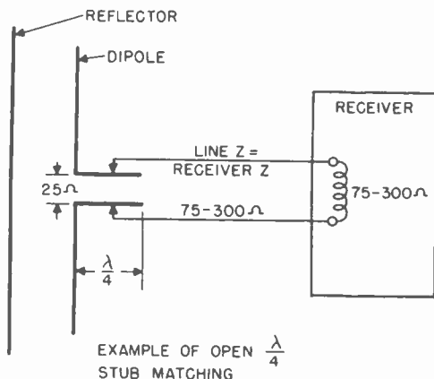
Figure 23. Quarter-wave stub matching section.
