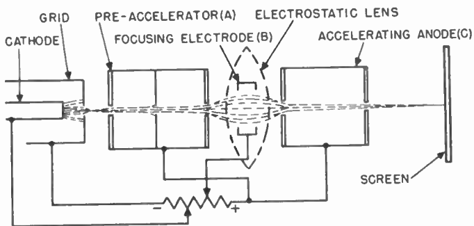
Figure 18. The electrostatic field inside the focusing electrode focuses the electron beam to a second crossover point.
