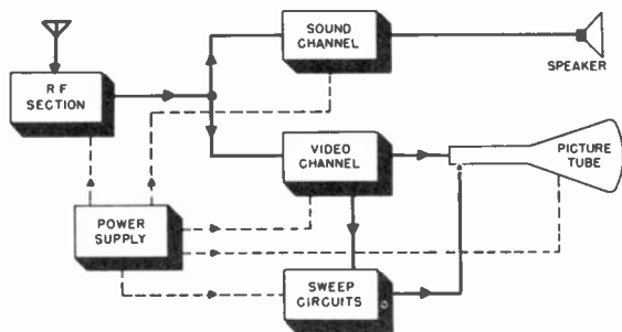
Figure 1. Block diagram of six basic sections of television receiver.
