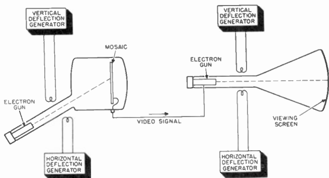
Figure 49. A simplified television system.
