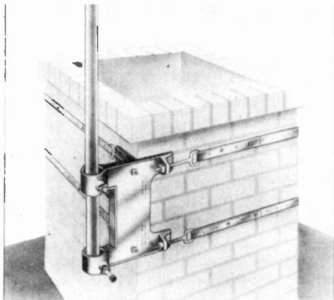
Figure 18. Chimney mounting bracket. (courtesy South River Metal Products)
