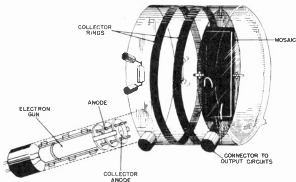
Figure 39. Construction of the Iconoscope.
