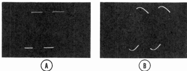
Figure 69. Square wave patterns obtained when checking low-frequency response of video amplifier. A. Good low-frequency response, B. Poor low-frequency response.
