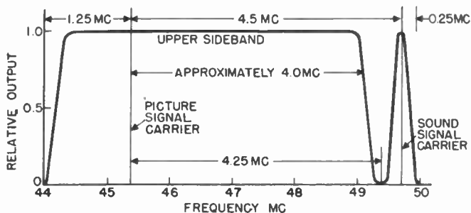
Figure 40. Single sideband television signal.
