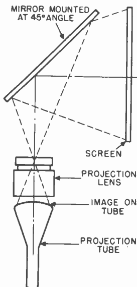
Figure 133. Refractive projection system.
