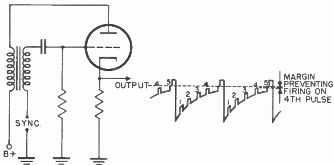
Figure 23. Blocking oscillator frequency divider.
