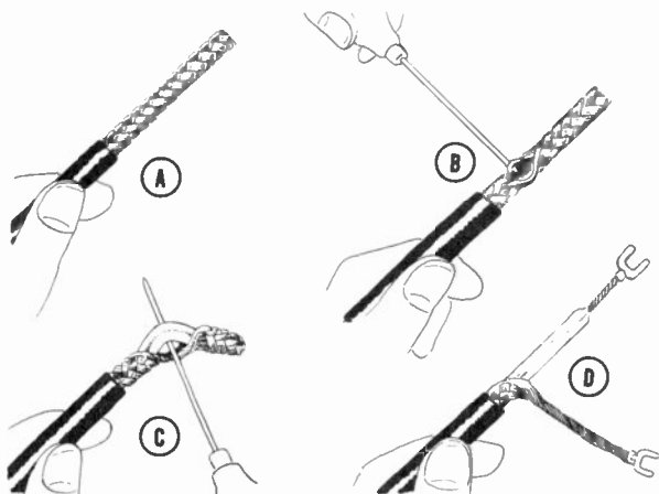
Figure 13. Finishing end of coaxial cable by making hole in braid. A, cut back rubber insulation. B, make hole in braid. C, pull center conductor through hole. D, strip insulation off center conductor and make hole at end of braid.
