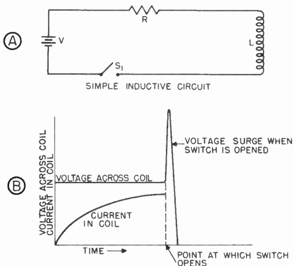
Figure 90. Operation of inductive differentiating circuit.
