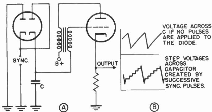
Figure 25. Pulse counting circuit.
