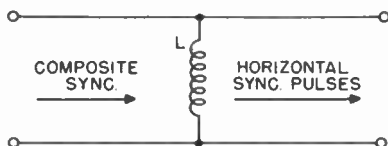
Figure 89. Inductive differentiating circuit.
