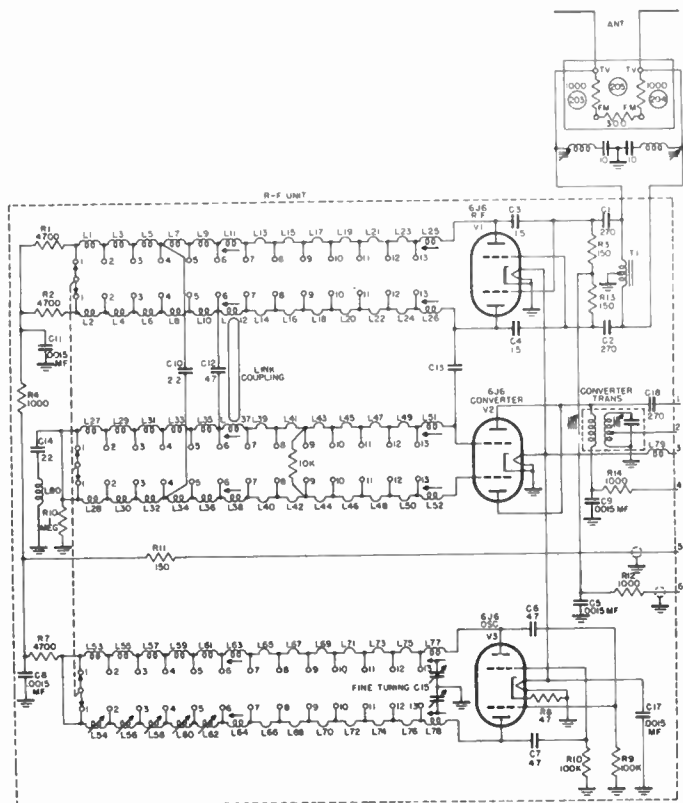
Figure 2. Schematic diagram of RCA tuner.
