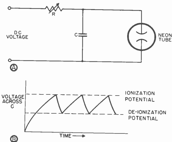
Figure 106. Simple electronic saw-tooth generator.
