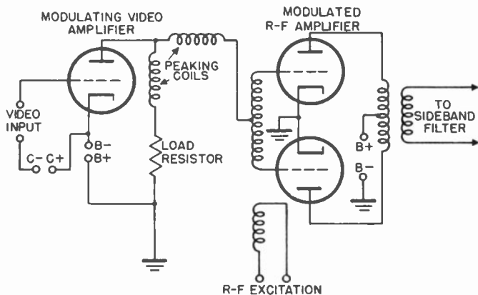
Figure 52. Modulated Class B amplifier.
