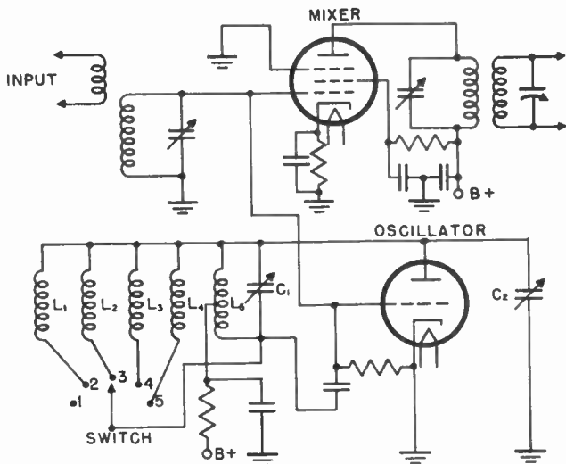
Figure 11. Hartley oscillator for covering widely separated frequencies.
