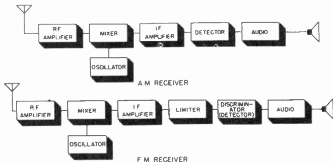
Figure 156. Block diagrams of conventional superhet and f-m receiver.
