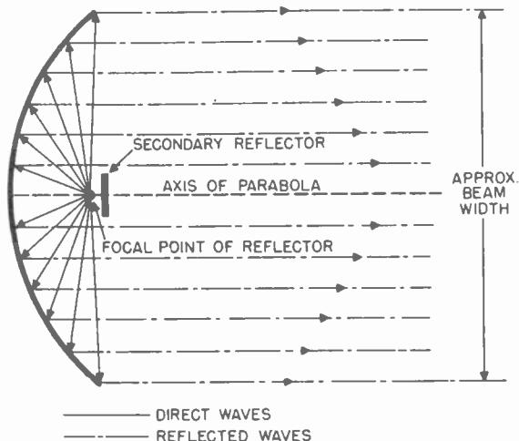
Figure 80. Reflecting action of parabolic surface.
