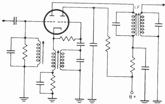
Figure 18. Mixer-oscillator using dual triode with common cathode.
