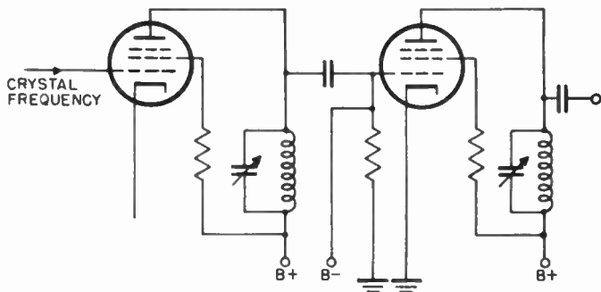
Figure 45. Simplified schematic of frequency multiplying stages.
