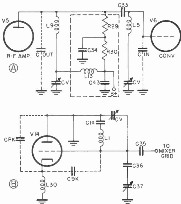
Figure 9. A. R-F amplifier circuit. B. Oscillator circuit.
