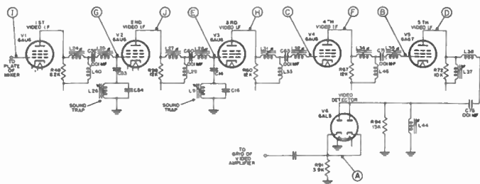
Figure 70. Simplified schematic of wide-band video i-f amplifier, showing points at which instruments are connected when alignment is performed.
