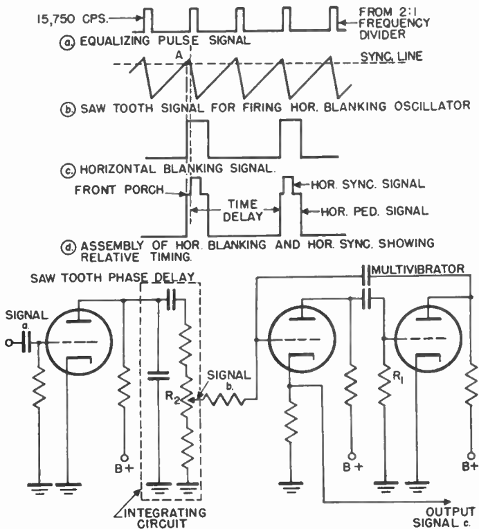
Figure 27. Generation of horizontal blanking pulses.
