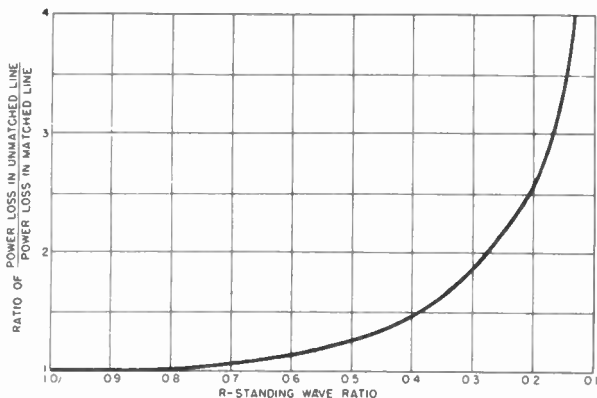
Figure 20. Ratio of power loss versus standing wave ratio.
