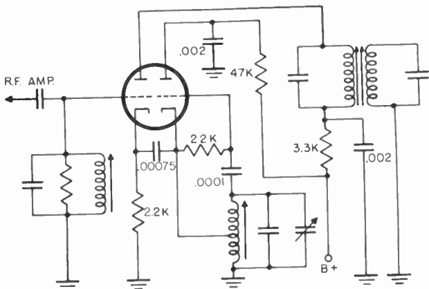
Figure 16. Mixer-oscillator using cathode injection.
