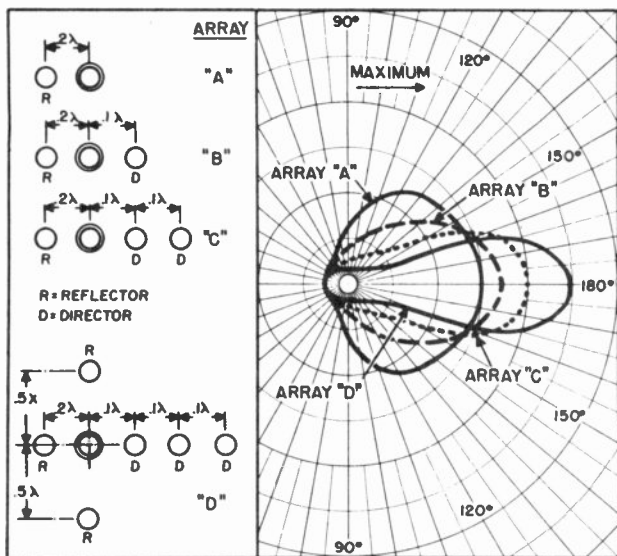
Figure 56. Field patterns of four parasitic arrays.
