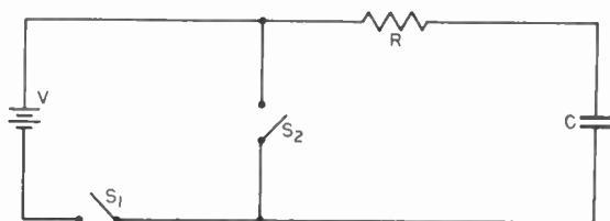
Figure 84. Integrating circuit.
