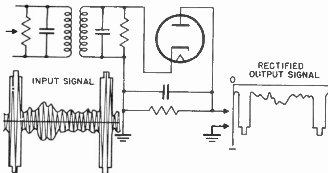
Figure 56. Diode detector and waveform.
