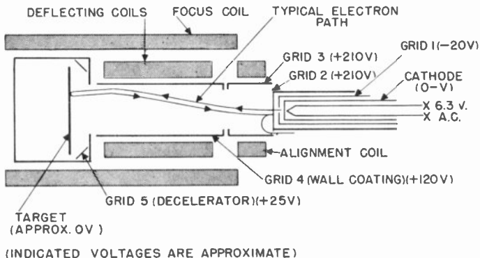
Figure 9. Scanning section of the image orthicon.
