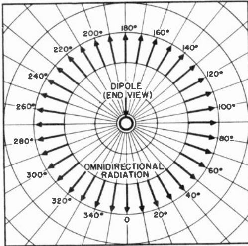
Figure 28. Vertical field pattern of horizontal dipole.
