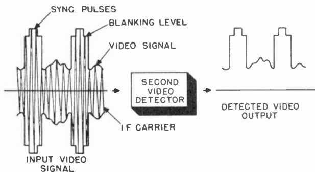
Figure 52. Input and output waveforms of the second detector.
