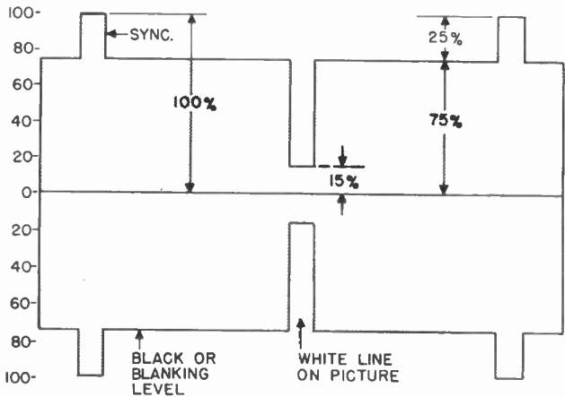
Figure 54. Modulation limits of transmitter.
