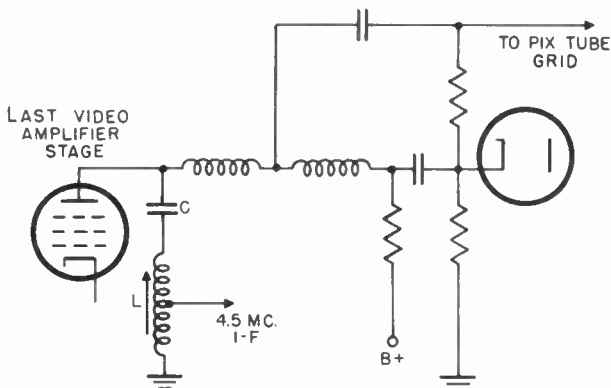
Figure 45. Circuit used to separate the sound carrier from the video signal in intercarrier receiver.
