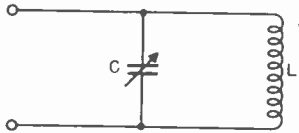
Figure 22. A parallel resonant circuit.
