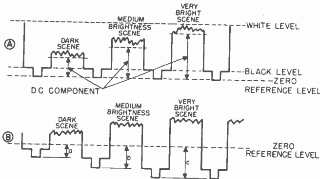
Figure 70. A, video signals of three different screen brightness levels. B, video signals with d-c component removed.
