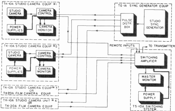
Figure 85. Block diagram of RCA studio camera equipment.
