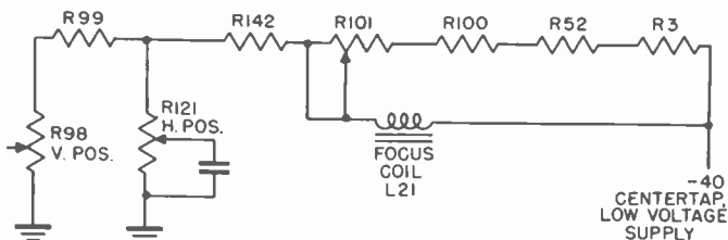
Figure 36. Focus coil circuit.
