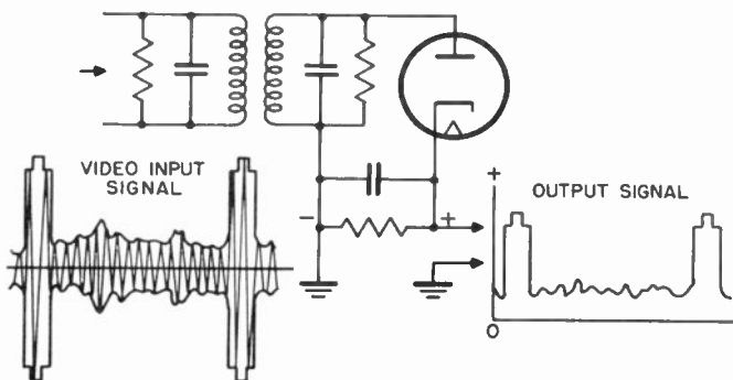
Figure 53. Diode detector and waveform.
