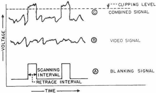
Figure 38. How blanking signal is combined with video signal.
