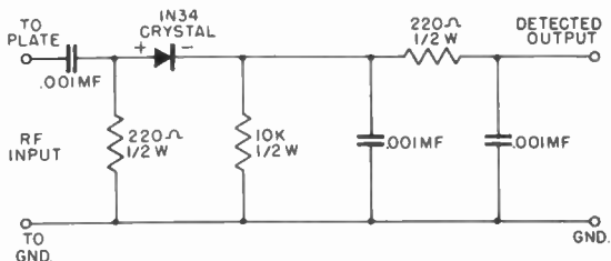
Figure 16. Probe detector.
