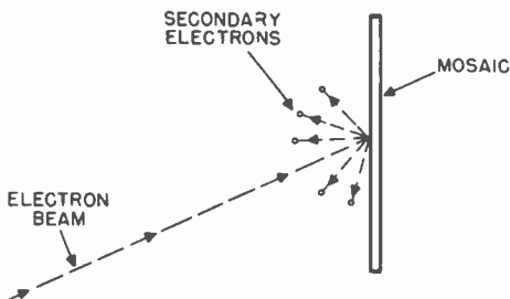
Figure 44. Secondary electrons emitted by a globule on the mosaic.
