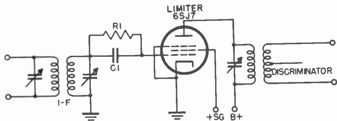
Figure 165. Simplified schematic of limiter circuit.
