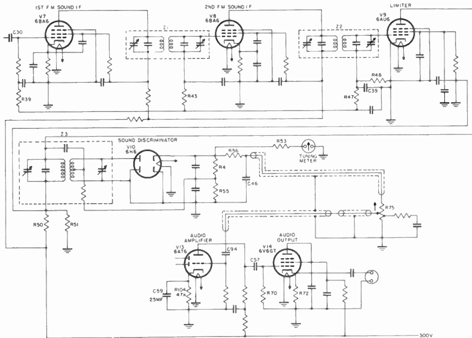
Figure 37. Sound channel.
