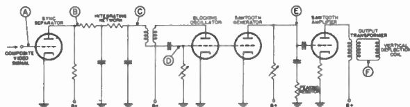
Figure 45. Simplified schematic showing points in vertical sweep circuits where waveform checks are made.
