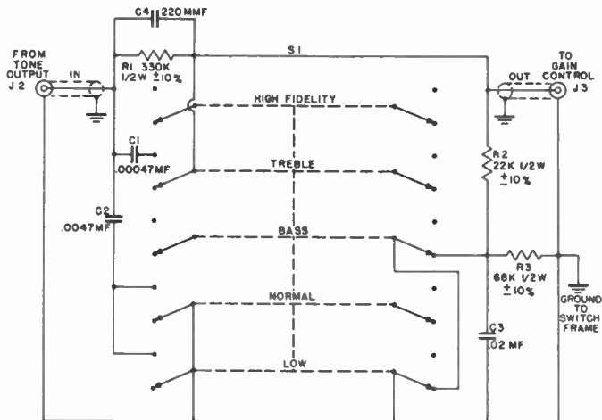
Figure 47. Tone selector schematic.
