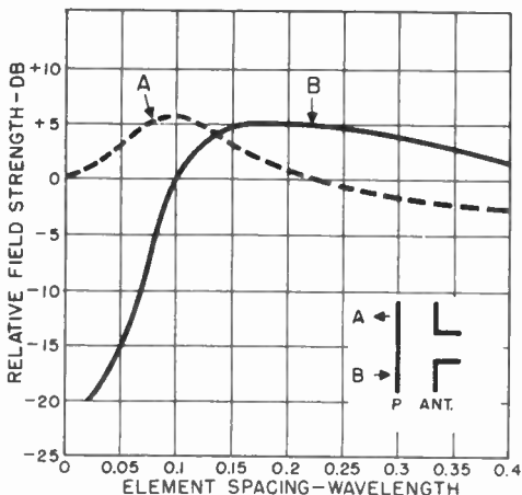
Figure 49. Maximum gain obtainable with single parasitic element. Curve A shows the gain when parasitic element, P, is director; curve B shows gain when P is reflector.
