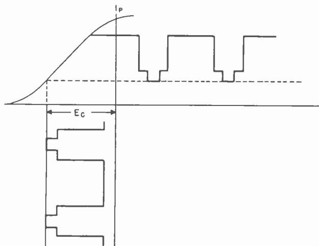
Figure 53. Grid characteristic of Class B modulated amplifier.
