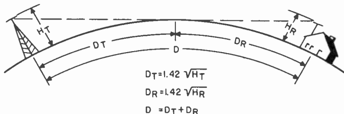
Figure 3. Radio horizon distance between transmitter and receiver.
