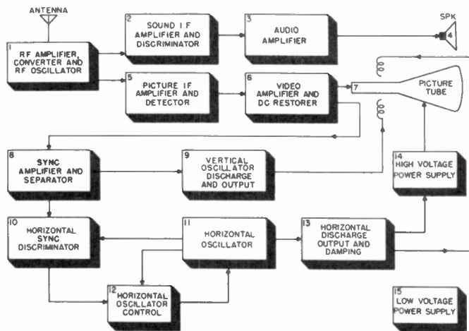
Figure 181. Block diagram of television receiver using ten-inch tube.
