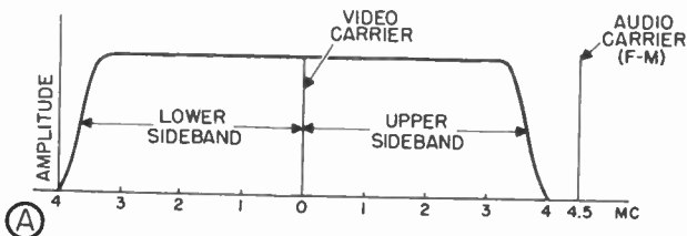
Figure 71A Band of frequencies which would be required for video signal if double side-band transmission were used.
