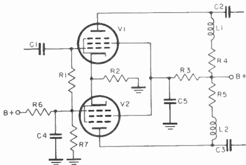
Figure 4. Cathode-coupled output stage.
