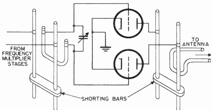
Figure 46. Transmission line tuned push-pull r-f amplifier stage.
