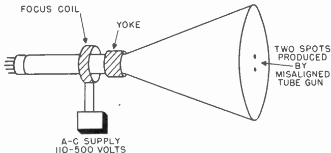
Figure 49. Method used to align focus coil using 60-cycle supply.
