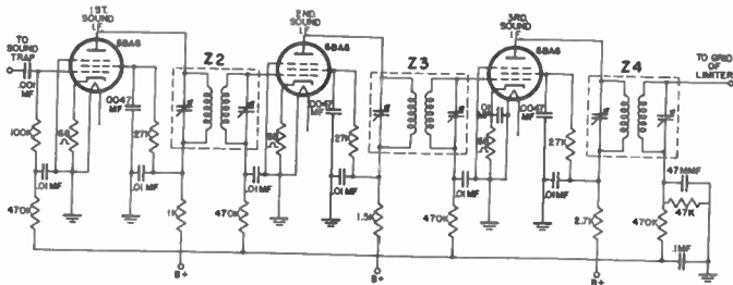
Figure 164. Three-stage sound i-f amplifier.
