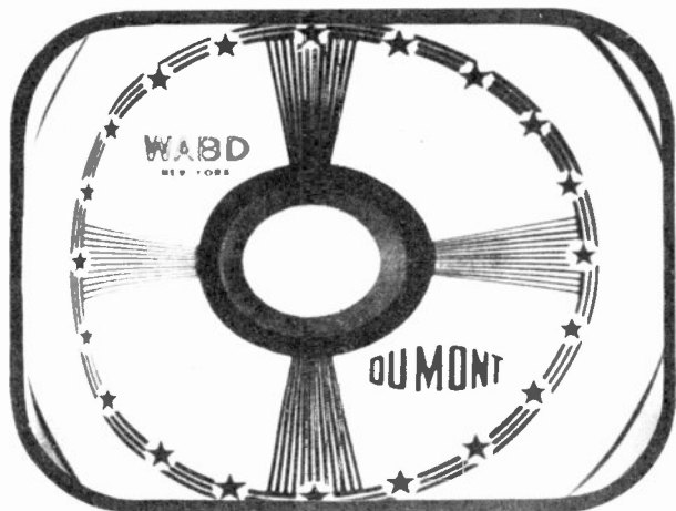
Figure 55. Horizontal distortion of test pattern caused by non-linear scanning.
