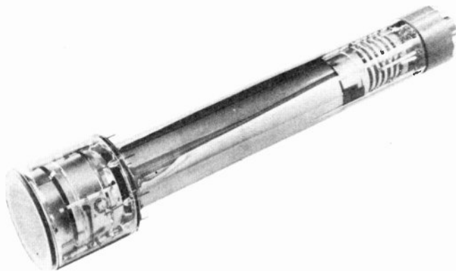
Figure 5. The image orthicon. (courtesy RCA)
