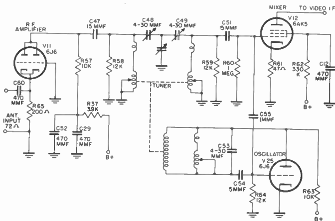
Figure 12. Schematic diagram of Inputuner.
