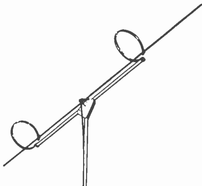
Figure 36. Duo-dipole antenna.
