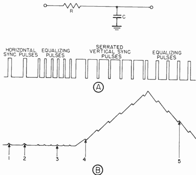
Figure 86. Input and output waveforms of integrating circuit.
