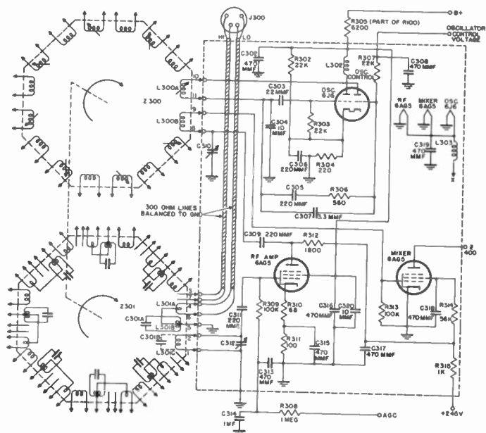
Figure 5. Schematic diagram of the Philco tuner.
