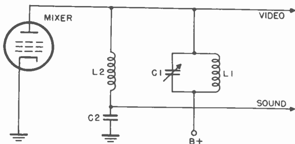
Figure 21. Series and parallel circuits for separating video and audio signals.
