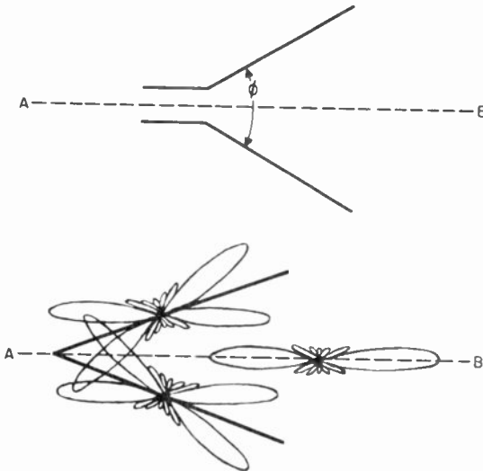
Figure 74. V antenna, and method whereby field patterns of two long-wire radiators are combined to produce highly directional V antenna field pattern.
