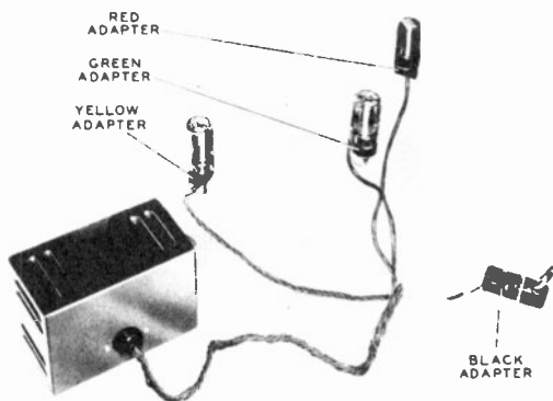
Figure 17. Philco Crosshatch Generator.
