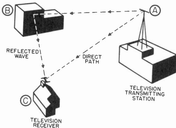
Figure 6. Direct wave and reflected wave striking antenna.
