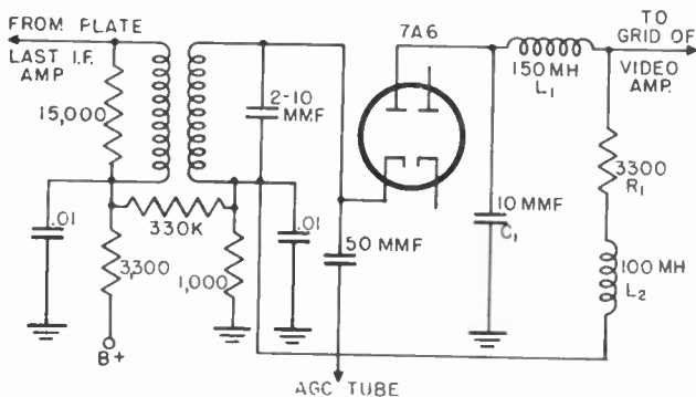
Figure 57. Schematic of video detector with bandpass filter.
