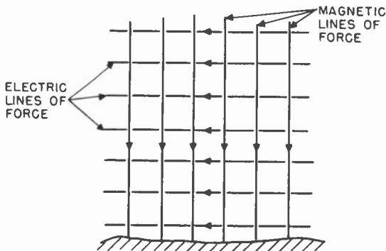
Figure 1. Representation of the magnetic and electric fields of horizontally polarized wave.
