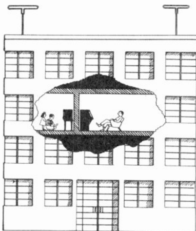
Figure 2. Cross-radiation is often caused by locating receivers back to back.
