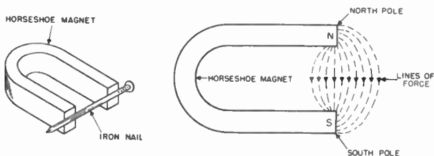
Figure 19. Left, the magnetic field between the poles of the horseshoe magnet pulls the nail to the magnet. Right, the lines of force around a horseshoe magnet.
