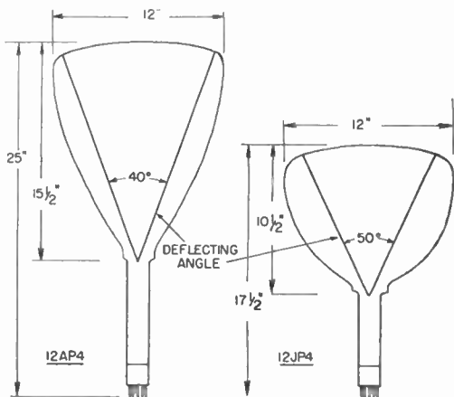
Figure 131. Relative shapes of old and new picture tubes.
