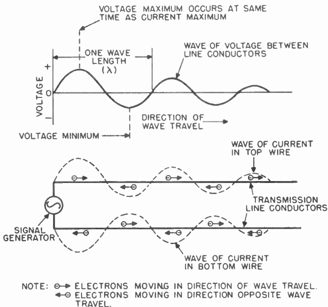
Figure 13. Voltage and current distribution along infinite line.
