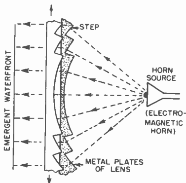
Figure 83. Focusing effect of metal plates of "stepped" construction.
