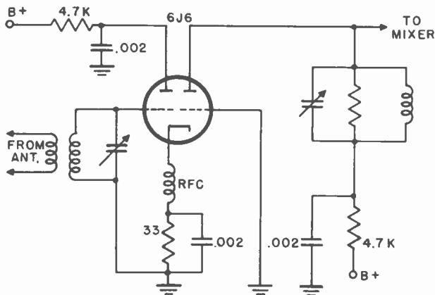
Figure 7. Cathode-coupled r-f amplifier.
