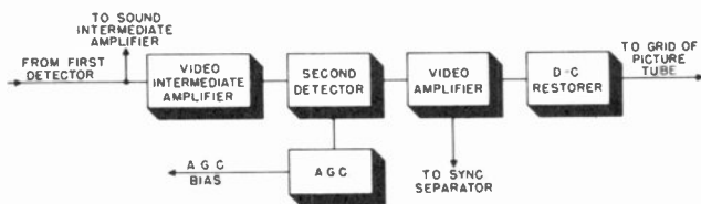
Figure 31. Block diagram of the video channel.
