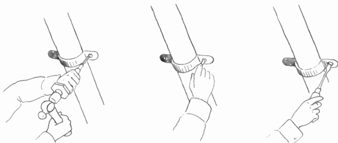
Figure 32. Drilling and mounting to masonry.
