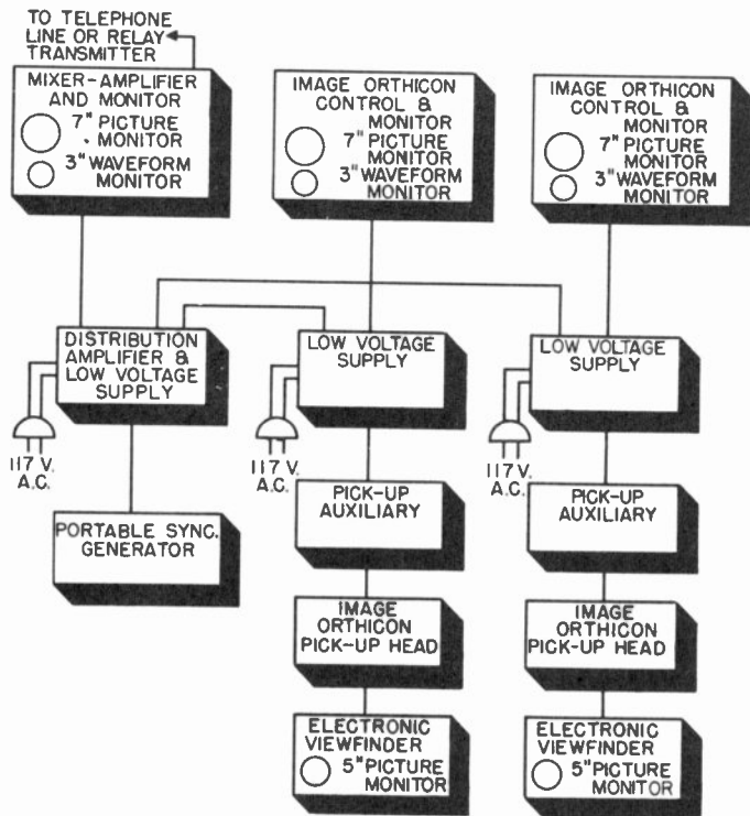
Figure 71. Block diagram of dual image-orthicon camera chain.
