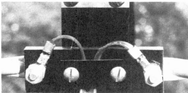
Figure 14. Method for connecting twin-lead to antenna. (courtesy Taco)
