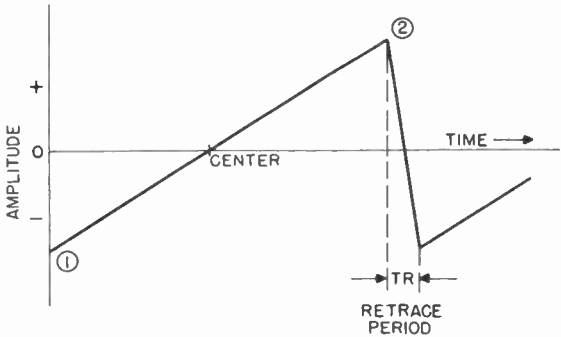
Figure 54. Sawtooth scanning voltage.
