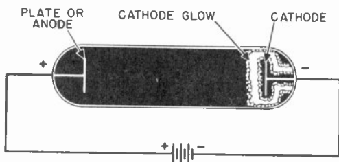
Figure 1. Plucker's simple gas tube.
