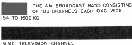
Figure 12. The space occupied in the frequency spectrum by all the a-m stations is less than that allotted to a single television station.
