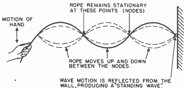
Figure 14. Standing waves produced in a rope.
