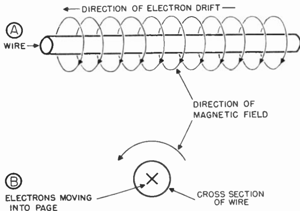
Figure 20. Direction of electron current flow in, and direction of magnetic field surrounding, a wire.
