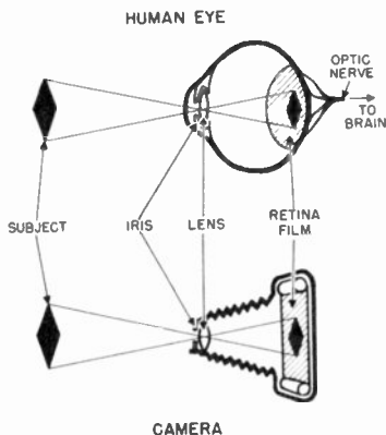
Figure 2. The action of the human eye is similar to that of a camera.
