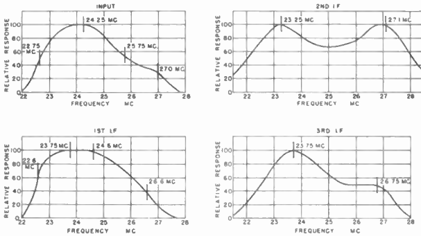
Figure 39. Response curves of the transformers of a broadband amplifier chain.
