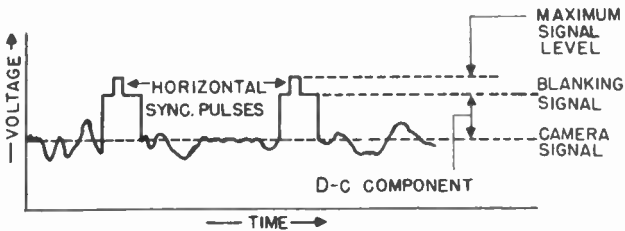
Figure 39. The completed composite video signal.
