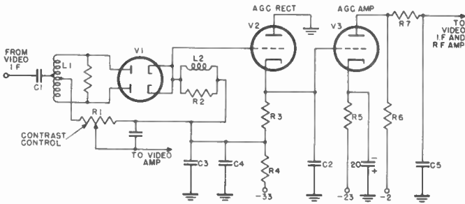
Figure 76. Delayed a.g.c. circuit.
