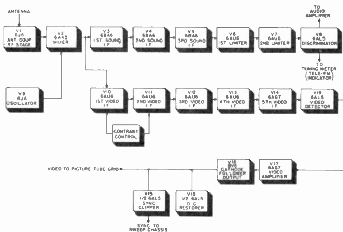
Figure 43. Block diagram of r-f, i-f chassis.
