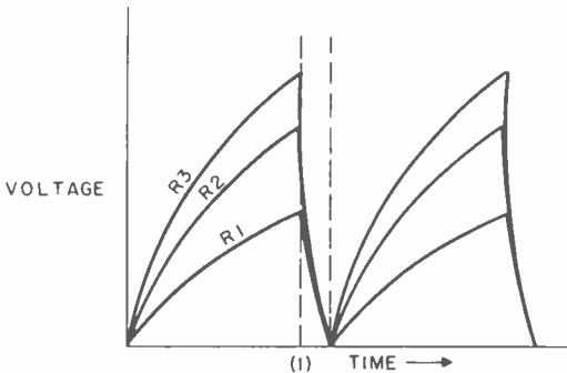
Figure 105. Effect on charging curve of different values of R in Figure 104.
