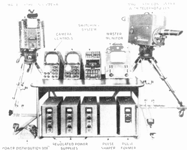
Figure 102. Field pickup camera chain. (courtesy RCA)
