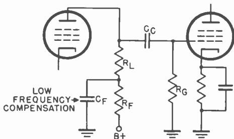
Figure 67. Parallel resistor-capacitor combination for low frequency compensation.
