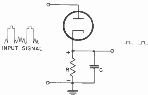
Figure 81. Self-biased diode sync clipper.
