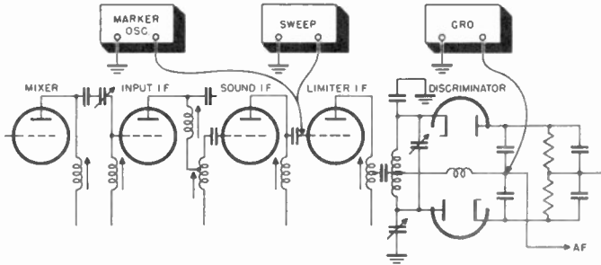
Figure 59. Connections used when aligning discriminator using oscillograph and sweep generator.
