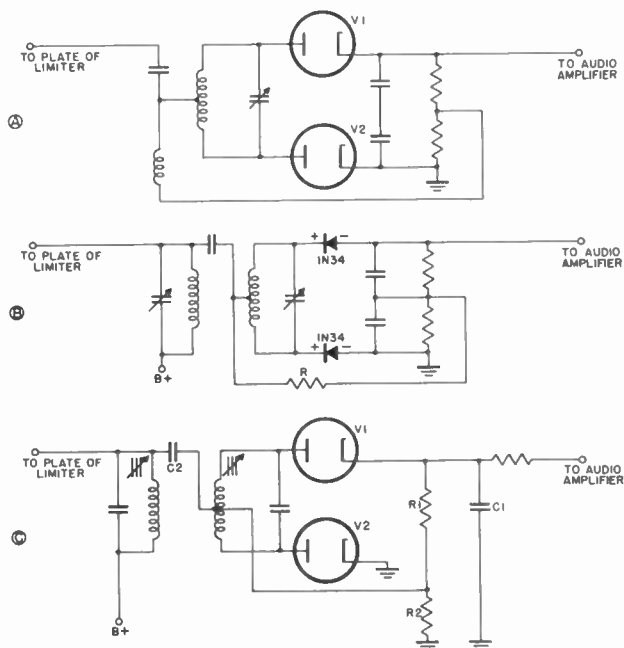
Figure 174. Modifications of the Foster-Seeley discriminator.
