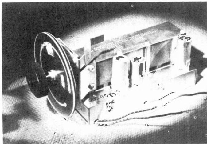
Figure 13. Complete Inputuner assembly for continuous 44-216 Mc coverage, showing manual drive dial. (courtesy DuMont)
