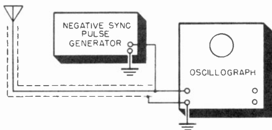
Figure 130. Method used to check antenna impedance match.
