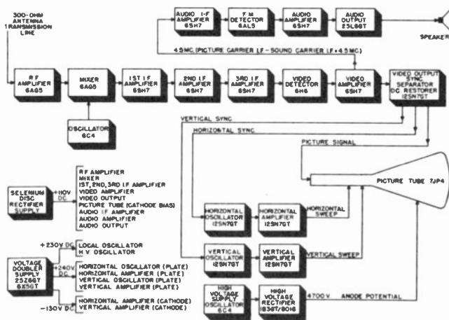
Figure 14. Block diagram of Hallicrafters Model T-54.
