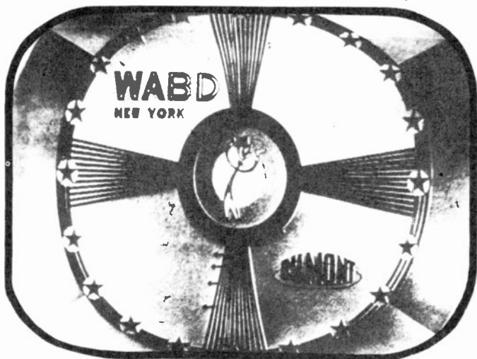
Figure 6. Contrast control set too high.
