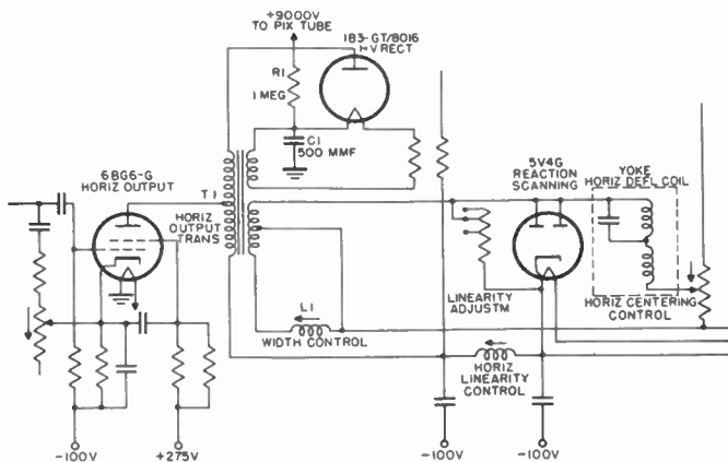
Figure 154. Typical kickback high-voltage supply used in a television receiver.
