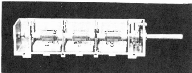
Figure 10. The Inductuner. (courtesy DuMont)
