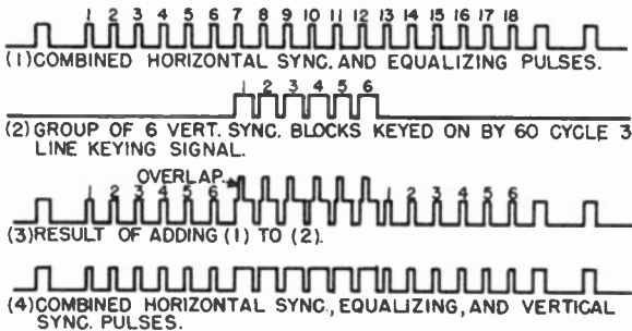
Figure 33. Circuit used to mix serrated vertical sync pulses with combined horizontal and equalizing pulses.
