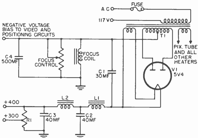
Figure 143. Typical low-voltage power supply.
