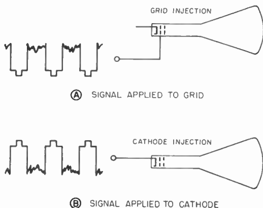
Figure 55. Polarity of signal required at grid and cathode of picture tube.
