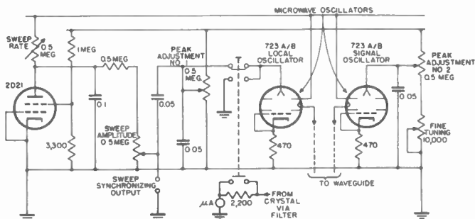
Figure 15. Basic schematic circuit of Mega-Sweep.
