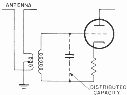
Figure 28. Antenna coupling circuit using untuned primary and tuned secondary.
