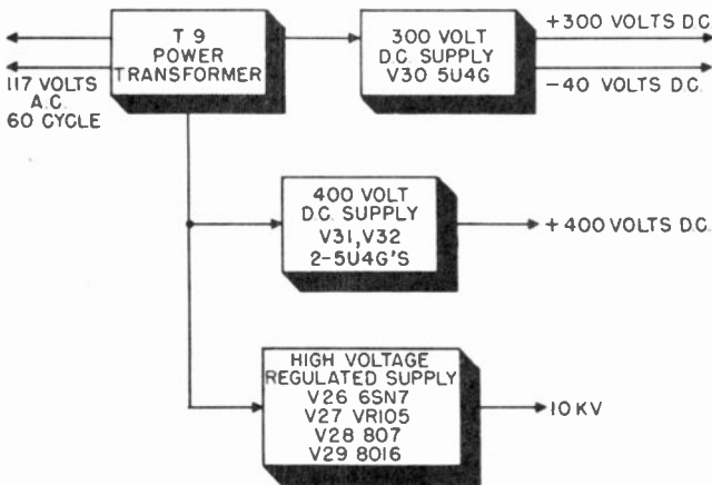
Figure 38. Block diagram of power supply chassis.
