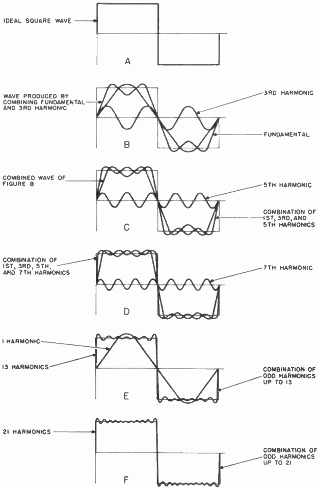
Figure 66. Creation of a square wave.
