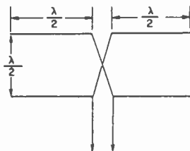
Figure 66. Lazy-H antenna.
