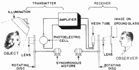
Figure 11. Transmitter and receiver apparatus for a mechanical television system.
