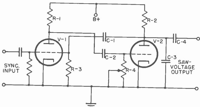
Figure 108. Multivibrator and discharge circuit.
