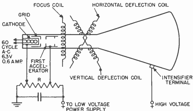
Figure 124. Points at which voltages are applied to electromagnetic picture tube.
