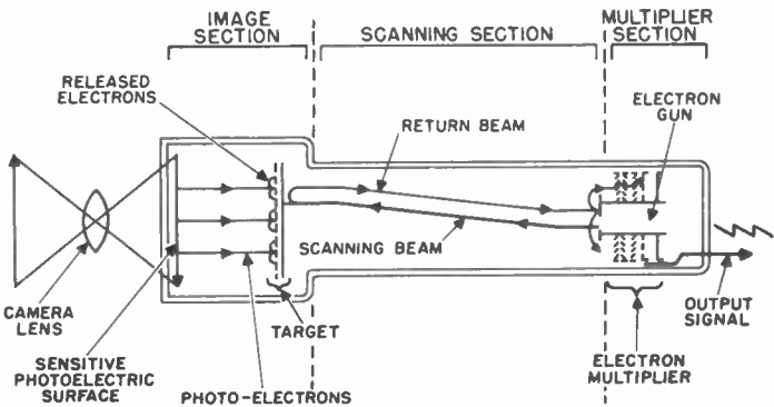
Figure 7. Construction of the image orthicon.
