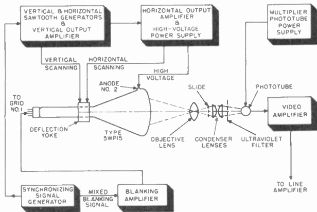
Figure 101. Block diagram of flying spot signal generator.
