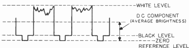
Figure 69. Composite video signal at the output of the video detector.
