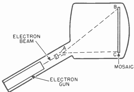
Figure 46. Keystoning occurs in the iconoscope because the electron beam travels unequal paths from the gun to the mosaic.
