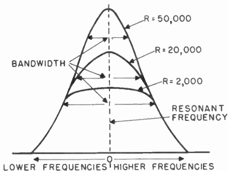
Figure 27. The effect of various values of load resistance on bandwidth of coupling transformers.
