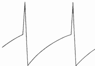
Figure 150. Pulses generated by blocking oscillator.
