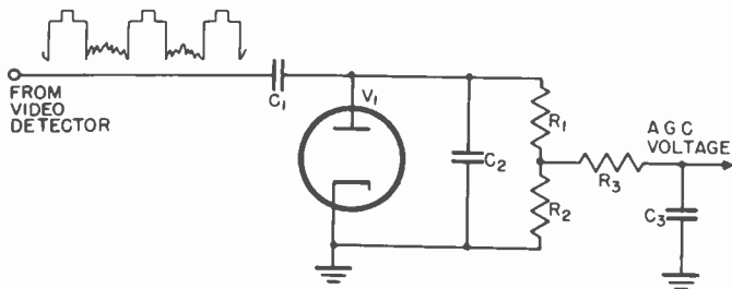
Figure 75. Simplified diagram of a.g.c. circuit.
