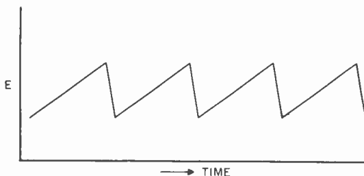
Figure 103. Waveform of current in deflection coils.
