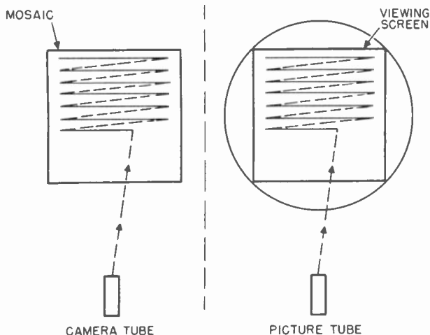
Figure 50. The electron beam scans the mosaic in exact synchronism with the electron beam in the picture tube.
