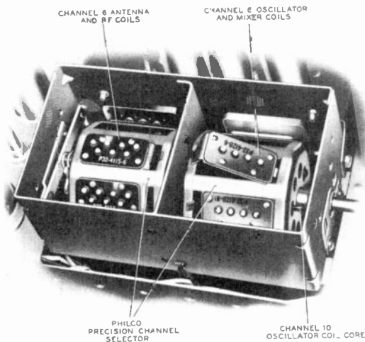
Figure 6. Octagonal turrets used in Philco tuner showing "snap-in" coils. (courtesy Philco)
