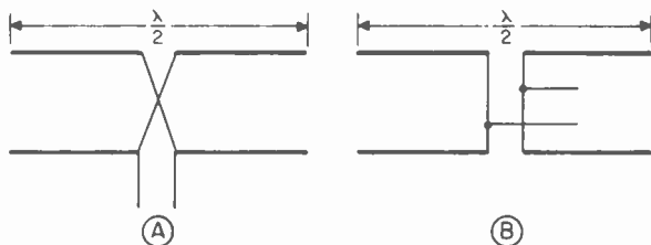
Figure 59. Stacked dipole arrays. (A) center fed; (B) transposed feeder.
