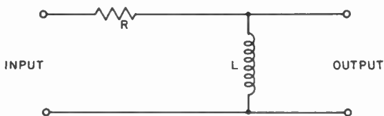
Figure 177. Pre-emphasis filter.
