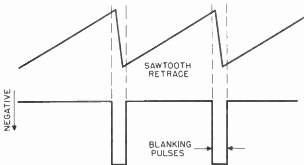
Figure 59. Waveshape and polarity of blanking pulses.
