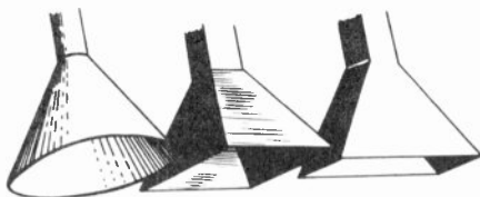
Figure 81. Electromagnetic horn: left, conical type; center, pyramidal type; right, rectangular type.
