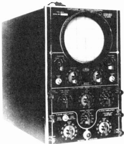
Figure 7. The Du Mont Type 208B Cathode-Ray Oscilloscope.
