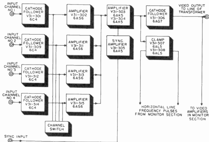
Figure 77. Block diagram of mixer amplifier.
