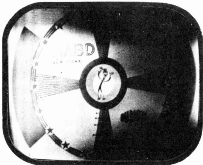
Figure 45. Uneven illumination of the test pattern caused by spurious secondary electrons in the iconoscope.
