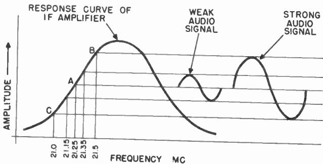
Figure 169. Operation of slope detector.
