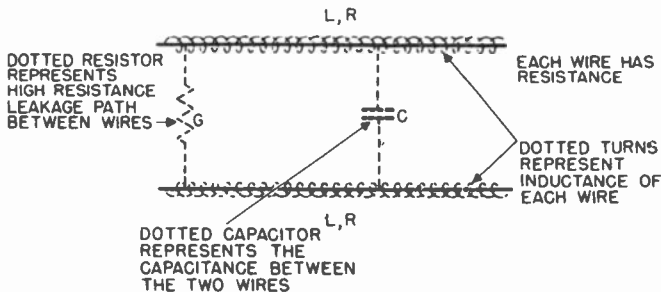
Figure 12. Distribution of resistance, capacitance, and inductance along section of two-wire transmission line.
