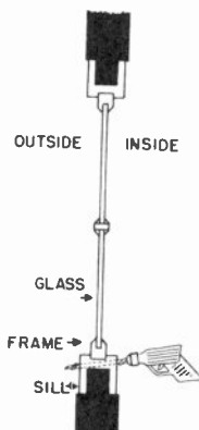
Figure 16. Drilling window sill at an angle to make hole for lead-in
