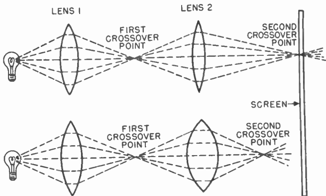
Figure 17. The distance to the second crossover point is determined by the curvature of lens 2.
