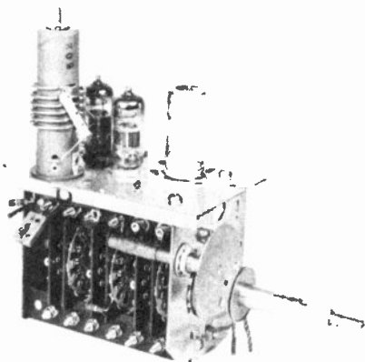
Figure 1. The RCA tuner. (courtesy RCA)
