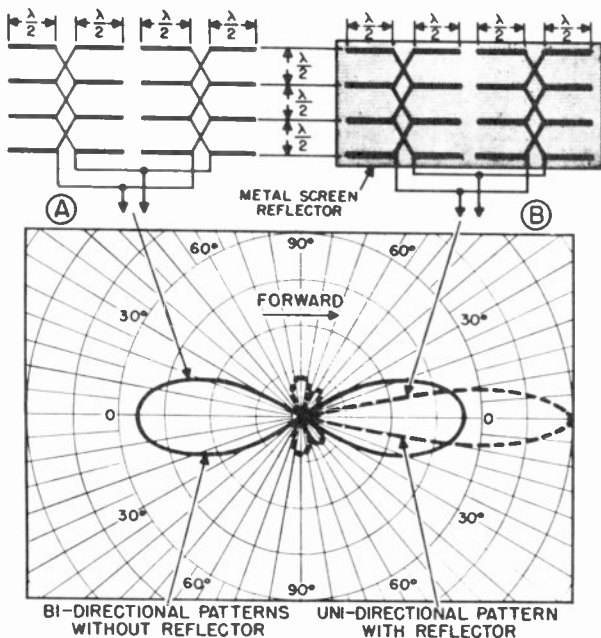
Figure 68. Field patterns of multi-element antenna array. (A) Bi-directional pattern without reflector; (B) Uni-directional pattern with metal screen reflector.
