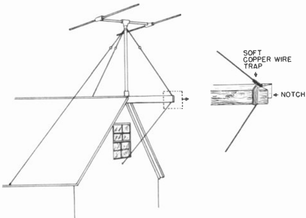
Figure 28. Outrigger used to obtain proper guy spacing.
