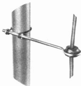
Figure 15. Mast eyelet for holding twin lead. (courtesy JFD)
