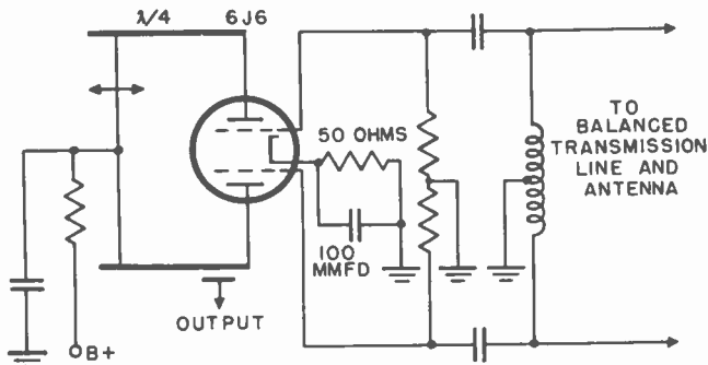
Figure 8. Push-pull r-f amplifier.
