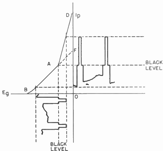
Figure 69. Grid-voltage, plate-current curves of non-linear amplifier stage.
