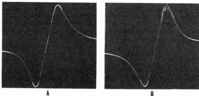
Figure 60. Signal on oscillograph produced by discriminator output. A. Marker signal at center frequency, B. Marker signal at signal peak.
