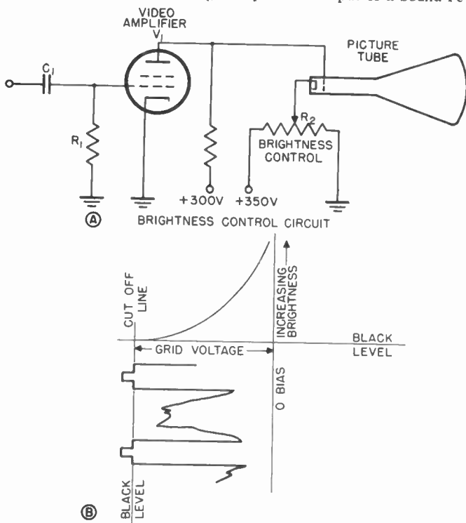
Figure 73. A, circuit for providing adjustment of picture tube bias. B, effect on picture brightness of variations in grid voltage.
