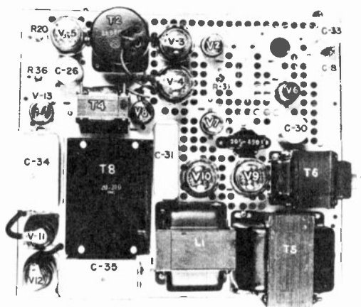
Figure 50. Sweep chassis. (courtesy DuMont)
