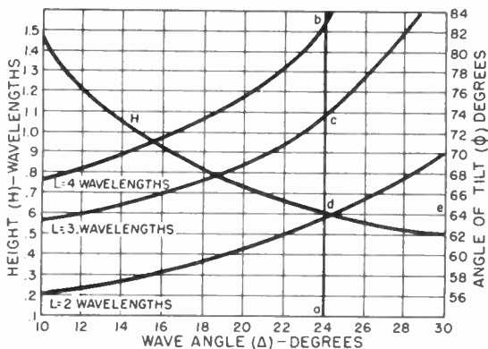
Figure 77. Design chart for rhombic antenna.
