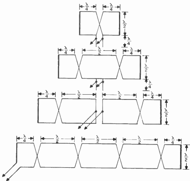
Figure 67. Four types of horizontal sterba arrays.
