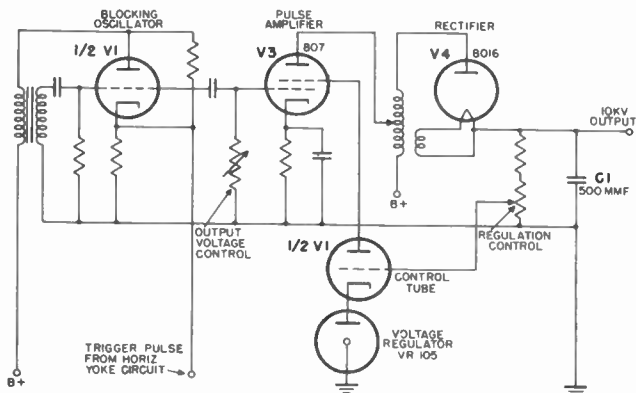
Figure 152. Regulated pulse type supply.
