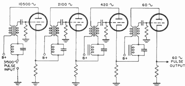
Figure 26. Frequency divider chain.
