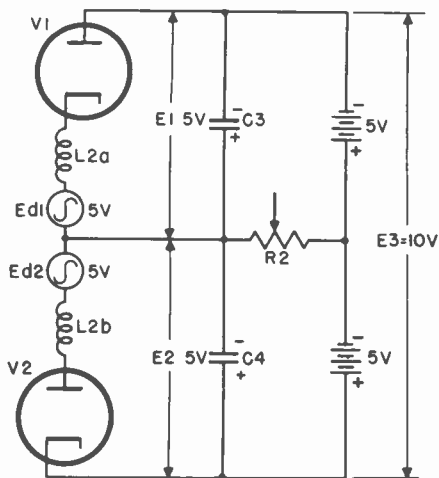
Figure 176. Equivalent circuit of ratio detector.
