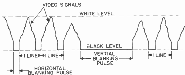
Figure 60. A composite video and blanking signal.
