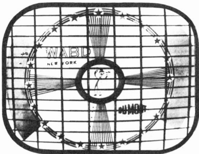
Figure 114. Linearity bars for adjustment of monitor sweep linearity. (courtesy DuMont)
