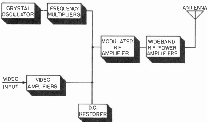
Figure 43. Block diagram of low level modulated transmitter.
