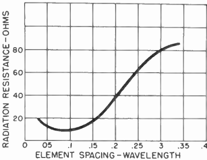
Figure 54. Variation of radiation resistance of dipole and reflector.
