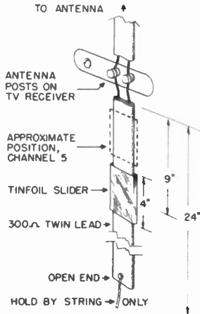
Figure 39. Simple wave trap.
