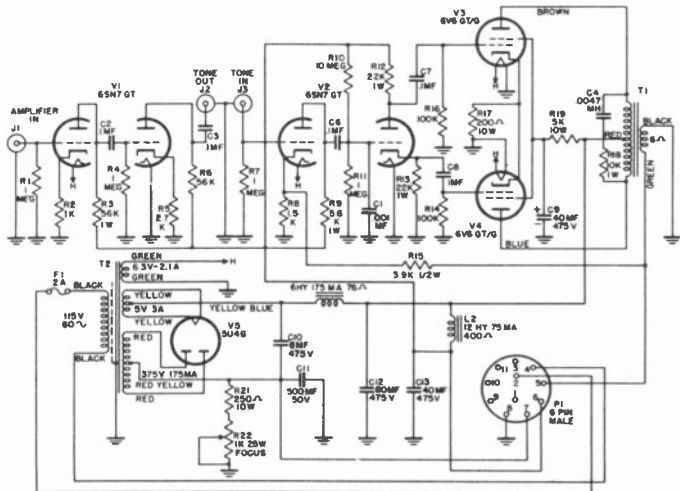
Figure 46. Audio amplifier schematic.
