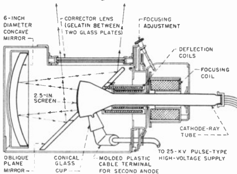
Figure 140. The North American Phillips version of the Schmidt projection system.
