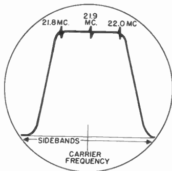
Figure 163. Response curve of a broadband i-f amplifier.
