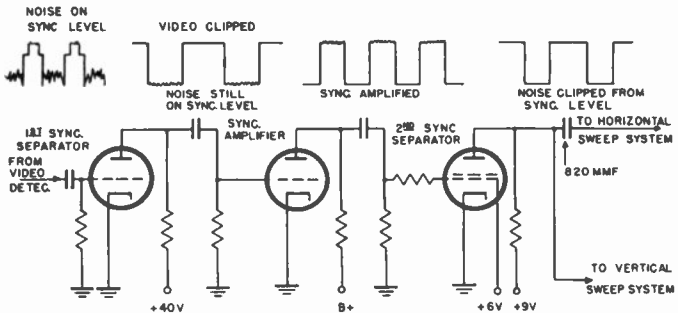
Figure 83. Cascade sync clipper.
