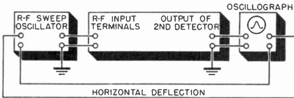
Figure 76. Connections used when aligning r-f section.
