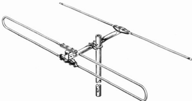
Figure 55. Folded dipole with reflector. (courtesy JFD)
