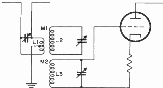
Figure 30. Double tuned antenna coupling circuit with tuned link added.
