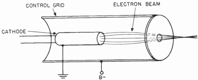
Figure 13. The grid limits the number of electrons which pass to screen.
