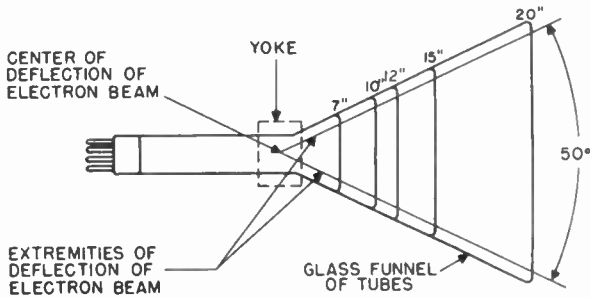
Figure 132. Relative sizes of magnetic picture tubes.
