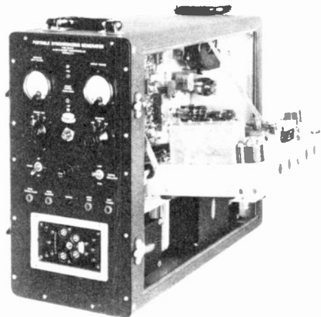
Figure 80 Portable sync generator. (courtesy DuMont)
