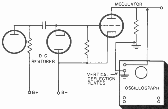
Figure 129. Method used to measure d-c restoration in transmitter.
