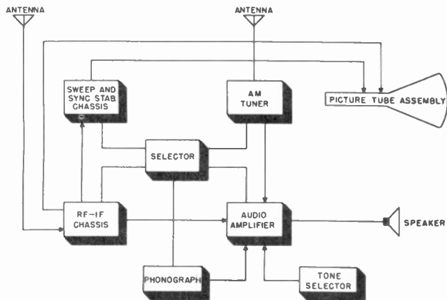
Figure 42. Block diagram of DuMont Model RA-101
