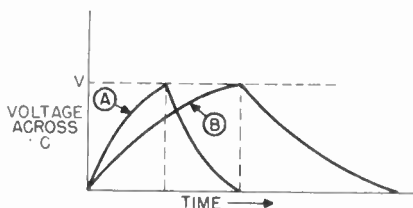
Figure 85. Operation of integrating circuit.
