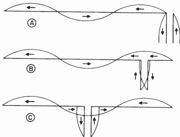
Figure 72. Long-wire antenna, showing current distribution and feed points.
