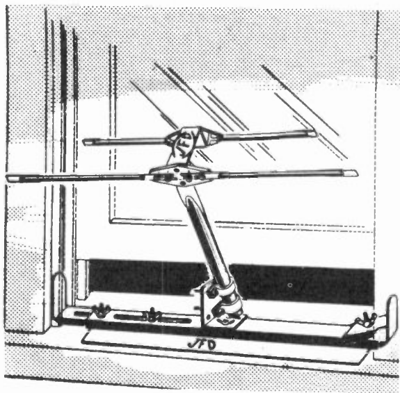
Figure 23. Window sill mounting bracket. (courtesy JFD)
