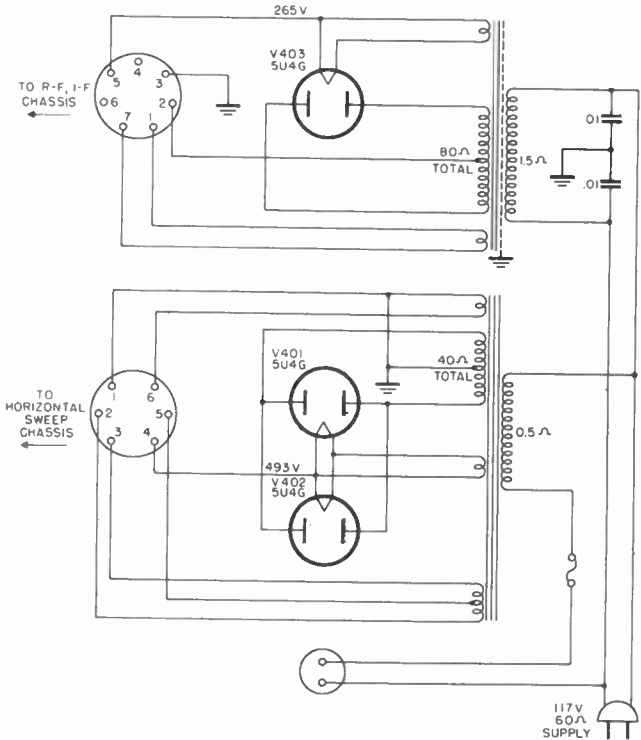
Figure 57. Low voltage power supply.
