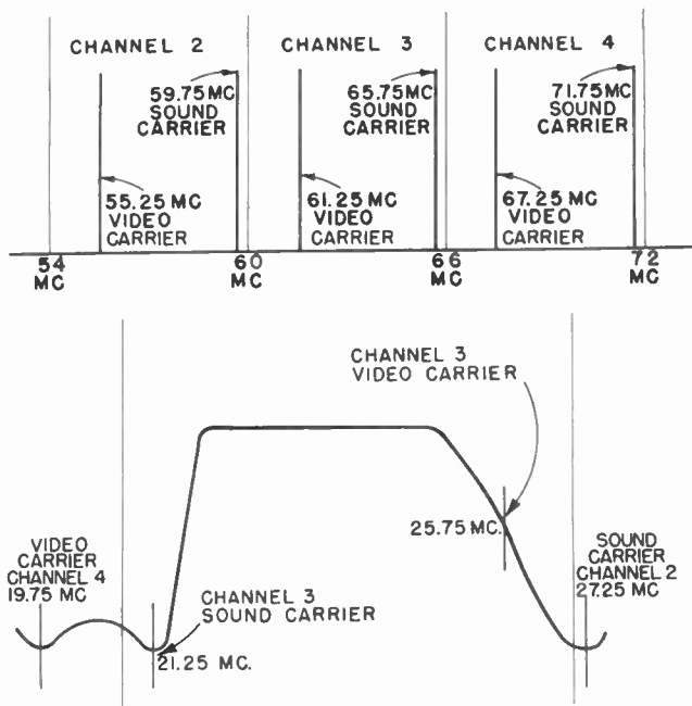
Figure 36. Video and sound r-f frequencies, and video and sound i-f frequencies.
