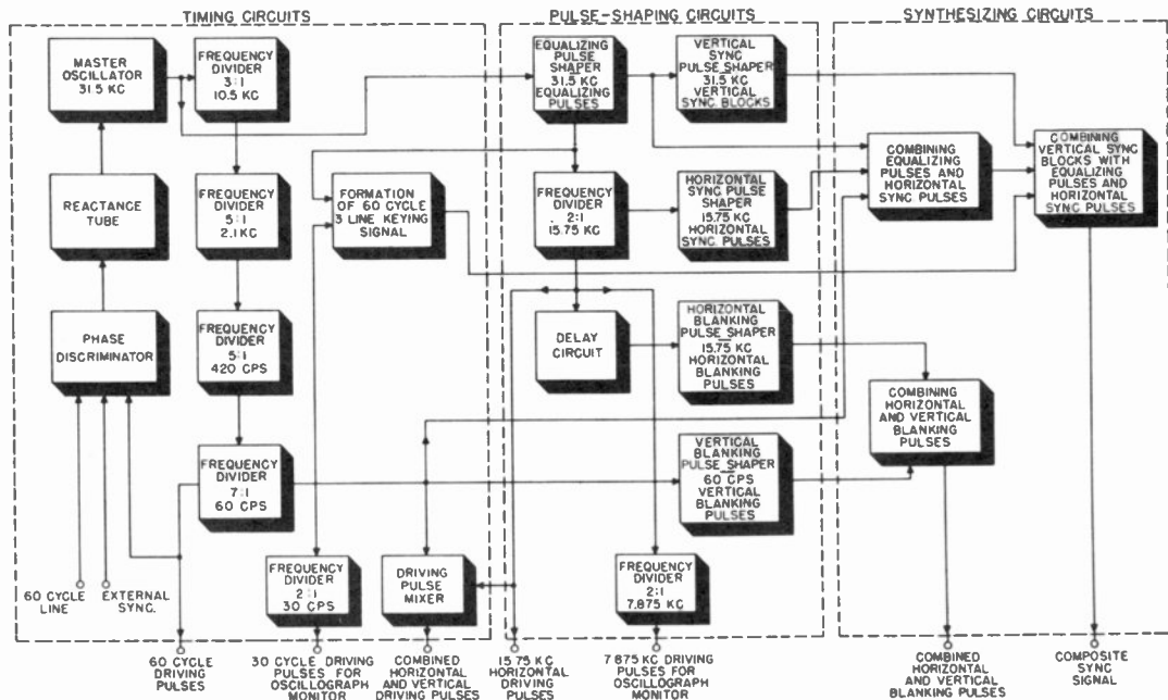
Figure 20. Block diagram of sync generator unit.
