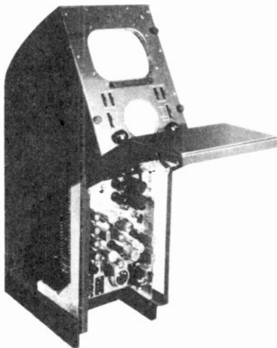
Figure 90. Studio picture monitor. (courtesy RCA)
