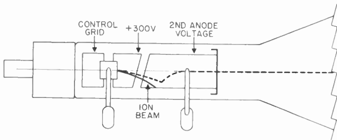
Figure 128A. Ion trap.
