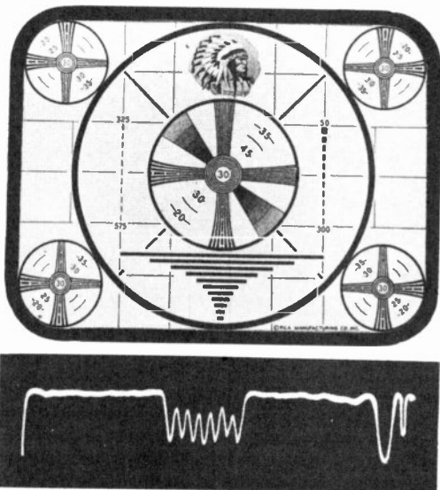
Figure 126. Oscillogram and test pattern used to measure resolution.
