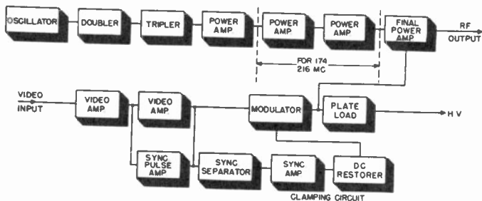
Figure 108. Block diagram of TT-5A transmitter.
