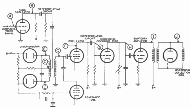
Figure 48. Simplified schematic of horizontal sweep circuit employing fly-wheel synchronization. Waveforms of Figure 47 appear at points indicated.
