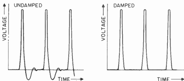
Figure 120. Spurious oscillations which appear across horizontal deflection coil during flyback time.
