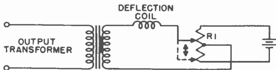
Figure 123. Positioning circuit for electromagnetic picture tube.
