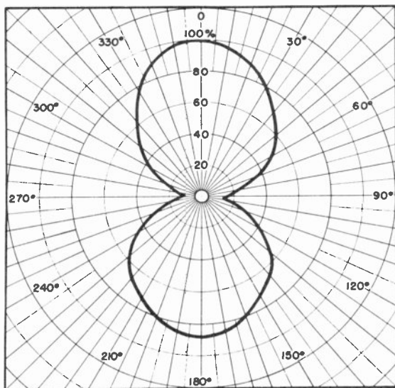
Figure 37. Horizontal field pattern of duo-dipole antenna at 70 Mc.
