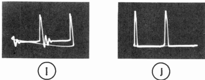
Figure 47. Waveforms in horizontal sweep circuit using flywheel synchronization. Points at which waveforms appear are indicated in Figure 48.
