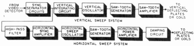
Figure 78. Block diagram of vertical and horizontal sweep circuits.
