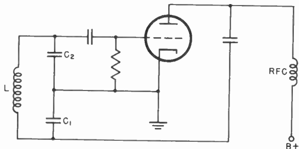
Figure 12. Colpitts oscillator.
