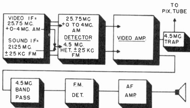
Figure 44. Operation of the intercarrier sound system.
