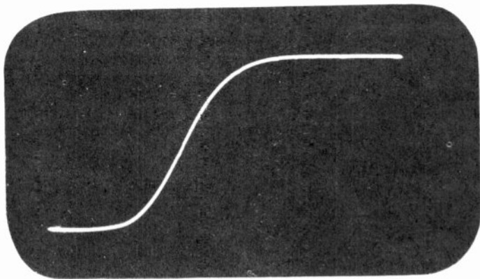
Figure 124. Leading edge of horizontal pulse.
