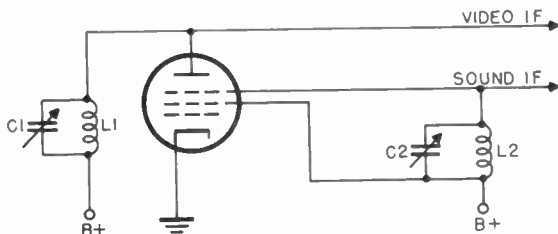
Figure 20. Plate and suppressor-screen tuned circuits for separating video and audio signals.
