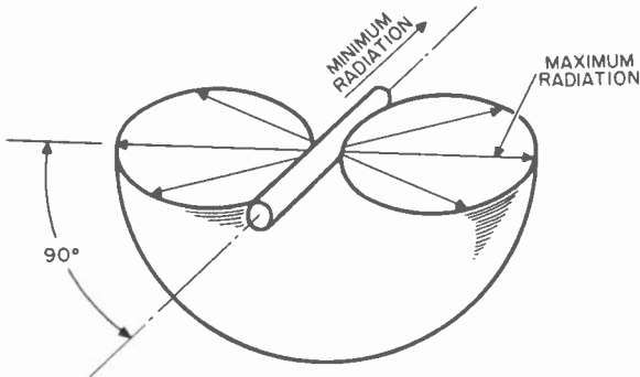
Figure 26 Radiation pattern of half-wave dipole in free space.
