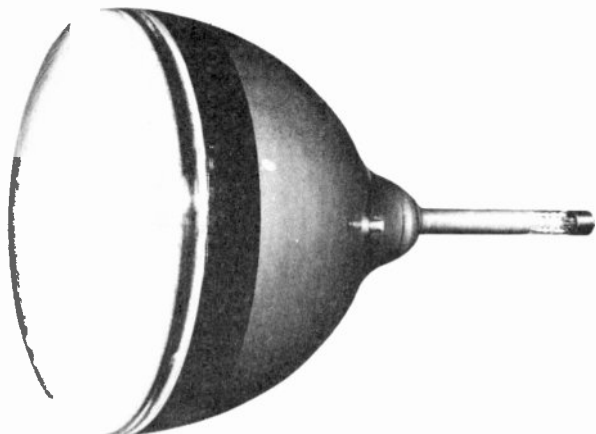
Figure 11. The glass envelope is coated on the inside with a conducting material. The second anode cap is connected to the aquadag coating. (courtesy DuMont)
