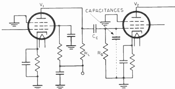
Figure 61. Simplified schematic of resistance coupled amplifier.
