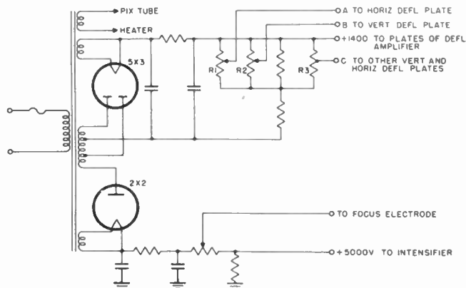
Figure 122. Power supply and positioning controls for electrostatic cathode-ray tube.
