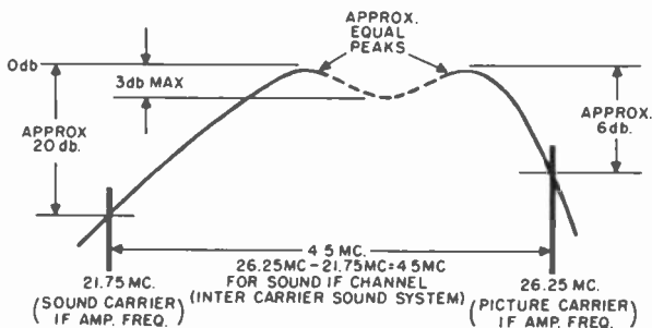
Figure 16. Response curve of intermediate frequency amplifiers which pass both the video and audio signals.
