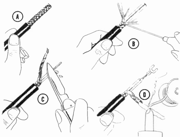
Figure 11. Step-by-step method of preparing coaxial cable by unbraiding and tinning braid. A, cut back rubber insulation. B, score braid. C, twist scored braid and cut back insulation to expose center conductor. D, tin braid and add lug.
