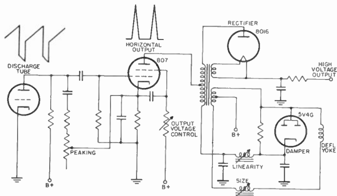
Figure 153. Simplified schematic of kickback high-voltage supply.
