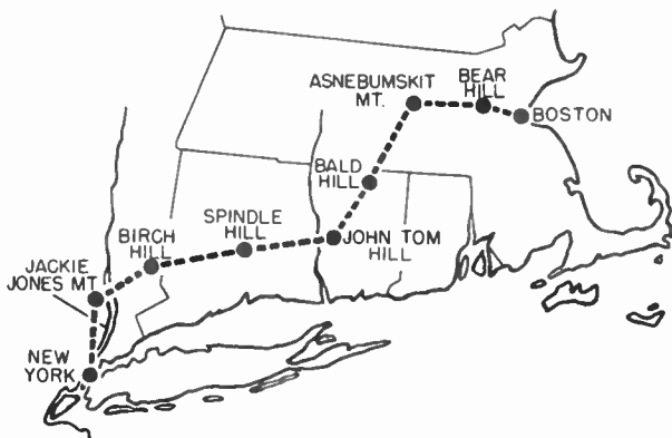
Figure 81. Microwave relay link between New York and Boston.
