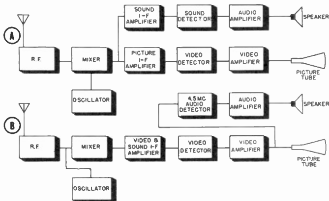
Figure 43. Block diagrams of receivers using conventional and intercarrier sound systems.
