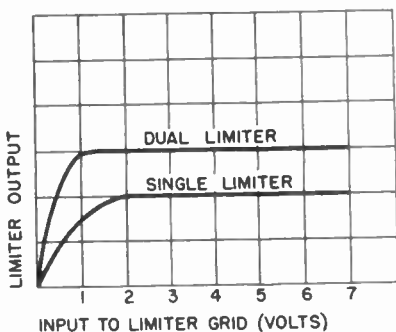
Figure 168. Comparison of single and dual limiter.
