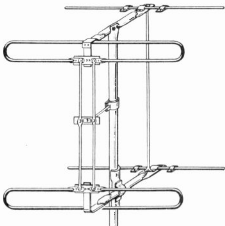
Figure 61. Stacked folded dipoles and reflectors. (courtesy Taco)
