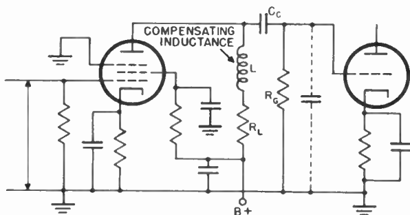
Figure 63. Shunt-peaking frequency compensation.
