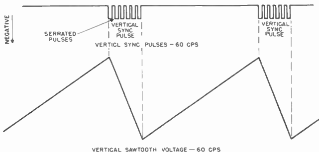
Figure 62. The vertical sync pulse consists of six serrated pulses.
