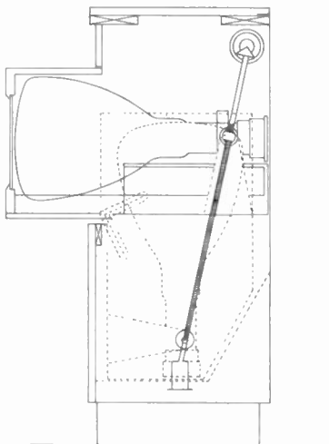
Figure 127. Mechanical lift mechanism used with large picture tubes.
