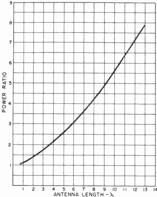
Figure 71. Power gain of long-wire antenna over half-wave antenna.
