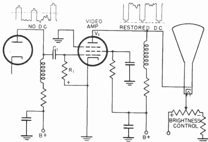
Figure 72. D-C restoration in the video amplifier stage.
