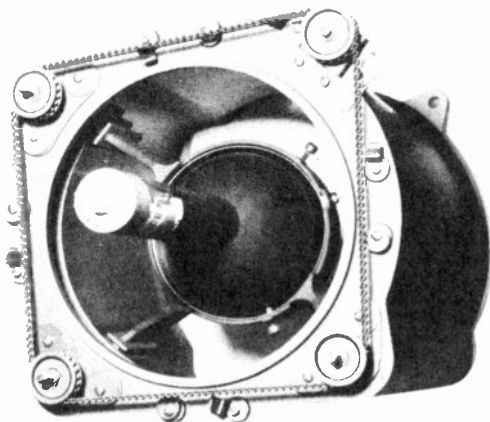
Figure 137. The tube and barrel of the RCA projection system.
