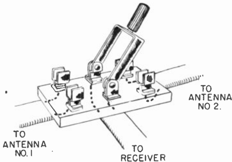
Figure 47. Double-pole, double-throw knife switch for connecting two antennas to receiver.
