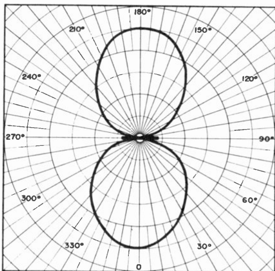
Figure 40. Field pattern of bat-wing antenna at 80 Mc.
