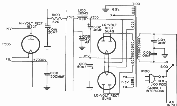
Figure 27. Power supplies.
