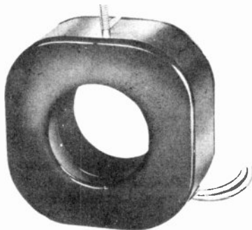
Figure 26. A commercial focus coil. (courtesy RCA)
