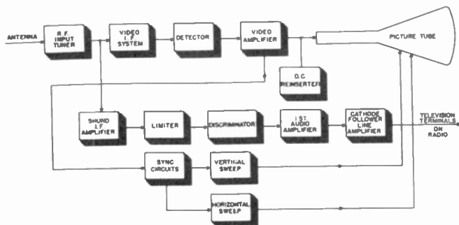
Figure 32. Block diagram of main chassis.
