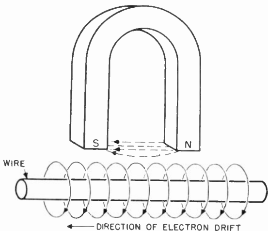
Figure 21. A wire which is parallel to the magnetic lines of force set up by a horseshoe magnet is not influenced by the magnet.
