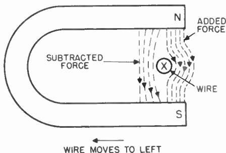
Figure 22. Wire placed at right angles to the lines of force from the horseshoe magnet.
