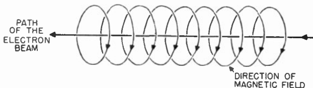
Figure 23. Direction of magnetic field set up by an electron beam.
