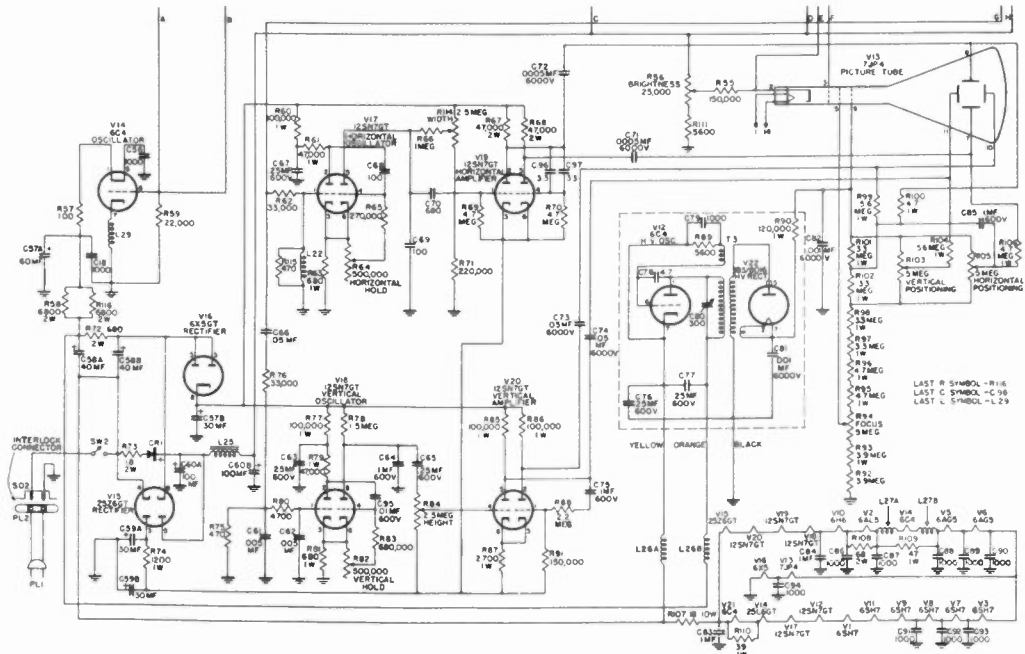
Figure 15. Schematic diagram of Hallicrafters Model T-54
