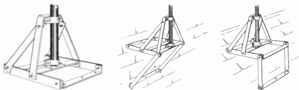
Figure 25. Bracket which can be used in several ways but is particularly suited for sloping roof. (courtesy Workshop Associates)
