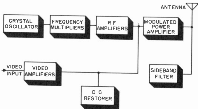
Figure 42. Block diagram of high level modulated transmitter.
