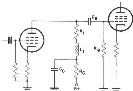
Figure 2. Oscillograph amplifier with high frequency compensation.
