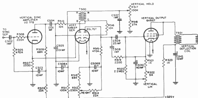
Figure 25. Vertical-deflection circuits.
