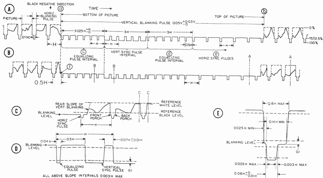
Figure 70. The FCC standard television signal.
