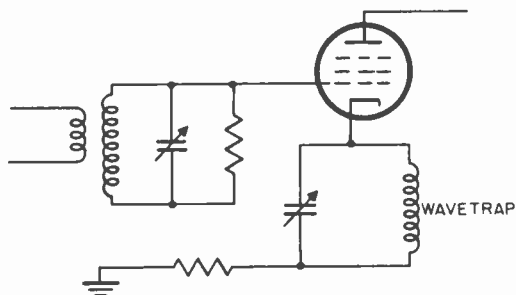
Figure 48. Simplified circuit of i-f amplifier with cathode wavetraps.
