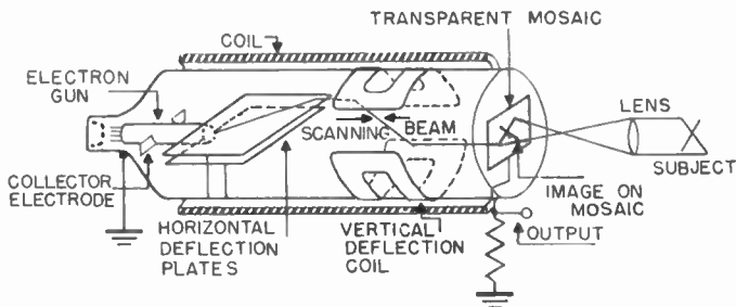
Figure 4. Construction of the orthiconoscope.
