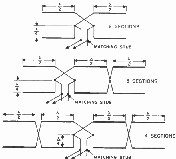
Figure 69. Center-fed flat-top arrays (top view).
