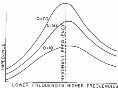
Figure 23. The effect of Q on the selectivity of a parallel tuned circuit.
