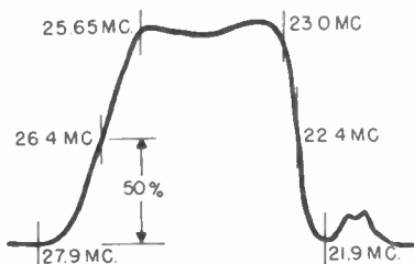
Figure 51. Response curve of i-f amplifier channel using over-coupled transformer and sound traps.
