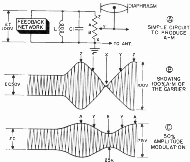
Figure 157. Simple method of amplitude modulation.
