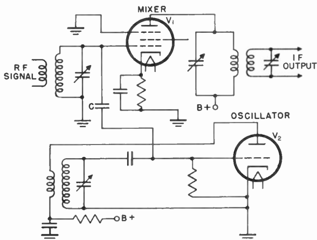
Figure 14. Capacitive-coupled mixer oscillator.
