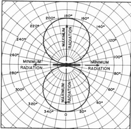
Figure 27. Horizontal field pattern of horizontally polarized half-wave dipole.
