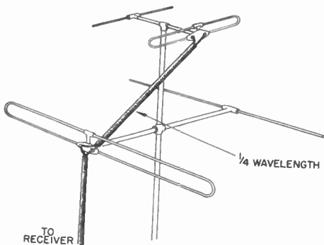
Figure 45. Antennas connected in parallel.
