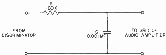
Figure 179. De-emphasis filter.
