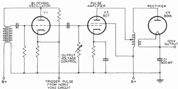
Figure 149. Circuit of a pulse type high-voltage power supply.
