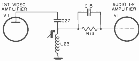
Figure 17. Coupling circuit for separating video and audio signals.
