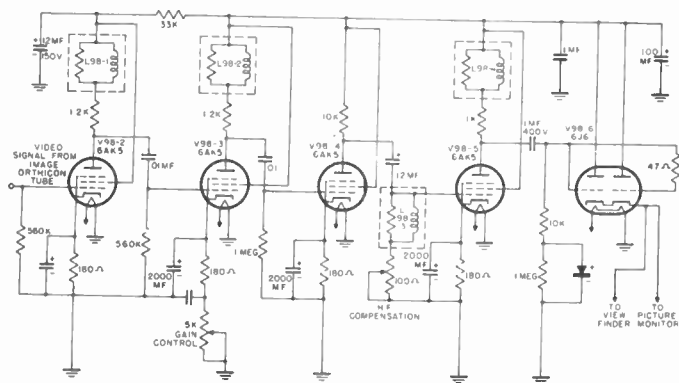
Figure 15. Circuit of video amplifier used in image orthicon camera.
