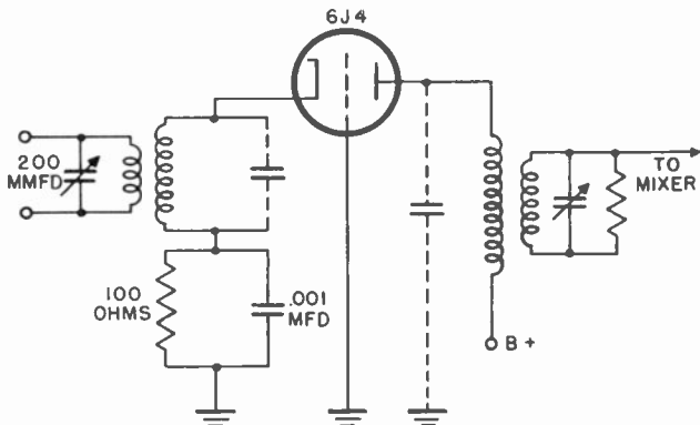
Figure 6. Grounded-grid r-f amplifier.
