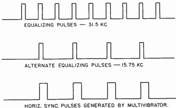
Figure 28. Relative phase of equalizing and horizontal sync pulses.
