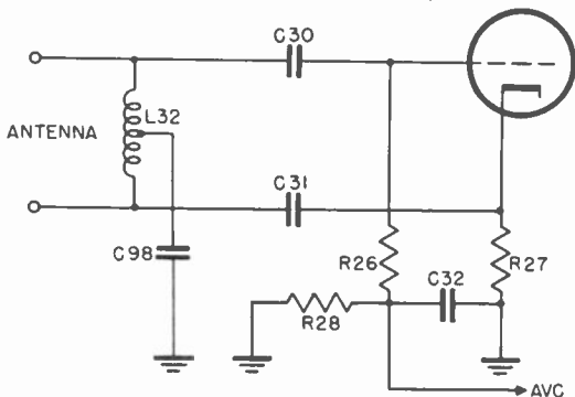
Figure 8. Antenna input circuit.
