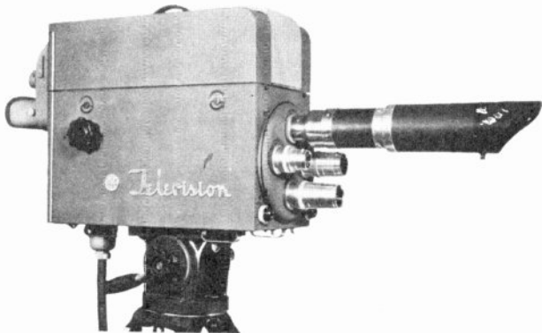
Figure 9. Studio camera equipped with lens turret.
