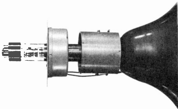
Figure 36. Positions of yoke and focus coils on the neck of a picture tube. (courtesy DuMont)
