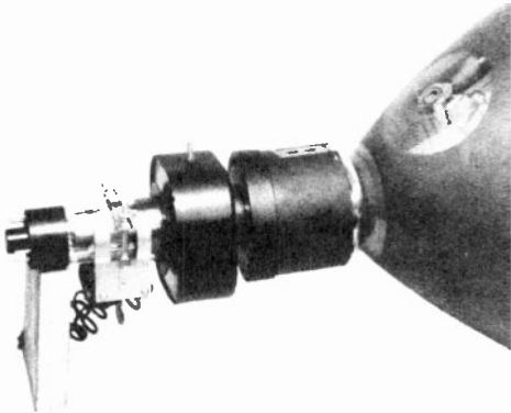
Figure 129. The ion trap magnet is mounted between the tube base and the focus coil.
