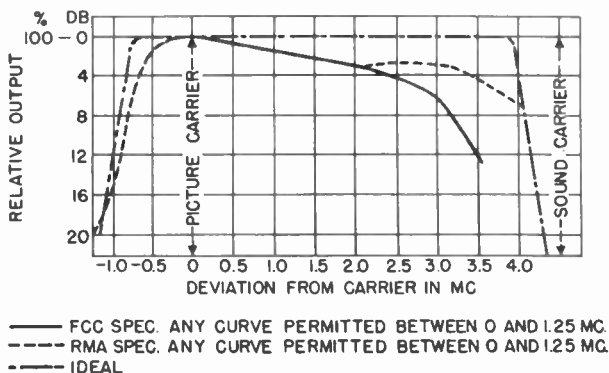
Figure 41. RMA and FCC specified transmission channels.
