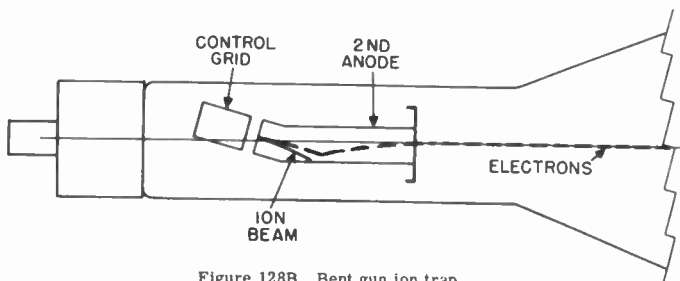
Figure 128B. Bent gun ion trap.
