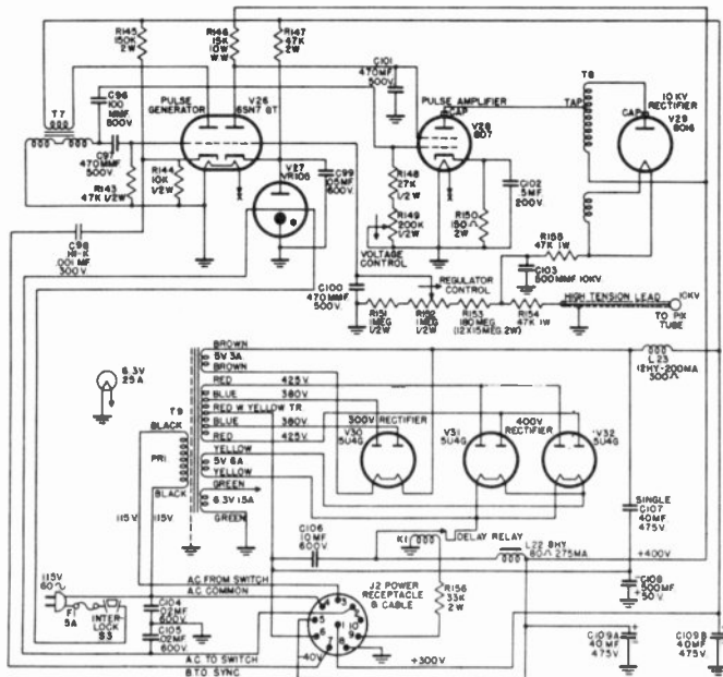
Figure 39. Schematic diagram of low and high voltage power supplies.
