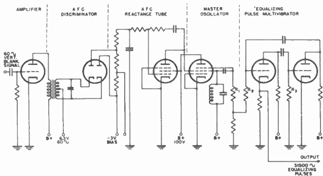
Figure 21. Master oscillator and a-f-c circuits of sync generator.
