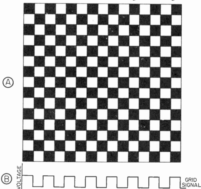
Figure 52. A, checkerboard pattern. Each black and white square is assumed to represent an element in a picture. B, grid voltage which is required to produce checkerboard pattern on the screen of the picture tube.
