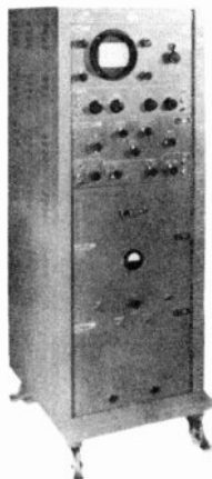
Figure 121. DuMont type 280 oscilloscope. (courtesy DuMont)
