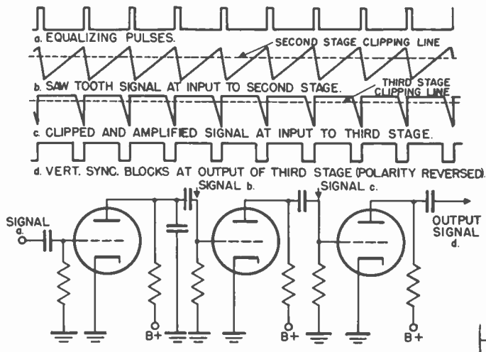
Figure 29. Formation of the vertical sync signal.
