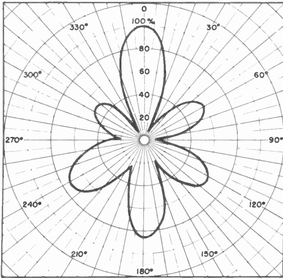
Figure 38 Horizontal field pattern of duo-dipole antenna at 195 Mc.
