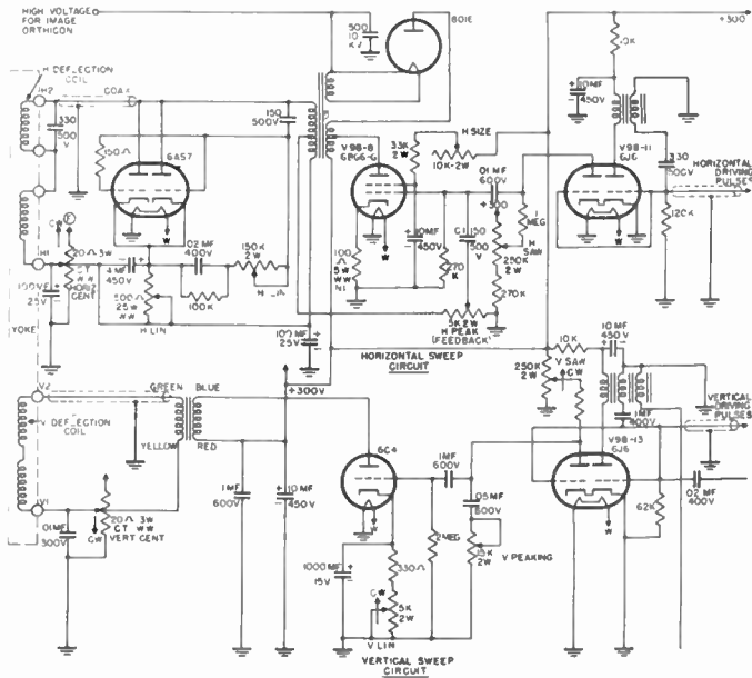
Figure 17. Vertical and horizontal circuits for use with image orthicon.
