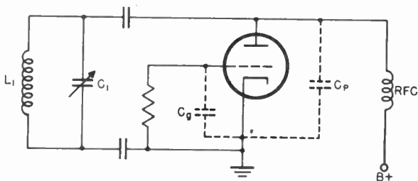
Figure 13. Ultraudion oscillator.
