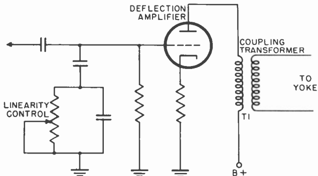
Figure 118. Simplified schematic of deflection amplifier with linearity control.
