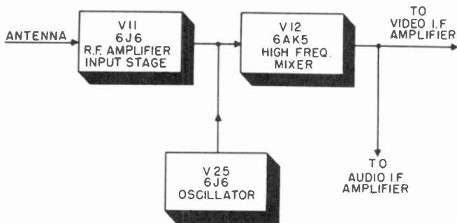
Figure 11. Block diagram of DuMont Inputuner.
