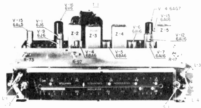
Figure 44. R-F, I-F chassis showing slide-rule dial. (courtesy DuMont)
