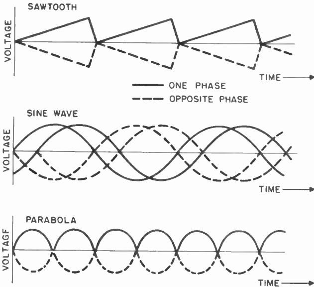
Figure 98. Waveshape used to shade picture.
