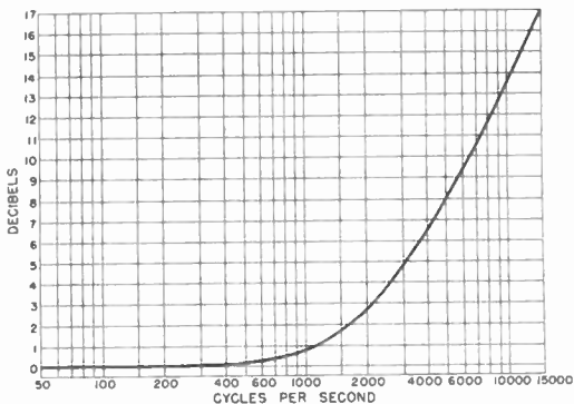
Figure 178. Response characteristic of pre-emphasis filter.
