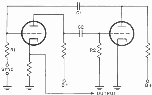
Figure 22. Multivibrator frequency divider.
