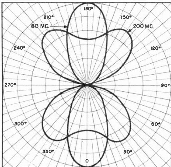
Figure 43. Horizontal field patterns of fan antenna at 80 Mc and 200 Mc.
