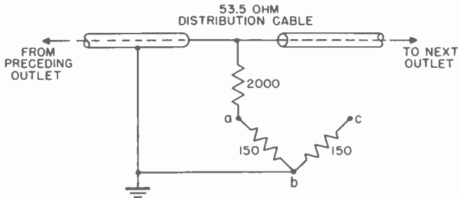
Figure 86. Matching network.
