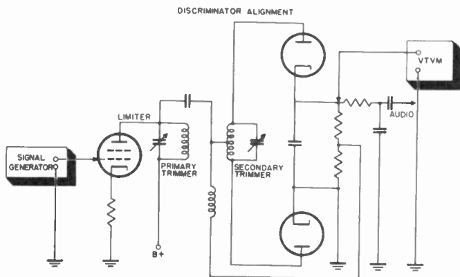
Figure 56. Connections used when aligning discriminator using v.t.v.m.
