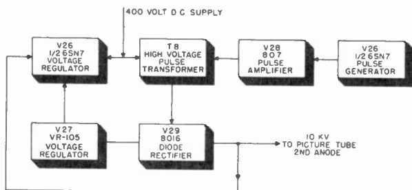
Figure 41. Block diagram of 10KV high voltage supply.
