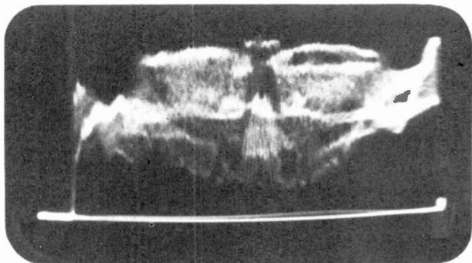
Figure 116. Waveform of properly shaded video signal as it appears on waveform monitor with 7,875-cycle sweep.
