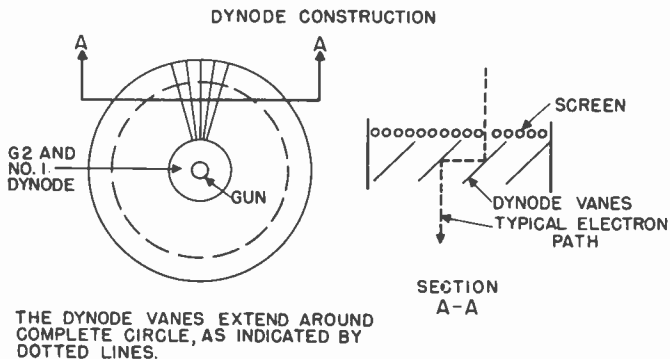
Figure 11. Construction of the dynode vanes in the image orthicon.
