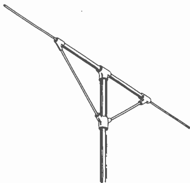
Figure 32. Extended V antenna.
