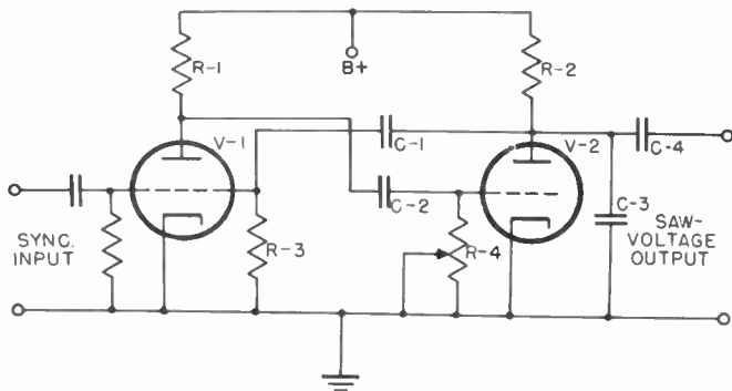
Figure 96. Multivibration circuit.
