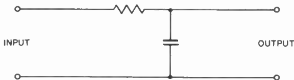
Figure 84. Integrating circuit.
