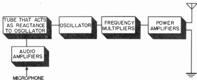
Figure 62. Block diagram of f-m sound transmitter.
