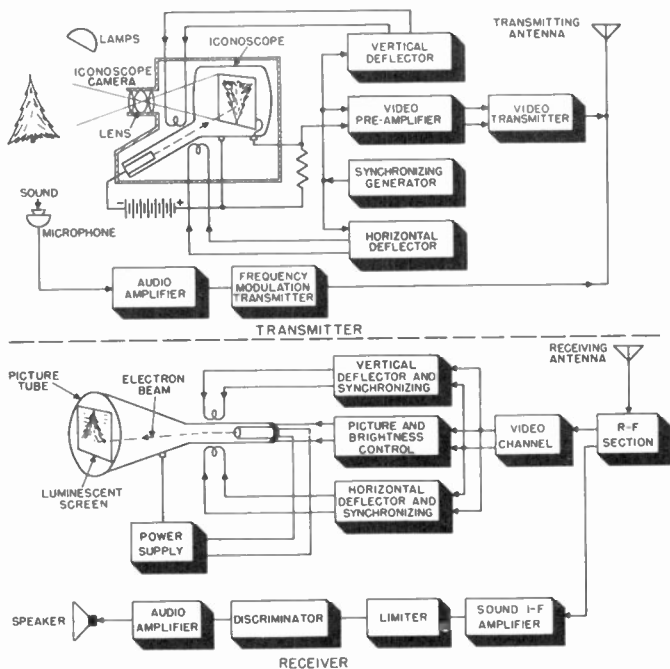
Figure 73. Block diagram of a complete electronic television system.
