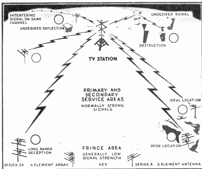
Figure 34. Typical reception problems. (courtesy Workshop Associates)
