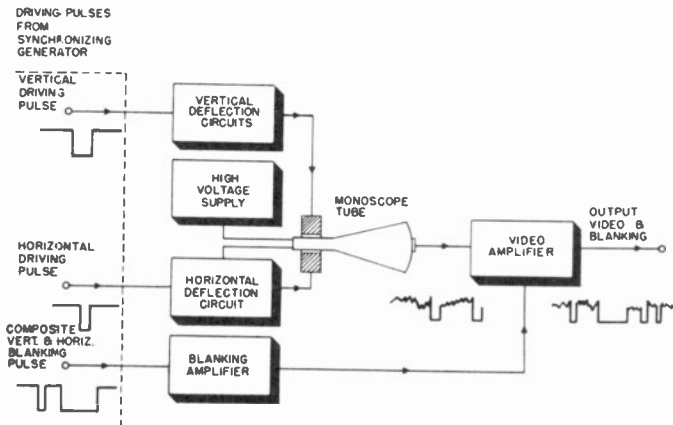
Figure 100. Block diagram of monoscope camera circuit.
