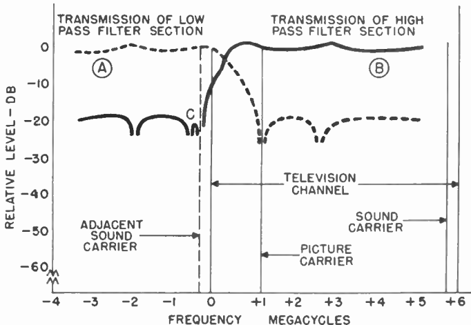
Figure 48. Transmission characteristics of vestigial sideband filter.
