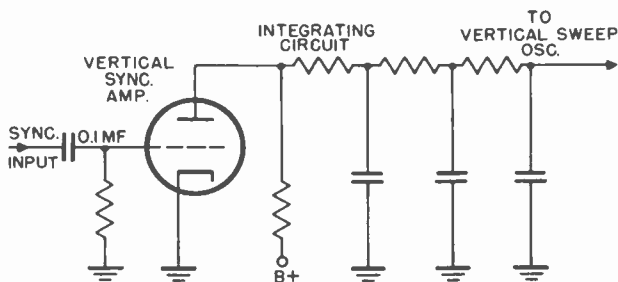
Figure 87. Cascaded integrating circuit.
