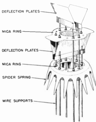
Figure 10. The deflection plate assembly.
