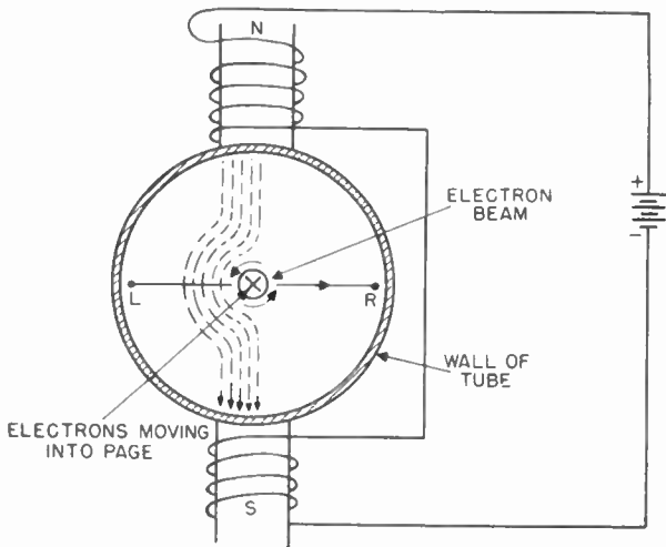
Figure 34. Method of magnetically deflecting the electron beam.
