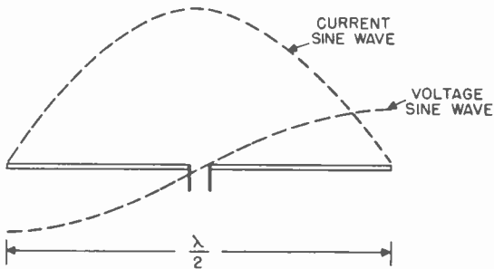
Figure 25. Current and voltage distribution on half-wave dipole.
