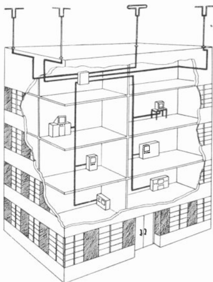
Figure 85. Typical master antenna installation.
