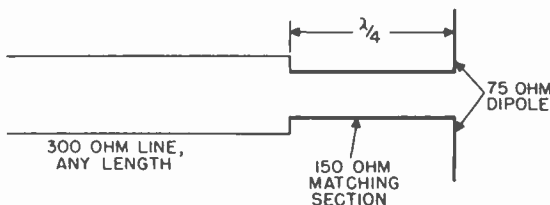
Figure 22. Q matching section.
