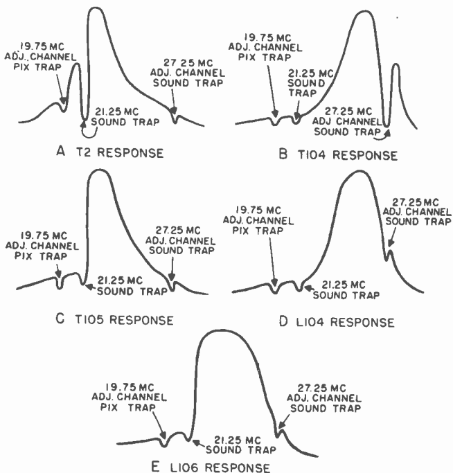
Figure 75. Response curves of stagger-tuned video i-f amplifiers.
