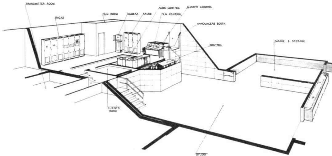
Figure 84. Layout of small television station.
