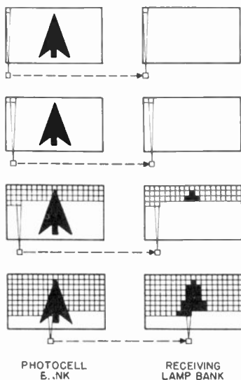
Figure 8. A practical light bulb television system.
