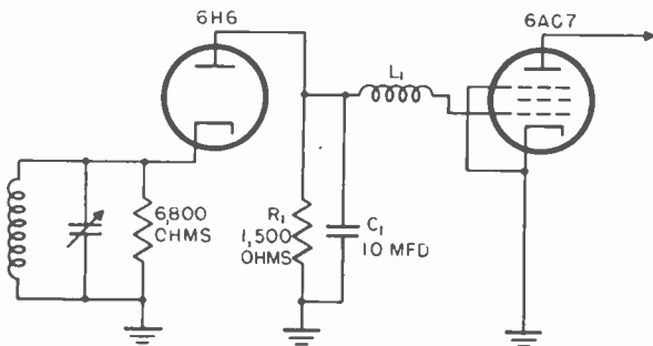
Figure 58. Direct coupled video detector.
