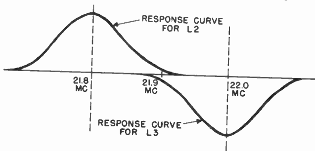
Figure 171. Response curve of tuned circuits of discriminator.
