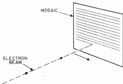
Figure 43. Scanning motion of electron beam across the mosaic.
