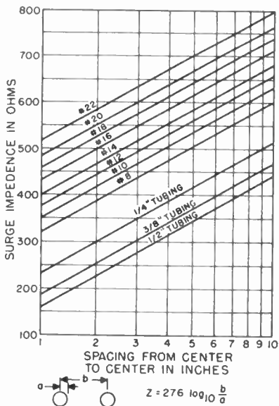
Figure 18. Characteristic impedance of two-conductor parallel transmission lines.
