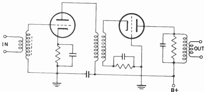
Figure 36. Cascode r-f amplifier.
