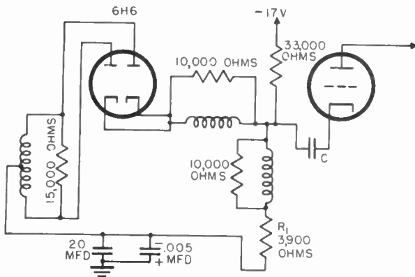
Figure 59. Push-pull video detector.
