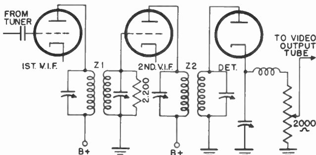
Figure 37. Simplified schematic of broadband overcoupled i-f amplifier.
