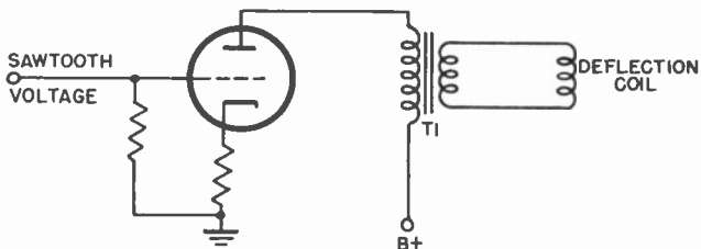
Figure 116. Sweep amplifier for magnetic deflection.
