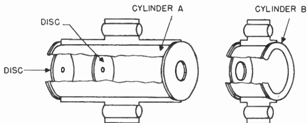
Figure 7. The pre-accelerator electrode assembly.
