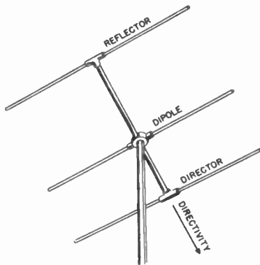
Figure 48. Three-element parasitic array; a reflector and a director with half-wave dipole.
