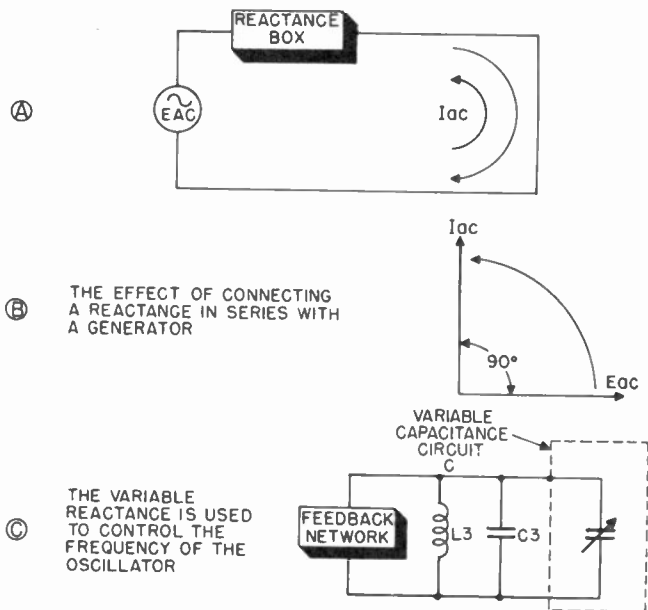
Figure 159. Operation of reactance modulator.
