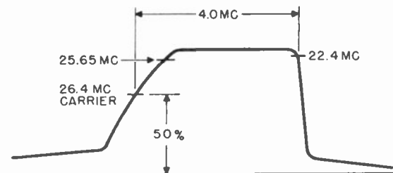
Figure 71. Ideal response curve for video i-f amplifier.
