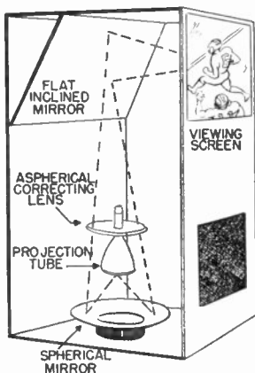
Figure 134. Schmidt projection system.
