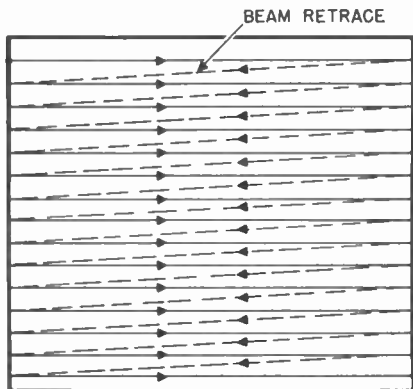
Figure 53A Simple scanning pattern.
