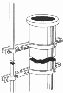
Figure 20. Bracket for mounting on vent pipe.
