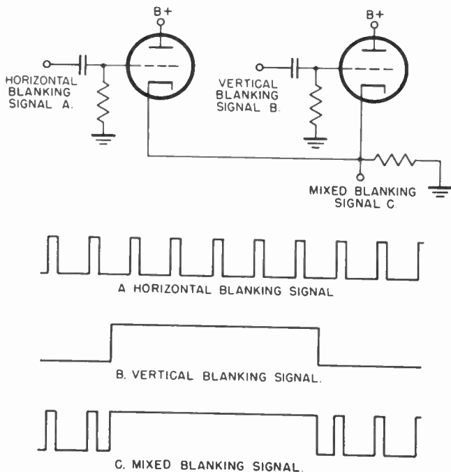
Figure 34. Circuit used to mix horizontal and vertical blanking signals.
