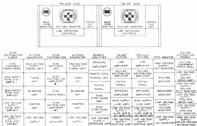
Figure 64. Master control desk and equipment layout.
