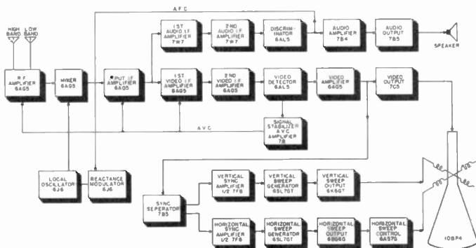
Figure 21. Block diagram of Philco Model 48-1000.
