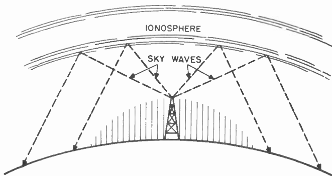
Figure 2. The two principal modes of wave propagation.
