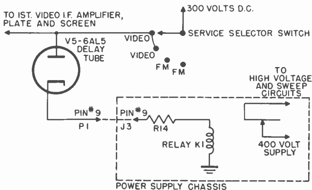
Figure 40. Automatic, high-voltage cutoff circuit.
