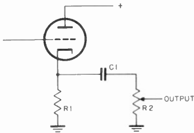
Figure 3. Cathode follower input stage.
