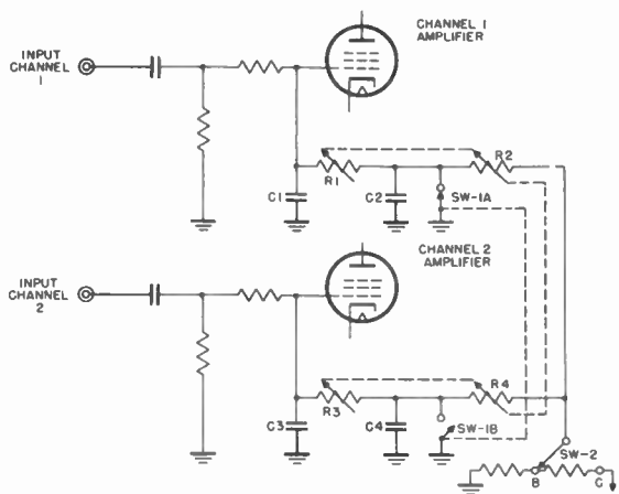
Figure 79. Simplified schematic of input switching circuits.
