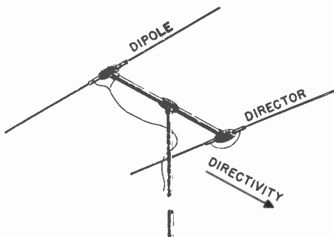
Figure 53. Dipole and director. (courtesy Oak Ridge)
