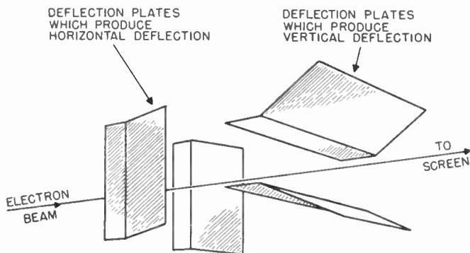
Figure 27. Two pairs of deflection plates mounted at right angles to each other.
