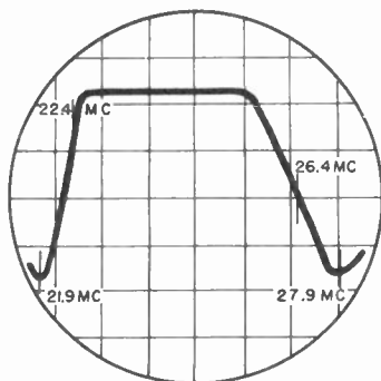
Figure 49. Response curve of video i-f amplifier with sound traps properly tuned.
