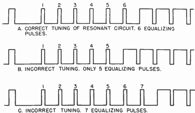
Figure 31. Effect of circuit tuning on composite synchronizing signal.
