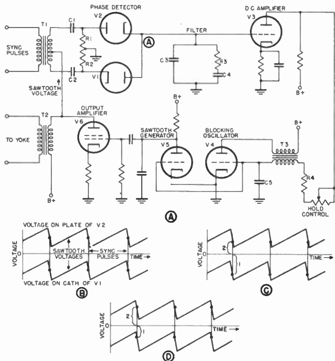
Figure 99. A.F.C. sync circuit and operating waveform.
