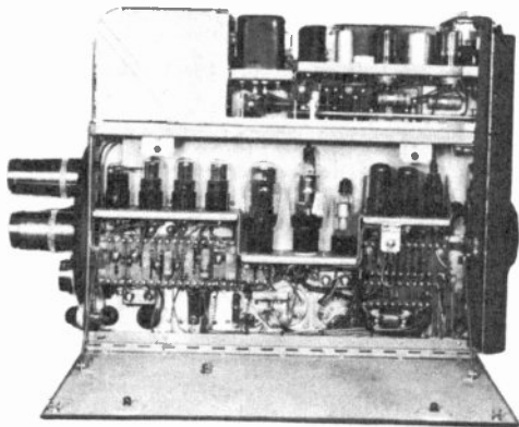
Figure 88. Interior of image-orthicon camera. (courtesy RCA)
