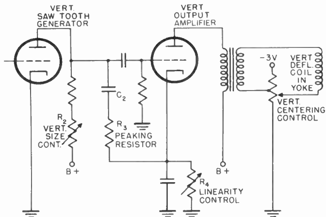
Figure 117. Vertical amplifier circuit.
