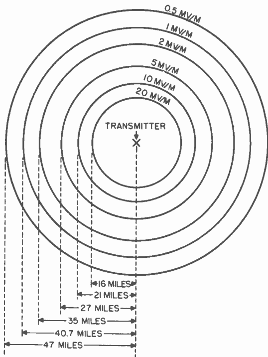
Figure 4. Ground-wave signal range of television station.
