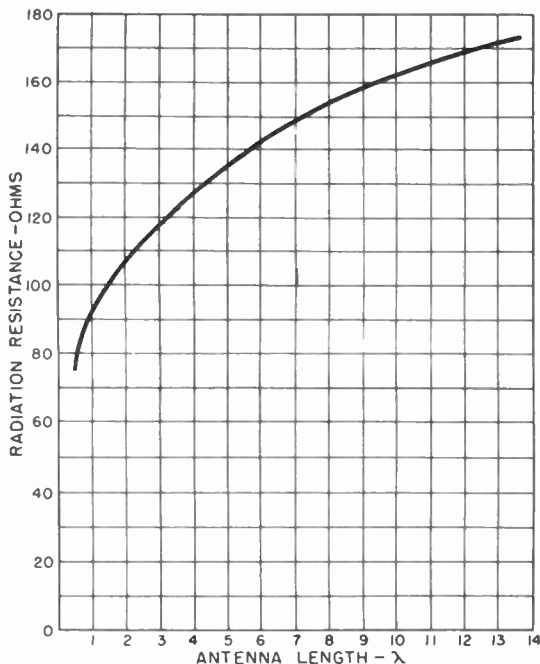
Figure 73. Radiation resistance of long-wire antenna.
