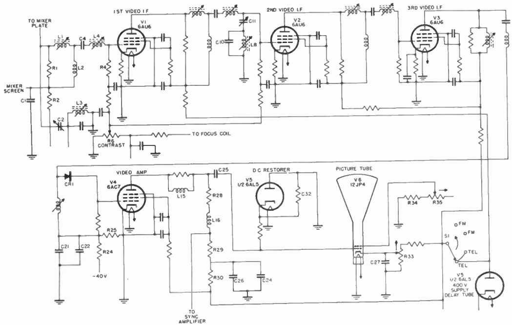
Figure 33. Video circuits.
