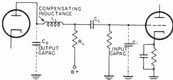
Figure 64. Series-peaking frequency compensation.
