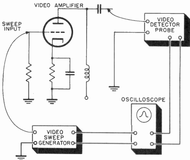
Figure 65. Connections used to adjust video amplifier using sweep generator and oscilloscope.
