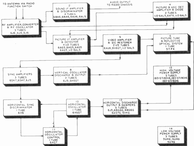
Figure 52. Block diagram of Model 648 PTK.
