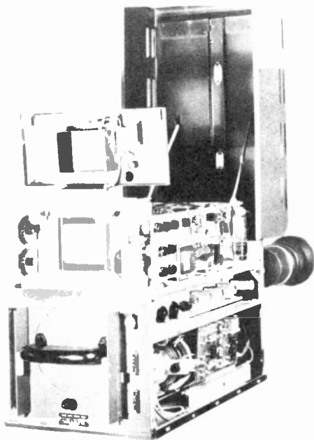
Figure 14. Pickup head and electronic viewfinder. (courtesy DuMont)
