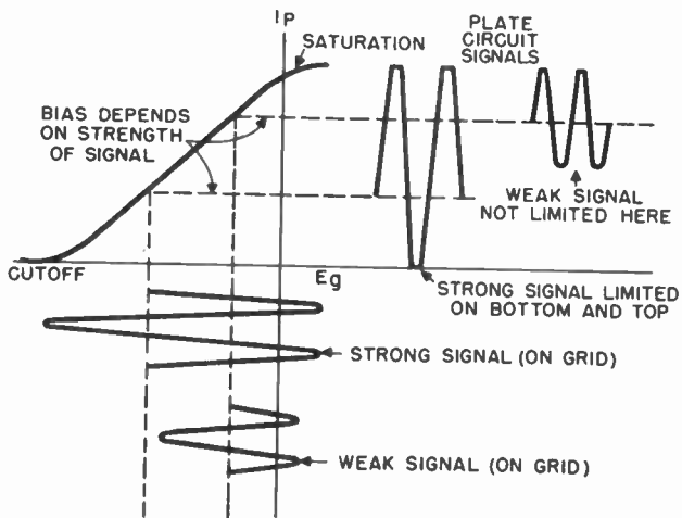
Figure 166. Operation of limiter circuit.
