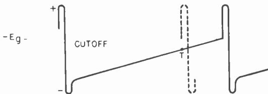
Figure 94. Grid voltage cycle of blocking oscillator.
