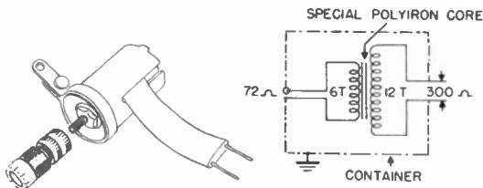
Figure 30. Circuit and appearance of line matching transformer.
