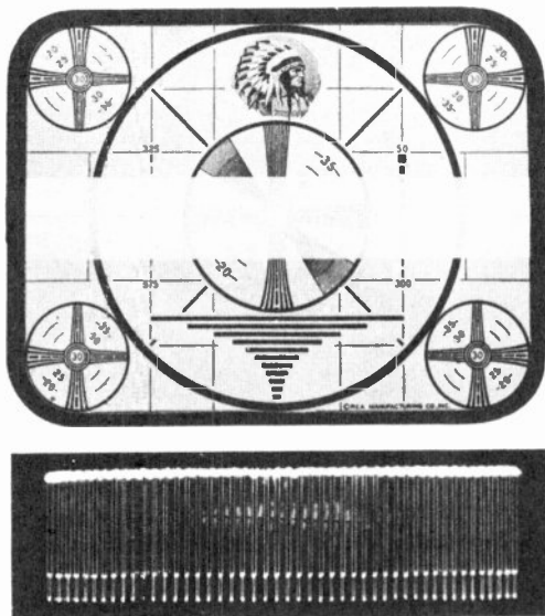
Figure 127. Oscilloscope of several horizontal lines and test pattern with marker to indicate portion of pattern used.
