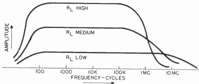
Figure 66. Effect of different load resistances on the response of resistance coupled amplifier.
