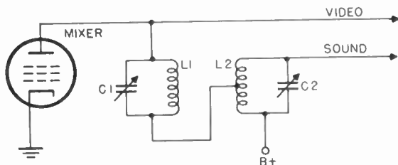
Figure 19. Circuit used to separate the video and audio signals.
