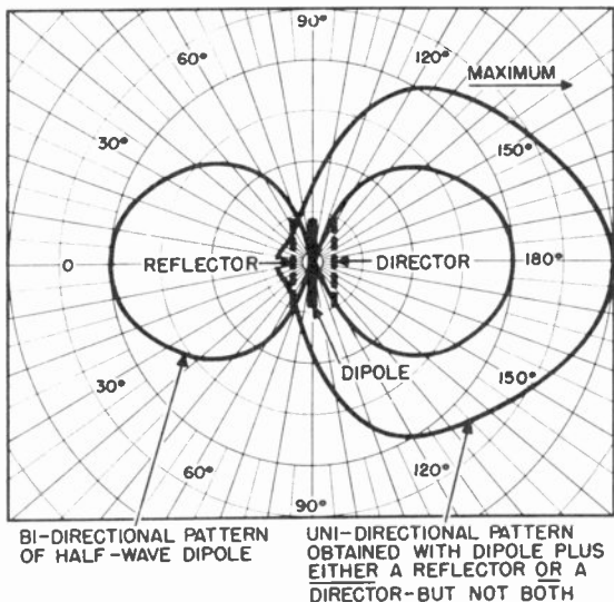
Figure 50. Change in bi-directional field pattern of dipole when either reflector or director is added to dipole.
