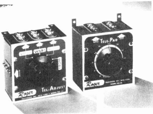
Figure 37. The Tel-Adjust and the Tele-Pad, used to reduce too strong a signal. (courtesy Roger Television)
