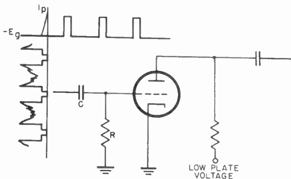
Figure 82. Simplified schematic of triode sync clipper.
