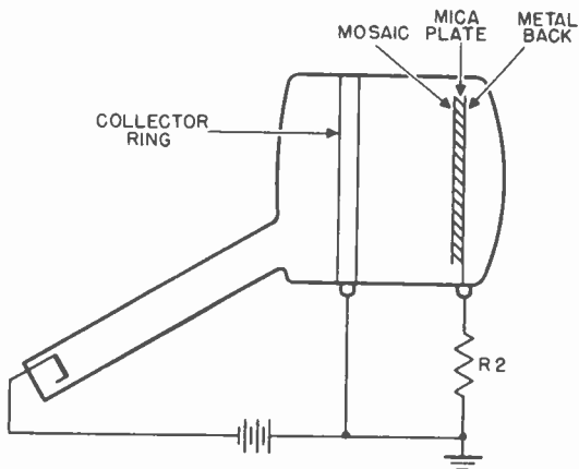
Figure 42. Path of electrons in iconoscope circuit.
