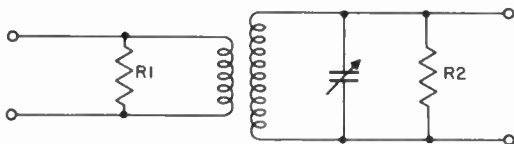
Figure 26. Transformer shunted with resistors to flatten and broaden its response.
