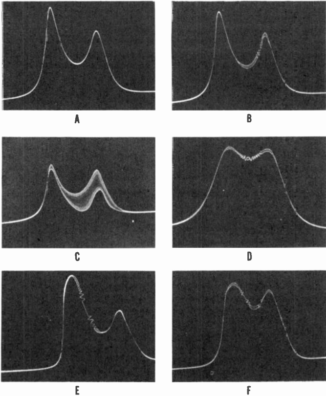
Figure 64. Response curves of sound i-f amplifiers. A. Single i-f response curve, B. Response curve with birdie at 21.9 Mc, C. Effect of too much birdie, D. Response curve of properly aligned i-f amplifier, E. Effect produced by slight overload, F. Effect produced by excessive overload.
