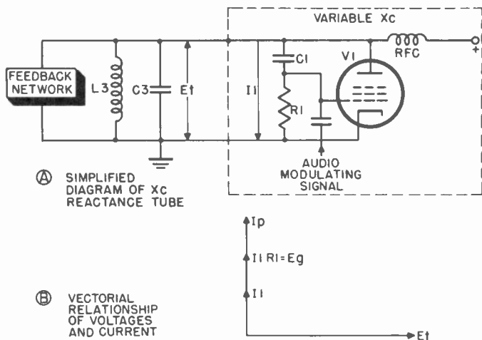
Figure 160. Simplified schematic of a reactance tube modulator.
