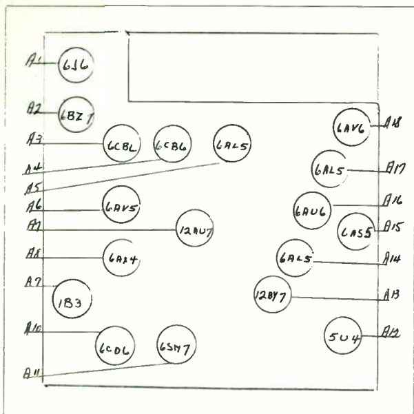
ADMIRAL - LAYOUT NO. 17
