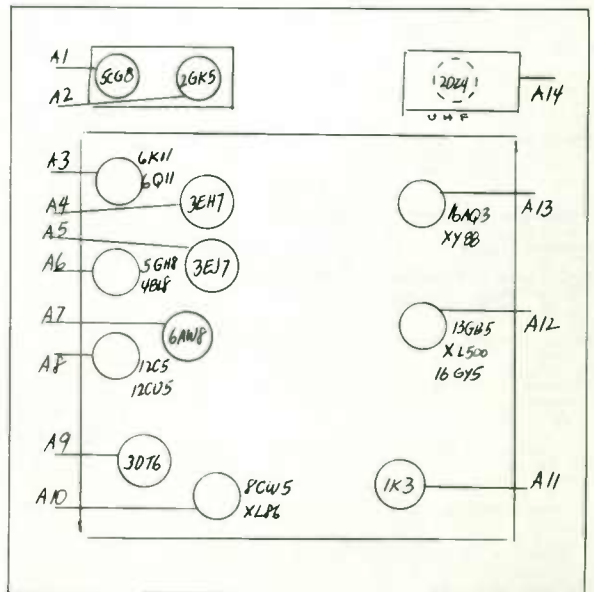
EMERSON - LAYOUT NO. 68
