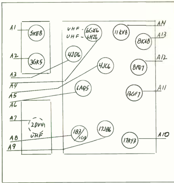
R.C.A. - LAYOUT NO. 151
