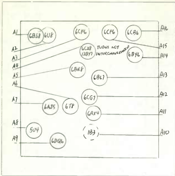
GENERAL ELECTRIC-LAYOUT NO. 109
