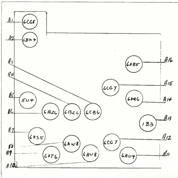
ADMIRAL - LAYOUT NO. 18
