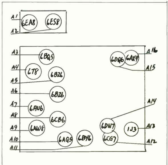
GENERAL ELECTRIC - LAYOUT NO. 94
