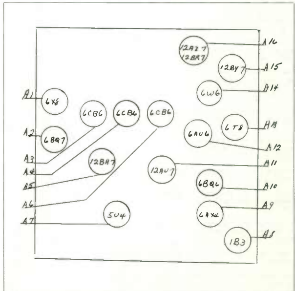
PHILCO - LAYOUT NO. 142
