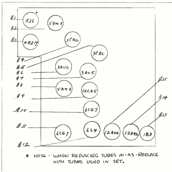
ADMIRAL - LAYOUT NO.10
