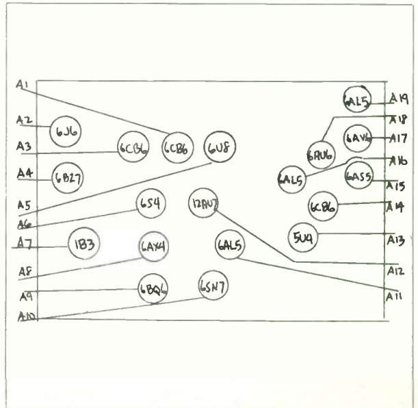
ADMIRAL - LAYOUT NO. 22
