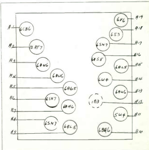
MOTOROLA - LAYOUT NO. 128
