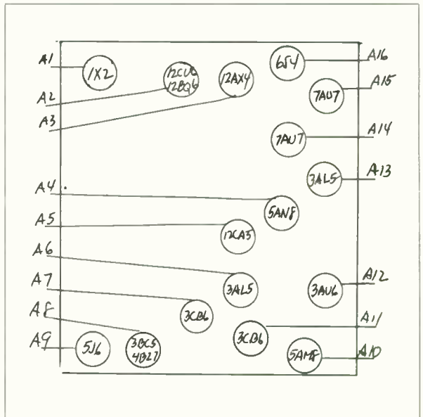
ADMIRAL - LAYOUT NO. 6
