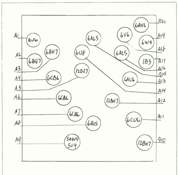
C.B.S. COLUMBIA - LAYOUT NO. 40
