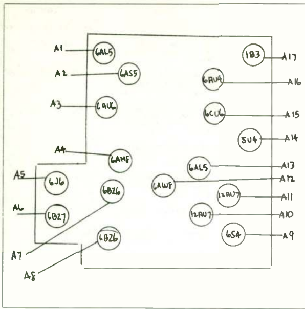
ADMIRAL - LAYOUT NO. 21
