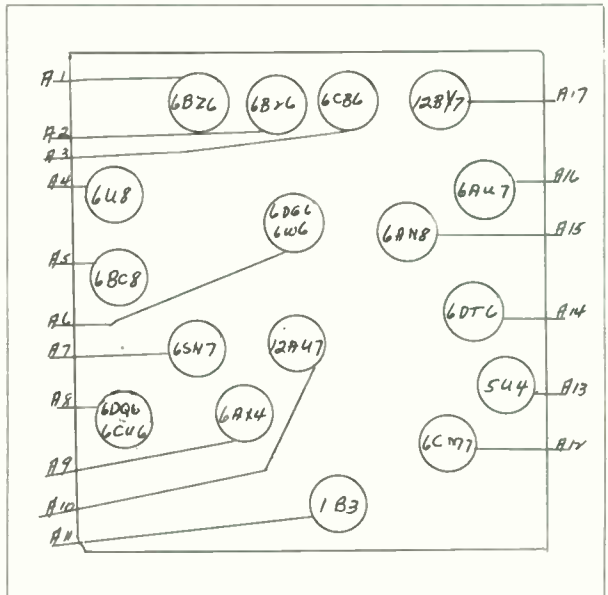
MAGNAVOX - LAYOUT NO. 120
