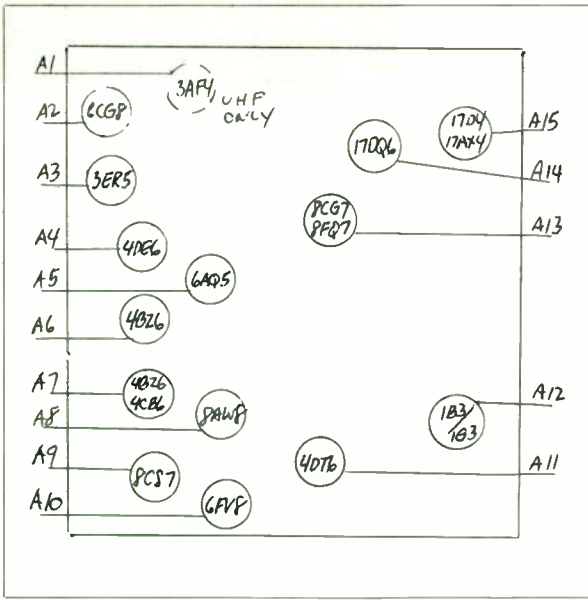
WESTINGHOUSE - LAYOUT NO. 201
