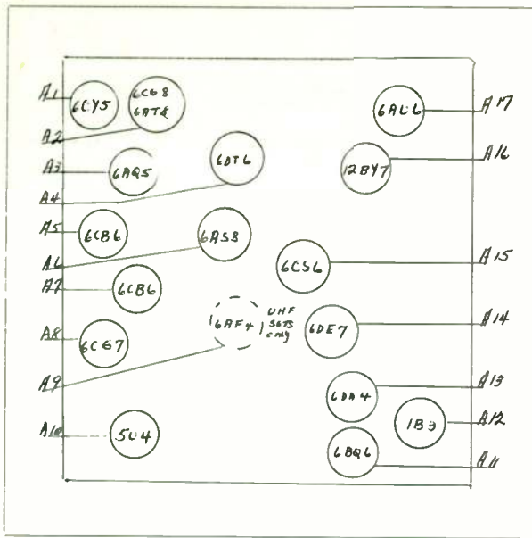
EMERSON - LAYOUT NO. 85
