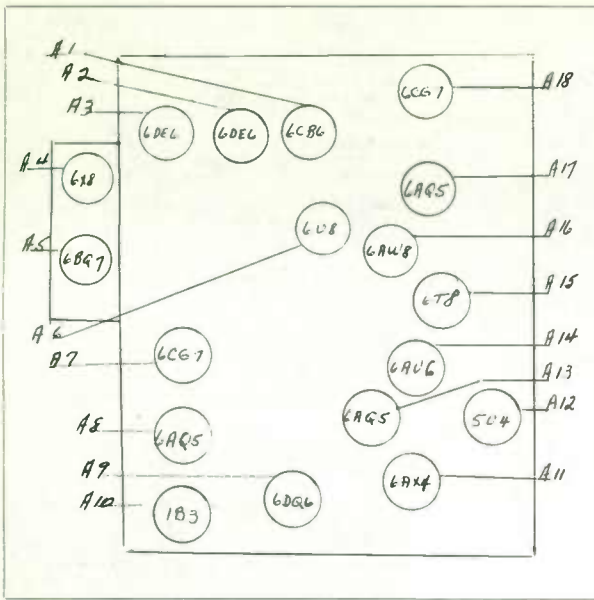
R.C.A. - LAYOUT NO. 167
