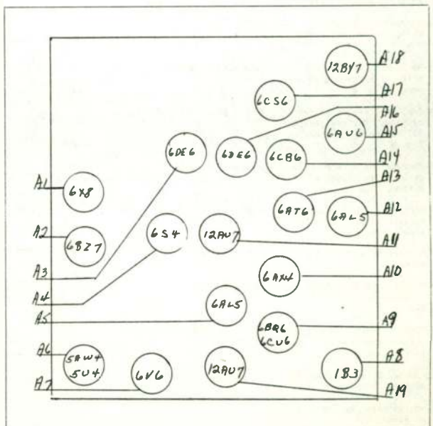
PHILCO - LAYOUT NO. 144
