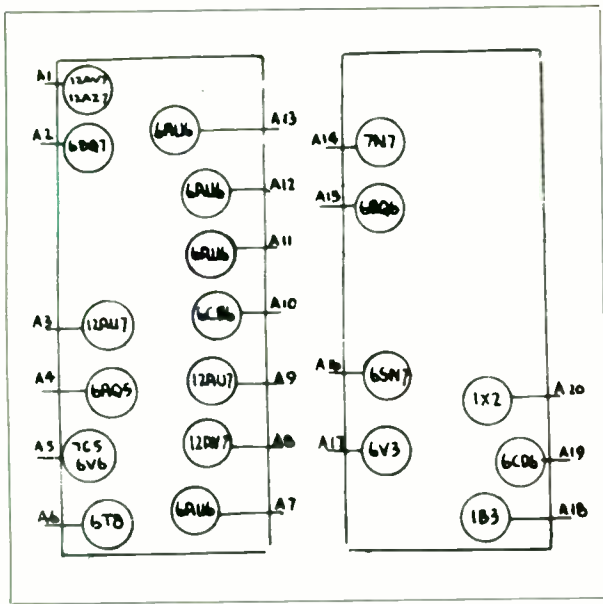
PHILCO - LAYOUT NO. 147
