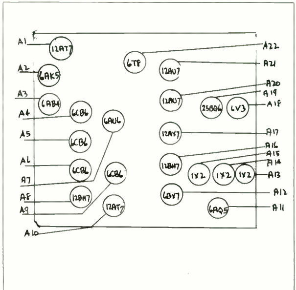
GENERAL ELECTRIC-LAYOUT NO. 114
