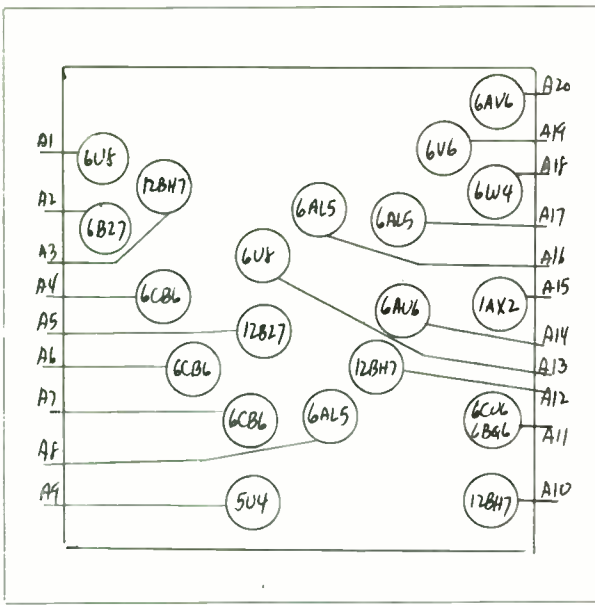
C.B.S. COLUMBIA - LAYOUT NO. 33
