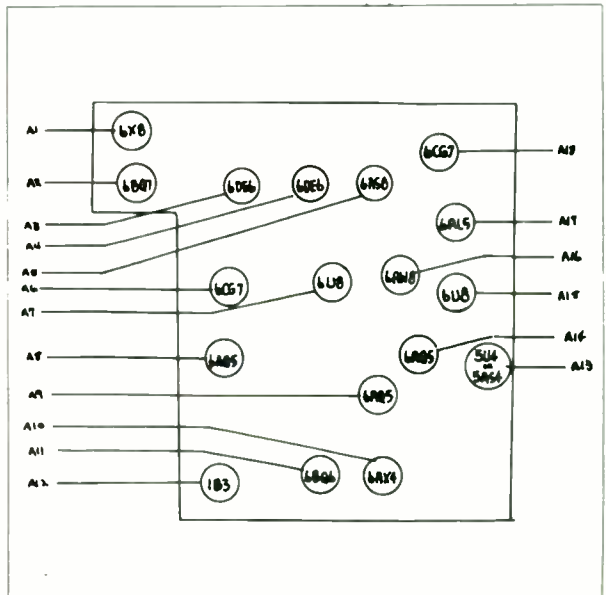
R.C.A. - LAYOUT NO. 156
