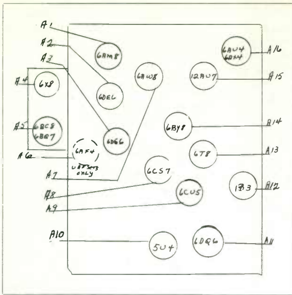
PHILCO - LAYOUT NO. 141
