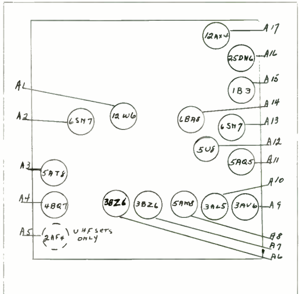
SYLVANIA - LAYOUT NO. 178
