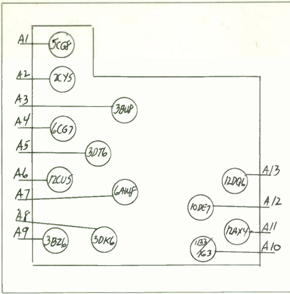
ADMIRAL - LAYOUT NO. 29
