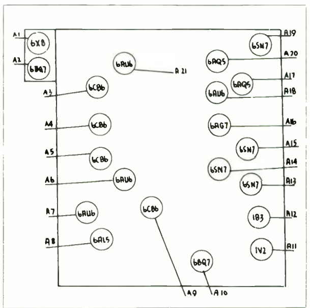
R.C.A. - LAYOUT NO. 162
