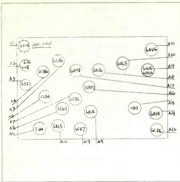
ADMIRAL - LAYOUT NO. 15
