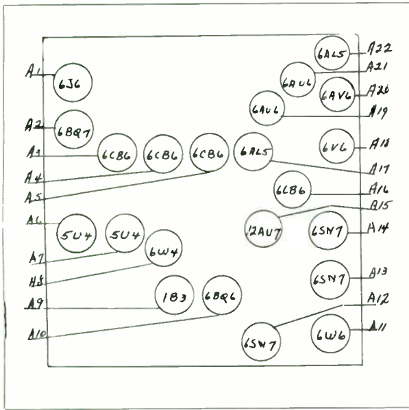
EMERSON - LAYOUT NO. 83
