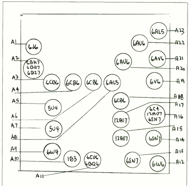
EMERSON - LAYOUT NO. 86
