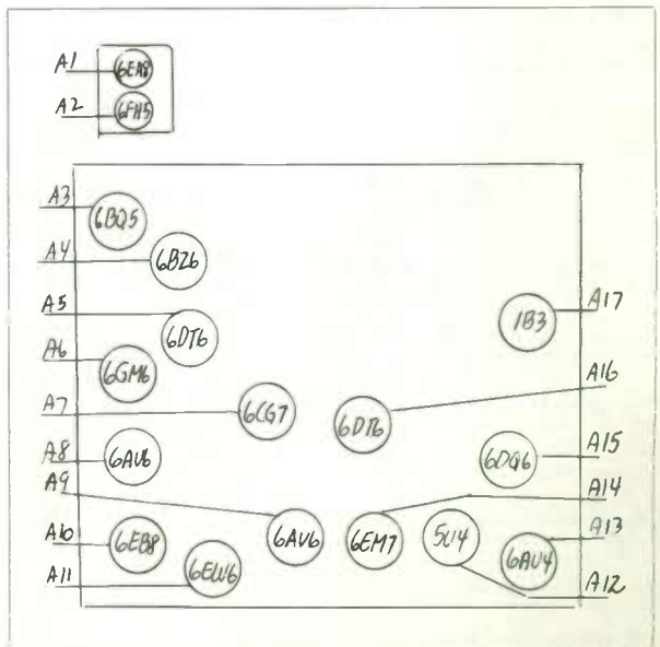
R.C.A. - LAYOUT NO. 160
