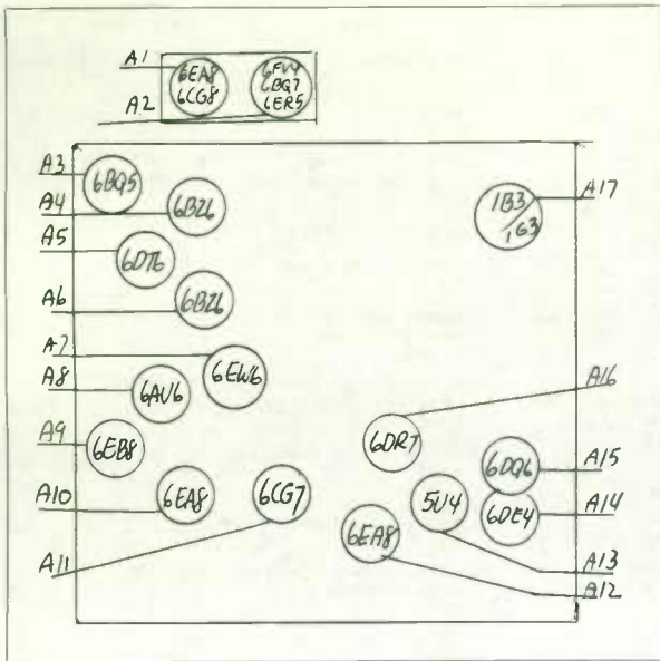
R.C.A. - LAYOUT NO. 159
