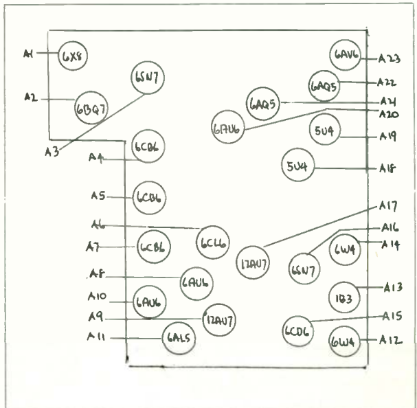
R.C.A. - LAYOUT NO. 152
