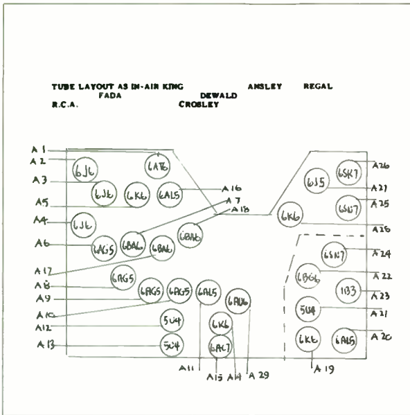
R.C.A. - LAYOUT NO. 161
