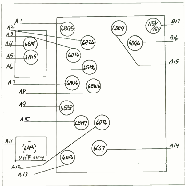
R.C.A. - LAYOUT NO. 154
