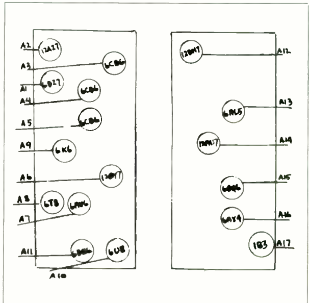
PHILCO - LAYOUT NO. 146
