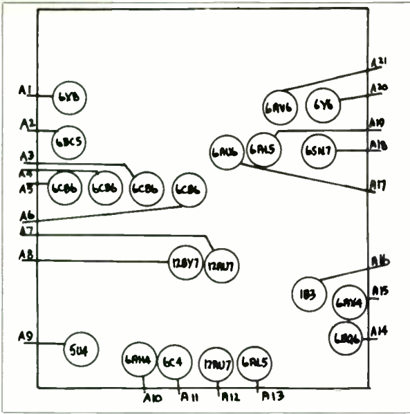
SYLVANIA - LAYOUT NO. 177
