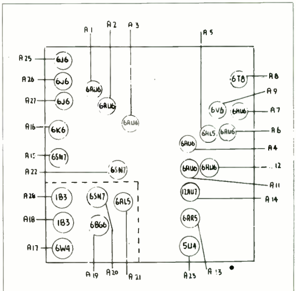
EMERSON - LAYOUT NO. 76
