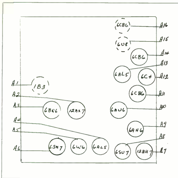
MOTOROLA - LAYOUT NO. 129
