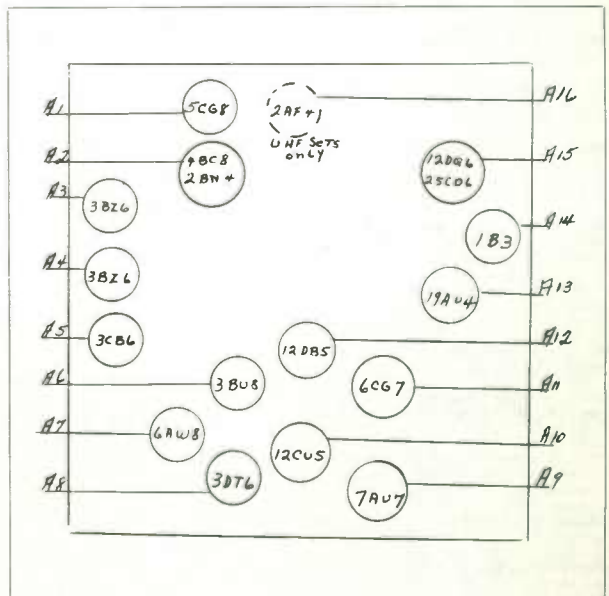
ADMIRAL - LAYOUT NO. 16
