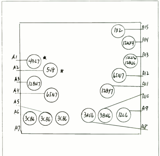
C.B.S. COLUMBIA - LAYOUT NO. 34
