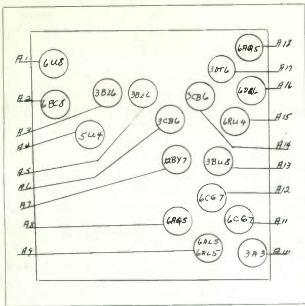
MOTOROLA - LAYOUT NO. 127
