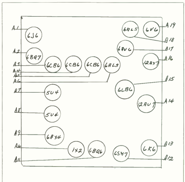
EMERSON - LAYOUT NO. 80
