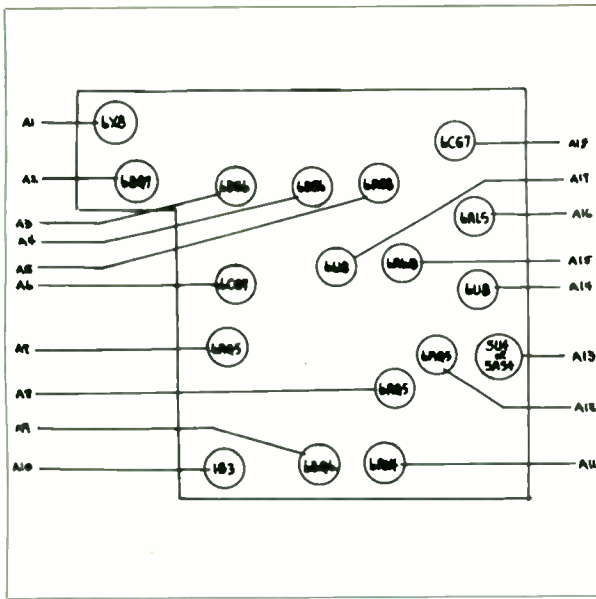
R.C.A. - LAYOUT NO. 155
