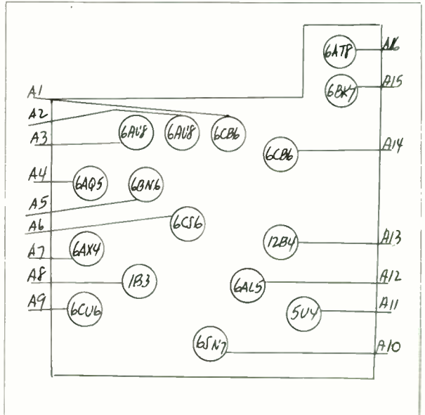
DUMONT - LAYOUT NO. 52
