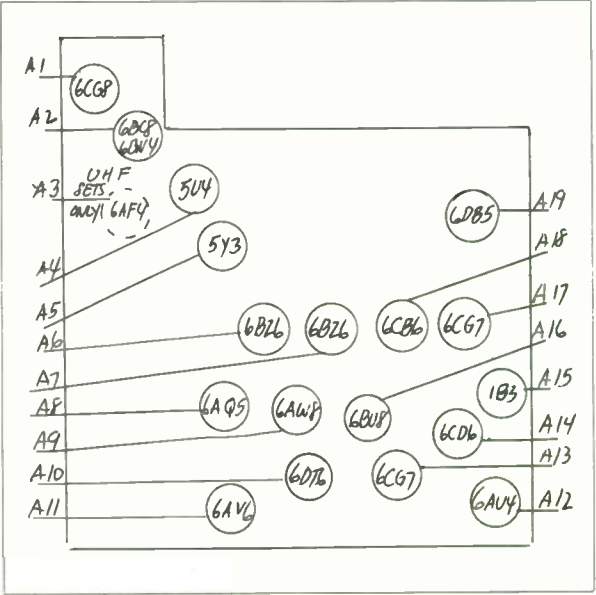
ADMIRAL - LAYOUT NO. 30
