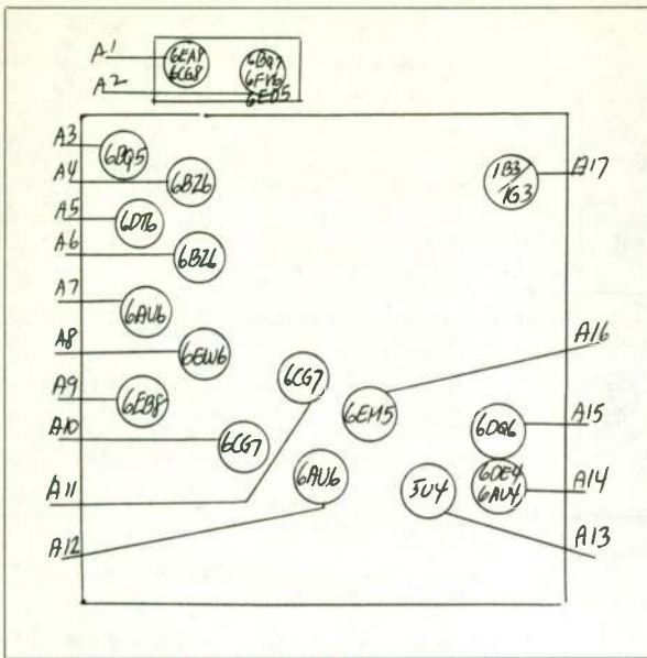
R.C.A. - LAYOUT NO. 157
