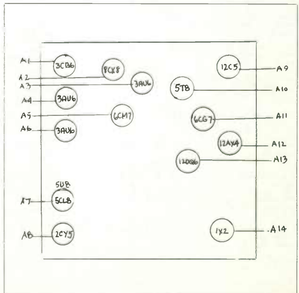
GENERAL ELECTRIC-LAYOUT NO. 110
