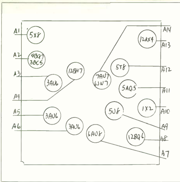
GENERAL ELECTRIC - LAYOUT NO. 93
