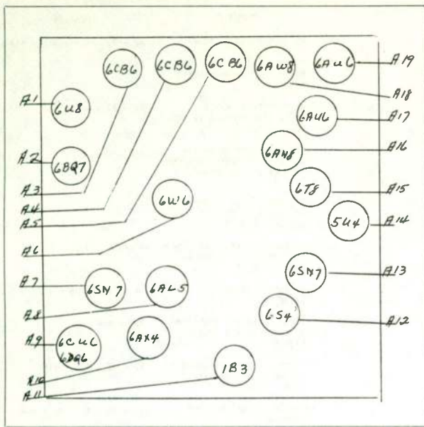
MAGNAVOX - LAYOUT NO. 119
