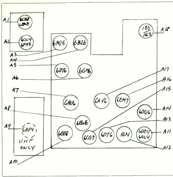
R.C.A. - LAYOUT NO. 153
