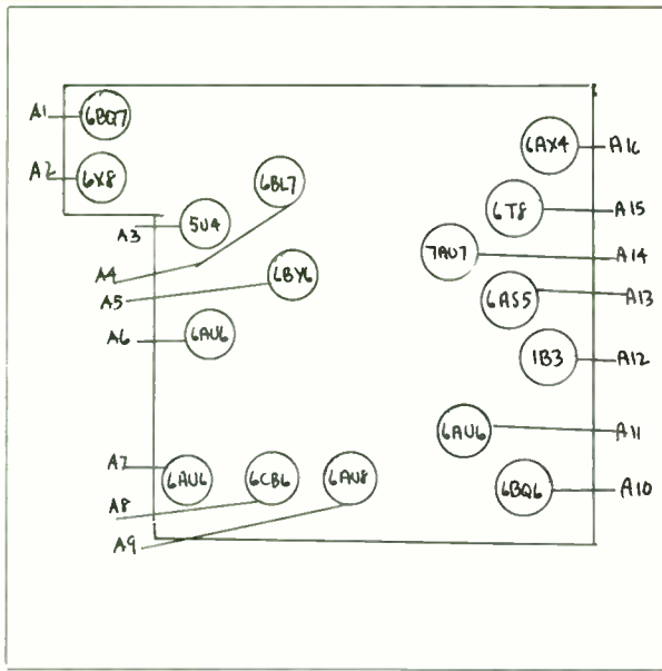
GENERAL ELECTRIC-LAYOUT NO. 113
