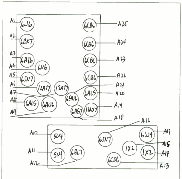
DUMONT - LAYOUT NO. 58
