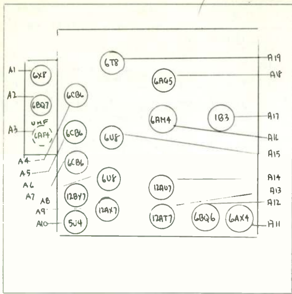
GENERAL ELECTRIC - LAYOUT NO. 101
