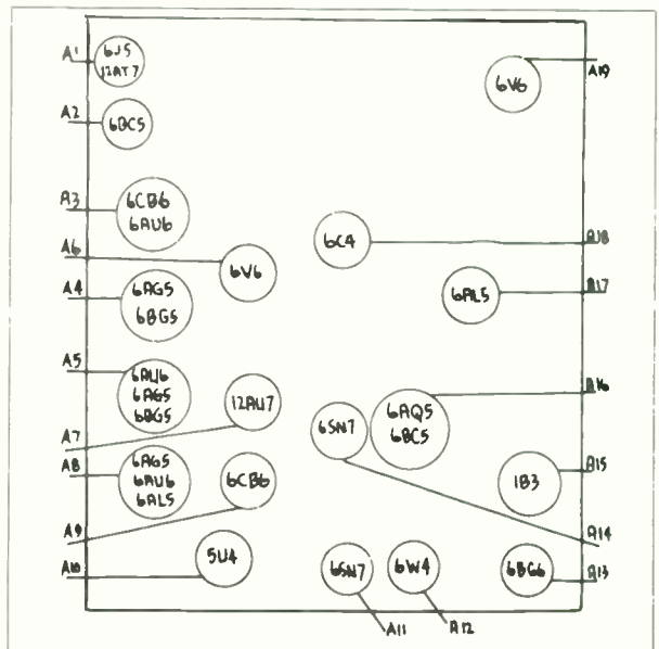
MAGNAVOX - LAYOUT NO. 122
