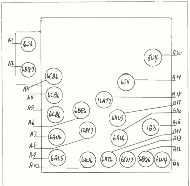
DUMONT - LAYOUT NO. 56
