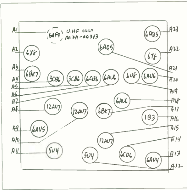
DUMONT - LAYOUT NO. 55
