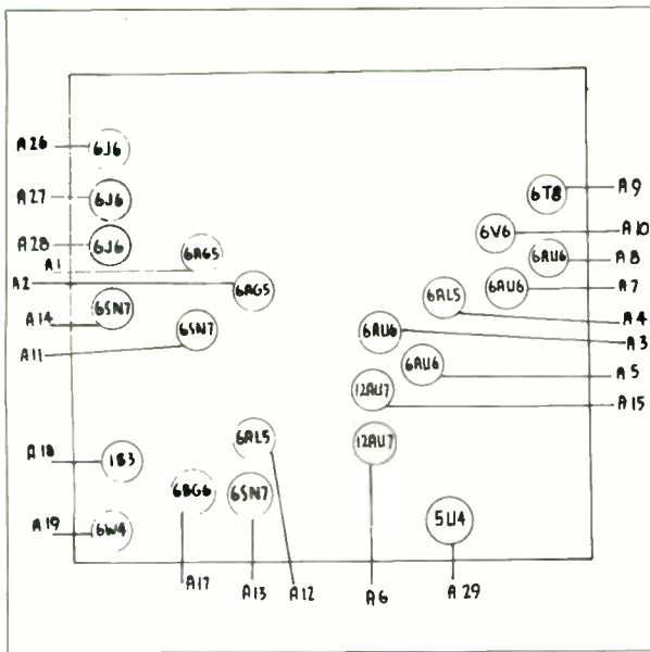
EMERSON - LAYOUT NO. 75
