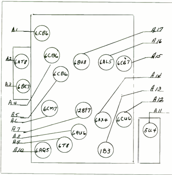
DUMONT - LAYOUT NO. 57
