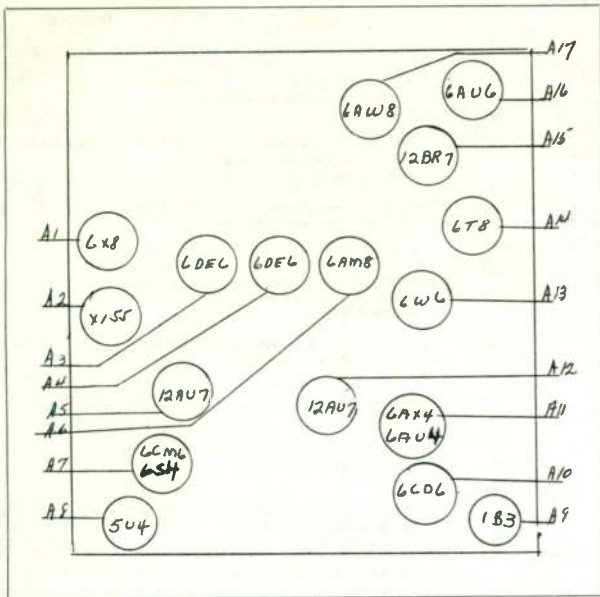
PHILCO - LAYOUT NO. 143
