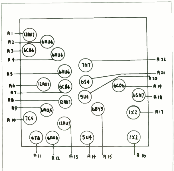
PHILCO - LAYOUT NO. 148
