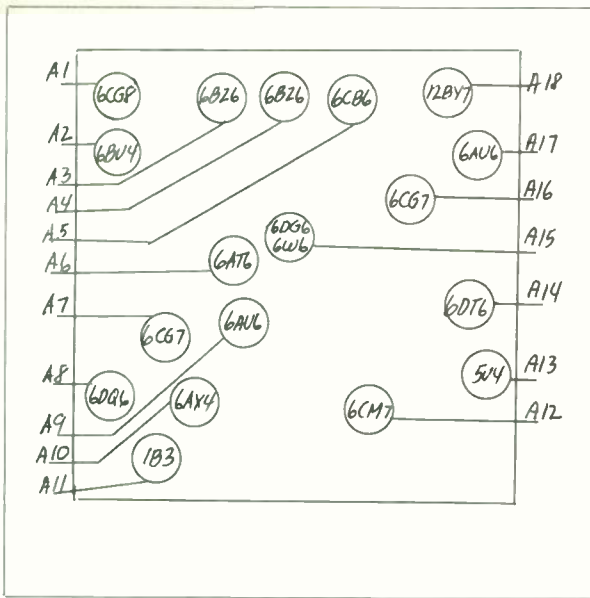
MAGNAVOX - LAYOUT NO. 121
