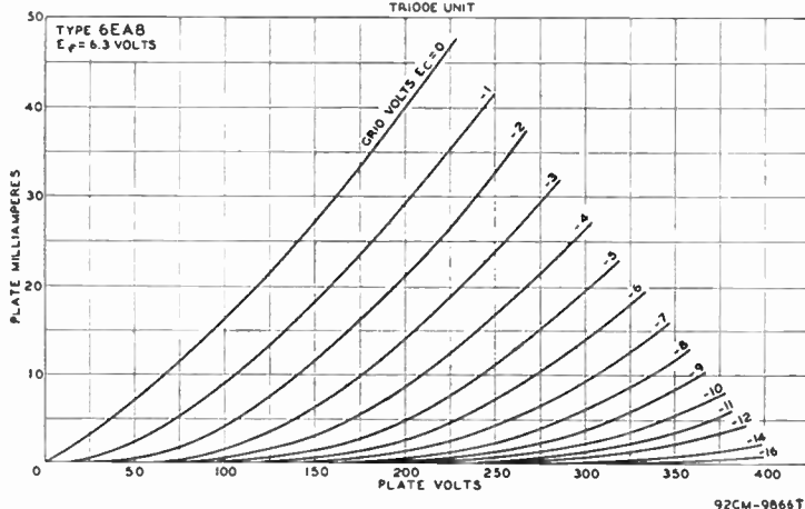
AVERAGE PLATE CHARACTERISTICS TRIODE UNIT
