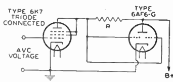
R: TYPICAL VALUE IS 0.5 MEGOHM Fig. 66
