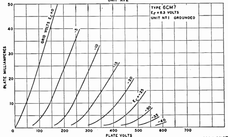
AVERAGE CHARACTERISTICS UNIT #2
