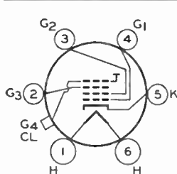
6AL ULTOR = G 4 + CL FOCUSING ELECTRODE = G 3
