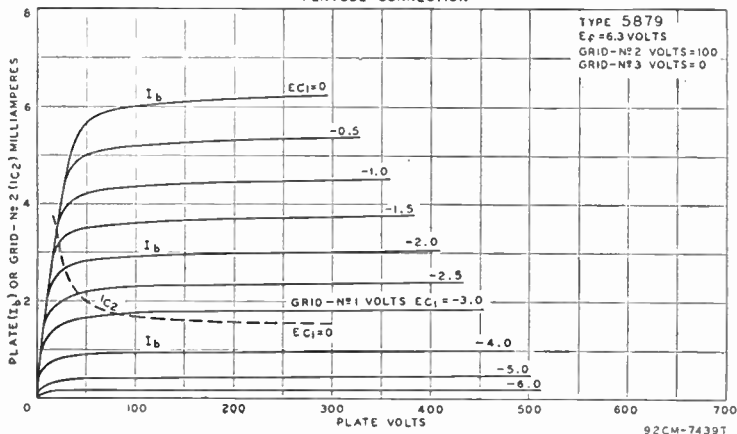
AVERAGE CHARACTERISTICS PENTODE CONNECTION
