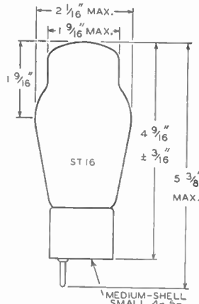
-51- MEDIUM-SHELL SMALL 4-5- OR 6-PIN; MEDIUM 7-PIN
