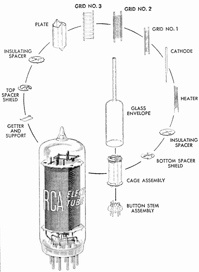
Parts of a Miniature Pentode
