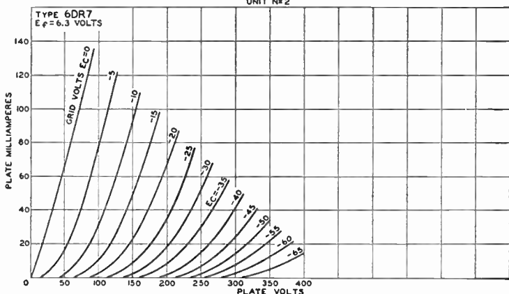
AVERAGE PLATE CHARACTERISTICS UNIT NR 2
