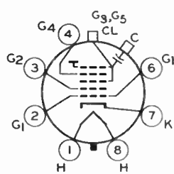
8HR ULTOR = G 3 + G 5 + CL FOCUSING ELECTRODE = G 4
