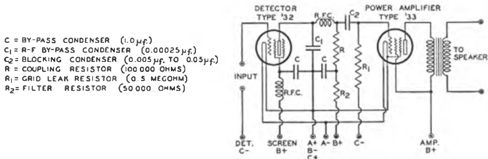
OPTIONAL DETECTOR AND AMPLIFIER—2-VOLT FILAMENT TYPES
