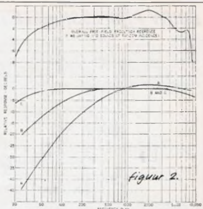
USASI (ASA) Standard S1-4-1961. Weighted curves for sound-level meters. Used in all instruments manufactured since 1951.
