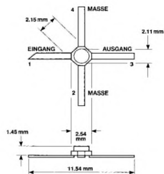
35 micro-X
