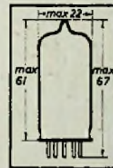
ECH 81 UCH 81
