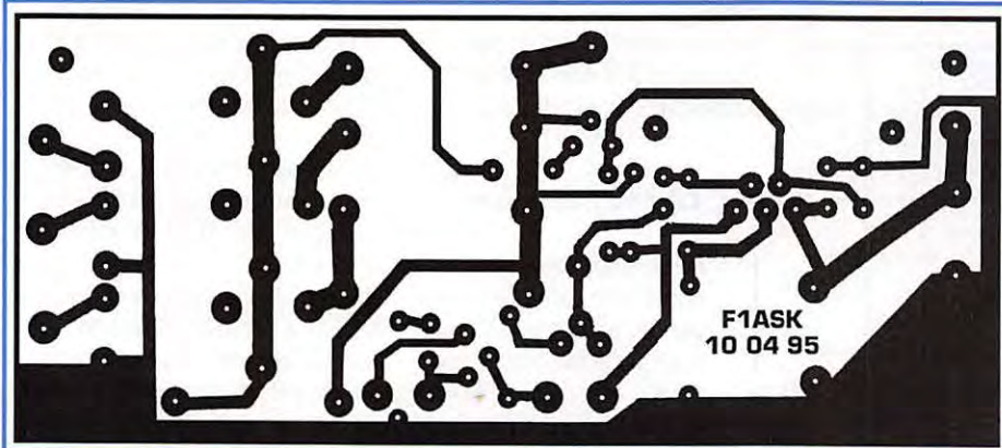
C.I. face composants.
