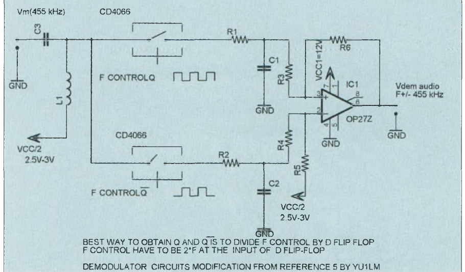
DEMODULATOR CIRCUITS MODIFICATION FROM REFERENCE 5 BY YU1LM
