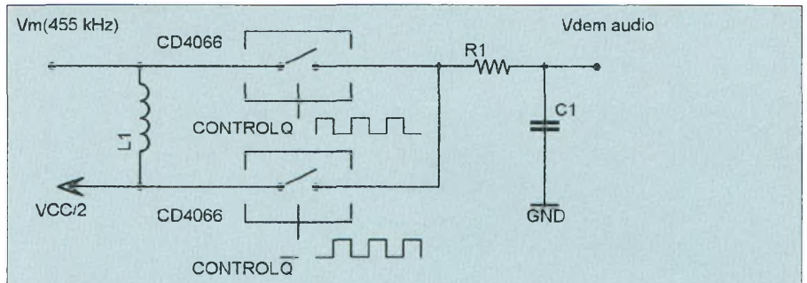
Simplified demodulator U.Rhode from reference 5
