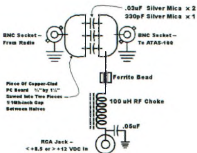
DC Coupler for Yaesu ATAS-100 1.8 - 450 MHz WA8LMF 28 Dec 1999
