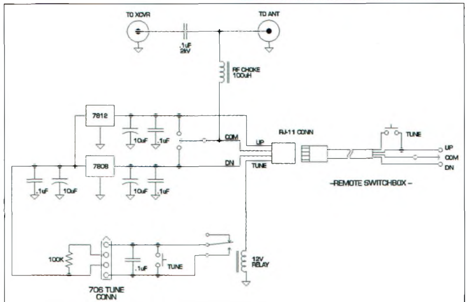
DC Coupler for Yaesu ATAS-100 1.8 - 450 MHz WA8LMF 28 Dec 1999
