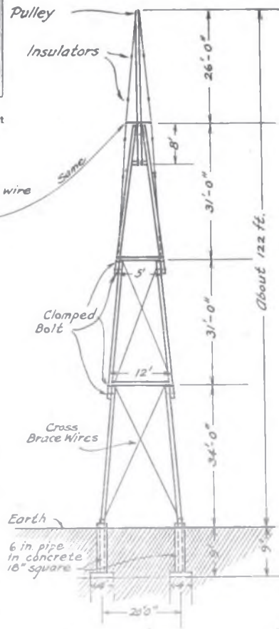
By comparing the photo and the working drawing an excellent idea of the construction of this tower may be gained.
