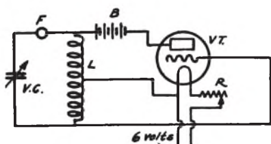
V.C.—Variable Cond max. capacity 0.00025 mfd. L—40 turns No. 20 wire on 3/2" diameter tube, with top in the center. B—Small, 22 1/2 volt "B" battery. V.T.—Amplifier tube. R—Rheostat. F—Flashlamp bulb.
