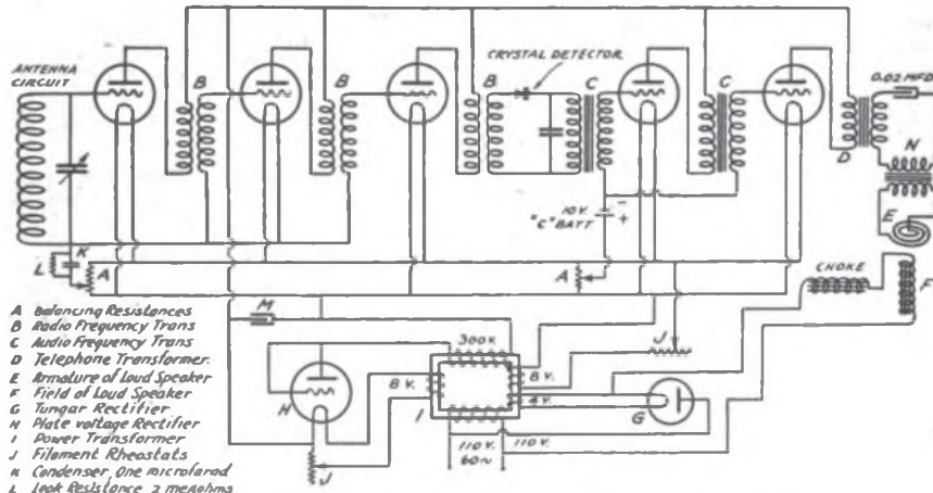
Fig 5 Final Complete Circuit of Five-Stage Amplifier using Crystal Detector Using 60 cycle alternating current to supply power for the filaments and plates.
