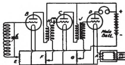
Fig. 1 Two-Stage Amplifier Circuit, using Tube Detector
