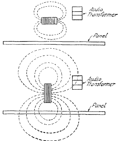
Keep the diameter small. The coil will then..... have less field.
