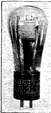
THE NEW UX-210. A HIGH POWER AMPLIFIER AND A 7.5 WATT OSCILLATOR
