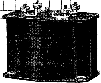
No. 3—A Transformer Ratio 4 to 1 Primary reactance, 125,600 ohms at 1000 cycles. Low core losses, thin laminations. Compact dimensions for sub panel or base board mount- ing. 2 3/4" long, 1-15/16" wide, 2-3/16" high. Shell type shielding. PRICE $4.50
