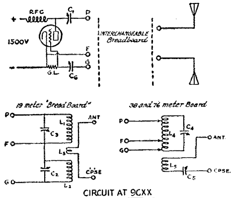
CIRCUIT AT 9CXX
