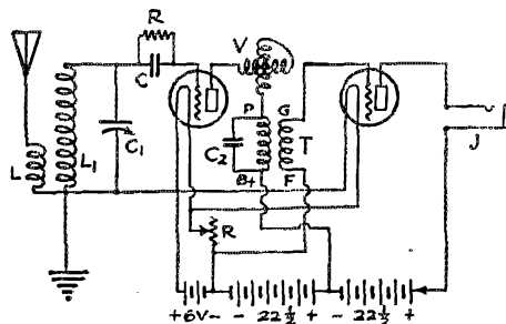
THE CIRCUIT
