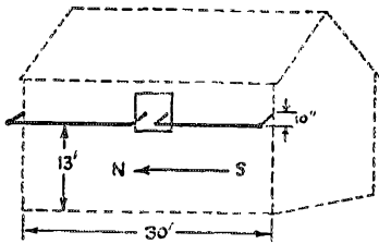
HORIZONTAL COLLECTOR
