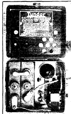
THE EXIDE A BATTERY WITH TICKLE CHARGER AND MASTER SWITCH. THERE IS ALSO A 6 VOLT TYPE.
