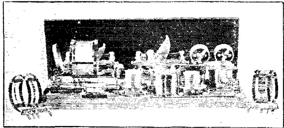
Fig. 3. Rear view of the receiver. Note plug-in grid leak and condenser and cushioned detector socket.
