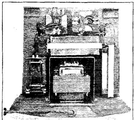
FRONT VIEW OF 6025B WESTERN ELECTRIC AMPLIFIER WITH SELF-CONTAINED CURRENT SUPPLY. On the shelf are the rectifier and amplifier tube. Underneath the shelf are resistances and a condenser belonging to the filter system.
