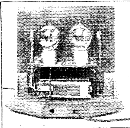
REAR VIEW OF THE WESTERN ELECTRIC 6025B AMPLIFIER AND CURRENT SUPPLY SET. At the lower center is the transformer supplying both the filament and the plate circuit. To the right and immediately above are condensers of the filter system. At the extreme left is a choke.
