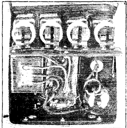
INTERNAL VIEW OF THE "PHILCO SOCKET POWER B" SEEN FROM ABOVE.
