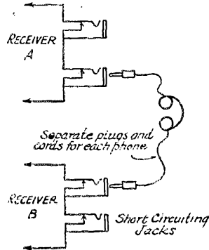
SIMPLE PLUG-JACK TRANSFER DUPLEX-TWO PHONES
