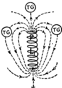
FIG. 3 PLOTING FIELD ABOUT PLATE COIL
