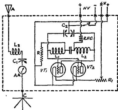
CIRCUIT DIAGRAM OF THE TRANSMITTER
