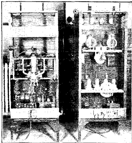
FIG. 2 REAR VIEW OF POWER PANEL AND 100-WATT TRANSMITTER
