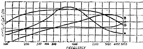
CURVES OF REPRESENTATIVE TRANSFORMERS UNDER NORMAL CONDITIONS
