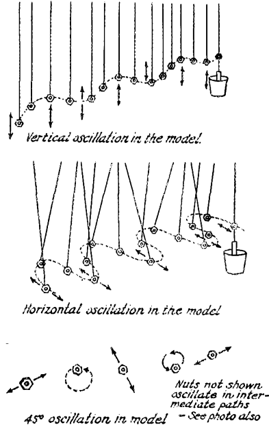
FIG. 7 EFFECT OF SENDING VARIOUS KINDS OF WAVES ALONG THE MECHANICAL ETHER-MODEL
