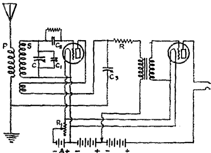
FIG. 1. THE CR-18 CIRCUIT C—Maximum of 130 \mu fd. C1—Vernier of 3 \mu fd. maximum capacity. C2—40 \mu fd. C3—220 \mu fd. R—25,000 ohms. R1—10 ohms.
