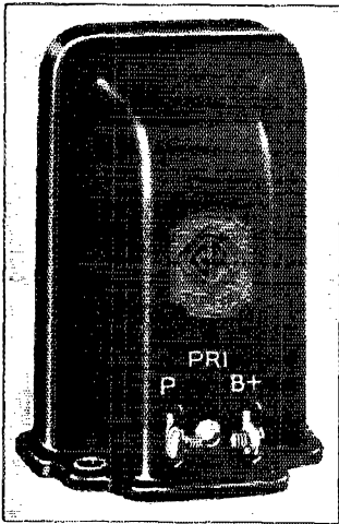
Transformers C. and D.—Modern "flat core" transformer used in making the C and D curves. C is general Radio Type 285L, having a turn ratio of 2:1 which D is type 285, having a turn ratio of 8:1.
