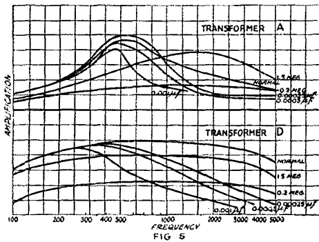
FIG 5 A GROUP OF CURVES SHOWING THE EFFECT OF SHUNTING VARIOUS DEVICES ACROSS THE TRANSFORMER SECONDARY
