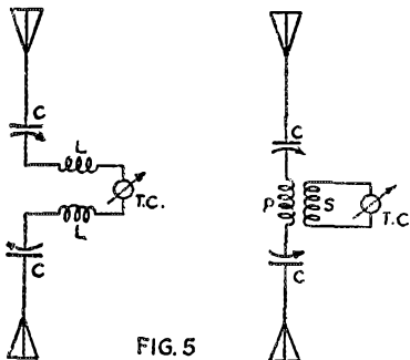
CIRCUIT OF THE EXPLORING ANTENNAS T.G. Thermo galvanometer. C.C. Tuning condensers.
