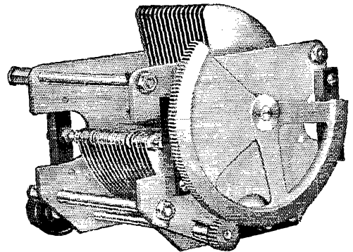
THE GENERAL RADIO TYPE 239 LABORATORY CONDENSER WHICH IS SUPPLIED WITH A CALIBRATION CHART
