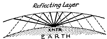
THE RADIANT RAY THEORY FIG. 2
