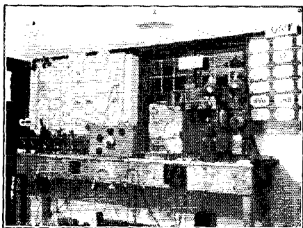
THE LAYOUT AT O-A6N, THE STATION OF MAJOR SWART AT MILNERTON, SO. AFRICA
