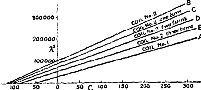
FIG. 4. MATCHING COILS
