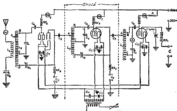
FIG. 1. THE CIRCUIT
