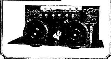
Front view of CR-18 with 200 meter coil intake and additional coils for 10, 20, 40 and 80 meter bands.
