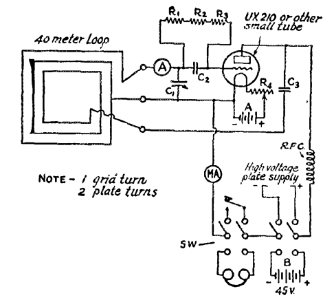
FIG. 1. THE CIRCUIT OF THE TRANSCIEVER C1—Bremer-Tully tuning condenser. A capacity of 250 \mu fds is enough. C2 & C3, grid and plate stopping condensers, 2000 \mu fds each. R1, R2 & R3—Bradleyohm resistance used as grid leak. R4—Filament rheostat. A—General Radio 0-2 hot wire ammeter. Ma.—Jewell 0-100 plate milliammeter. R.F.C.—R.F. choke coil, 50-100 turns on 3\frac{1}{2} " tube. Sw.—Four-pole, double-throw camswitch.
