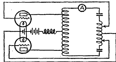
B - BALANCED HARTLEY PLATE & GRID DIRECT COUPLED
