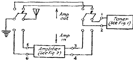
FIG. 2 THE SWITCHING ARRANGEMENT USED. NO SPECIAL CLAIMS ARE MADE FOR IT
