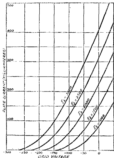
FIGURE 7. STATIC GRID VOLTAGE-PLATE CURRENT CURVES WITH DIFFERENT PLATE VOLTAGES
