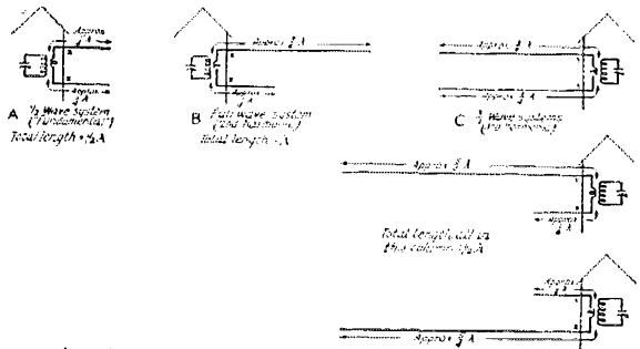
NOTE—Losses tend to be high at points X unless they are near voltage node. Antenna forms shown are general and external parts may be slanting or vertical.
