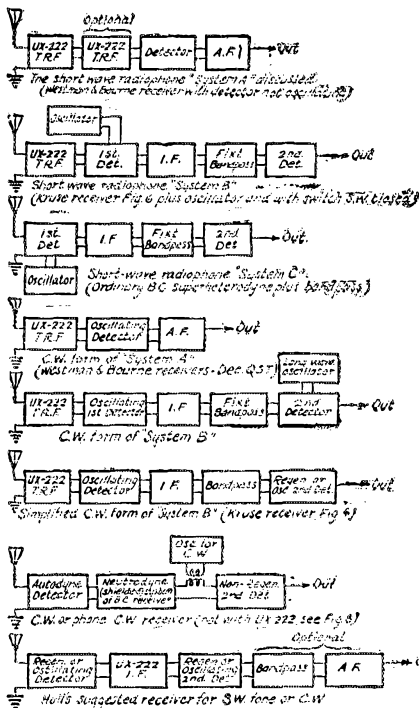
FIG. 9. THE VARIOUS RECEIVER SYSTEMS DISCUSSED
