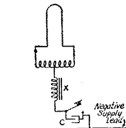
X = 30 Henry "B" eliminator choke C = 2 \mu f paper condenser
