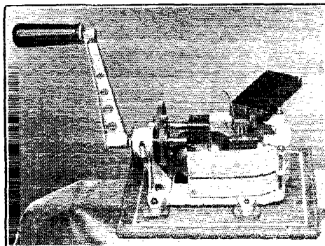
THE "POWER PLANT" REMOVED FROM ITS CASE AND WITH THE SMOOTHING CONDENSER DISCONNECTED TO PERMIT SHOWING THE BRUSHING AND ARMATURE.
