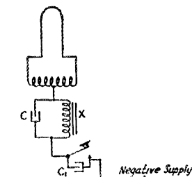
X = 30 Henry "B" eliminator choke C = 2 \mu f paper condenser C 1 = "bum" 1 \mu f paper condenser
