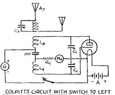
COLPITTS CIRCUIT WITH SWITCH TO LEFT
