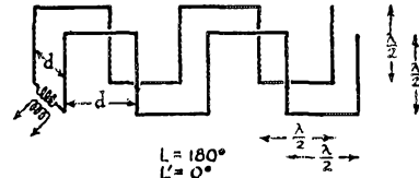
FIG. 25. ENDWISE DOUBLE-ROW GROUP, FOR SHARPENING THE BEAM ABOVE THAT OF FIG. 24
