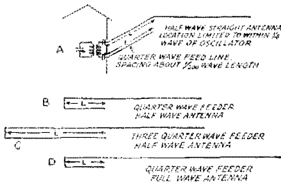
FIG. 3. VOLTAGE FEED BY MEANS OF A NON-RADIATING 2-WIRE LINE
