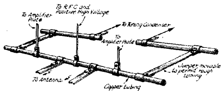
FIG. 3. THE PLATE "TANK" OF THE 20-Kw. 21,000 Kc. EXPERIMENTAL TRANSMITTER
