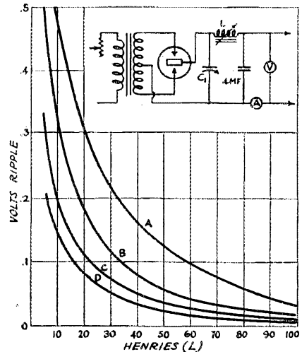
FIG. 5. THE EFFECT ON THE OUTPUT RIPPLE OF A SINGLE SECTION FILTER WHEN VARYING C_1 AND L_1
