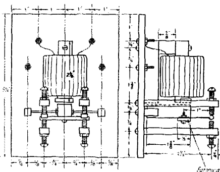
FIG 3. LARGE KEYING RELAY
