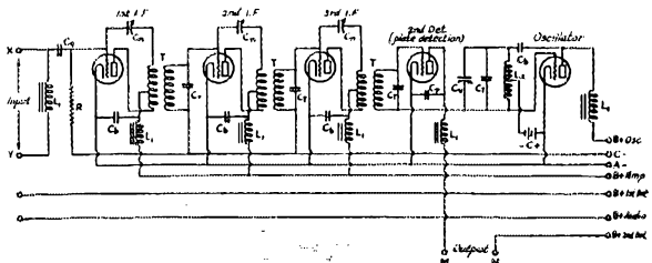
FIG. 2. THE INTERMEDIATE FREQUENCY AMPLIFIER, 2ND. DETECTOR AND LONG-WAVE HETERO-DNYE OSCILLATOR
