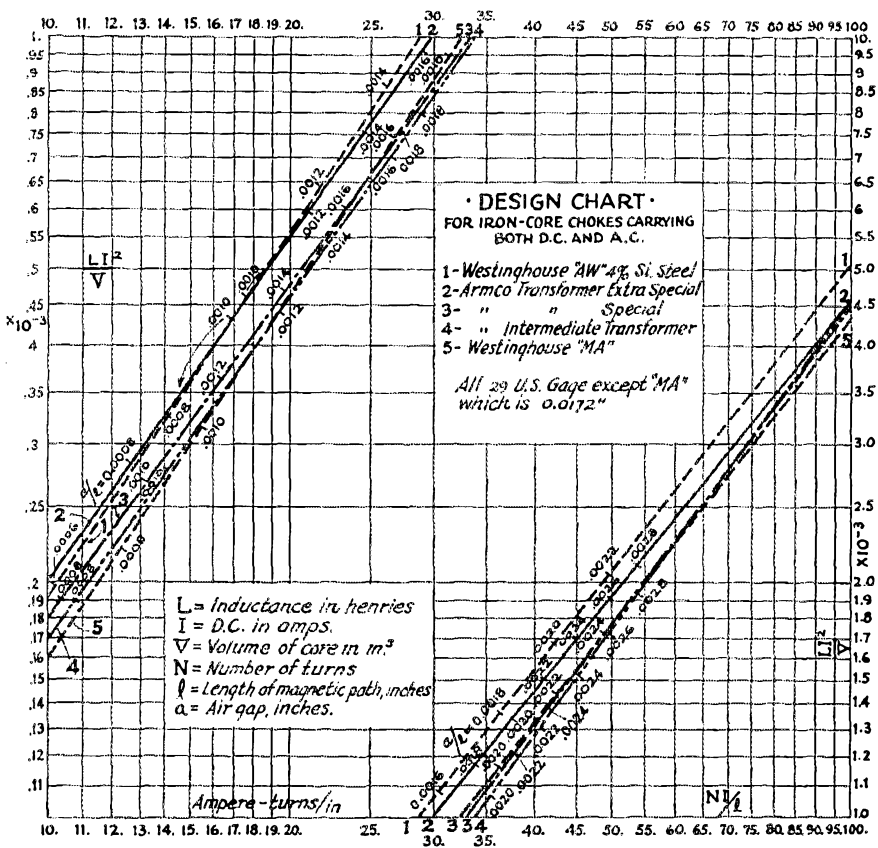
THE CURVES ARE REALLY CONTINUOUS BUT HAVE BEEN CLIPPED IN HALF TO MAKE THE CHART MORE CONVENIENT IN SIZE Use the curves on the left side for values between .1 and 1.0 and the right hand curves for values between 1.0 and 10.
