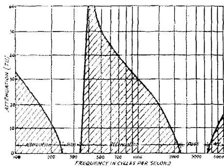
FIG. 6. CHARACTERISTICS FOR THE L-SECTION ACOUSTIC FILTER SHOWN IN FIG. 4
