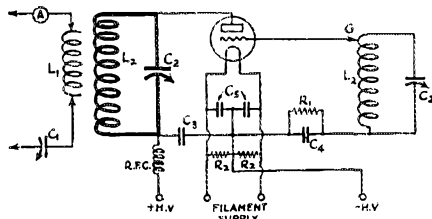
FIG. 9. SHOWING SIMILAR MODIFICATION OF THE TUNED-GRID TUNED-PLATE CIRCUITS. The grid clip "G" is provided to permit effective adjustment of grid excitation. The letters correspond to those of Fig. 8.
