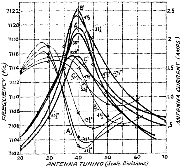
FIG. 2. PROVIDING SOME INDICATION OF THE INSTABILITY ACCOMPANYING LOW VALUES OF GRID EXCITATION
