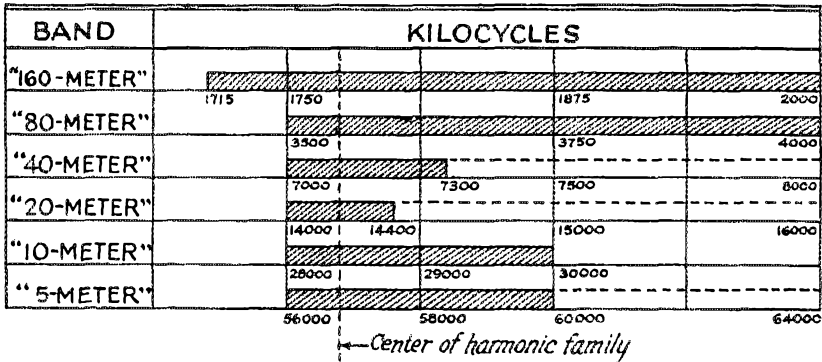
SHOWING RELATIVE WIDTHS OF 1929 AMATEUR BANDS FIG. 5
