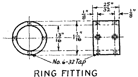
FIG. 4. DIMENSIONS OF THE MOUNTING UNITS TO CONNECT FOUR CONDENSERS IN PARALLEL
