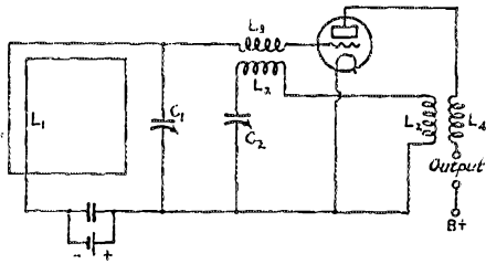
FIGURE 1. THE DIAGRAM OF THE COMBINED DETECTOR-OSCILLATOR
