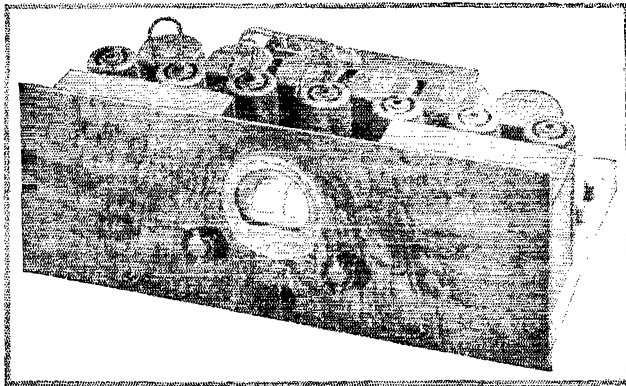
Tyrman "80" full A-C Socket operation using (3) A-C Shielded Grid (4) 327 (2) 381 (1) 350 or 310 Tubes. Dimensions 8" x 21" x 11½". One Spot-10 K. C. Separation. "The year ahead receiver."
