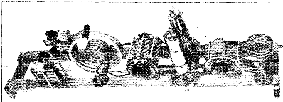
THE 100-WATT PUSH-PULL, TUNED-GRID, TUNED-PLATE TRANSMITTER
