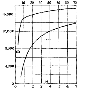
INDUCTION CURVE OF FOLLANSBEE SHEETS FIGURE 7
