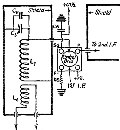
FIGURE 12. THE WIRING OF THE FIRST INTERMEDIATE-FREQUENCY STAGE
