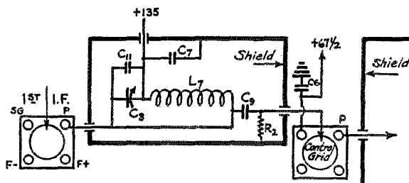
FIGURE 13. APPARATUS OF THE SECOND INTERMEDIATE STAGE CONTAINED IN THE SHIELD SEEN AT THE REAR CENTER OF THE BASE-BOARD
