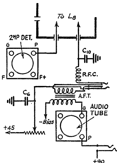
FIGURE 18. THE APPARATUS OF THE SECOND DETECTOR AND AUDIO AMPLIFIER, LOCATED AT THE RIGHT FRONT OF THE RECEIVER, DETAILED IN THIS DIAGRAM
