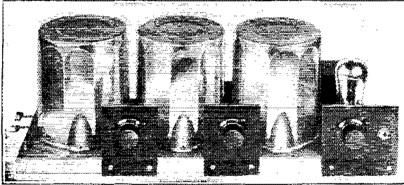
FIGURE 5. AN EXPERIMENTAL SCREEN-GRID-TUBE AMPLIFIER
