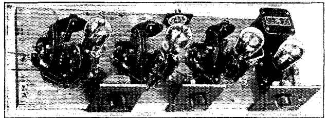
FIGURE 6. THE SCREEN-GRID AMPLIFIER WITH THE SHIELDS REMOVED
