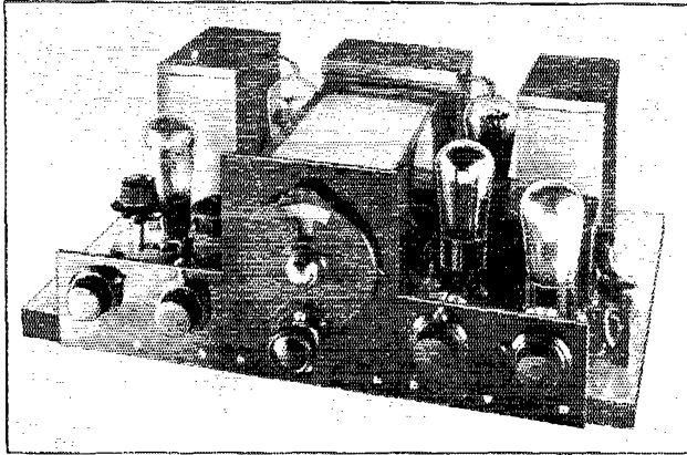
THE COMPLETE SUPER-HETERODYNE AWAITING AN OPPORTUNITY TO RUCKLE UP A FEW LOUD-SPEAKER DIAPHRAMS
