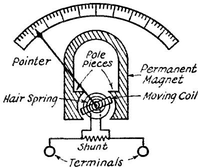
FIG. 3.—THIS SHOWS THE METHOD BY WHICH THE D'ARSONVAL MOVEMENT IS APPLIED TO THE MEASUREMENT OF CURRENT
