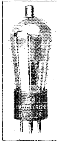
THE UX-245, AN A.C. SCREEN-GRID TUBE
