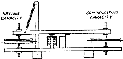
FIG. 1 — COMPENSATED KEYING
