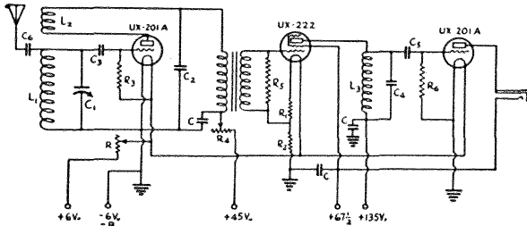
FIG. 3. — THE RECEIVER
