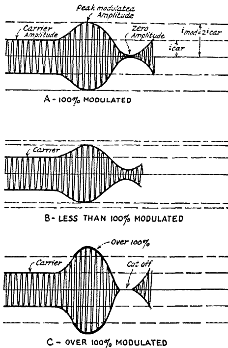
FIG. 4. — THE WAY THE MODULATED CARRIER WOULD LOOK
