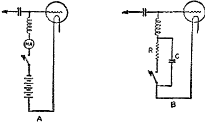
FIG. 3—MINIMIZING KEY THUMPS
