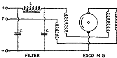
FIG. 4.—THE GENERATOR AND FILTER CIRCUIT
