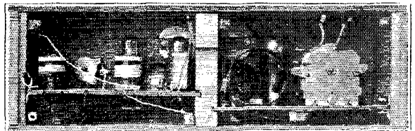
A REAR VIEW OF THE SET WITH THE BACK OF THE CABINET REMOVED
