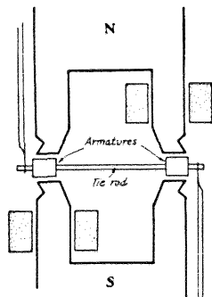
FIG. 2.—THE ARRANGEMENT BY WHICH THE ARMATURE IS ALLOWED TO "FLOAT" WITHIN THE GAP BETWEEN OPPOSING POLE PIECES AND STILL NOT MOVE IN A DIRECTION THAT WILL ALTER THE LENGTH OF THE GAPS AS INDICATED HERE
