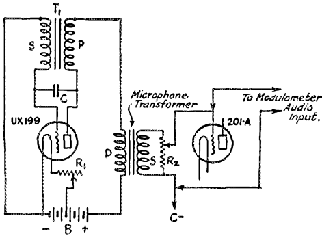
FIG. 2.—THE SIGNAL GENERATOR
