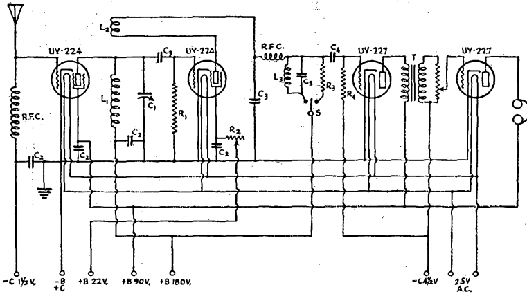
FIG. 2.—ANOTHER ARRANGEMENT USING TWO AUDIO STAGES WITH THE FILAMENTS OF ALL TUBES IN PARALLEL
