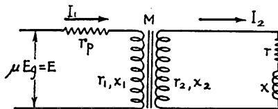
FIG. 2. — EQUIVALENT CIRCUIT OF THAT SHOWN IN FIG. 1
