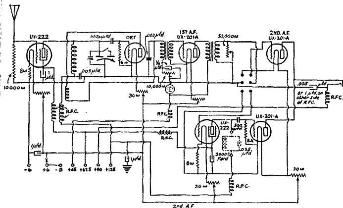
FIG. 1.— WIRING DIAGRAM OF THE RECEIVER AT WIAOF Details of this receiver were published in the December, 1929, QST.
