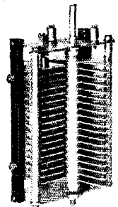
T199—A super transmitting condenser. Cap. .00033. Air-gap— 3/32 " measured from stator to adjacent rotor.
