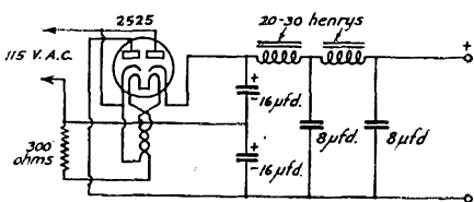
VOLTAGE DOUBLING
