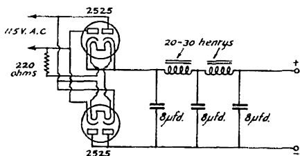
FULL WAVE
