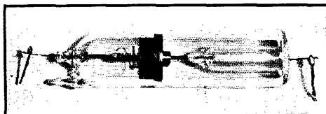
THE HOME-MADE VACUUM TYPE CRYSTAL MOUNTING
