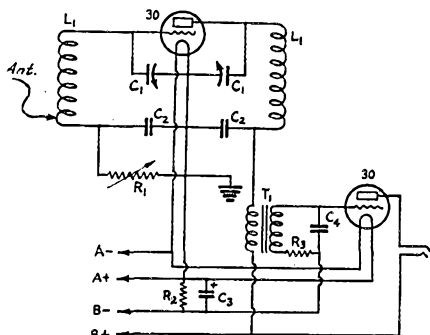
FIG. 3—THE CIRCUIT
