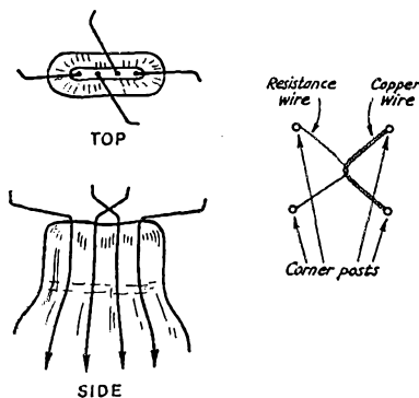
FIG. 3 — HOW THE R.F. THERMOCOUPLE IS MADE
