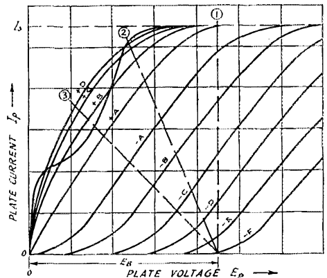
FIG. 4—TYPICAL PLATE CHARACTERISTICS
