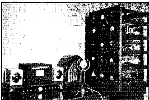
GENERAL VIEW OF W7VS, SHOWING THE TRANSMITTER AT THE RIGHT, FACING THE OPERATING POSITION, WITH THE CONTROL PANEL LOCATED DIRECTLY UNDER THE E.C. FREQUENCY METER, RECEIVER, AND THE DOUBLET ANTENNA TUNER
