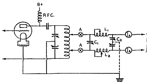
FIG. 2—THE BALANCED ARRANGEMENT FOR TWO-WIRE ANTENNA FEED
