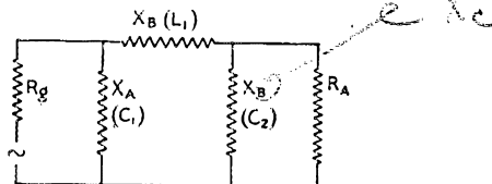
FIG. 3—EQUIVALENT CIRCUIT OF THE IMPEDANCE-MATCHING NETWORK
