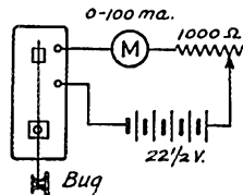
THE CIRCUIT USED FOR BUG ADJUSTMENT
