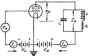
FIG. 6—THE R.F. POWER AMPLIFIER CIRCUIT UNDER CONSIDERATION
