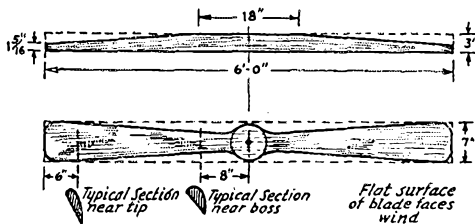
FIG. 2 — IMPELLER CONSTRUCTION
