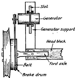
TOP VIEW SHOWING METHOD OF SUPPORTING GENERATOR
