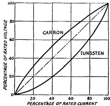
FIG. 2 — FROM THESE CURVES IT IS POSSIBLE TO DETERMINE THE VOLTAGE REQUIRED TO CAUSE A GIVEN CURRENT TO FLOW IN EITHER CARBON OR TUNGSTEN LAMPS PROVIDED THE CURRENT AT RATED VOLTAGE IS KNOWN
