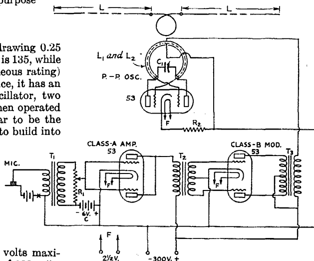
FIG. 1 — CIRCUIT FOR 53'S USED AT WIQP
