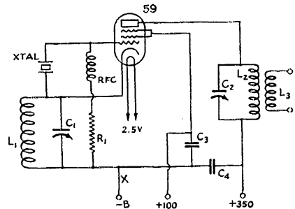
FIG. 1—CIRCUIT OF THE SINGLE-TUBE CRYSTAL TRANSMITTER
