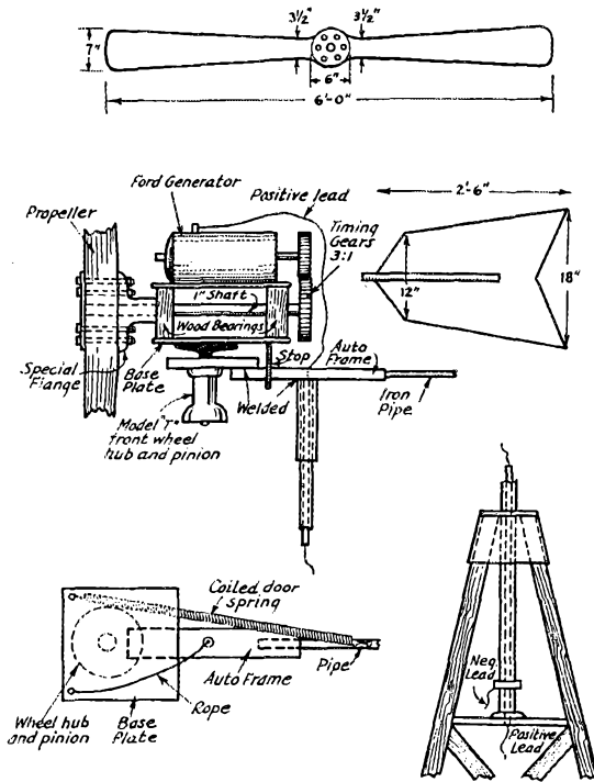
FIG. 1 — DETAILS OF THE W9BW WIND CHARGER The drawing is not to scale. See text for further details.
