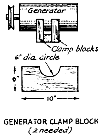
FIG. 3—CONSTRUCTION OF THE WIND-DRIVEN CHARGER BUILT BY RODNEY C. MITCHELL The drawing is not to scale.
