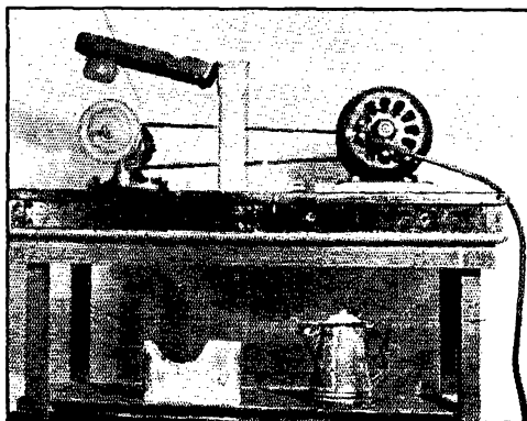
CRYSTAL CUTTING RIG BUILT BY THE AUTHOR AND WIGF
