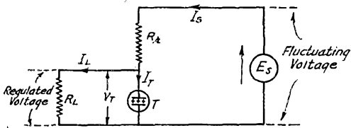
FIG. 2—THE EQUIVALENT CIRCUIT OF THE VOLTAGE REGULATOR
