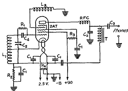
FIG. 5 — ELECTRON-COUPLED FREQUENCY-METER MONITOR USING 2A7 TUBE
