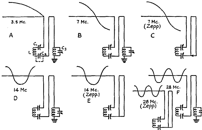
FIG. 6—CONTROLLED-RADIATION OR CONVENTIONAL ZEPP CONNECTIONS FOR OPERATION ON VARIOUS AMATEUR BANDS, WITH VOLTAGE CURVES SHOWN FOR THE HORIZONTAL SECTION
