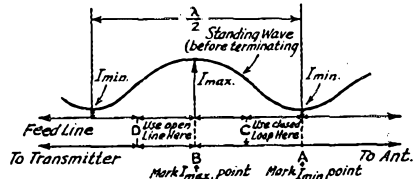
FIG. 25—SHOWING THE TWO POINTS D OR C AT WHICH THE AUXILIARY OPEN LINE OR CLOSED LOOP MAY BE PLACED (POINT D TAKING THE LINE AND POINT C THE LOOP), AND CALCULATIONS SHOWING THE RESPECTIVE DISTANCES FROM POINTS OF MINIMUM AND MAXIMUM CURRENT ALONG THE LINE AS DETERMINED BY THE MEASURING DEVICE (SEE TEXT) IN TERMS OF \lambda AND LENGTH OF AUXILIARY LINE OR LOOP TO BE USED
