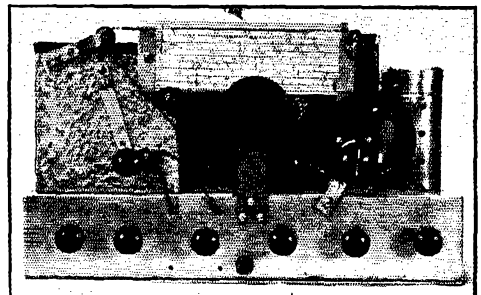
FRONT VIEW OF THE TURRET-TUNED RECEIVER CHASSIS
