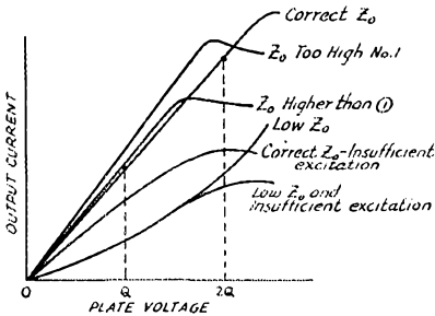
FIG. 2—ILLUSTRATING THE MANNER IN WHICH EXCITATION AND LOAD IMPEDANCE AFFECT THE LINEARITY OF THE CLASS-C MODULATING STAGE
