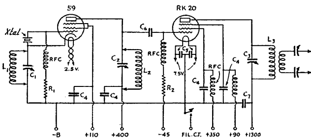
FIG. 1—CIRCUIT DIAGRAM OF THE TWO-STAGE PENTODE TRANSMITTER
