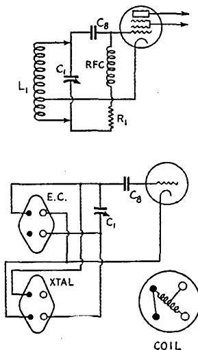
FIG. 2—ALTERNATIVE OSCILLATOR GRID CIRCUIT CONNECTIONS FOR SELF-CONTROLLED OPERATION
