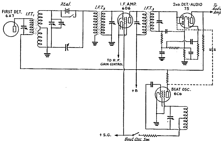
FIG. 1—SCHEMATIC ARRANGEMENT OF THE SINGLE-STAGE I.F. AMPLIFIER USING IRON-CORE TRANSFORMERS
