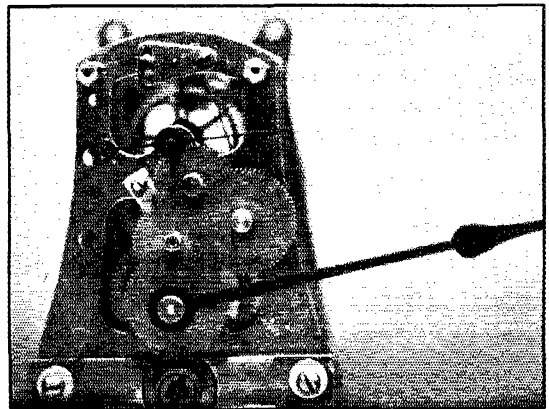
A CLOSE-UP OF THE HOUR-HAND GEAR ARRANGEMENT IN W7AVM'S CLOCK
