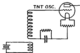
FIG. 5—TNT CIRCUIT WITH CRYSTAL LOCK
