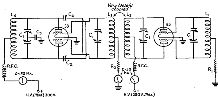
FIG. 1—CIRCUIT OF THE SIMPLE OSCILLATOR-AMPLIFIER TRANSMITTER
