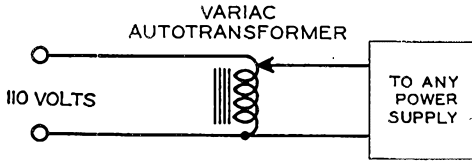
THE CIRCUIT
