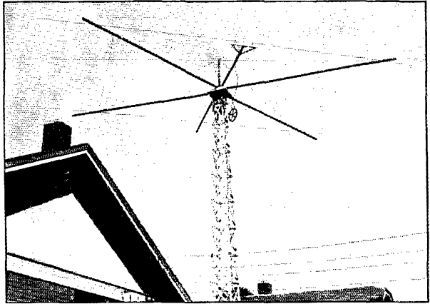
THE ROTABLE 14-MC. SIGNAL SQUIRTER MOUNTED ON ITS 31-FOOT LATTICE TOWER IS CONTROLLED FROM A CRANK RIGHT AT THE OPERATING POSITION IN THE SHACK. IT NOT ONLY GIVES REAL GAIN IN TRANSMISSION BUT ALSO LESSENS INTERFERENCE CORRESPONDINGLY WHEN USED FOR RECEPTION
