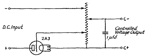
FIG. 2—TRIODE SERIES REGULATOR FOR CLOSE CONTROL OF CLASS-B AMPLIFIER BIAS
