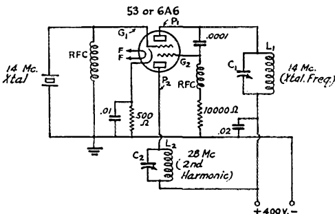
FIG. 3.—TWIN-TRIODE DOUBLER CIRCUIT
