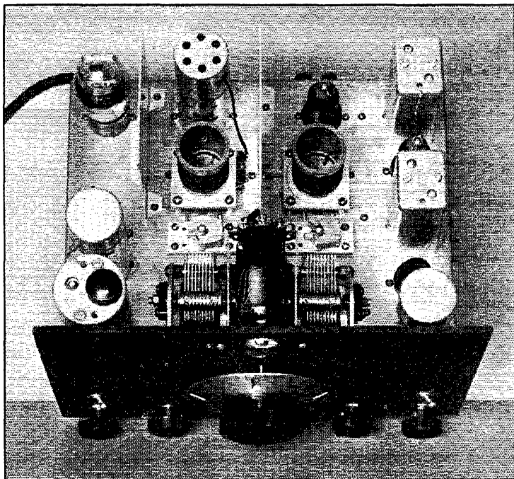
A TOP VIEW, SHOWING THE LAYOUT OF COMPONENTS The physical arrangement is discussed fully in the text.
