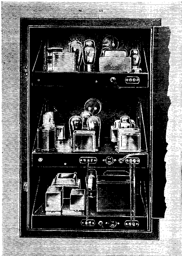
REAR VIEW SHOWING CONSTRUCTION AND PARTS
