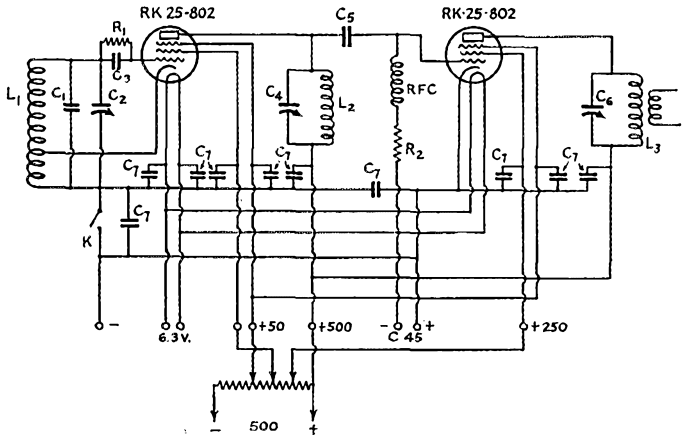
FIG. 1—CIRCUIT OF THE ELECTRON-COUPLED EXCITER UNIT
