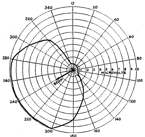
FIELD CHART OF W6JN ANTENNA
