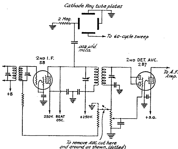
FIG. 1—METHOD OF CONNECTING THE CATHODE-RAY TUBE TO THE SECOND OR THIRD I.F. STAGE OF A TYPICAL SUPERHET
