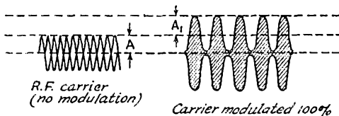
FIG. 2—TYPES OF PATTERNS OBTAINED ON 'PHONE SIGNALS
