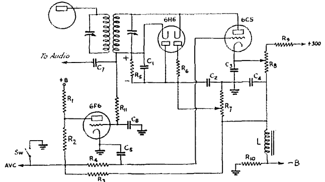
FIG. 2—AUTOMATIC SILENCER CIRCUIT WITH AMPLIFIED AVC
