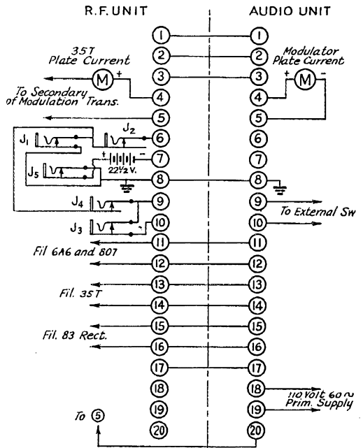
FIG. 3—TERMINAL CONNECTIONS
