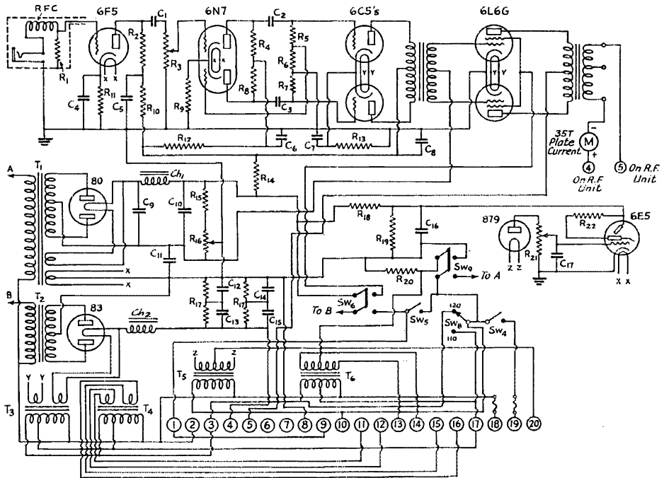
FIG. 2—THE AUDIO SECTION
