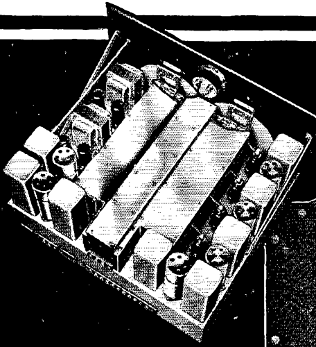
STANDARD 'SUPER-PRO' RECEIVER CHASSIS
