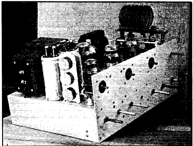
THE R.F. UNIT REMOVED FROM THE FRAME
