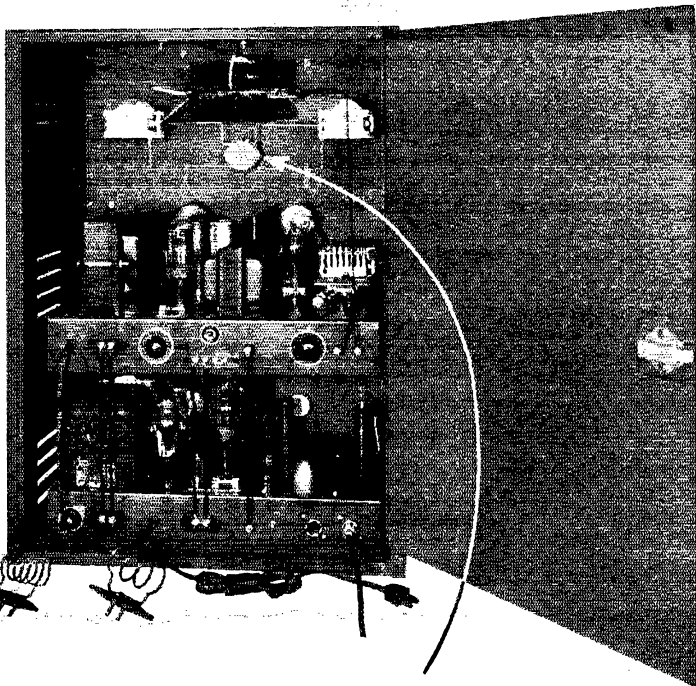
Centralab Antenna Matching Switch on 5B 40W Transmitter made by WHOLESALE RADIO of New York, N. Y.
