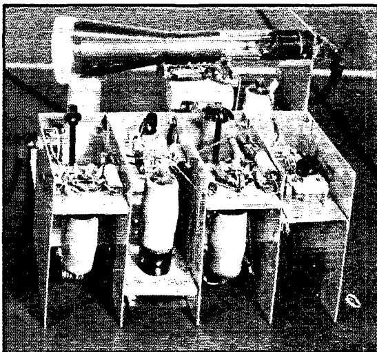
SHOWING THE R.F. SECTION OF THE SIMPLE RECEIVER
