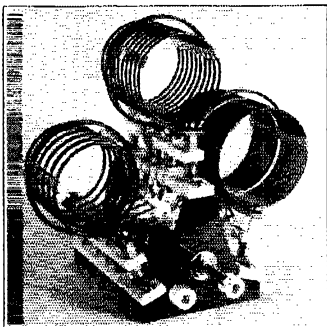
3 Band Switching Turret using Centralab Isolantite Switch made by BARKER and WILLIAMSON Ardmore, Pa.
