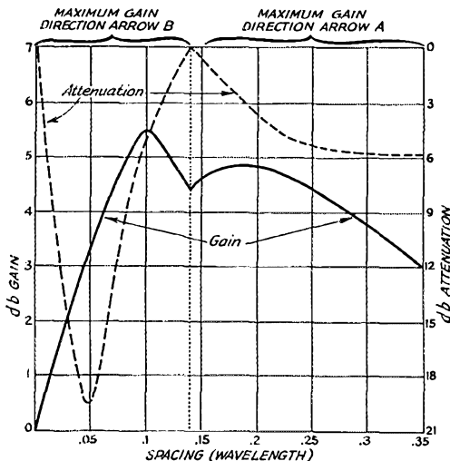
FIG. 5—FORWARD GAIN AND BACKWARD ATTENUATION FOR A HALF-WAVE ANTENNA WITH A SINGLE PARASITIC ELEMENT, AS A FUNCTION OF SPACING
