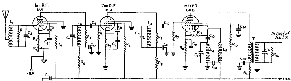
FIG. 1—THE CIRCUIT OF THE TWO R.F. STAGES AND MIXER OF THE SUPERHET RECEIVER
