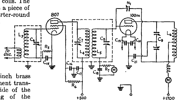
FIG. 2—THE TRANSMITTER CIRCUIT DIAGRAM C 6 , C 7 , C 8 —25- \mu fd. variable, 2000-volt spacing. C 9 , C 10 —35- \mu fd. per section split-stator variable, 3000-volt spacing (Cardwell NF-35-ND). C 11 —44- \mu fd. per section split-stator variable, 1/2" spacing (Atkins-Brown ABC445). C 12 —100- \mu fd. variable, 0.2" spacing (Cardwell XC-100-XS). C 13 , C 14 —100- \mu fd. receiving-type variable (Hammarlund MC-100-S). C 16 , C 19 , C 17 —0.01- \mu fd. 600-volt paper. C 18 —0.006- \mu fd. receiving type mica.
