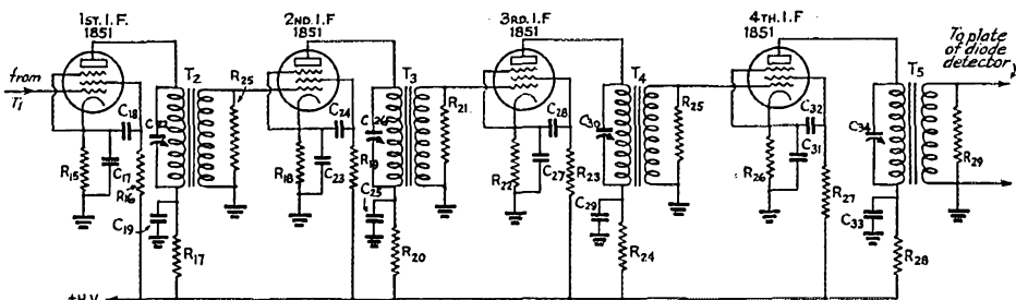
FIG. 2—THE COMPLETE CIRCUIT OF THE I.F. AMPLIFIER
