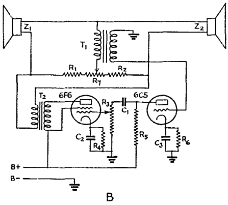
FIG. 3—LOUDSPEAKER SYSTEM REQUIRING NO SWITCHING
