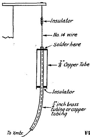
Fig. 4—The 5-meter coaxial antenna built by W8PK, using materials easily available to the average amateur. This antenna gave a good account of itself as compared to a rotary beam.
