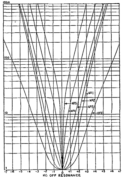
Curves for Crystal Filter
