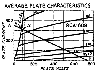
Fig. 3—809 plate-voltage plate-current family, showing load line.
