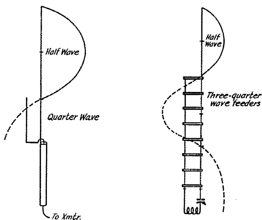
Fig. 2 — The "J" antenna, showing a "net" standing wave on the matching section, because of current or phase unbalance. Radiation from the matching section will tend to raise the angle of radiation.
