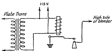
Fig. 4 — Circuit of gravity-operated relay for shorting the output of the power supply when the primary power is cut off, thus ensuring the discharge of filter condensers.
