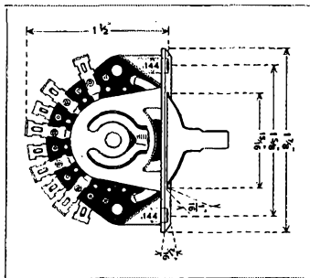
Contact clips of spring brass heavily plated (silver) treated for easy soldering. Switching combinations available use up to 12 clips per section.
