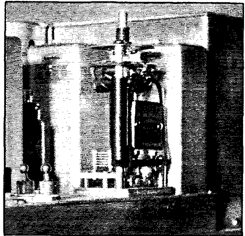
A close-up of the crystal unit, with the shield can be removed. The selectivity switch is mounted vertically, with its shaft projecting through the top of the shield.
