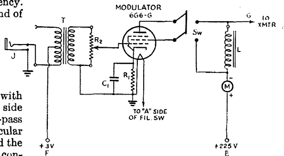
Fig. 4 — Modulator wiring diagram. C 1 — 25- \mu fd., 25-volt electrolytic. R 1 — 600 ohms, 1-watt. R 2 — 0.5-megohm potentiometer. J — Open circuit jack. T — D.h. mike to single-grid transformer (Stancor A-4708). L — Filter choke used as modulation choke (Stancor C-1002) (30 henrys, 50 ma., 400 ohms d.c. resistance). Sw — D.p.d.t. toggle switch. M — 0-50 milliammeter (Triplett).
