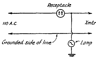
Fig. 1—The series plug on page 43 of QST for April fitted with a lamp indicating when the series plug is in the ungrounded side of the line as it should be.
