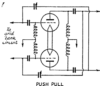
Fig. 5—In certain cases, it is feasible to remove d.c. voltages from the neutralizing condensers by using parallel feed in both grid and plate circuits.
