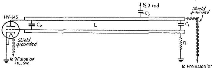
Fig. 6 — The transmitter circuit.
