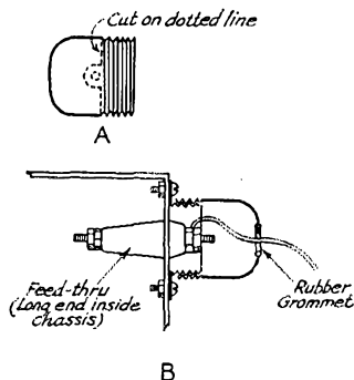
Fig. 2—Shield for exposed high-voltage chassis terminal made from Amphenol cable-connector shell. Insulation on the wire should be adequate for the voltage employed.
