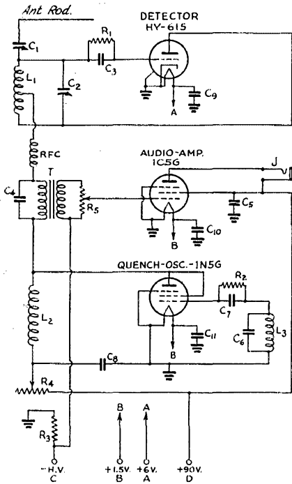
Fig. 3 — Circuit diagram of the receiving section. C 1 — 35- \mu fd. variable (Hammarlund HF-35). C 2 — 15- \mu fd. variable (National UM-15 with all but two plates removed). C 3 — 100- \mu fd. midget mica. C 4 — 0.005- \mu fd. midget mica. C 5 , C 6 — 0.002- \mu fd. midget mica. C 7 — 0.001- \mu fd. midget mica. C 8 — 0.1- \mu fd., 400-volt paper tubular. C 9 , C 10 , C 11 — 0.01- \mu fd., 400-volt paper tubular. R 1 — 5 megohms, \frac{1}{2} -watt. R 2 — 50,000 ohms, \frac{1}{2} -watt. R 3 — 1000 ohms, \frac{1}{2} -watt. R 4 — 0.1-megohm potentiometer. R 5 — 0.5-megohm potentiometer. RFC — 25 turns No. 20 d.s.c., diameter \frac{1}{4} inch, close-wound. J — Open-circuit jack. T — Audio transformer, 3:1 ratio (Stancor A-53). L 1 — 3 turns No. 14 tinned wire, diameter \frac{1}{2} inch, length \frac{3}{8} inch. L 2 , L 3 — Windings of National quench-oscillator unit.
