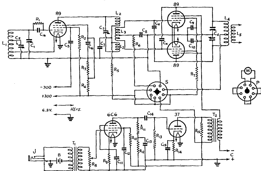
Fig. 1 — Circuit diagram of the low-cost 5-meter transmitter.
