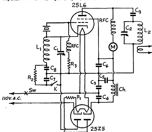
Fig. 1 — Complete circuit diagram.
