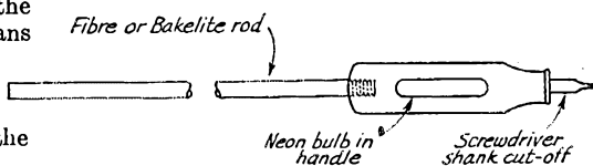
Fig. 4—Combination insulated screwdriver with neon-bulb indicator in the handle.
