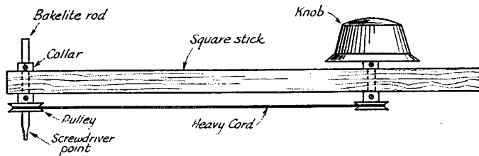
Fig. 3—Another gadget for adjusting neutralizing condensers with safety.
