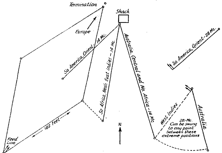
© The terminated rhombic for Europe at W6OCH is supplemented by five 8-element Sterba curtains for the other directions.
